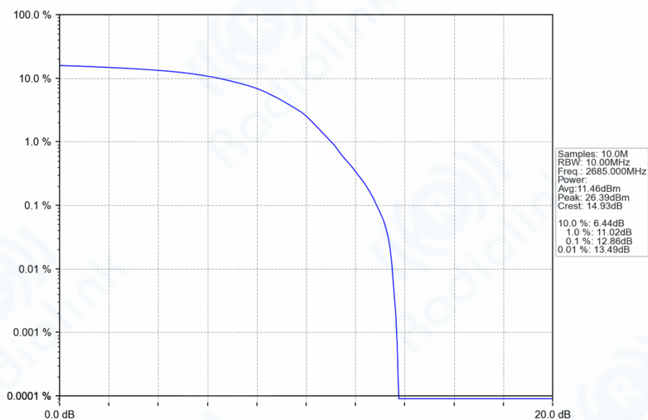
n41_30kHz_SISO_NTNV_10MHz_DFT-s-OFDM_64_QAM_2685MHz_Outer_Full_Ant1
