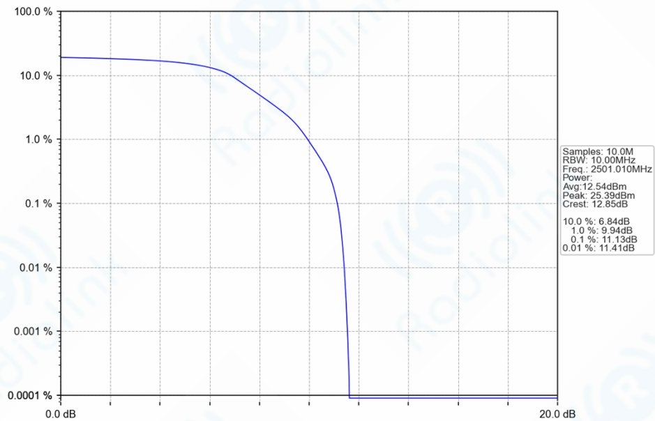
n41_30kHz_SISO_NTNV_10MHz_DFT-s-OFDM QPSK_2501.01MHz_Outer_Full_Ant1
