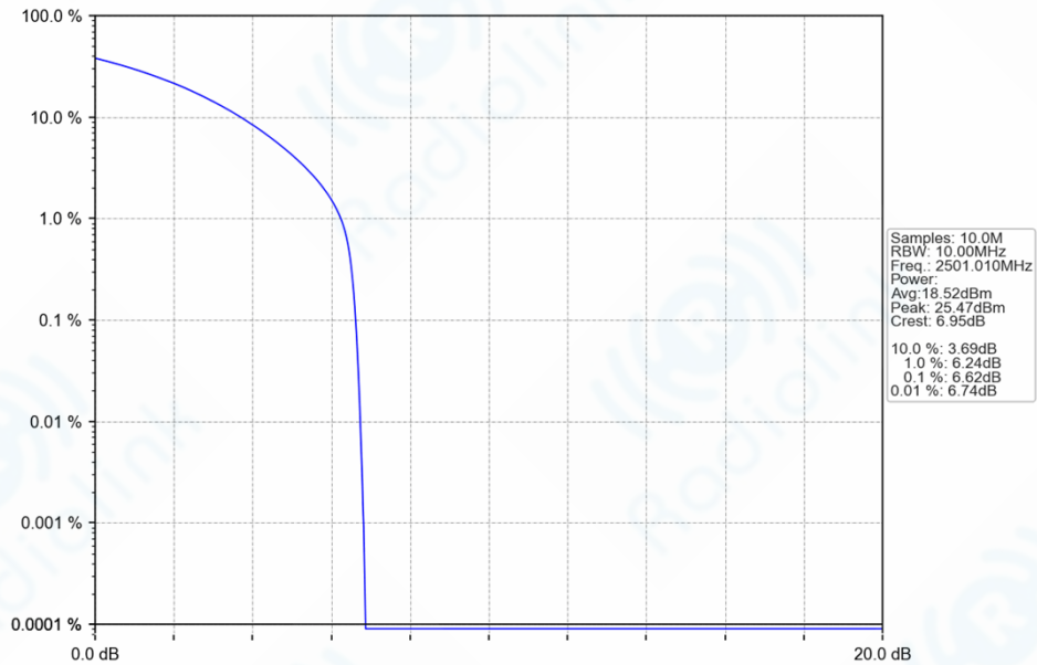
n41_30kHz_SISO_NTNV_10MHz_CP-OFDM_QPSK_2501.01MHz_Outer_Full_Ant1
