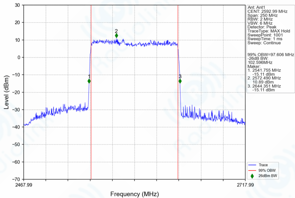
n41_30kHz_SISO_NTNV_100MHz_CP-OFDM_256_QAM_2592.99MHz_Outer_Full_Ant1
