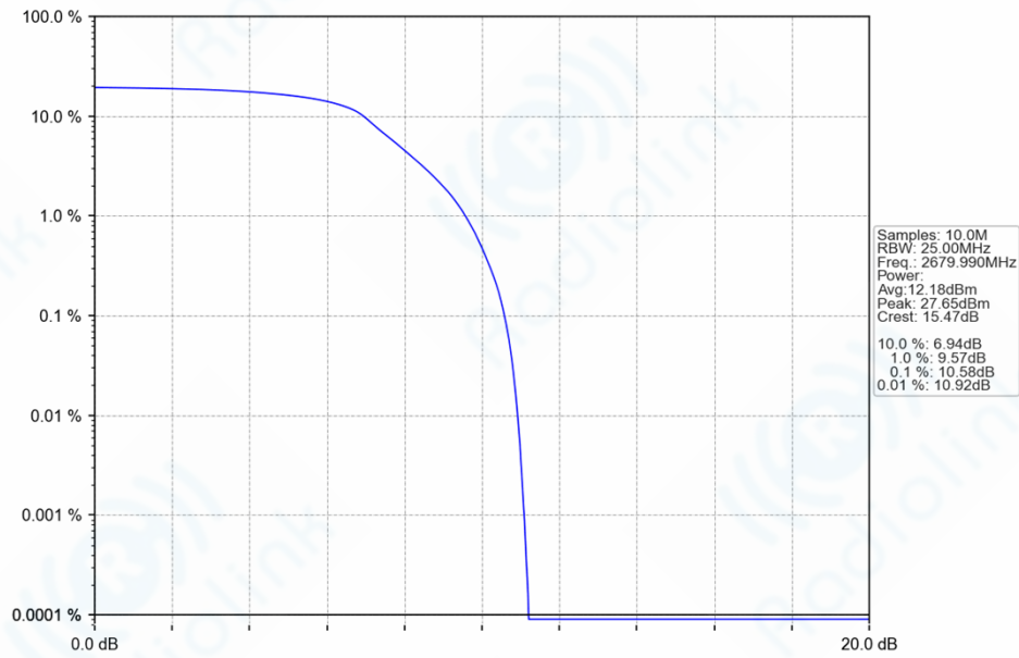
n41_30kHz_SISO_NTNV_20MHz_DFT-s-OFDM_PI/2_BPSK_2679.99MHz_Outer_Full_Ant1
