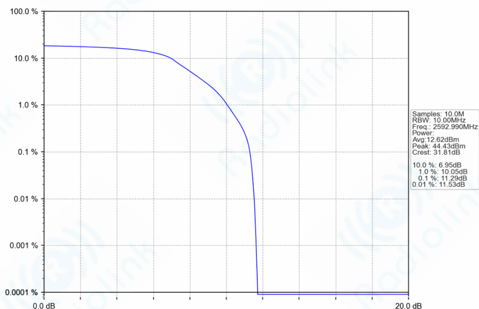
n41_30kHz_SISO_NTNV_10MHz_DFT-s-OFDM_QPSK_2592.99MHz_Outer_Full_Ant1
