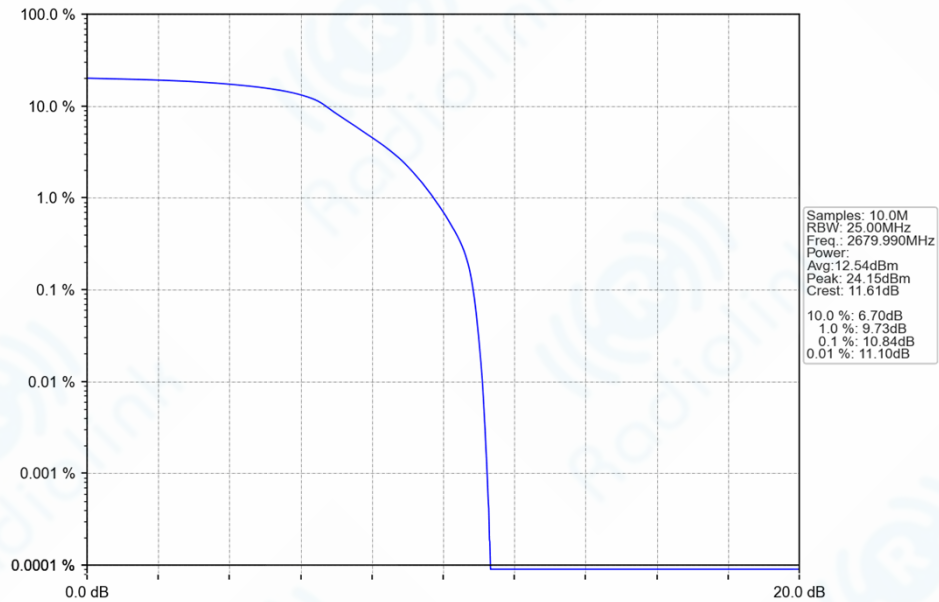
n41_30kHz_SISO_NTNV_20MHz_DFT-s-OFDM_QPSK_2679.99MHz_Outer_Full_Ant1
