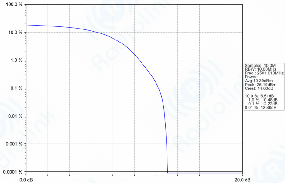
n41_30kHz_SISO_NTNV_10MHz_DFT-s-OFDM_64_QAM_2501.01MHz_Outer_Full_Ant1
