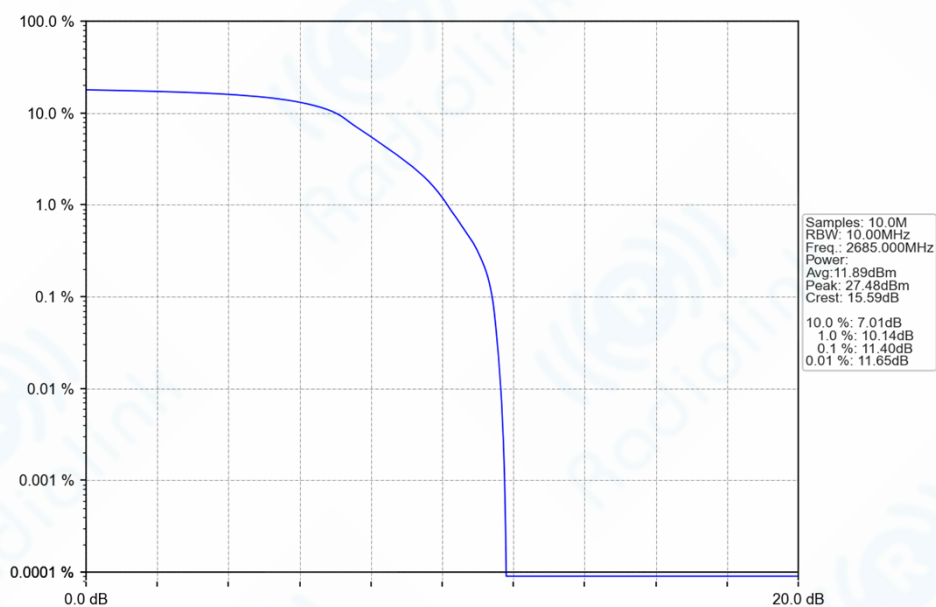
n41_30kHz_SISO_NTNV_10MHz_DFT-s-OFDM_QPSK_2685MHz_Outer_Full_Ant1
