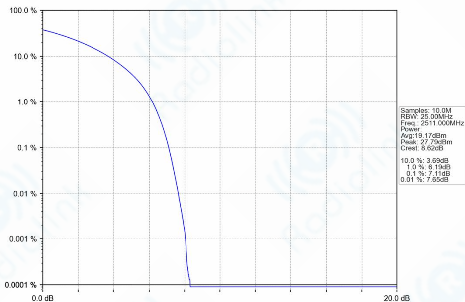
n41_30kHz_SISO_NTNV_30MHz_CP-OFDM_QPSK_2511MHz_Outer_Full_Ant1
