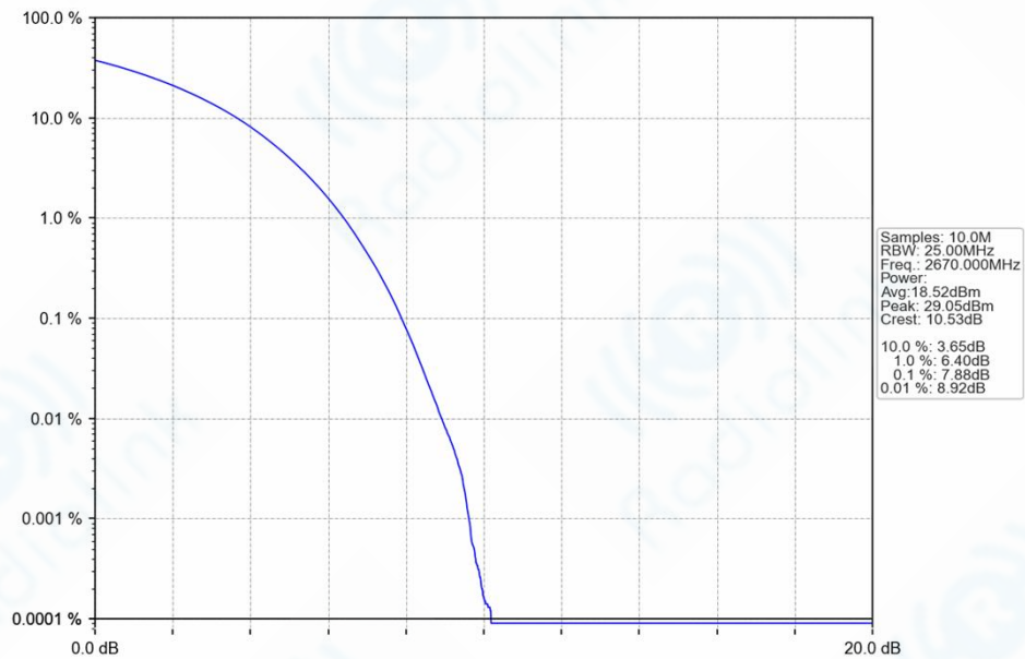
n41_30kHz_SISO_NTNV_40MHz_CP-OFDM QPSK_2670MHz_Outer_Full_Ant1
