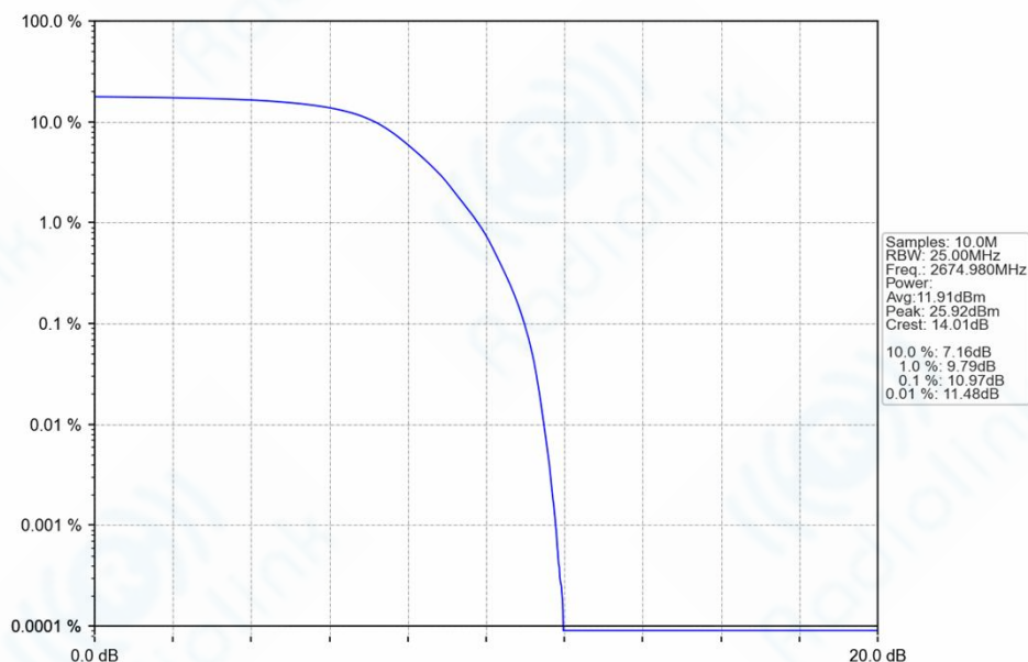
n41_30kHz_SISO_NTNV_30MHz_DFT-s-OFDM_PI/2_BPSK_2674.98MHz_Outer_Full_Ant1
