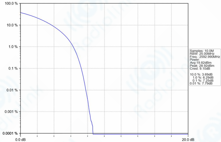
n41_30kHz_SISO_NTNV_30MHz_CP-OFDM_16_QAM_2592.99MHz_Outer_Full_Ant1
