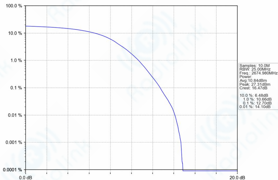
n41_30kHz_SISO_NTNV_30MHz_DFT-s-OFDM_256_QAM_2674.98MHz_Outer_Full_Ant1
