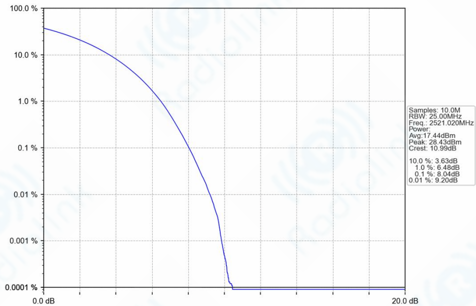
n41_30kHz_SISO_NTNV_50MHz_DFT-s-OFDM_QPSK_2521.02MHz_Outer_Full_Ant1
