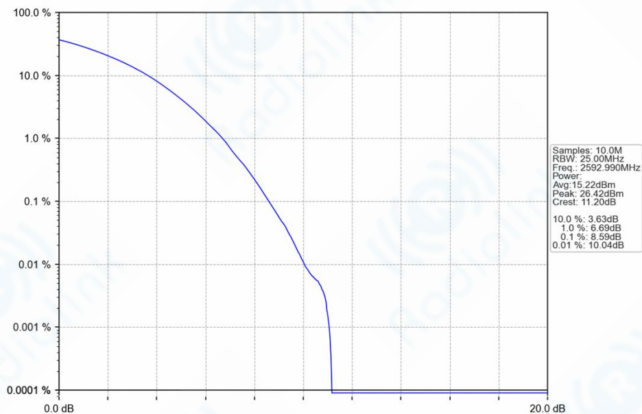
n41_30kHz_SISO_NTNV_40MHz_CP-OFDM 256 QAM 2592.99MHz_Outer_Full_Ant1
