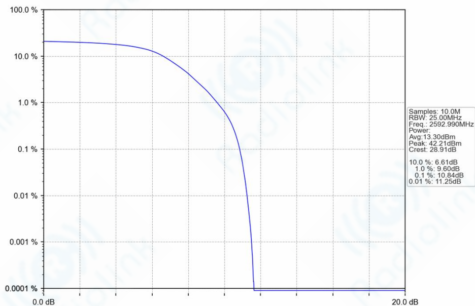
n41_30kHz_SISO_NTNV_30MHz_DFT-s-OFDM_QPSK_2592.99MHz_Outer_Full_Ant1
