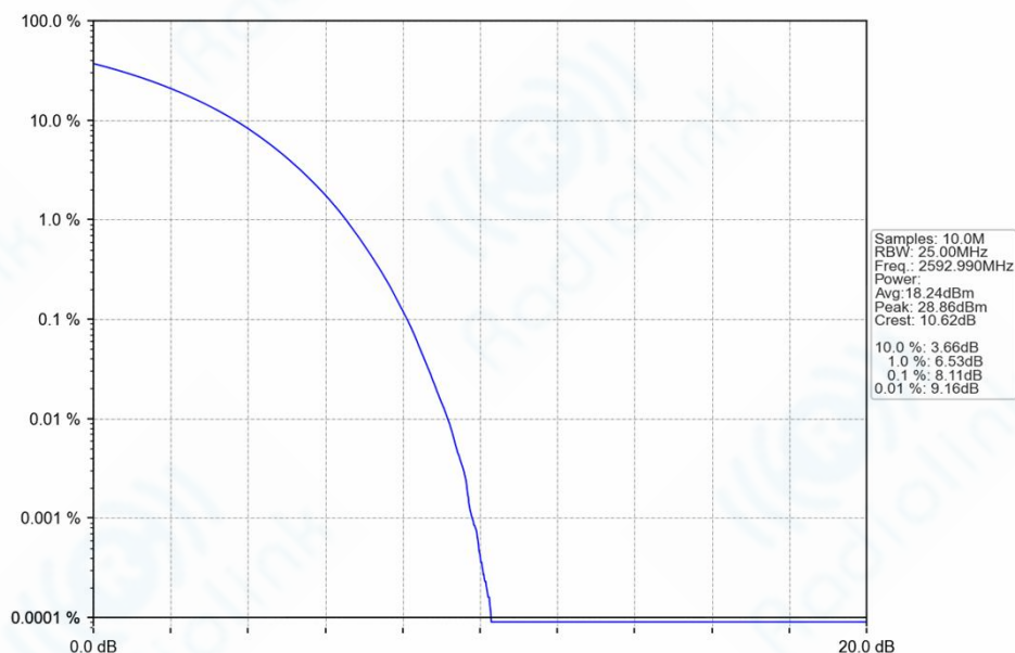
n41_30kHz_SISO_NTNV_40MHz_CP-OFDM_64_QAM_2592.99MHz_Outer_Full_Ant1
