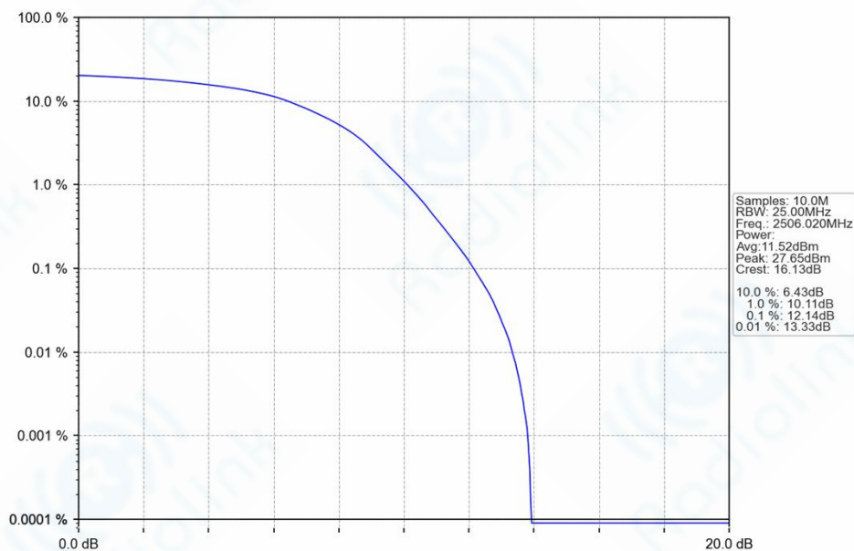
n41_30kHz_SISO_NTNV_20MHz_DFT-s-OFDM_256_QAM_2506.02MHz_Outer_Full_Ant1
