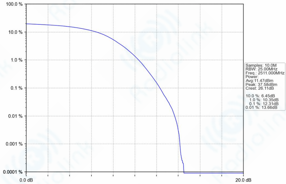
n41_30kHz_SISO_NTNV_30MHz_DFT-s-OFDM_256_QAM_2511MHz_Outer_Full_Ant1
