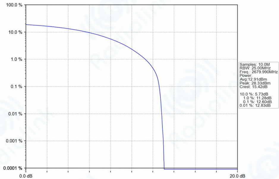
n41_30kHz_SISO_NTNV_20MHz_CP-OFDM QPSK_2679.99MHz_Outer_Full_Ant1
