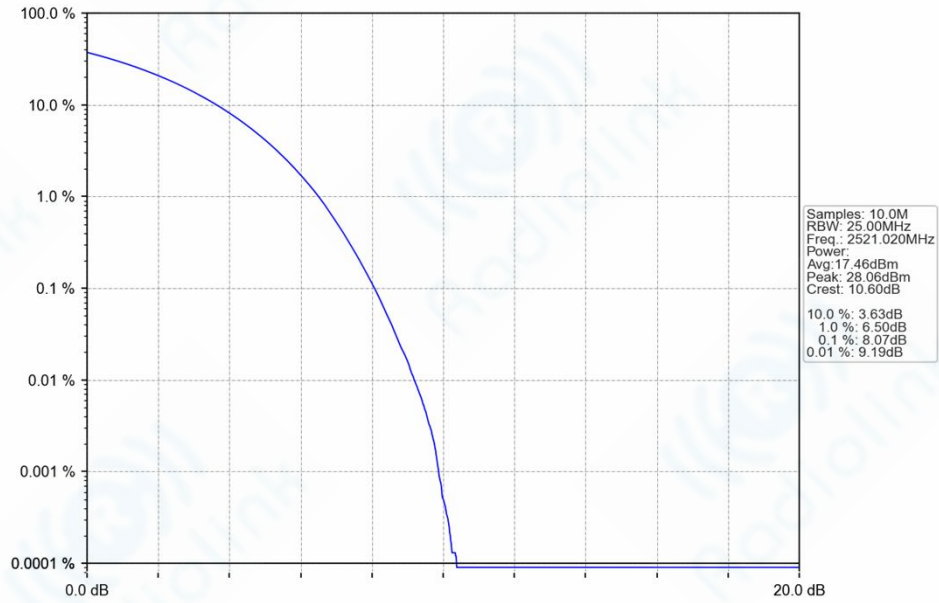
n41_30kHz_SISO_NTNV_50MHz_DFT-s-OFDM_16_QAM_2521.02MHz_Outer_Full_Ant1
