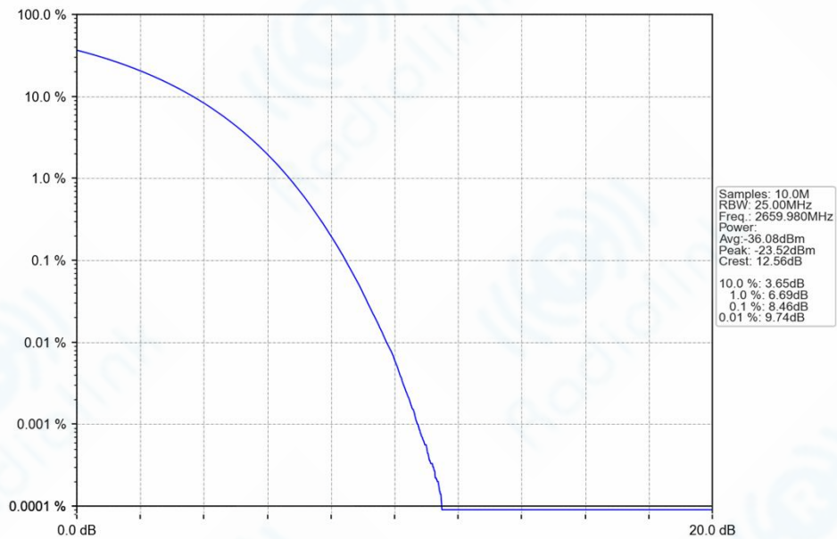
n41_30kHz_SISO_NTNV_60MHz_DFT-s-OFDM_QPSK_2659.98MHz_Outer_Full_Ant1
