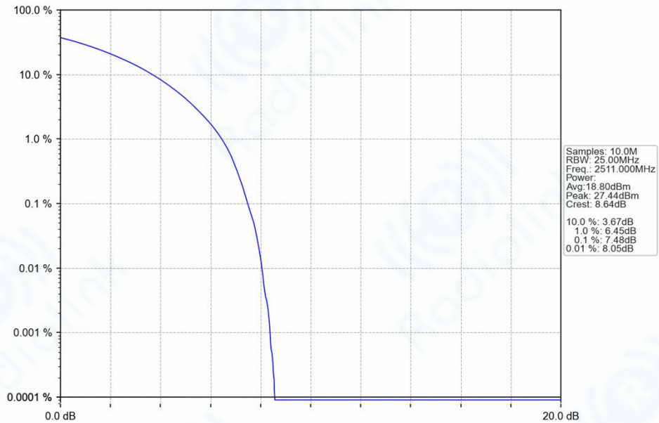
n41_30kHz_SISO_NTNV_30MHz_CP-OFDM_64_QAM_2511MHz_Outer_Full_Ant1
