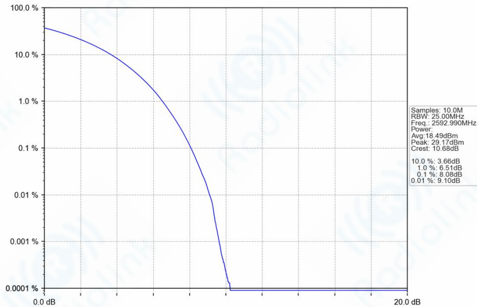
n41_30kHz_SISO_NTNV_40MHz_DFT-s-OFDM_64_QAM_2592.99MHz_Outer_Full_Ant1
