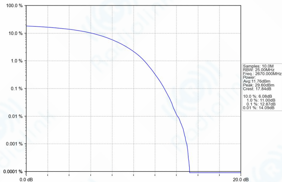
n41_30kHz_SISO_NTNV_40MHz_DFT-s-OFDM_64_QAM_2670MHz_Outer_Full_Ant1
