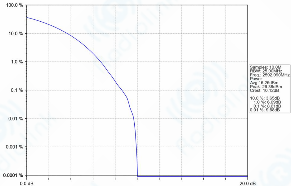
n41_30kHz_SISO_NTNV_20MHz_CP-OFDM 256 QAM_2592.99MHz_Outer_Full_Ant1
