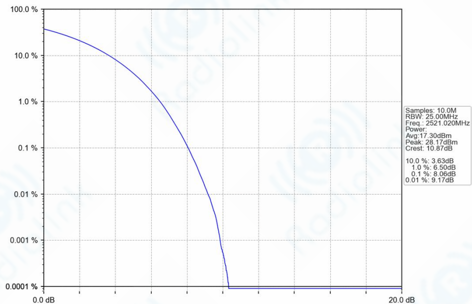
n41_30kHz_SISO_NTNV_50MHz_CP-OFDM_QPSK_2521.02MHz_Outer_Full_Ant1
