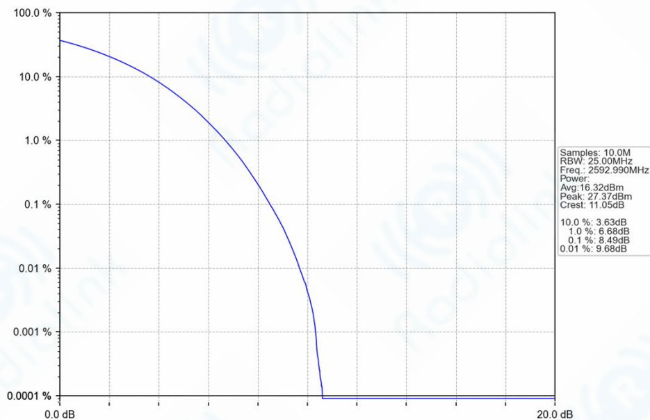
n41_30kHz_SISO_NTNV_30MHz_CP-OFDM_256_QAM_2592.99MHz_Outer_Full_Ant1
