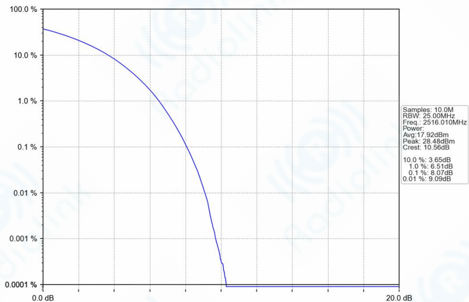
n41_30kHz_SISO_NTNV_40MHz_DFT-s-OFDM_64_QAM_2516.01MHz_Outer_Full_Ant1
