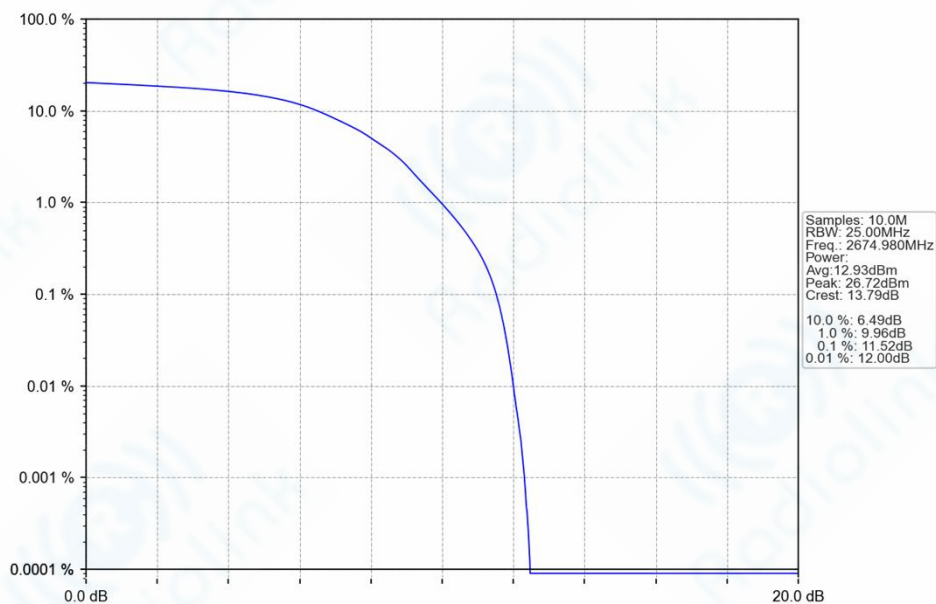
n41_30kHz_SISO_NTNV_30MHz_DFT-s-OFDM_16_QAM_2674.98MHz_Outer_Full_Ant1
