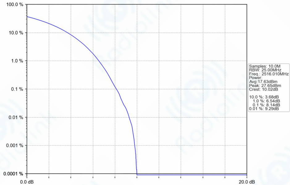
n41_30kHz_SISO_NTNV_40MHz_CP-OFDM_64_QAM_2516.01MHz_Outer_Full_Ant1
