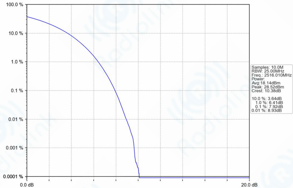
n41_30kHz_SISO_NTNV_40MHz_CP-OFDM_QPSK_2516.01MHz_Outer_Full_Ant1
