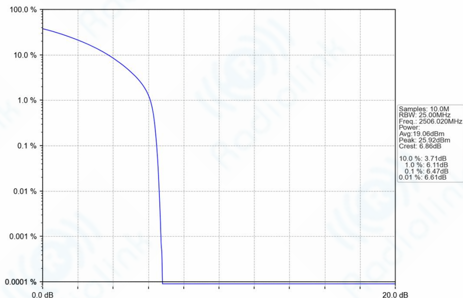
n41_30kHz_SISO_NTNV_20MHz_CP-OFDM_16_QAM_2506.02MHz_Outer_Full_Ant1
