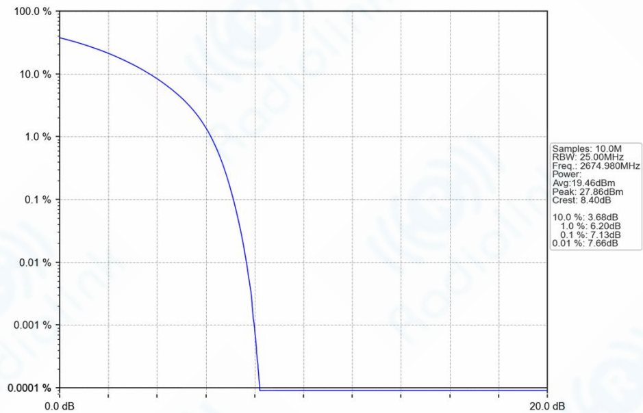
n41_30kHz_SISO_NTNV_30MHz_CP-OFDM QPSK_2674.98MHz_Outer_Full_Ant1
