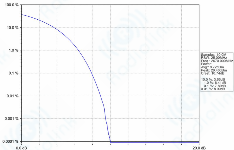
n41_30kHz_SISO_NTNV_40MHz_DFT-s-OFDM_16_QAM_2670MHz_Outer_Full_Ant1
