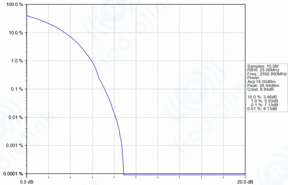
n41_30kHz_SISO_NTNV_50MHz_DFT-s-OFDM_16_QAM_2592.99MHz_Outer_Full_Ant1
