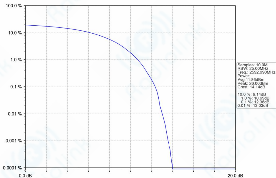
n41_30kHz_SISO_NTNV_50MHz_DFT-s-OFDM_QPSK_2592.99MHz_Outer_Full_Ant1
