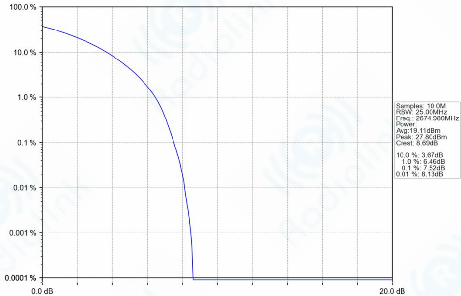
n41_30kHz_SISO_NTNV_30MHz_CP-OFDM_64_QAM_2674.98MHz_Outer_Full_Ant1
