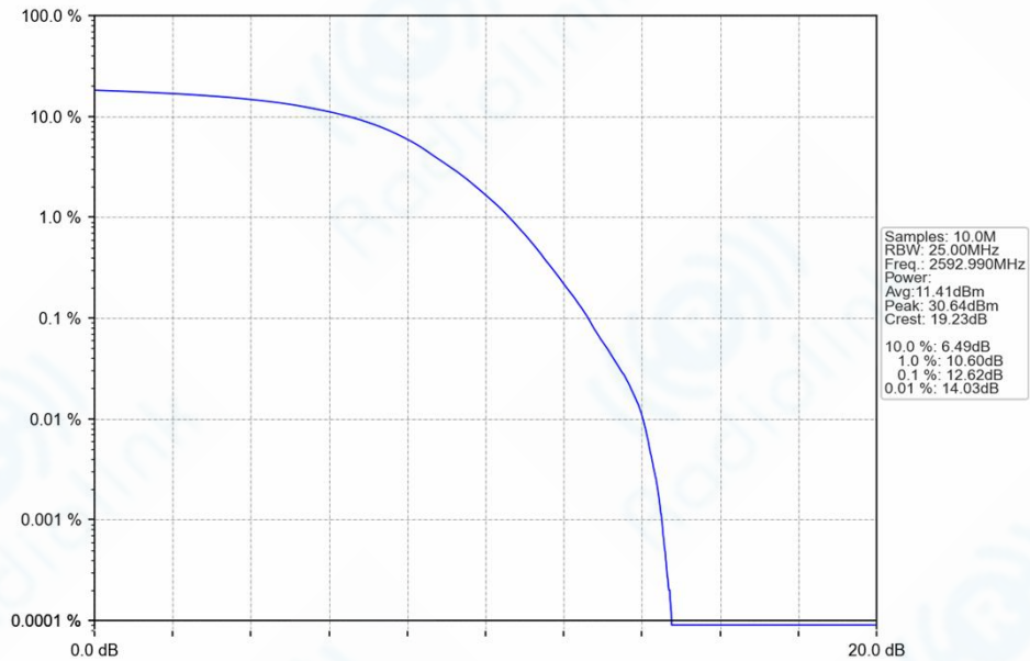
n41_30kHz_SISO_NTNV_30MHz_DFT-s-OFDM_256_QAM_2592.99MHz_Outer_Full_Ant1
