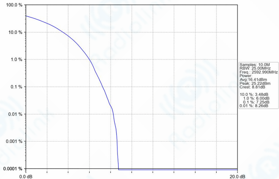
n41_30kHz_SISO_NTNV_50MHz_DFT-s-OFDM_256_QAM_2592.99MHz_Outer_Full_Ant1
