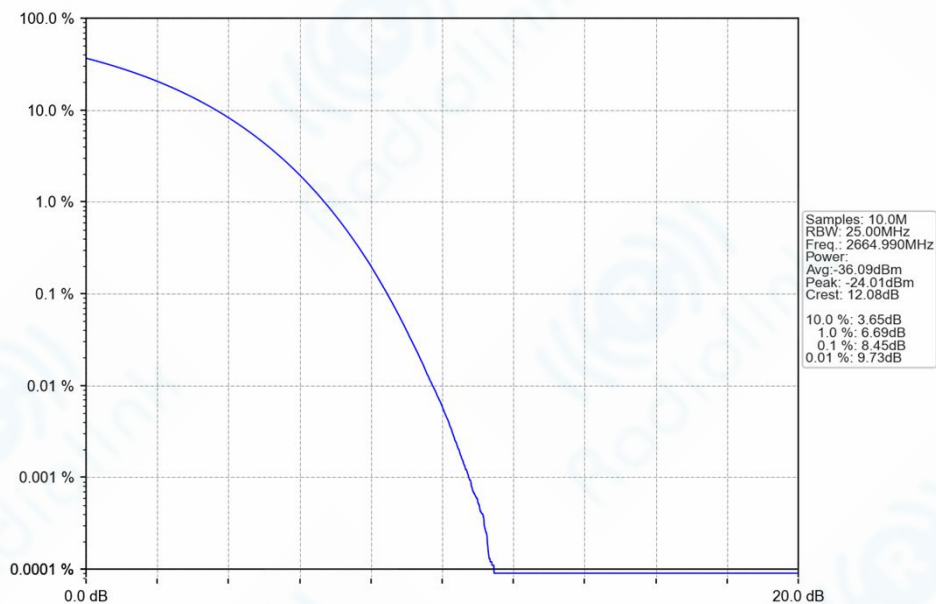
n41_30kHz_SISO_NTNV_50MHz_DFT-s-OFDM_QPSK_2664.99MHz_Outer_Full_Ant1
