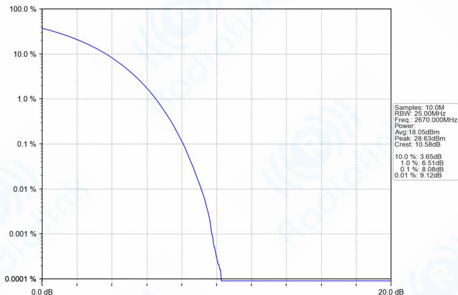
n41_30kHz_SISO_NTNV_40MHz_CP-OFDM_64_QAM_2670MHz_Outer_Full_Ant1
