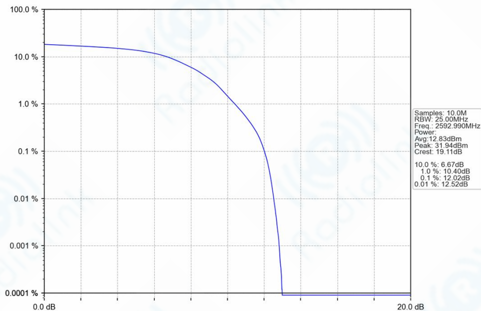
n41_30kHz_SISO_NTNV_30MHz_DFT-s-OFDM_16_QAM_2592.99MHz_Outer_Full_Ant1
