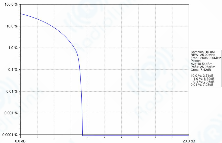
n41_30kHz_SISO_NTNV_20MHz_CP-OFDM_64_QAM_2506.02MHz_Outer_Full_Ant1
