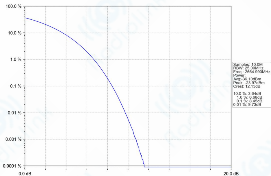
n41_30kHz_SISO_NTNV_50MHz_CP-OFDM_QPSK_2664.99MHz_Outer_Full_Ant1
