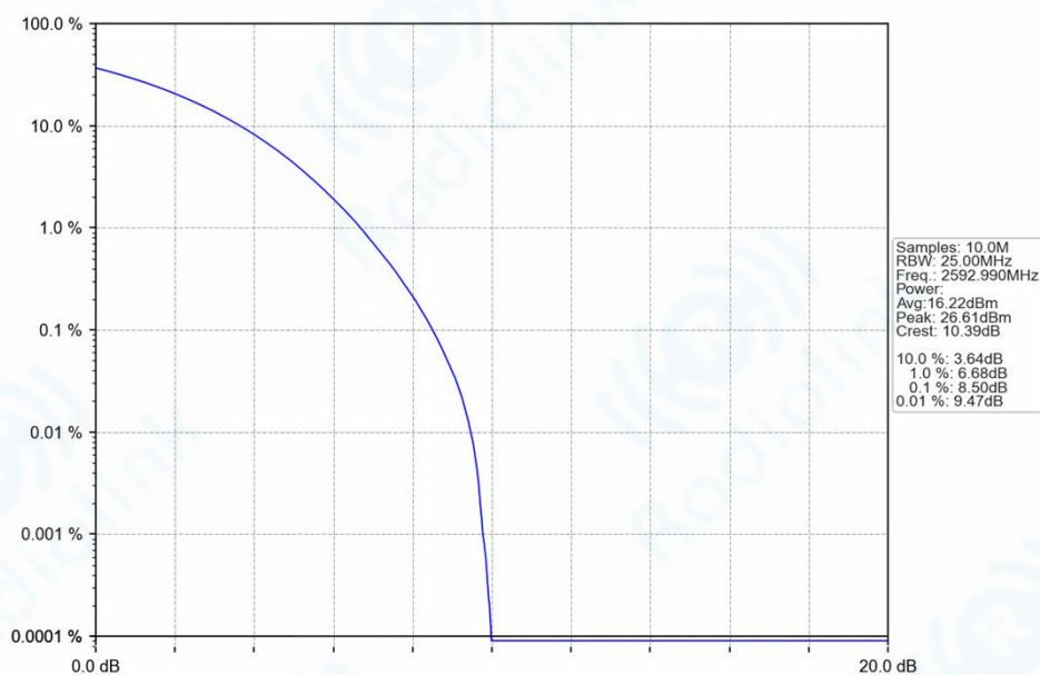
n41_30kHz_SISO_NTNV_20MHz_DFT-s-OFDM_256_QAM_2592.99MHz_Outer_Full_Ant1
