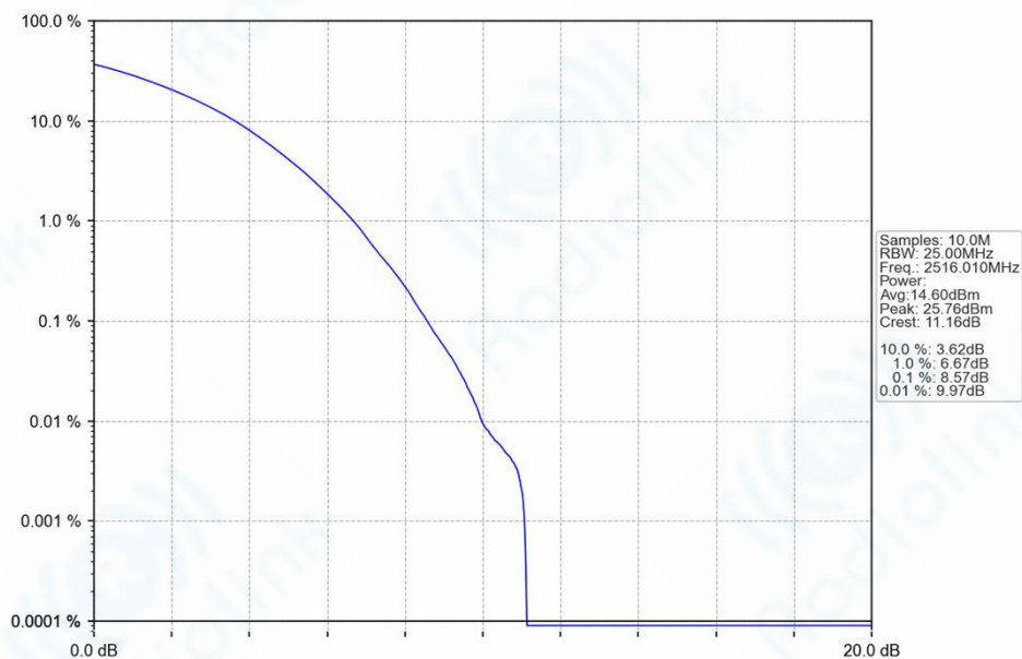
n41_30kHz_SISO_NTNV_40MHz_CP-OFDM 256 QAM 2516.01MHz_Outer_Full_Ant1
