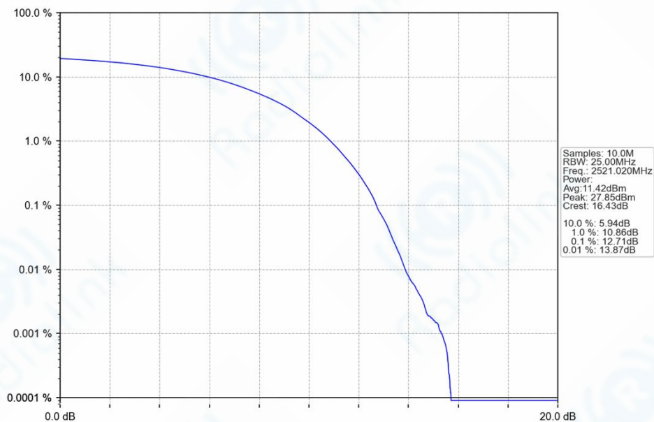
n41_30kHz_SISO_NTNV_50MHz_DFT-s-OFDM_64_QAM_2521.02MHz_Outer_Full_Ant1
