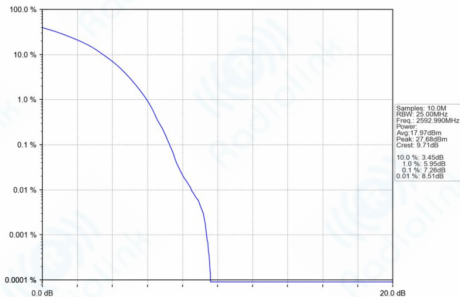
n41_30kHz_SISO_NTNV_50MHz_DFT-s-OFDM_64_QAM_2592.99MHz_Outer_Full_Ant1
