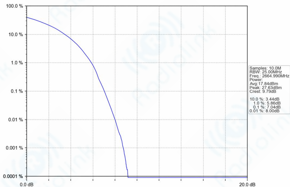
n41_30kHz_SISO_NTNV_50MHz_DFT-s-OFDM_16_QAM_2664.99MHz_Outer_Full_Ant1
