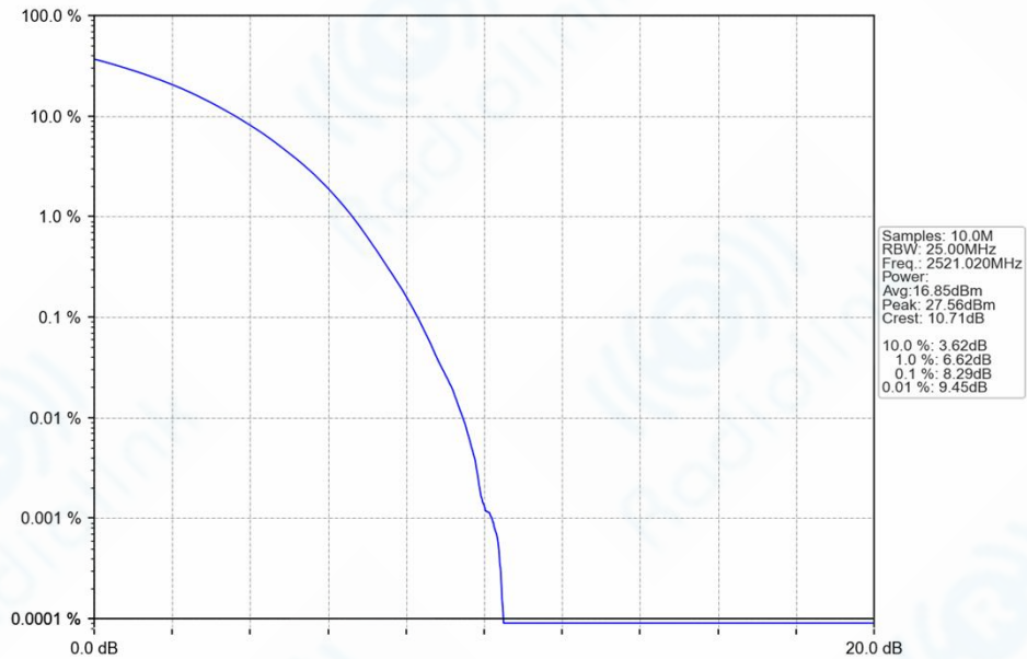
n41_30kHz_SISO_NTNV_50MHz_CP-OFDM_64_QAM_2521.02MHz_Outer_Full_Ant1
