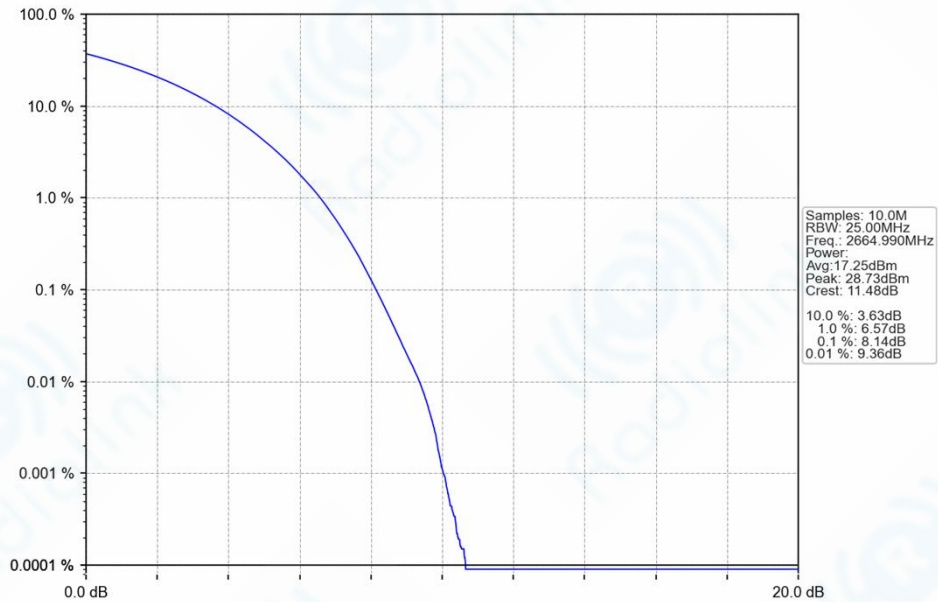
n41_30kHz_SISO_NTNV_50MHz_CP-OFDM_64_QAM_2664.99MHz_Outer_Full_Ant1
