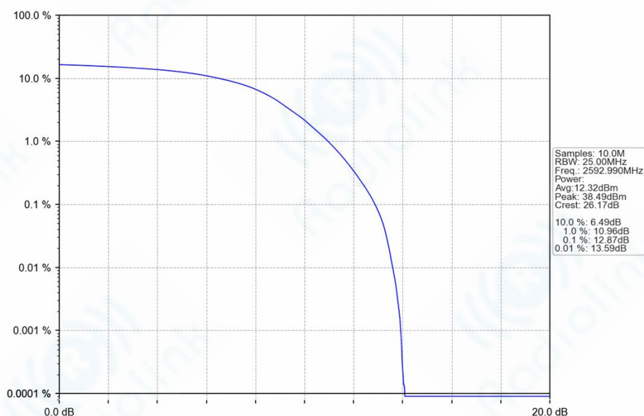
n41_30kHz_SISO_NTNV_30MHz_DFT-s-OFDM_64_QAM_2592.99MHz_Outer_Full_Ant1
