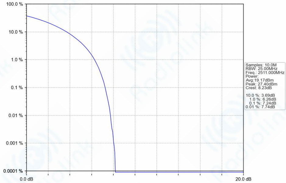
n41_30kHz_SISO_NTNV_30MHz_CP-OFDM_16_QAM_2511MHz_Outer_Full_Ant1
