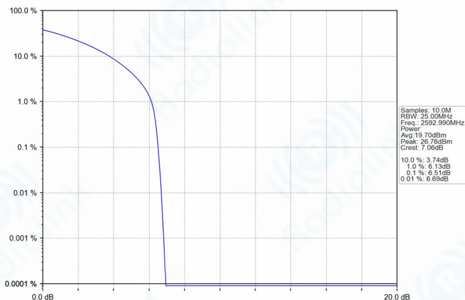
n41_30kHz_SISO_NTNV_20MHz_CP-OFDM_16_QAM_2592.99MHz_Outer_Full_Ant1
