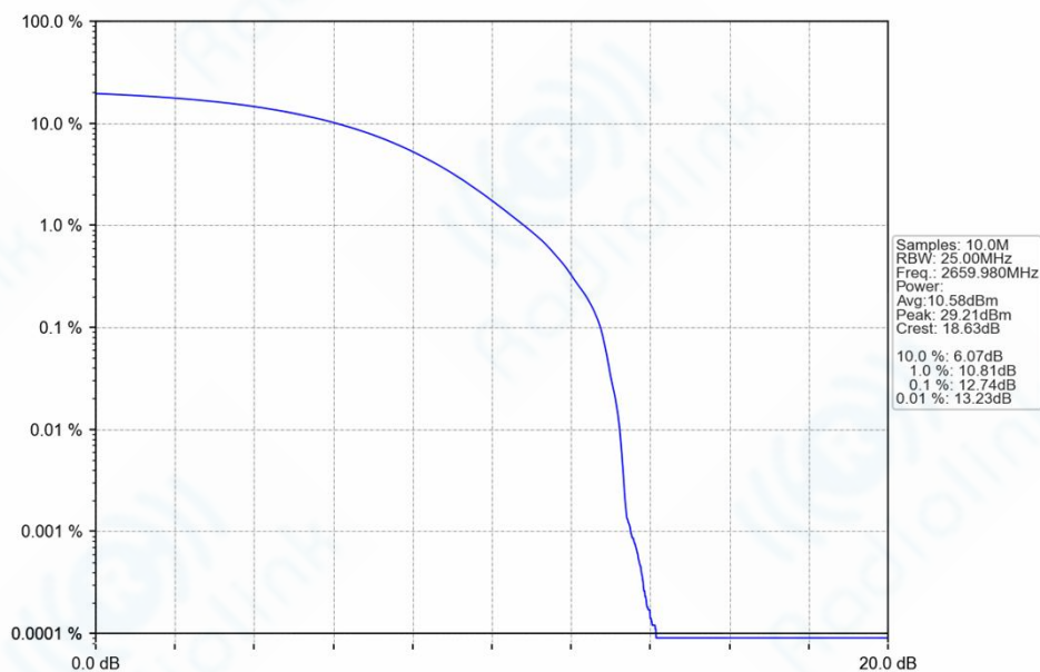
n41_30kHz_SISO_NTNV_60MHz_DFT-s-OFDM_PI/2_BPSK_2659.98MHz_Outer_Full_Ant1
