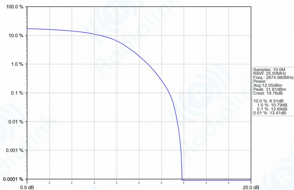
n41_30kHz_SISO_NTNV_30MHz_DFT-s-OFDM_64_QAM_2674.98MHz_Outer_Full_Ant1
