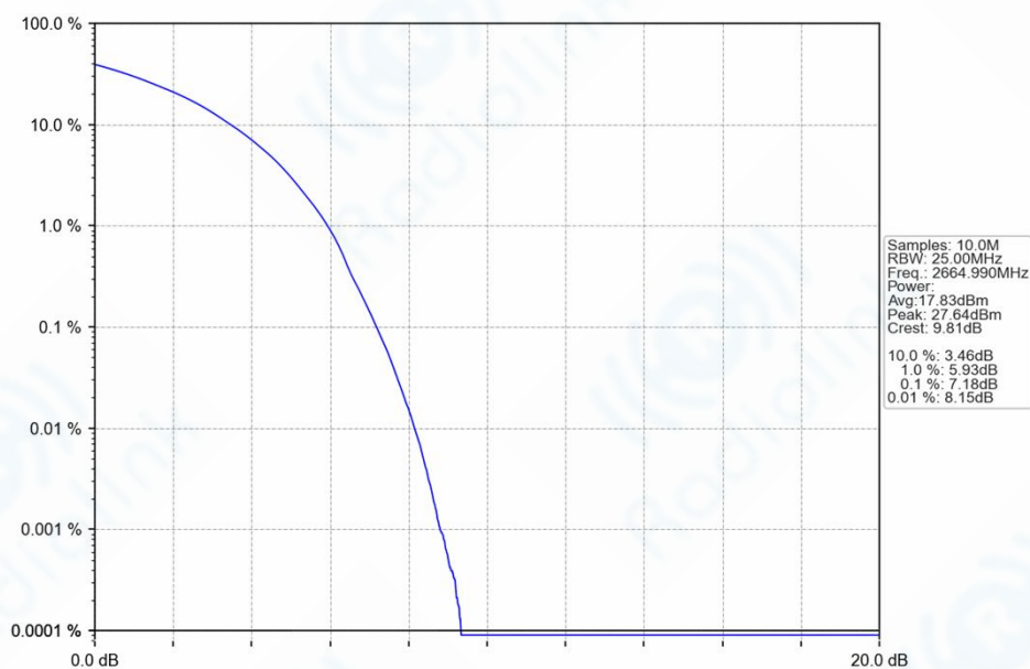
n41_30kHz_SISO_NTNV_50MHz_DFT-s-OFDM_64_QAM_2664.99MHz_Outer_Full_Ant1
