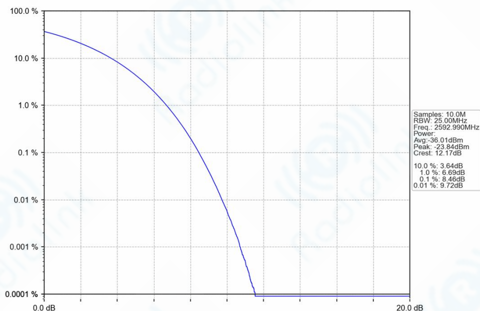
n41_30kHz_SISO_NTNV_50MHz_CP-OFDM_16_QAM_2592.99MHz_Outer_Full_Ant1
