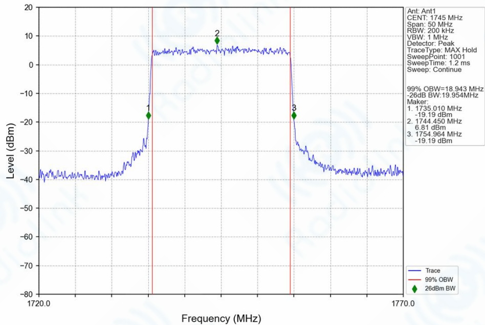
n66_15kHz_SISO_NTNV_20MHz_CP-OFDM_16_QAM_1745MHz_Outer_Full_Ant1
