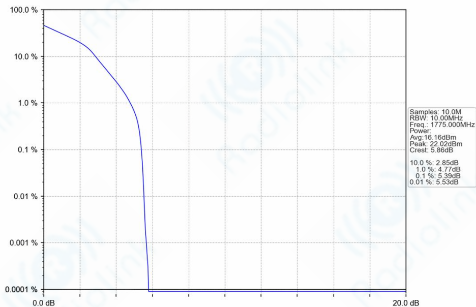
n66_15kHz_SISO_NTNV_10MHz_DFT-s-OFDM_16_QAM_1775MHz_Outer_Full_Ant1
