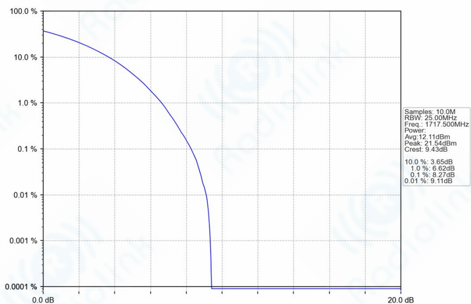
n66_15kHz_SISO_NTNV_15MHz_CP-OFDM 256 QAM_1717.5MHz_Outer_Full_Ant1
