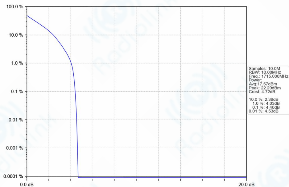
n66_15kHz_SISO_NTNV_10MHz_DFT-s-OFDM QPSK_1715MHz_Outer_Full_Ant1
