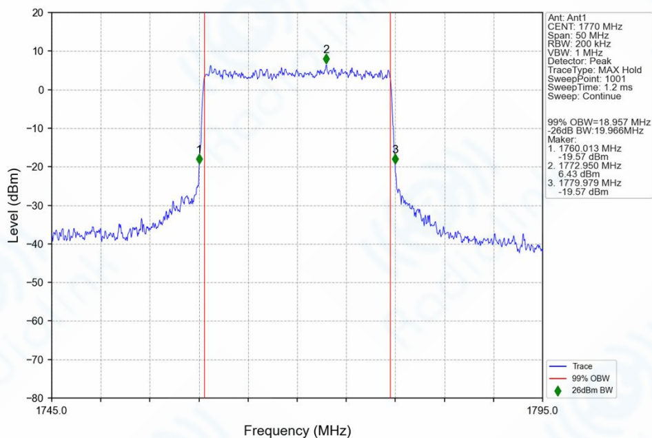
n66_15kHz_SISO_NTNV_20MHz_CP-OFDM_64_QAM_1770MHz_Outer_Full_Ant1
