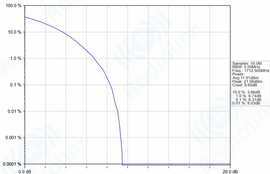
n66_15kHz_SISO_NTNV_5MHz_CP-OFDM_256_QAM_1712.5MHz_Outer_Full_Ant1
