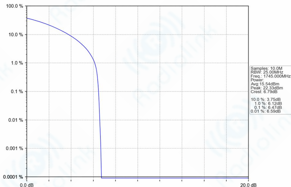
n66_15kHz_SISO_NTNV_15MHz_CP-OFDM QPSK_1745MHz_Outer_Full_Ant1
