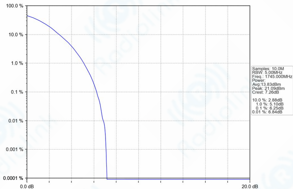
n66_15kHz_SISO_NTNV_5MHz_DFT-s-OFDM_256_QAM_1745MHz_Outer_Full_Ant1
