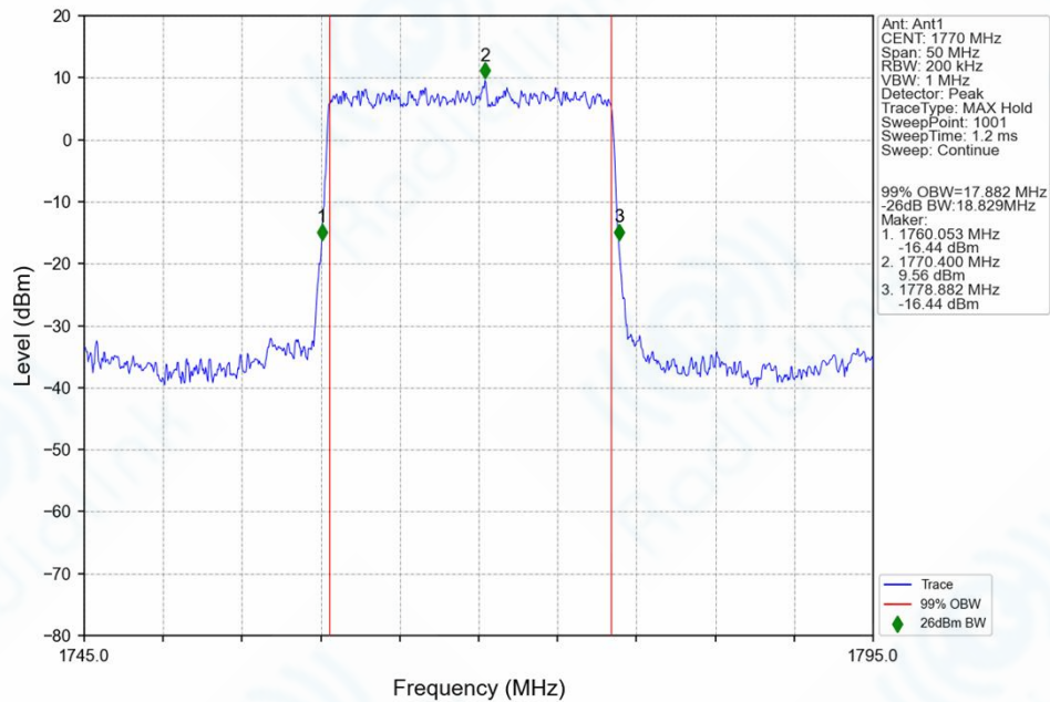
n66_15kHz_SISO_NTNV_20MHz_DFT-s-OFDM QPSK_1770MHz_Outer_Full_Ant1
