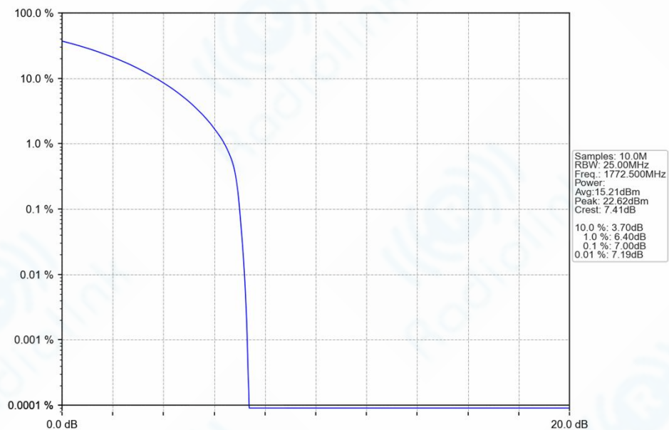
n66_15kHz_SISO_NTNV_15MHz_CP-OFDM_64_QAM_1772.5MHz_Outer_Full_Ant1
