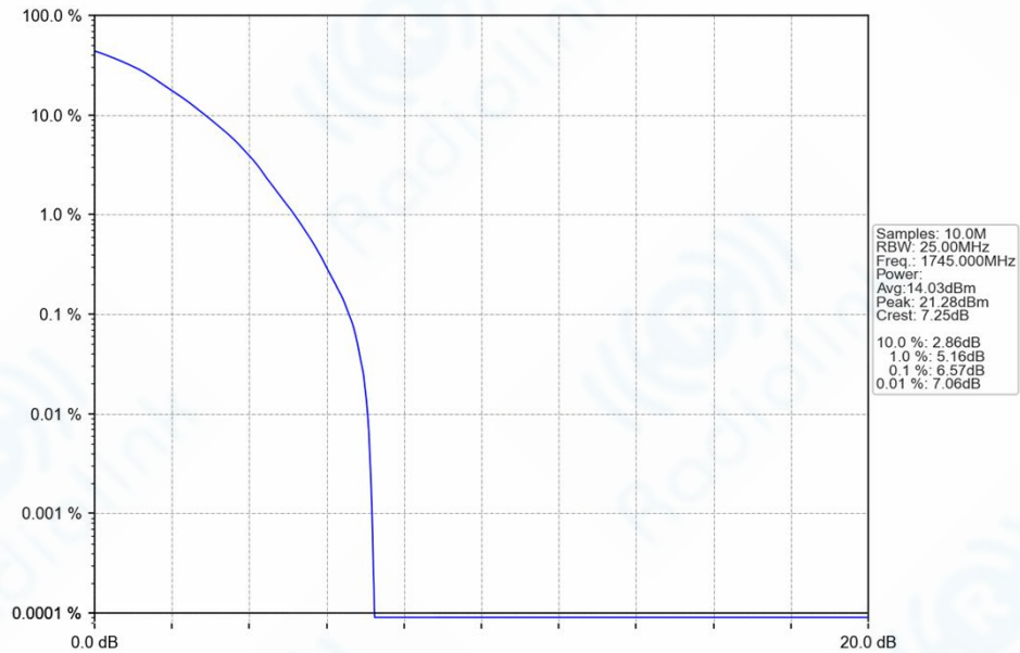
n66_15kHz_SISO_NTNV_15MHz_DFT-s-OFDM_256_QAM_1745MHz_Outer_Full_Ant1
