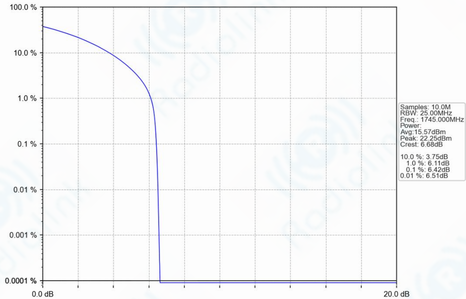
n66_15kHz_SISO_NTNV_15MHz_CP-OFDM_16_QAM_1745MHz_Outer_Full_Ant1
