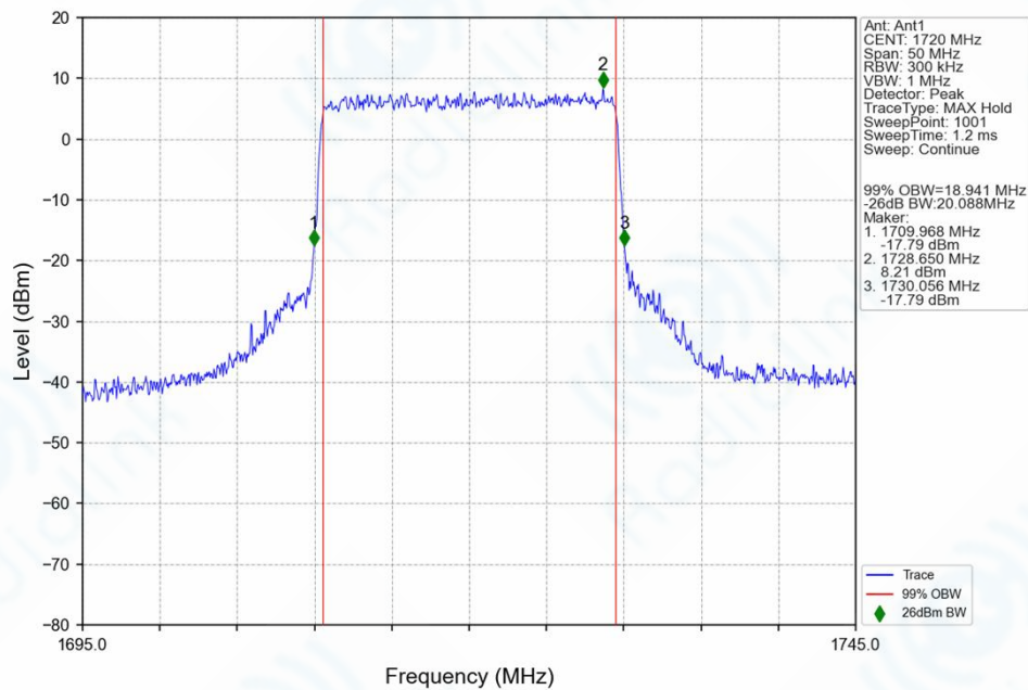
n66_15kHz_SISO_NTNV_20MHz_CP-OFDM_64_QAM_1720MHz_Outer_Full_Ant1
