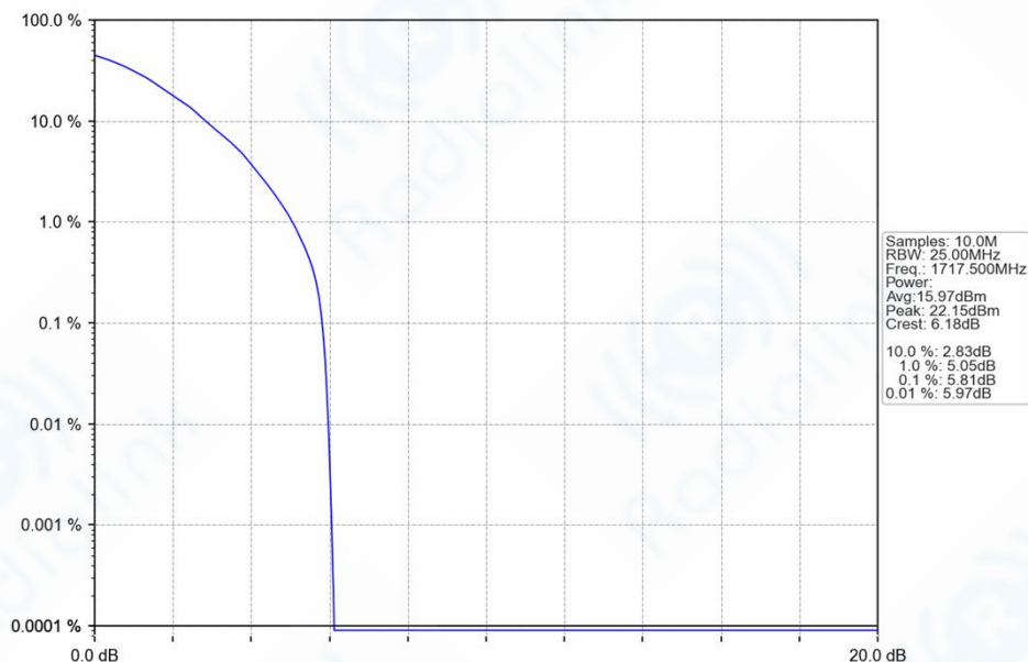
n66_15kHz_SISO_NTNV_15MHz_DFT-s-OFDM_64_QAM_1717.5MHz_Outer_Full_Ant1
