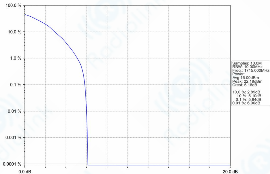
n66_15kHz_SISO_NTNV_10MHz_DFT-s-OFDM_64_QAM_1715MHz_Outer_Full_Ant1
