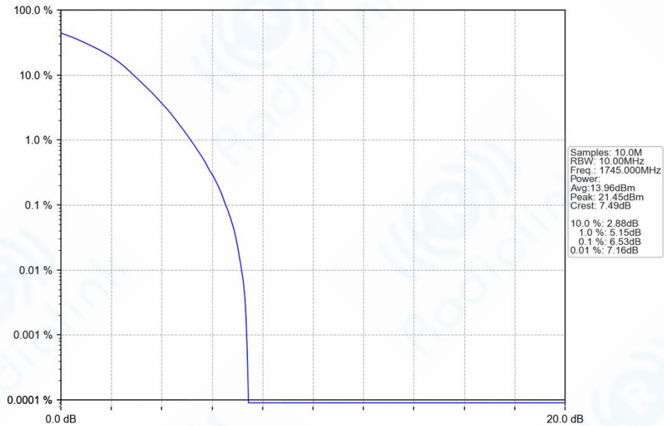
n66_15kHz_SISO_NTNV_10MHz_DFT-s-OFDM_256_QAM_1745MHz_Outer_Full_Ant1
