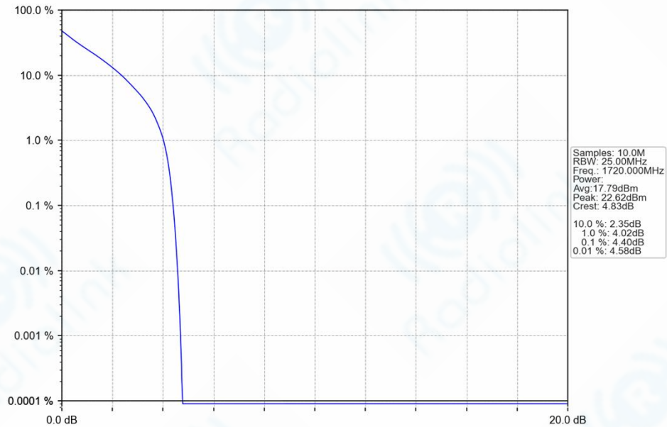
n66_15kHz_SISO_NTNV_20MHz_DFT-s-OFDM QPSK_1720MHz_Outer_Full_Ant1
