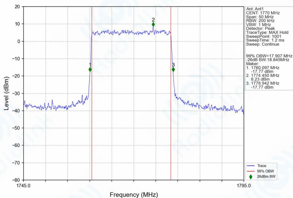
n66_15kHz_SISO_NTNV_20MHz_DFT-s-OFDM_64_QAM_1770MHz_Outer_Full_Ant1
