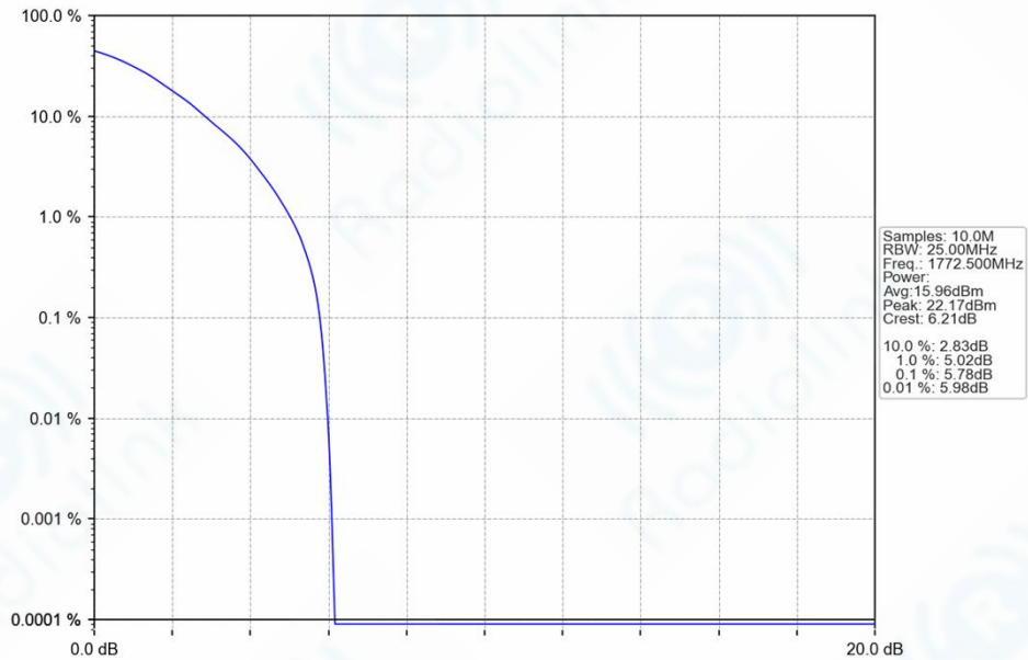
n66_15kHz_SISO_NTNV_15MHz_DFT-s-OFDM_64_QAM_1772.5MHz_Outer_Full_Ant1
