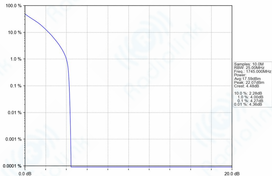
n66_15kHz_SISO_NTNV_15MHz_DFT-s-OFDM_QPSK_1745MHz_Outer_Full_Ant1
