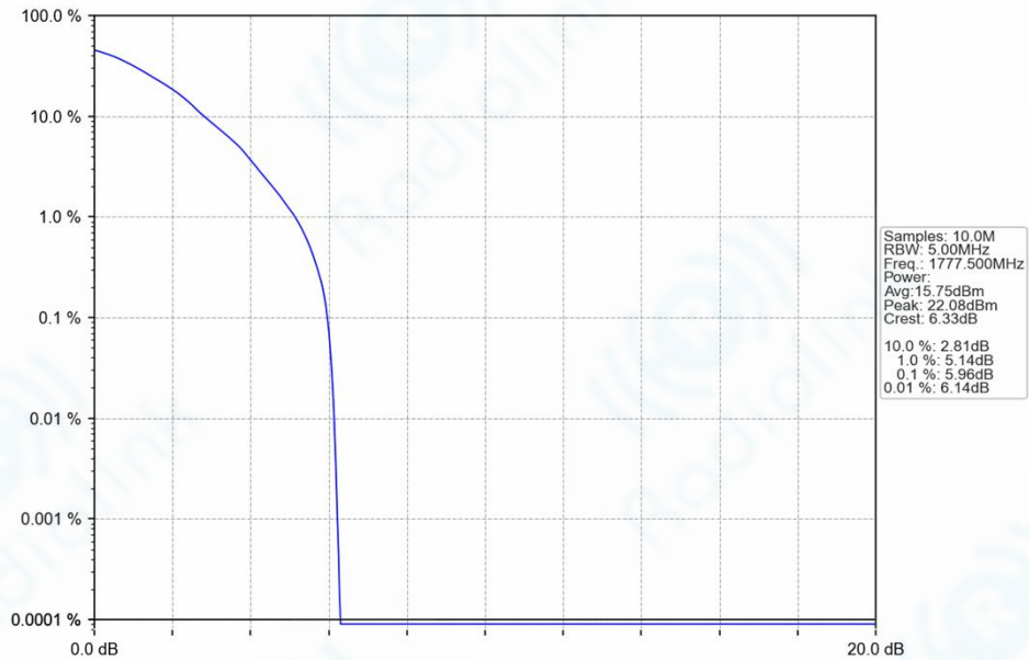
n66_15kHz_SISO_NTNV_5MHz_DFT-s-OFDM_64_QAM_1777.5MHz_Outer_Full_Ant1
