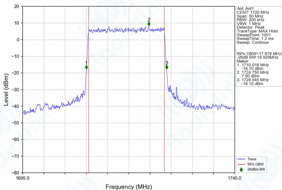
n66_15kHz_SISO_NTNV_20MHz_DFT-s-OFDM_64_QAM_1720MHz_Outer_Full_Ant1
