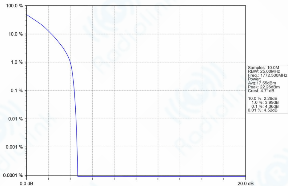
n66_15kHz_SISO_NTNV_15MHz_DFT-s-OFDM_QPSK_1772.5MHz_Outer_Full_Ant1
