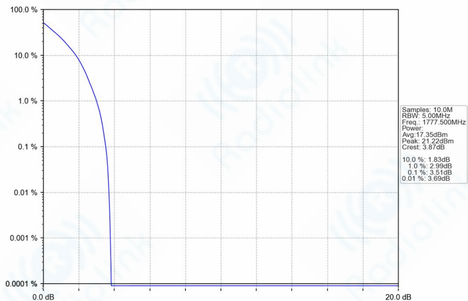
n66_15kHz_SISO_NTNV_5MHz_DFT-s-OFDM_PI/2_BPSK_1777.5MHz_Outer_Full_Ant1
