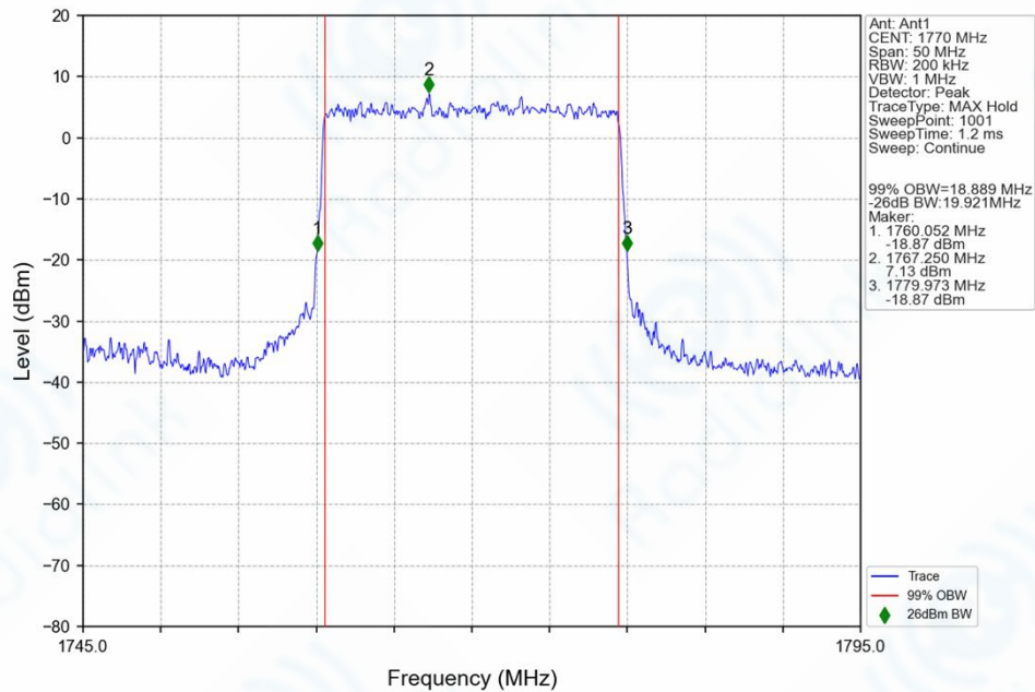
n66_15kHz_SISO_NTNV_20MHz_CP-OFDM QPSK_1770MHz_Outer_Full_Ant1
