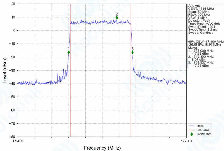
n66_15kHz_SISO_NTNV_20MHz_DFT-s-OFDM_16_QAM_1745MHz_Outer_Full_Ant1
