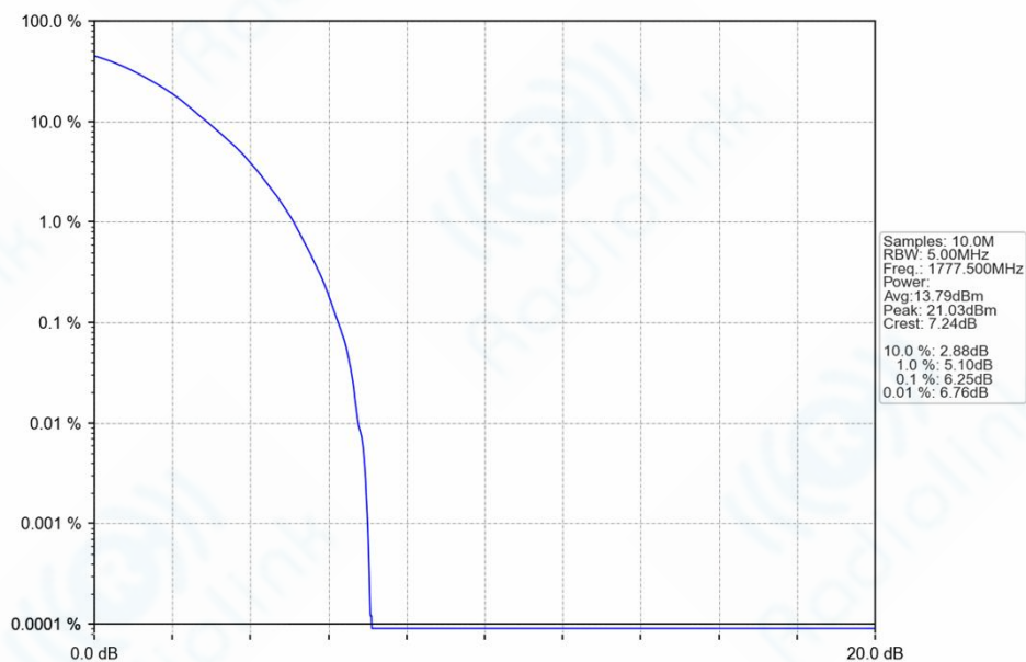
n66_15kHz_SISO_NTNV_5MHz_DFT-s-OFDM_256_QAM_1777.5MHz_Outer_Full_Ant1
