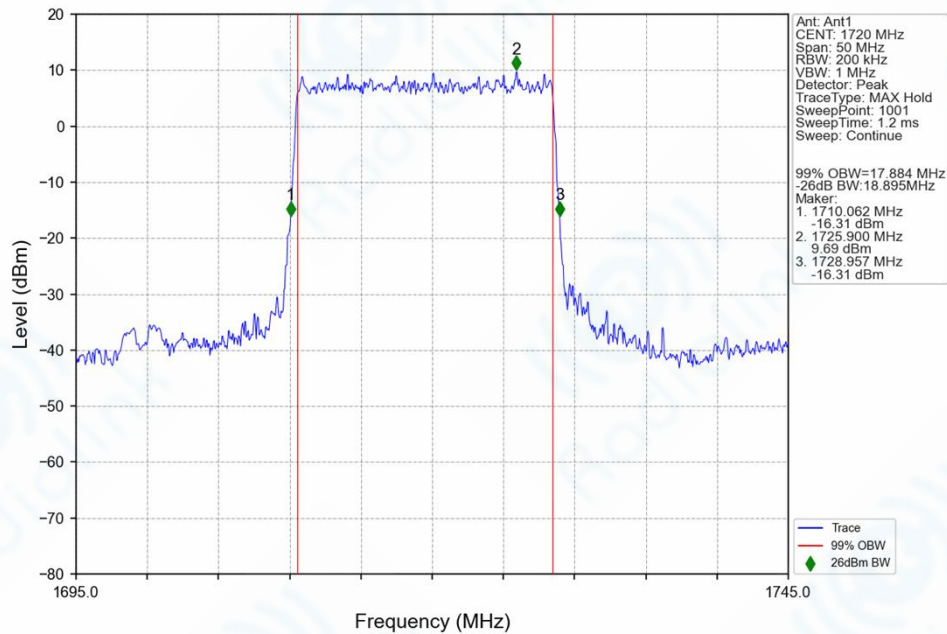
n66_15kHz_SISO_NTNV_20MHz_DFT-s-OFDM QPSK_1720MHz_Outer_Full_Ant1
