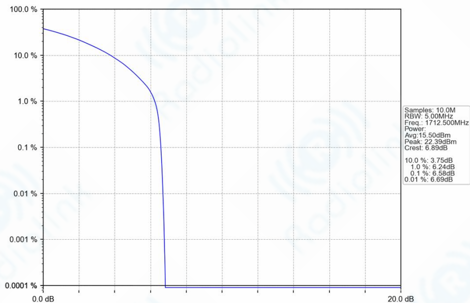
n66_15kHz_SISO_NTNV_5MHz_CP-OFDM_QPSK_1712.5MHz_Outer_Full_Ant1
