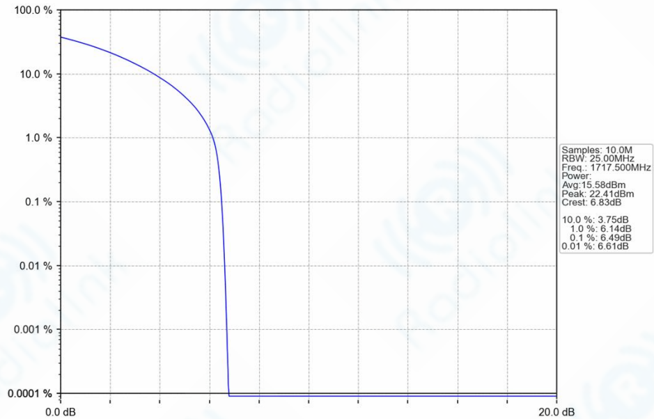
n66_15kHz_SISO_NTNV_15MHz_CP-OFDM_QPSK_1717.5MHz_Outer_Full_Ant1
