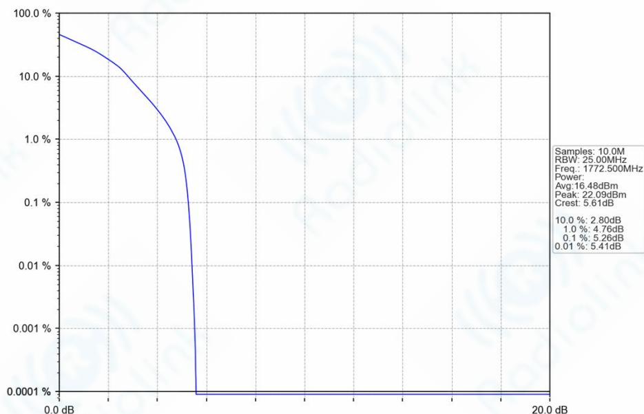
n66_15kHz_SISO_NTNV_15MHz_DFT-s-OFDM_16_QAM_1772.5MHz_Outer_Full_Ant1
