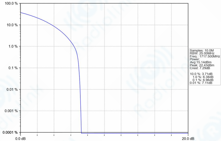
n66_15kHz_SISO_NTNV_15MHz_CP-OFDM_64_QAM_1717.5MHz_Outer_Full_Ant1
