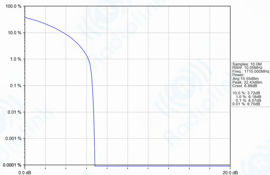
n66_15kHz_SISO_NTNV_10MHz_CP-OFDM QPSK 1715MHz_Outer_Full_Ant1
