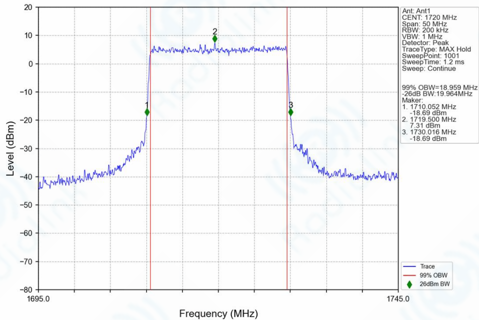
n66_15kHz_SISO_NTNV_20MHz_CP-OFDM QPSK_1720MHz_Outer_Full_Ant1
