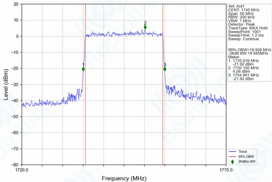
n66_15kHz_SISO_NTNV_20MHz_CP-OFDM_256_QAM_1745MHz_Outer_Full_Ant1
