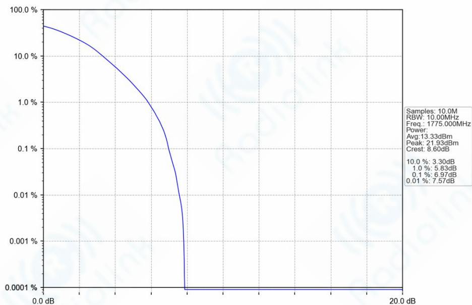
n66_15kHz_SISO_NTNV_10MHz_DFT-s-OFDM 256 QAM 1775MHz_Outer_Full_Ant1
