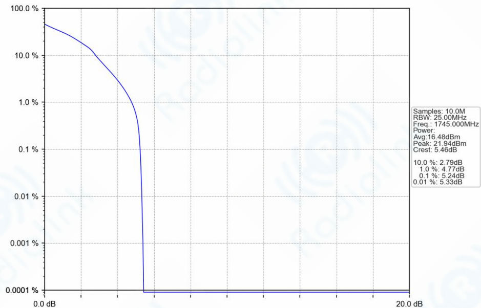
n66_15kHz_SISO_NTNV_15MHz_DFT-s-OFDM_16_QAM_1745MHz_Outer_Full_Ant1
