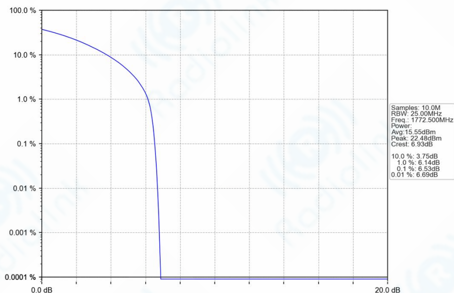
n66_15kHz_SISO_NTNV_15MHz_CP-OFDM QPSK_1772.5MHz_Outer_Full_Ant1
