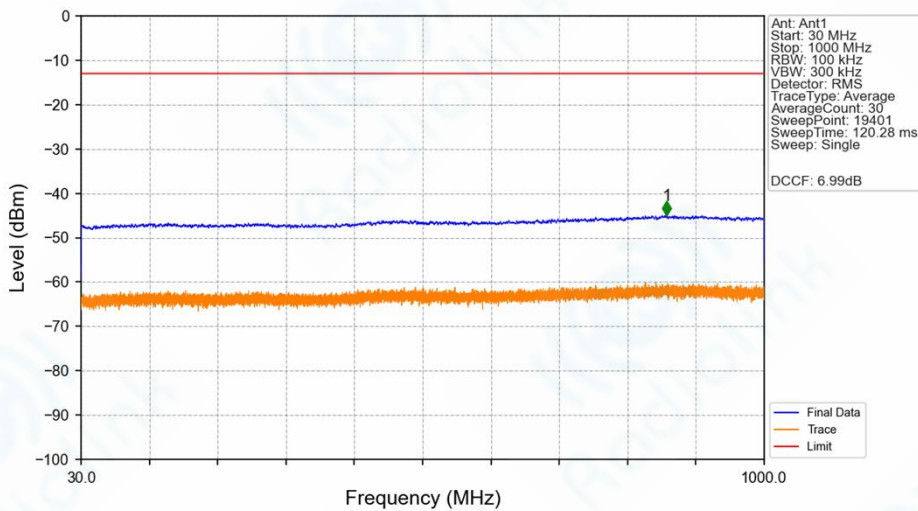
n77a_30kHz_SISO_NTNV_30MHz_DFT-s-OFDM_QPSK_3715.02MHz_Edge_1RB_Left_Ant1
