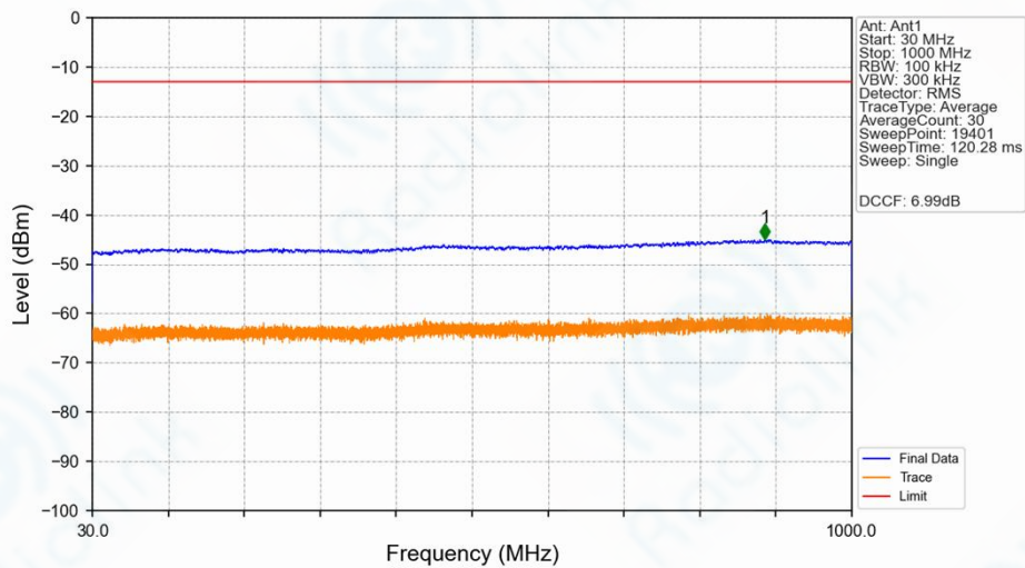
n77a_30kHz_SISO_NTNV_30MHz_CP-OFDM_QPSK_3715.02MHz_Edge_1RB_Left_Ant1
