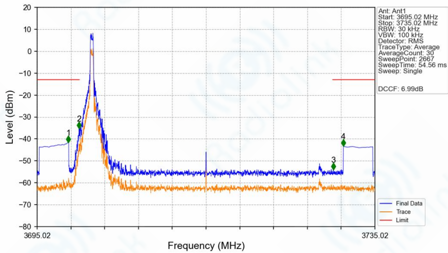
n77a_30kHz_SISO_NTNV_30MHz_CP-OFDM_QPSK_3715.02MHz_Inner_1RB_Left_Ant1
