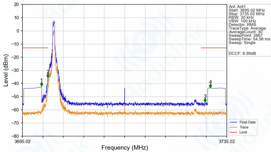
n77a_30kHz_SISO_NTNV_30MHz_CP-OFDM_QPSK_3715.02MHz_Edge_1RB_Left_Ant1
