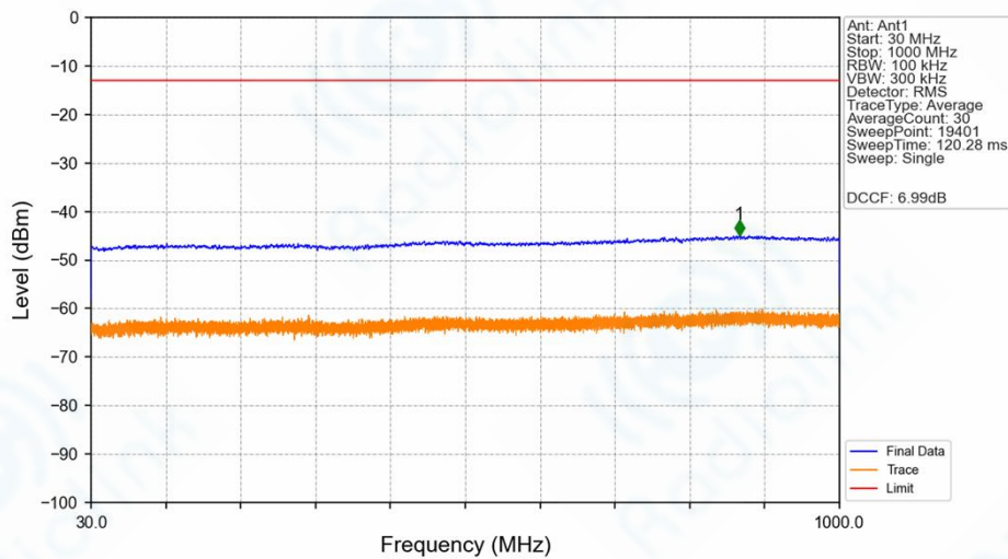
n77a_30kHz_SISO_NTNV_30MHz_CP-OFDM_QPSK_3840MHz_Edge_1RB_Left_Ant1
