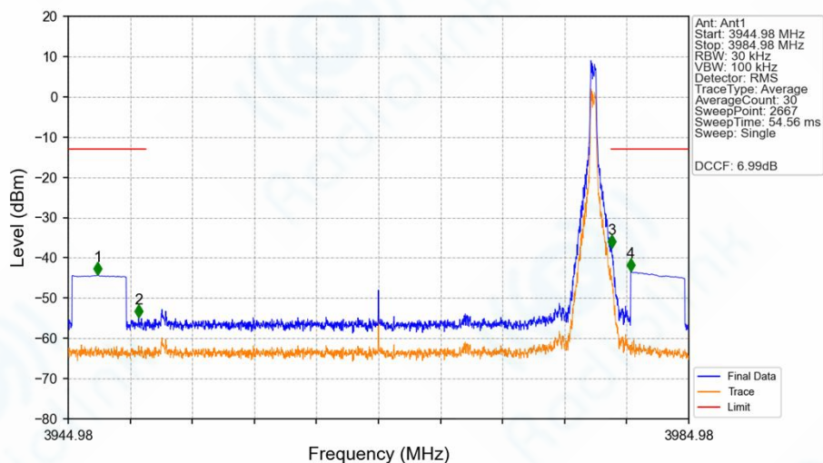
n77a_30kHz_SISO_NTNV_30MHz_DFT-s-OFDM PI/2 BPSK 3964.98MHz_Edge_1RB_Right_Ant1
