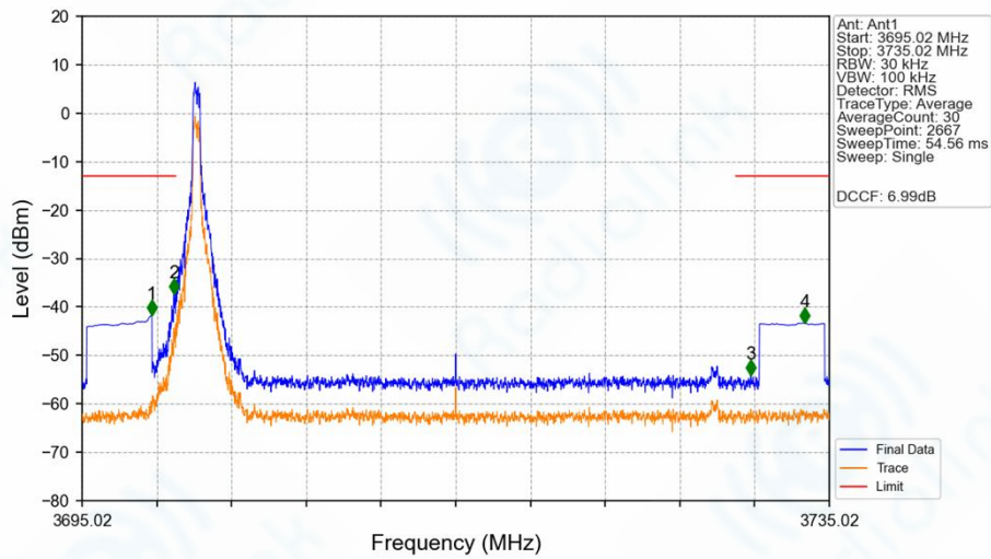
n77a_30kHz_SISO_NTNV_30MHz_DFT-s-OFDM_QPSK_3715.02MHz_Edge_1RB_Left_Ant1
