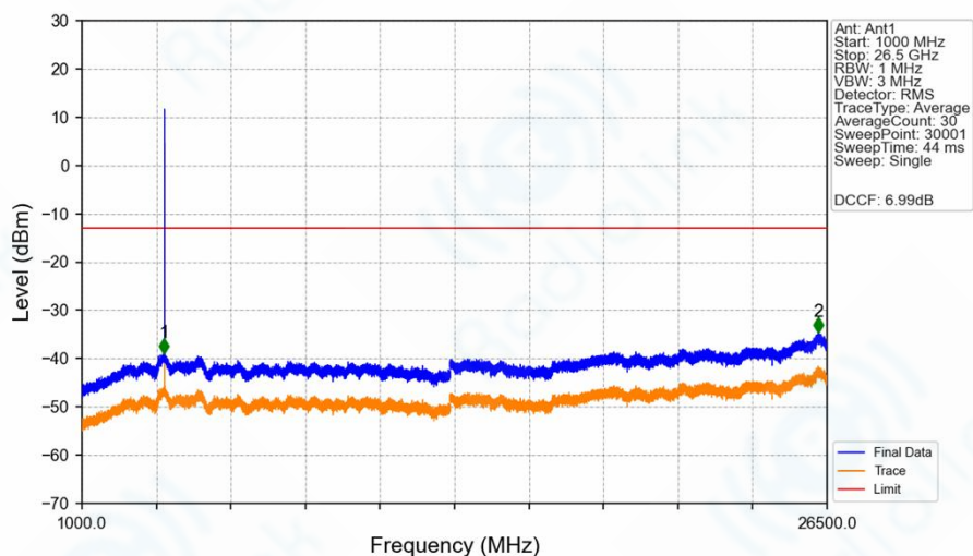
n77a_30kHz_SISO_NTNV_30MHz_DFT-s-OFDM PI/2 BPSK 3840MHz_Edge_1RB_Left_Ant1
