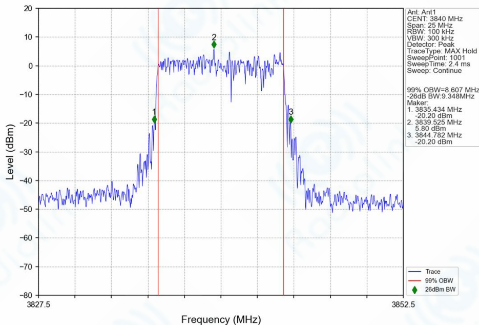
n77a_30kHz_SISO_NTNV_10MHz_DFT-s-OFDM_256_QAM_3840MHz_Outer_Full_Ant1
