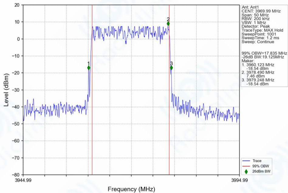
n77a_30kHz_SISO_NTNV_20MHz_DFT-s-OFDM_64_QAM_3969.99MHz_Outer_Full_Ant1
