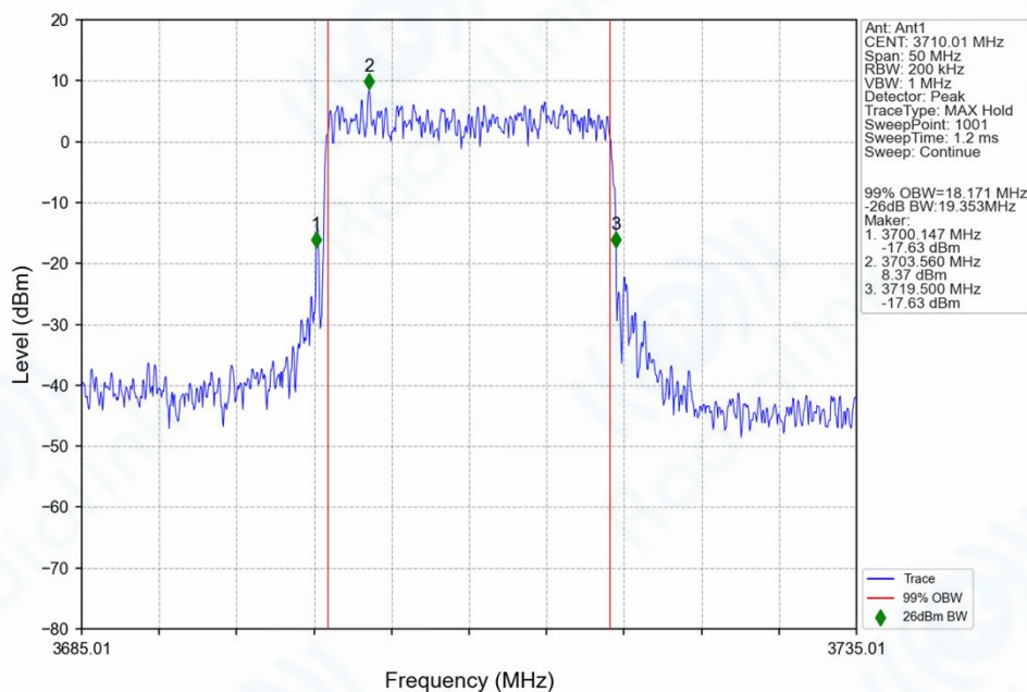
n77a_30kHz_SISO_NTNV_20MHz_CP-OFDM_QPSK_3710.01MHz_Outer_Full_Ant1
