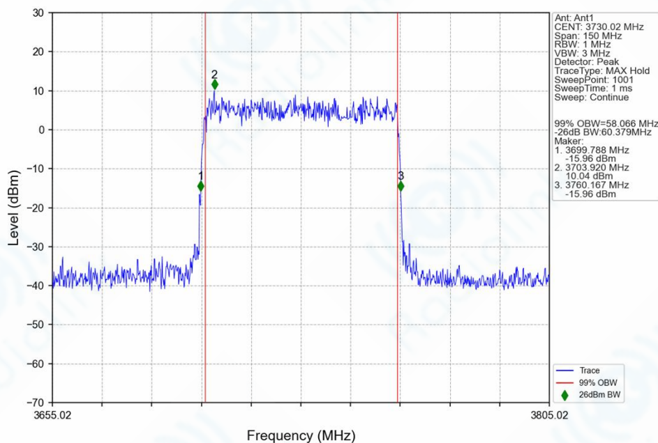
n77a_30kHz_SISO_NTNV_60MHz_DFT-s-OFDM_QPSK_3730.02MHz_Outer_Full_Ant1
