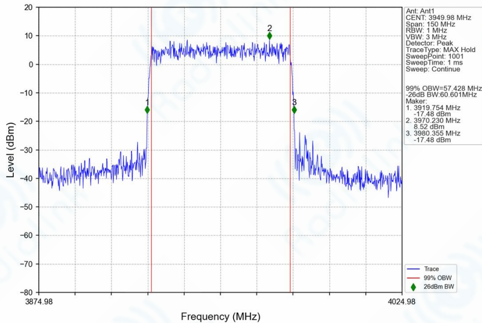
n77a_30kHz_SISO_NTNV_60MHz_DFT-s-OFDM_64_QAM_3949.98MHz_Outer_Full_Ant1
