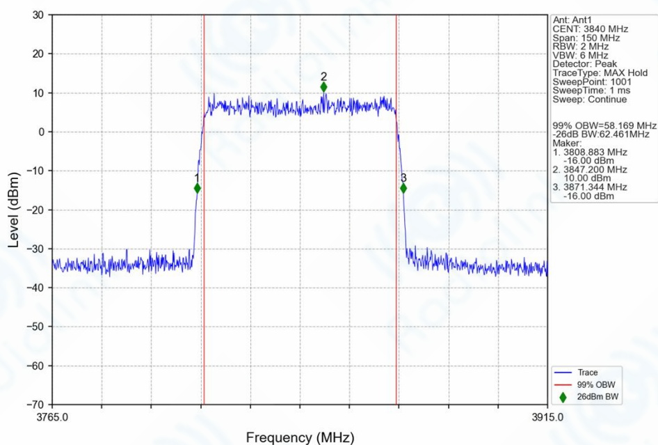
n77a_30kHz_SISO_NTNV_60MHz_CP-OFDM_256_QAM_3840MHz_Outer_Full_Ant1
