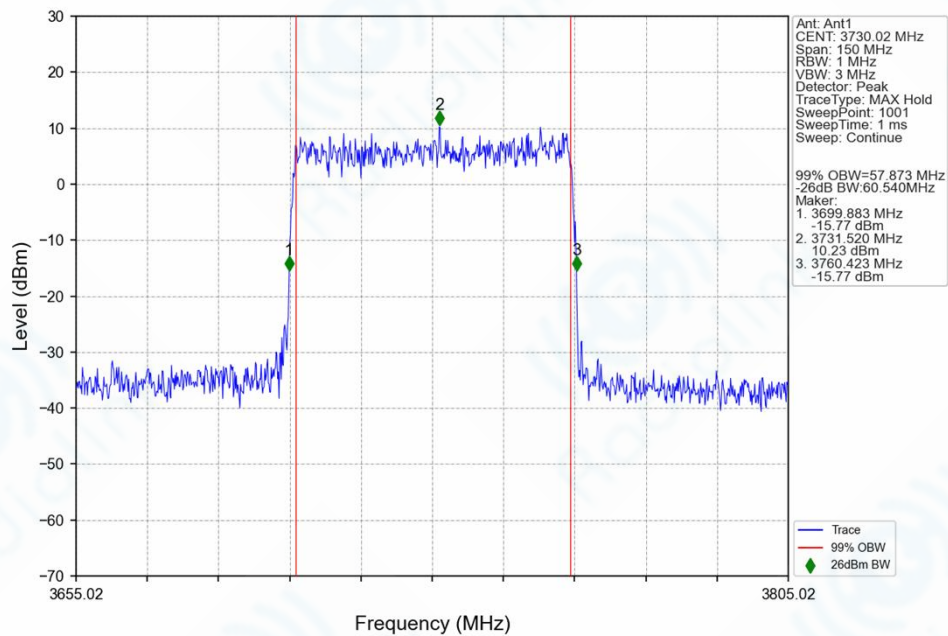
n77a_30kHz_SISO_NTNV_60MHz_DFT-s-OFDM_64_QAM_3730.02MHz_Outer_Full_Ant1
