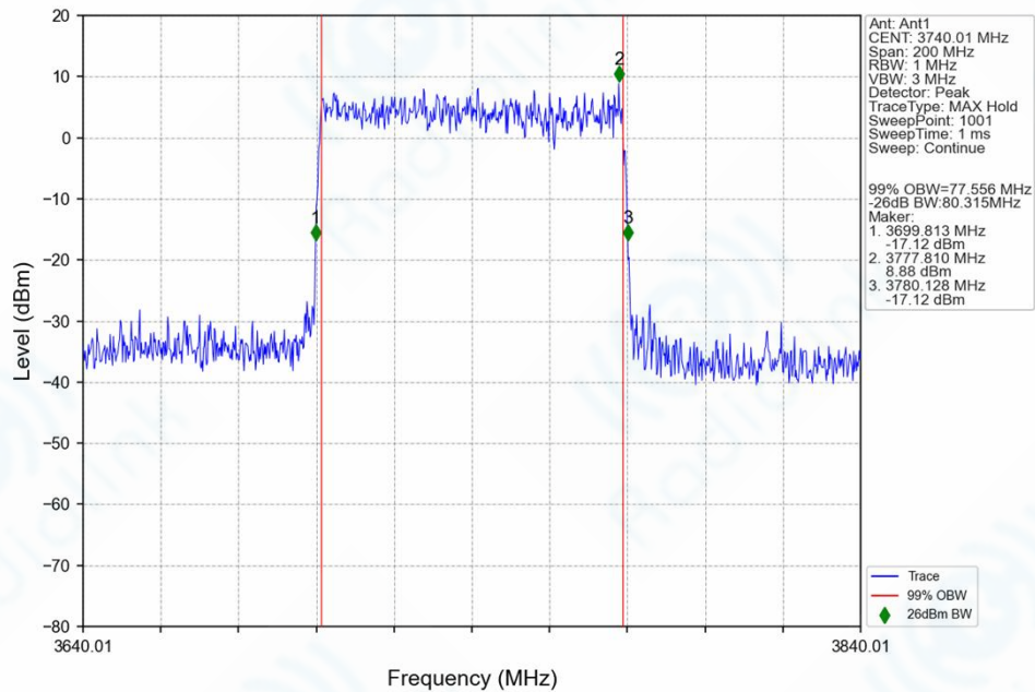
n77a_30kHz_SISO_NTNV_80MHz_CP-OFDM_64 QAM_3740.01MHz_Outer_Full_Ant1
