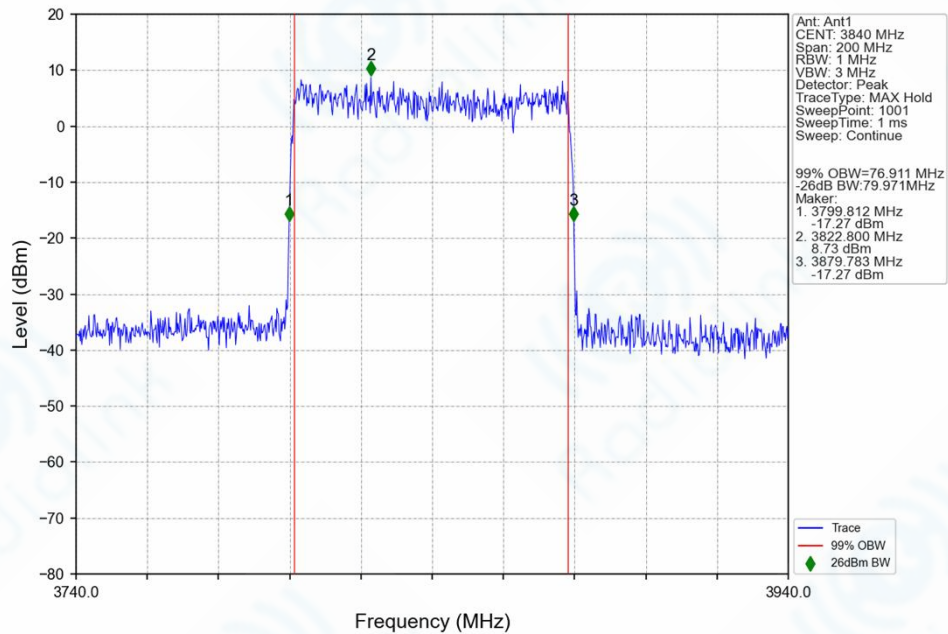
n77a_30kHz_SISO_NTNV_80MHz_DFT-s-OFDM_16_QAM_3840MHz_Outer_Full_Ant1
