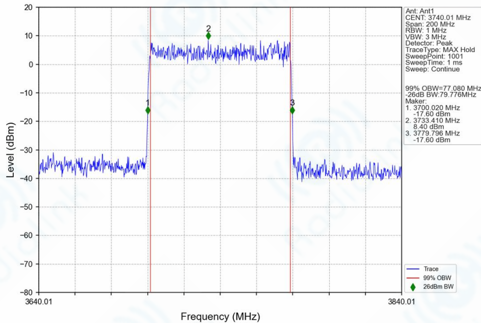
n77a_30kHz_SISO_NTNV_80MHz_DFT-s-OFDM_64_QAM_3740.01MHz_Outer_Full_Ant1
