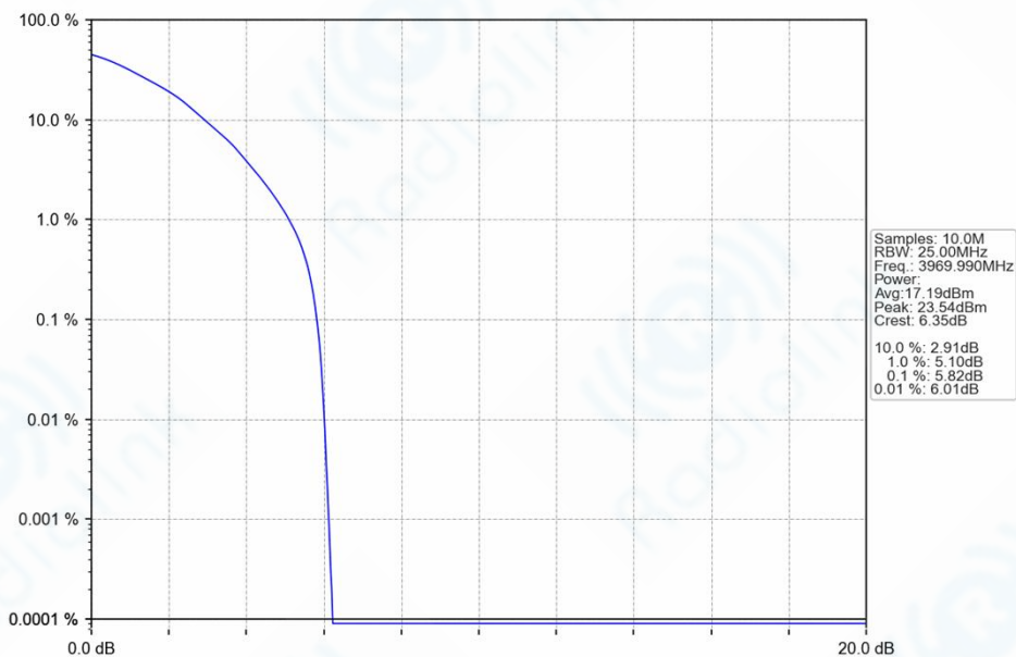
n77a_30kHz_SISO_NTNV_20MHz_DFT-s-OFDM_64_QAM_3969.99MHz_Outer_Full_Ant1
