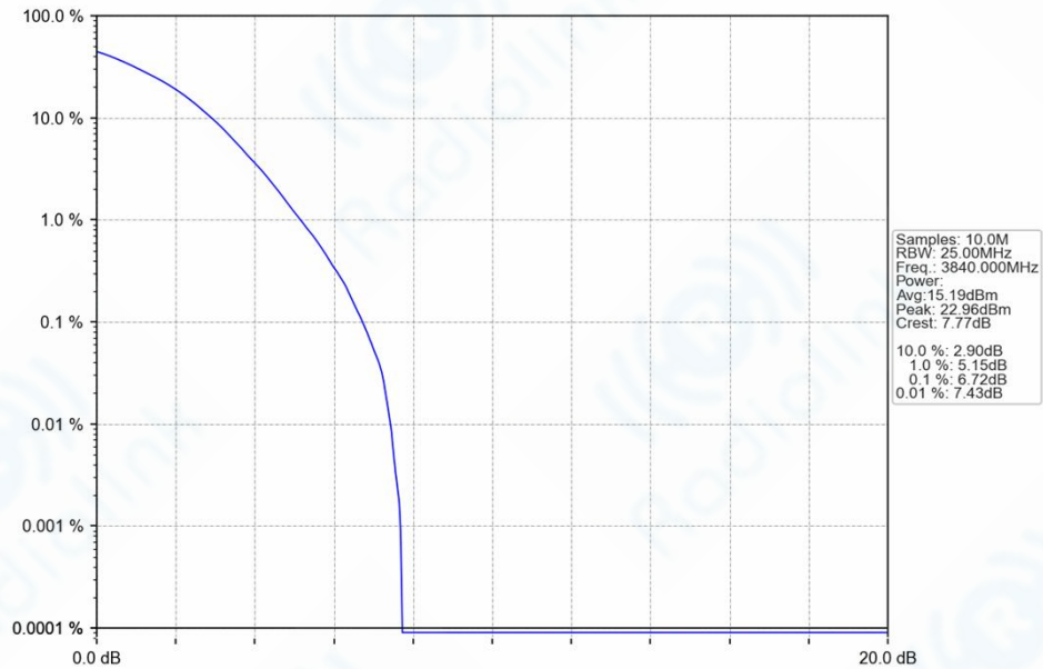
n77a_30kHz_SISO_NTNV_20MHz_DFT-s-OFDM_256_QAM_3840MHz_Outer_Full_Ant1
