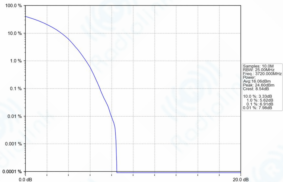
n77a_30kHz_SISO_NTNV_40MHz_DFT-s-OFDM_64_QAM_3720MHz_Outer_Full_Ant1
