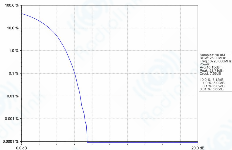
n77a_30kHz_SISO_NTNV_40MHz_DFT-s-OFDM QPSK_3720MHz_Outer_Full_Ant1
