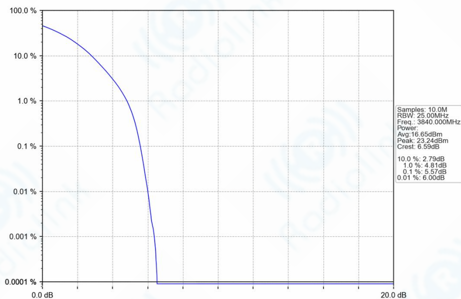
n77a_30kHz_SISO_NTNV_30MHz_DFT-s-OFDM_16_QAM_3840MHz_Outer_Full_Ant1
