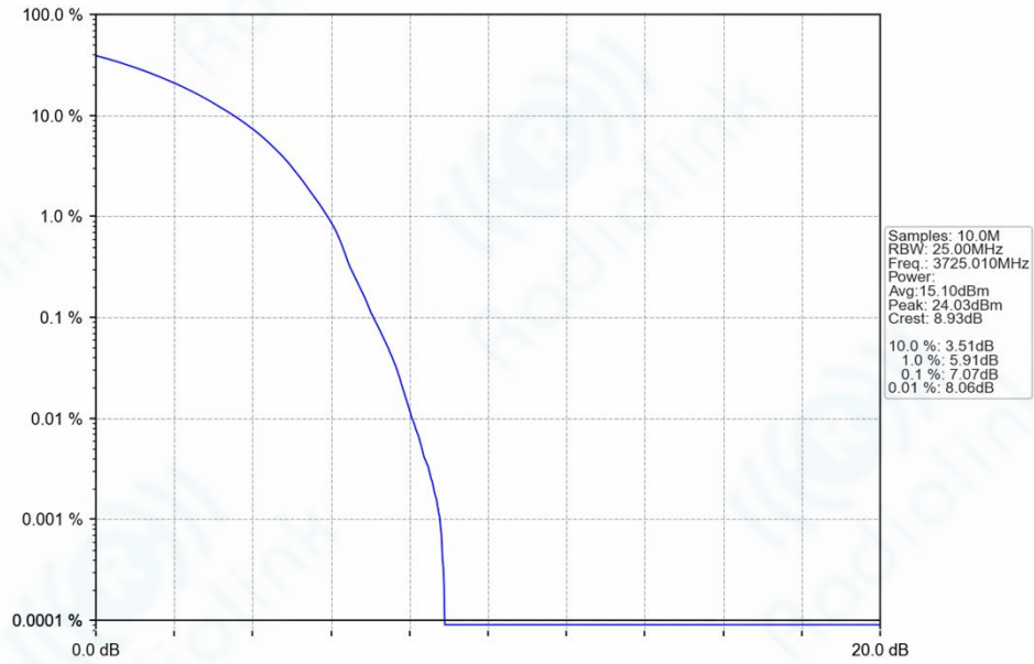
n77a_30kHz_SISO_NTNV_50MHz_DFT-s-OFDM_16_QAM_3725.01MHz_Outer_Full_Ant1
