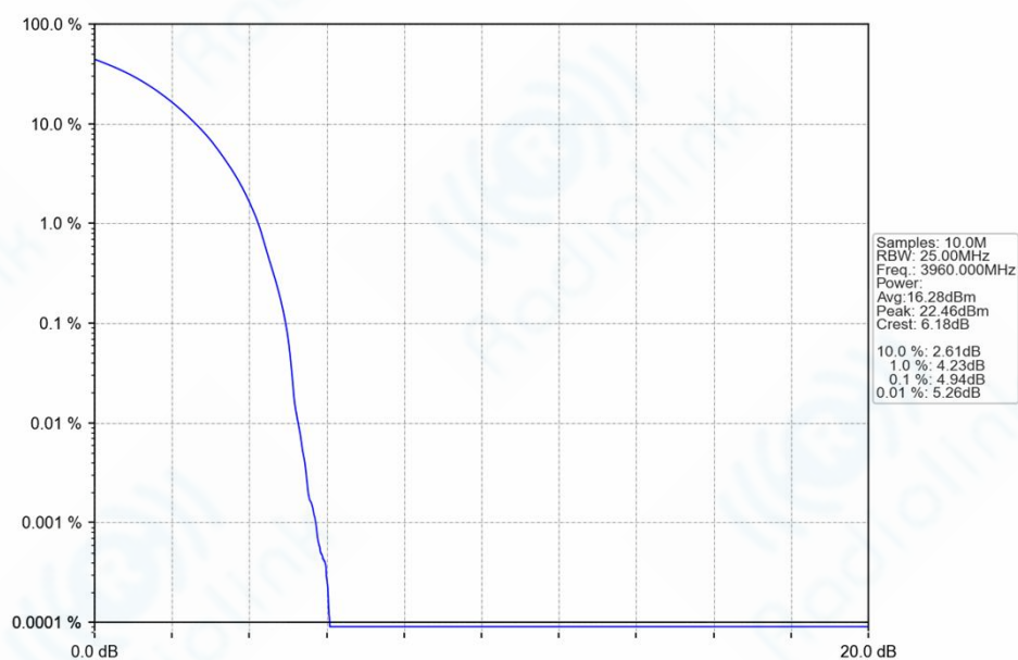
n77a_30kHz_SISO_NTNV_40MHz_DFT-s-OFDM PI/2 BPSK_3960MHz_Outer_Full_Ant1
