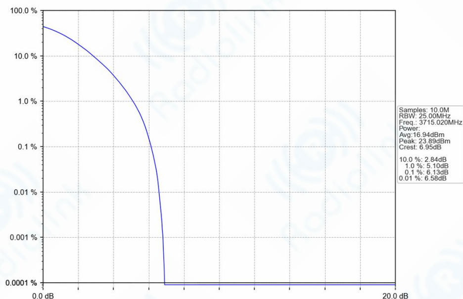
n77a_30kHz_SISO_NTNV_30MHz_DFT-s-OFDM_64_QAM_3715.02MHz_Outer_Full_Ant1
