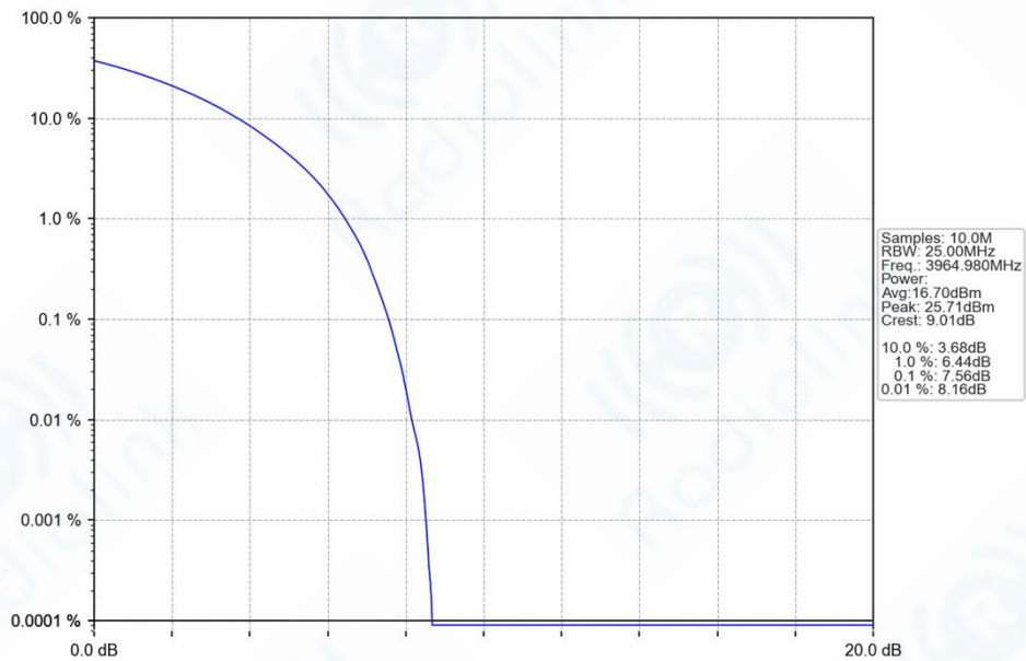
n77a_30kHz_SISO_NTNV_30MHz_CP-OFDM_64_QAM_3964.98MHz_Outer_Full_Ant1
