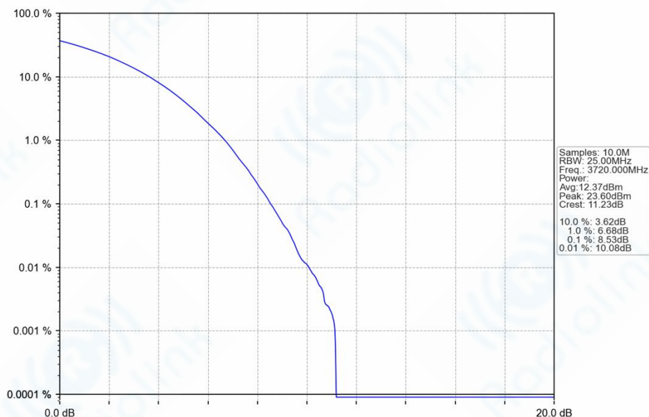
n77a_30kHz_SISO_NTNV_40MHz_CP-OFDM_256_QAM_3720MHz_Outer_Full_Ant1
