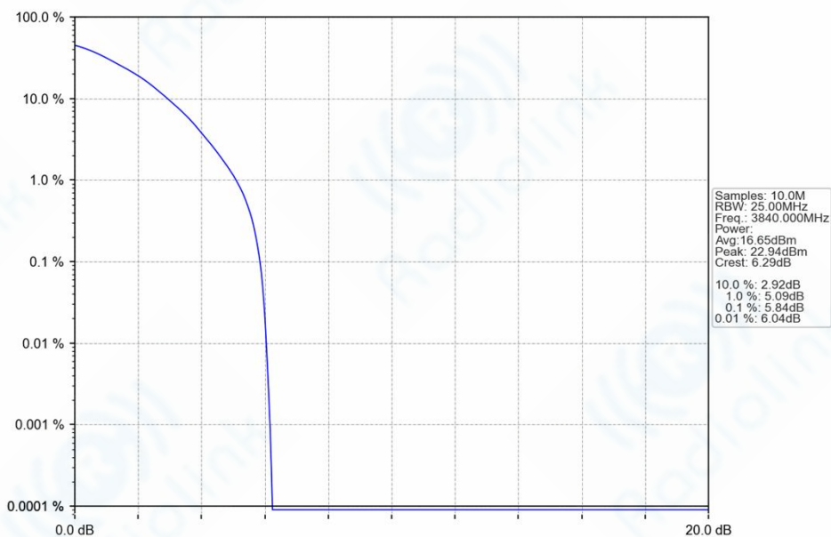
n77a_30kHz_SISO_NTNV_20MHz_DFT-s-OFDM_64_QAM_3840MHz_Outer_Full_Ant1
