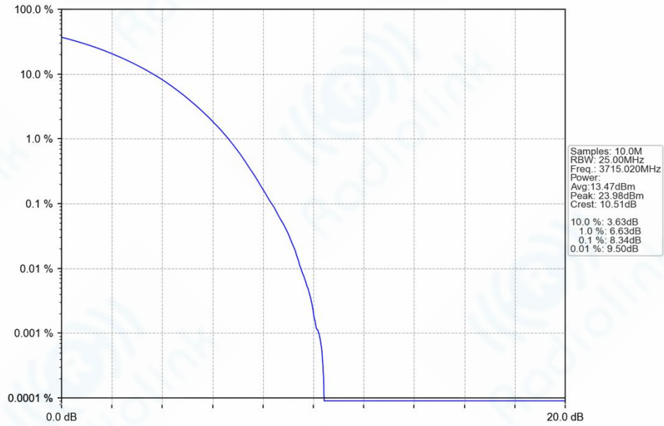
n77a_30kHz_SISO_NTNV_30MHz_CP-OFDM_256_QAM_3715.02MHz_Outer_Full_Ant1
