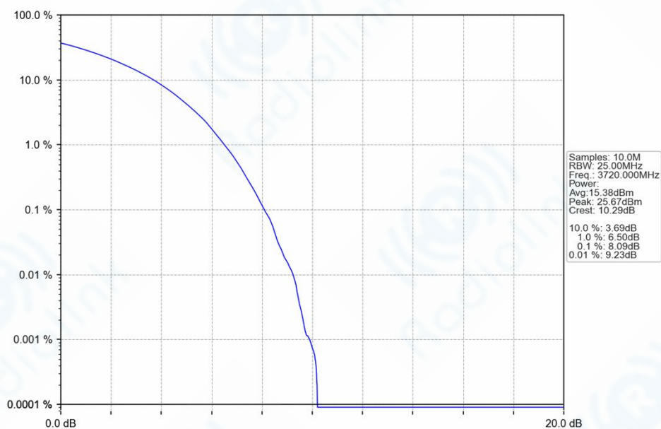
n77a_30kHz_SISO_NTNV_40MHz_CP-OFDM 64 QAM 3720MHz_Outer_Full_Ant1
