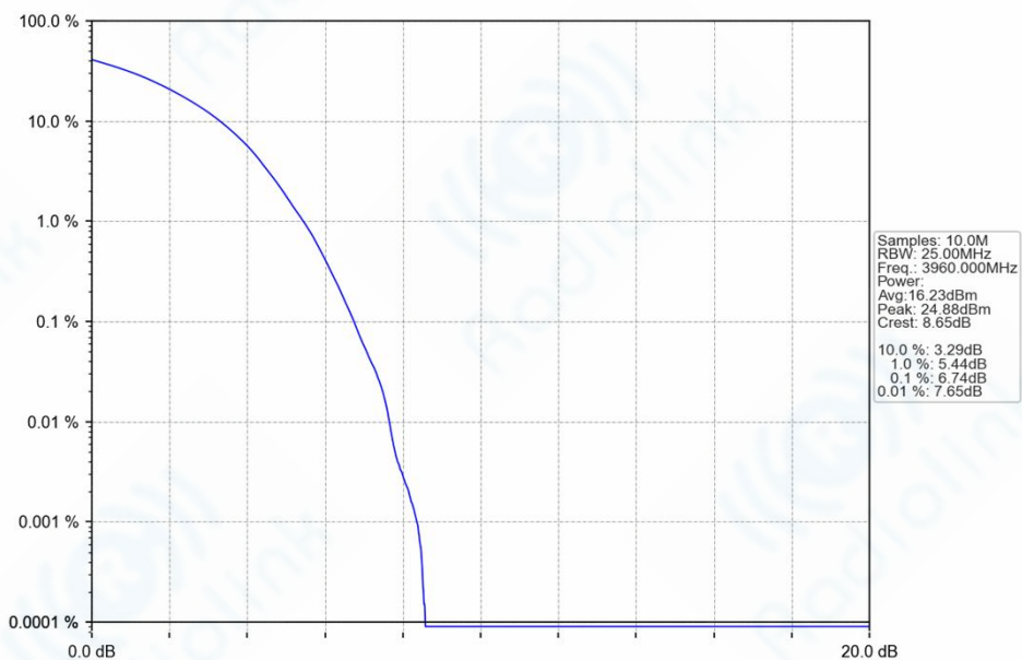
n77a_30kHz_SISO_NTNV_40MHz_DFT-s-OFDM_16_QAM_3960MHz_Outer_Full_Ant1
