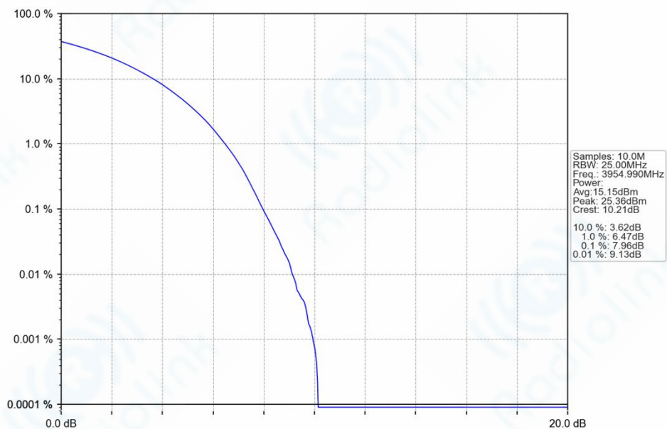
n77a_30kHz_SISO_NTNV_50MHz_CP-OFDM_16_QAM_3954.99MHz_Outer_Full_Ant1
