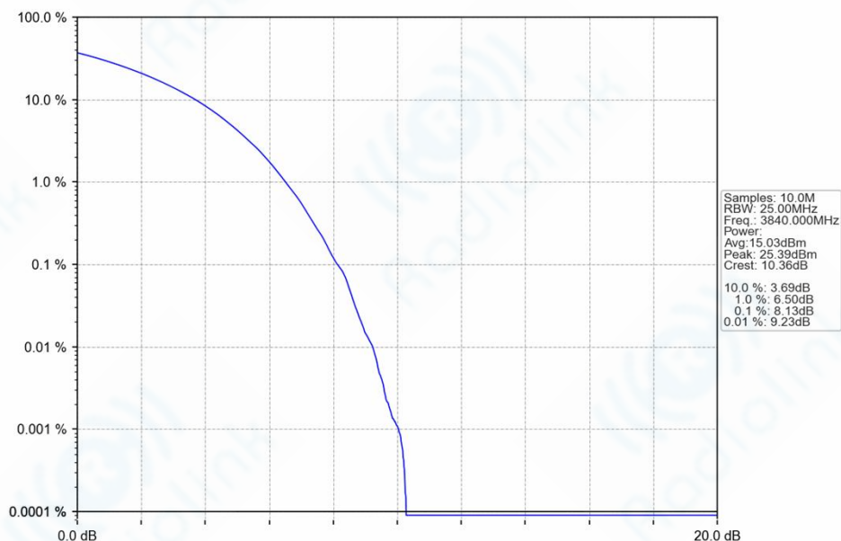
n77a_30kHz_SISO_NTNV_40MHz_CP-OFDM_64_QAM_3840MHz_Outer_Full_Ant1
