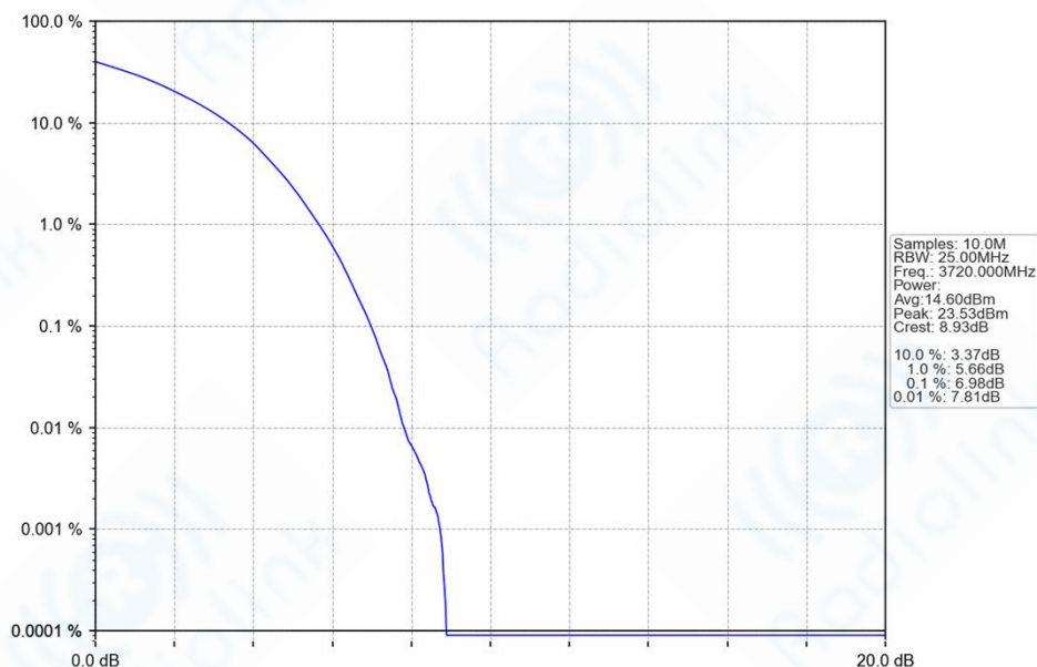
n77a_30kHz_SISO_NTNV_40MHz_DFT-s-OFDM_256_QAM_3720MHz_Outer_Full_Ant1
