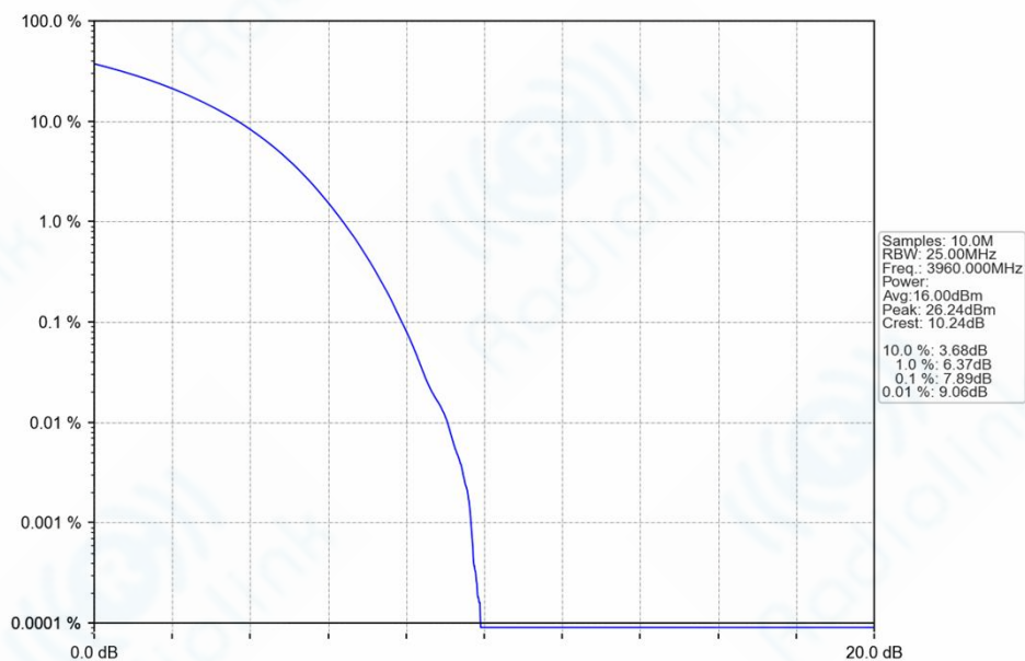
n77a_30kHz_SISO_NTNV_40MHz_CP-OFDM 16 QAM 3960MHz_Outer_Full_Ant1
