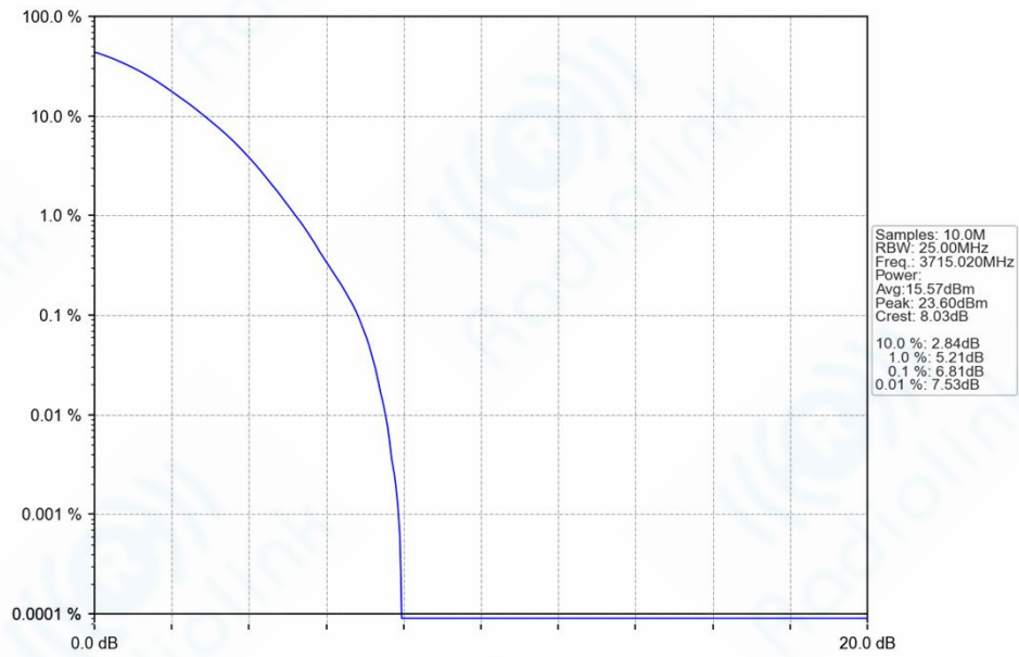
n77a_30kHz_SISO_NTNV_30MHz_DFT-s-OFDM_256_QAM_3715.02MHz_Outer_Full_Ant1
