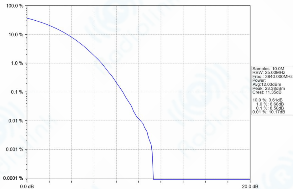
n77a_30kHz_SISO_NTNV_40MHz_CP-OFDM_256_QAM_3840MHz_Outer_Full_Ant1
