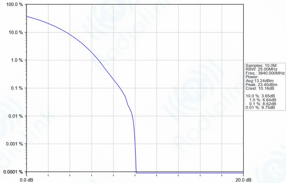
n77a_30kHz_SISO_NTNV_20MHz_CP-OFDM_256_QAM_3840MHz_Outer_Full_Ant1
