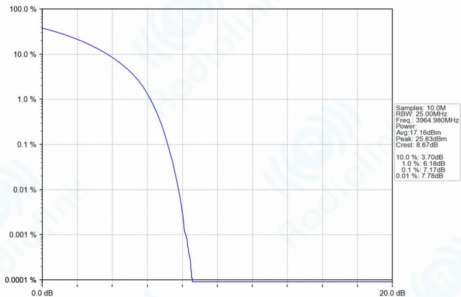
n77a_30kHz_SISO_NTNV_30MHz_CP-OFDM_QPSK_3964.98MHz_Outer_Full_Ant1
