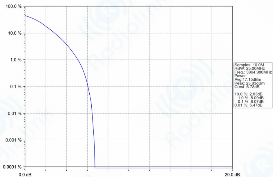
n77a_30kHz_SISO_NTNV_30MHz_DFT-s-OFDM_64_QAM_3964.98MHz_Outer_Full_Ant1
