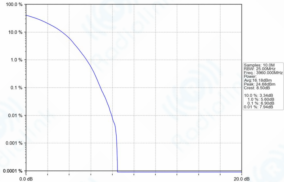
n77a_30kHz_SISO_NTNV_40MHz_DFT-s-OFDM_64_QAM_3960MHz_Outer_Full_Ant1
