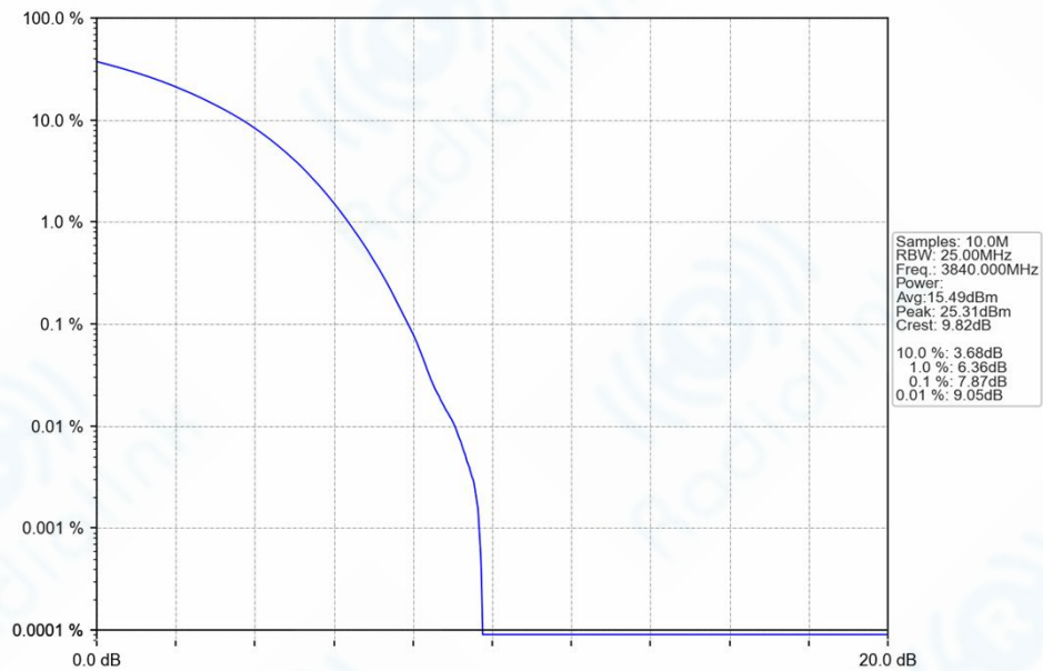
n77a_30kHz_SISO_NTNV_40MHz_CP-OFDM_16_QAM_3840MHz_Outer_Full_Ant1
