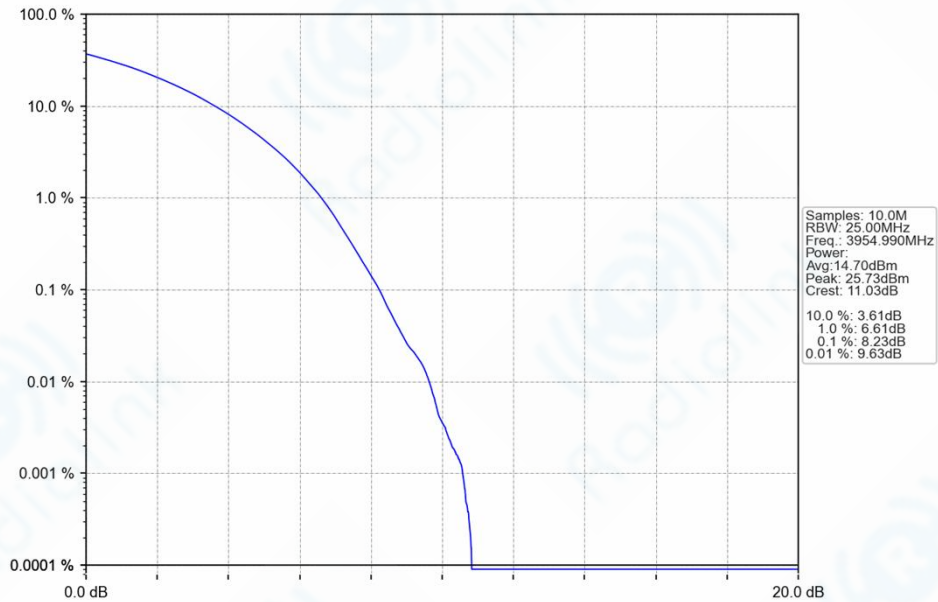
n77a_30kHz_SISO_NTNV_50MHz_CP-OFDM_64_QAM_3954.99MHz_Outer_Full_Ant1
