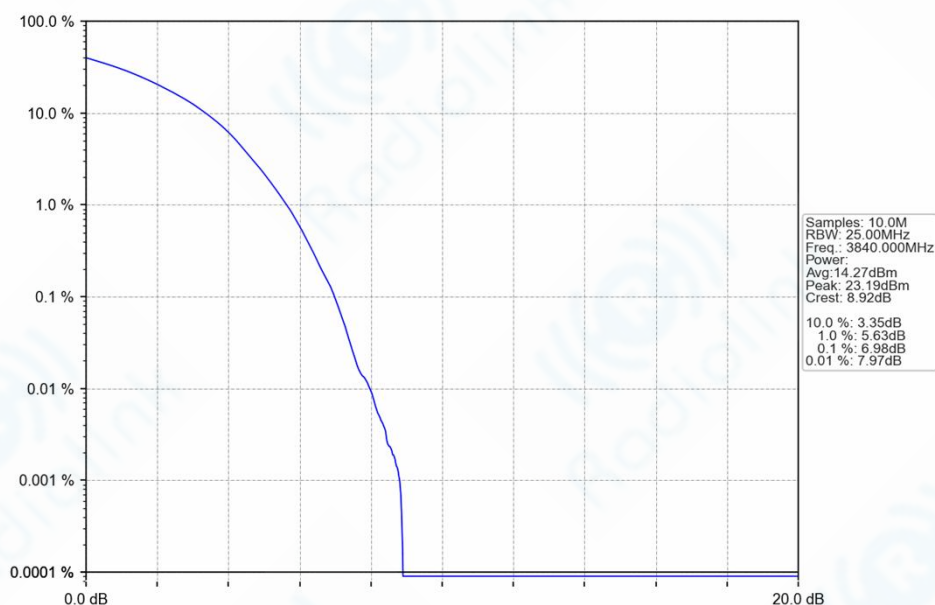
n77a_30kHz_SISO_NTNV_40MHz_DFT-s-OFDM_256_QAM_3840MHz_Outer_Full_Ant1
