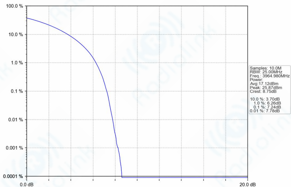
n77a_30kHz_SISO_NTNV_30MHz_CP-OFDM_16_QAM_3964.98MHz_Outer_Full_Ant1
