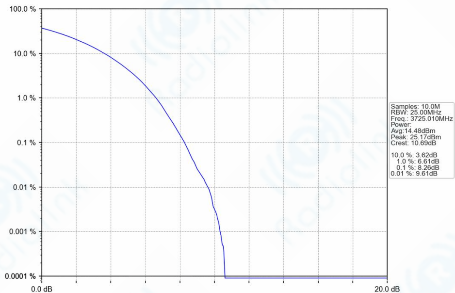
n77a_30kHz_SISO_NTNV_50MHz_CP-OFDM_64_QAM_3725.01MHz_Outer_Full_Ant1
