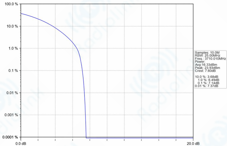
n77a_30kHz_SISO_NTNV_20MHz_CP-OFDM_64_QAM_3710.01MHz_Outer_Full_Ant1
