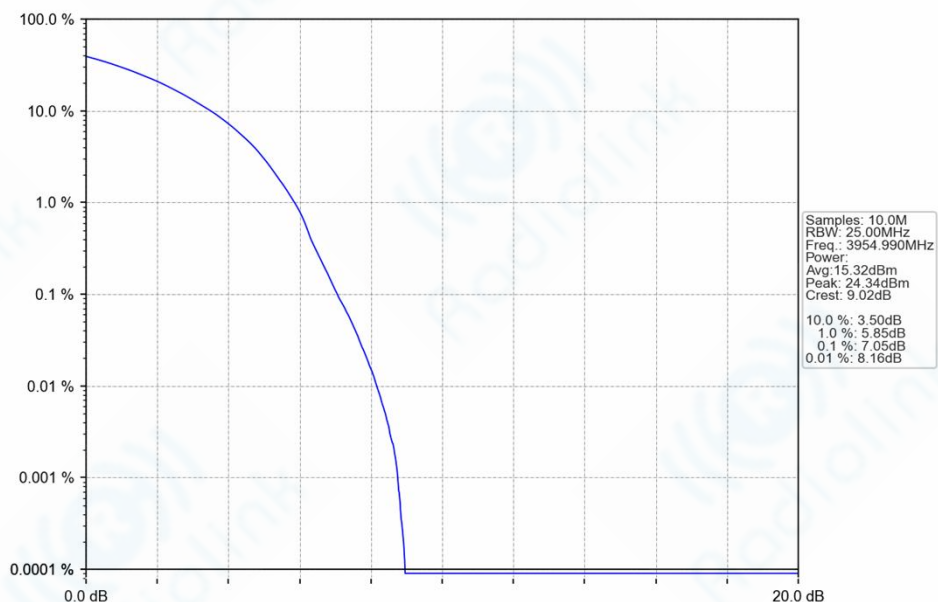
n77a_30kHz_SISO_NTNV_50MHz_DFT-s-OFDM_16_QAM_3954.99MHz_Outer_Full_Ant1
