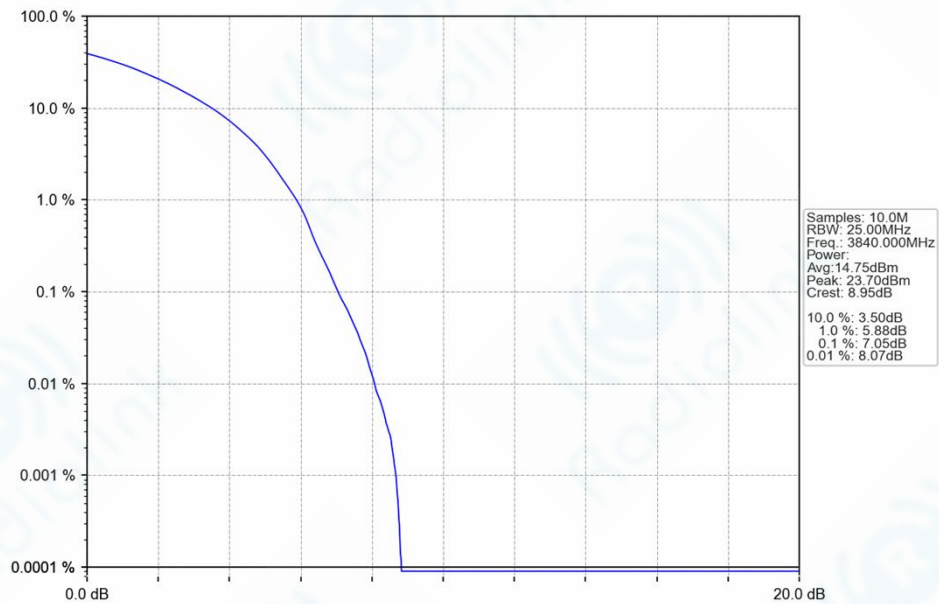
n77a_30kHz_SISO_NTNV_50MHz_DFT-s-OFDM_16_QAM_3840MHz_Outer_Full_Ant1
