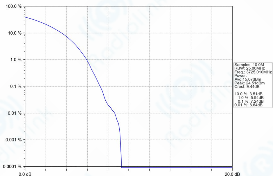
n77a_30kHz_SISO_NTNV_50MHz_DFT-s-OFDM_64_QAM_3725.01MHz_Outer_Full_Ant1
