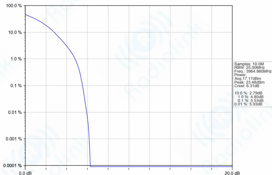
n77a_30kHz_SISO_NTNV_30MHz_DFT-s-OFDM_16_QAM_3964.98MHz_Outer_Full_Ant1
