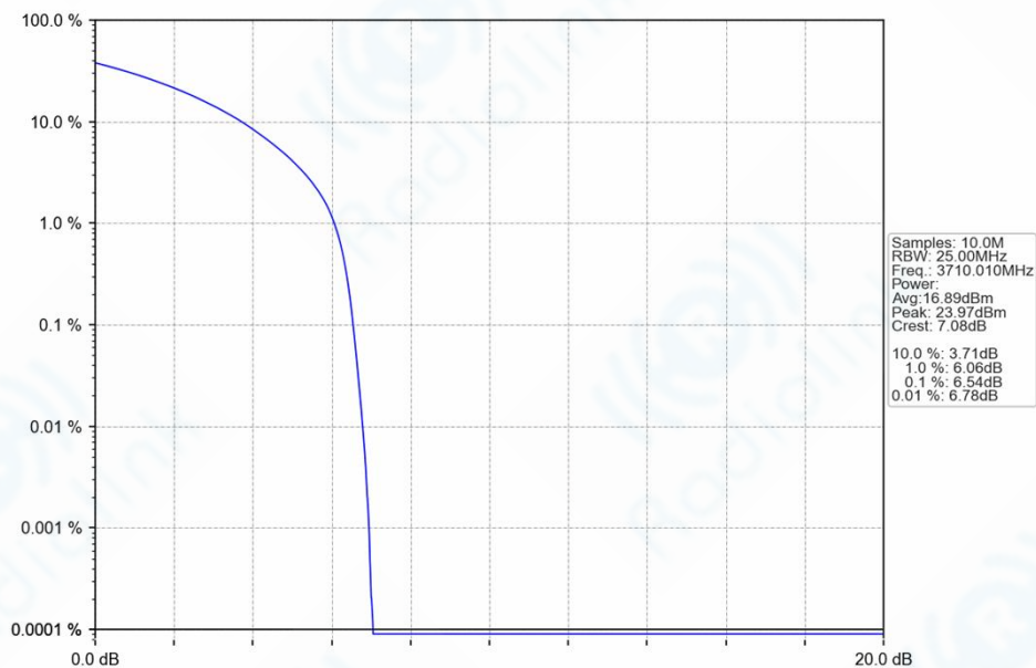
n77a_30kHz_SISO_NTNV_20MHz_CP-OFDM_QPSK_3710.01MHz_Outer_Full_Ant1
