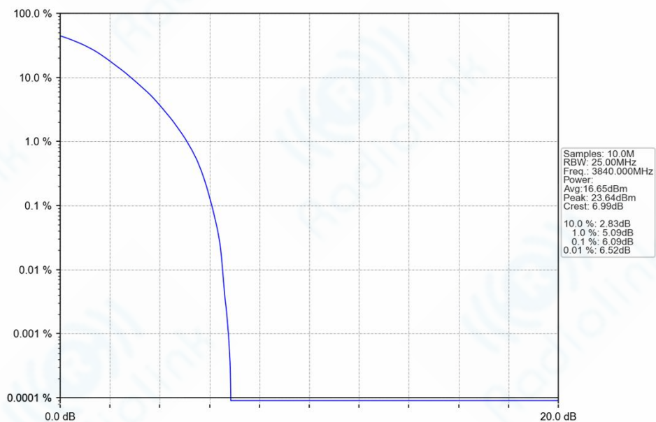
n77a_30kHz_SISO_NTNV_30MHz_DFT-s-OFDM_64_QAM_3840MHz_Outer_Full_Ant1
