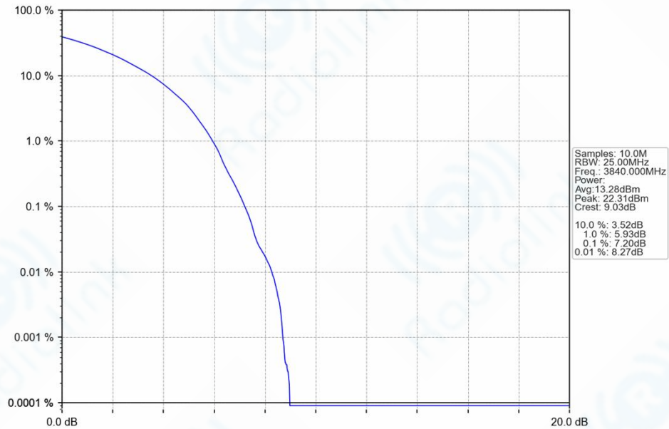
n77a_30kHz_SISO_NTNV_50MHz_DFT-s-OFDM_256_QAM_3840MHz_Outer_Full_Ant1
