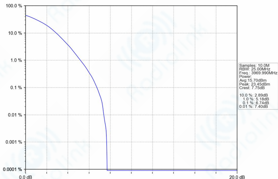
n77a_30kHz_SISO_NTNV_20MHz_DFT-s-OFDM_256_QAM_3969.99MHz_Outer_Full_Ant1
