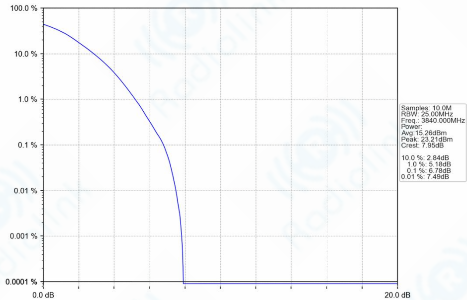
n77a_30kHz_SISO_NTNV_30MHz_DFT-s-OFDM_256_QAM_3840MHz_Outer_Full_Ant1
