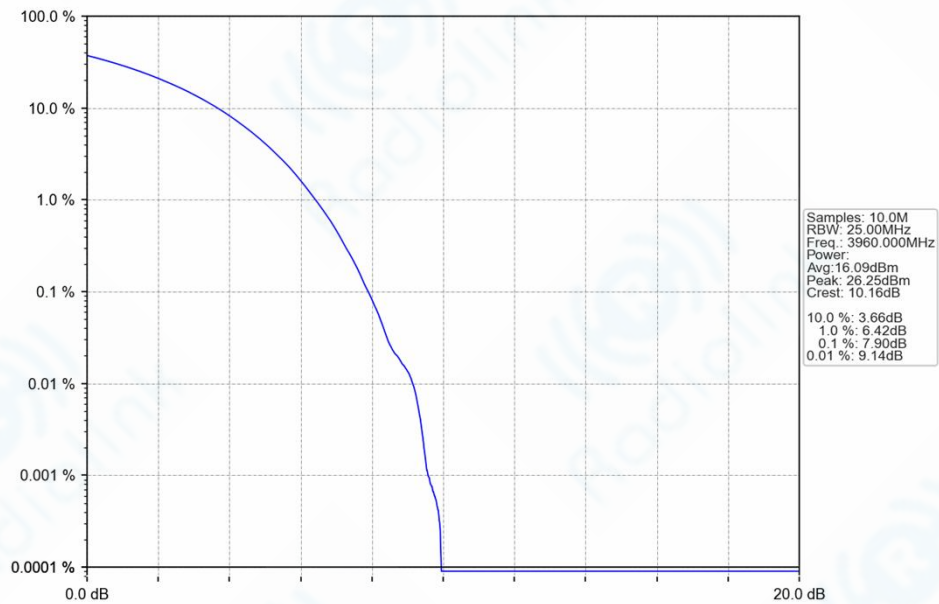
n77a_30kHz_SISO_NTNV_40MHz_CP-OFDM_QPSK_3960MHz_Outer_Full_Ant1
