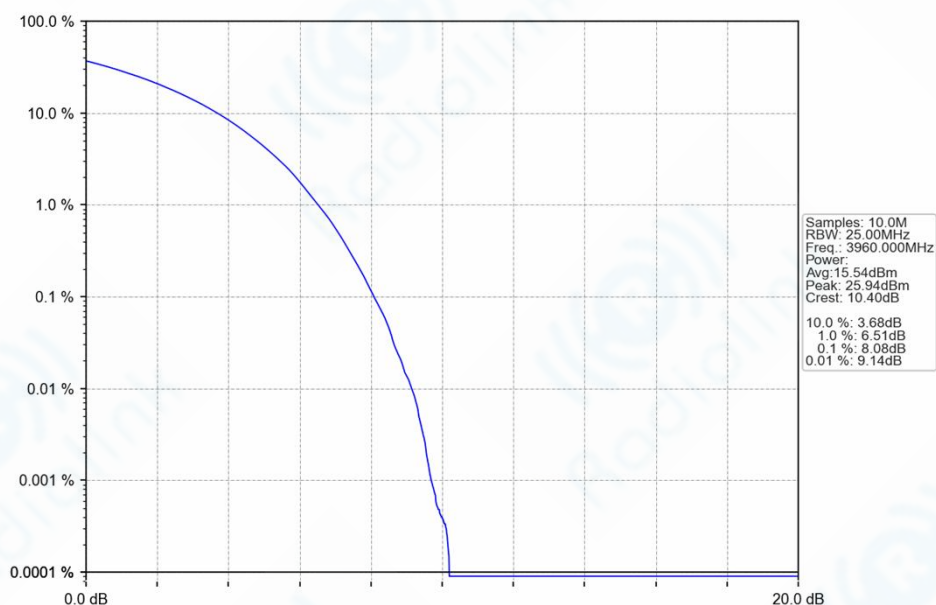
n77a_30kHz_SISO_NTNV_40MHz_CP-OFDM_64_QAM_3960MHz_Outer_Full_Ant1
