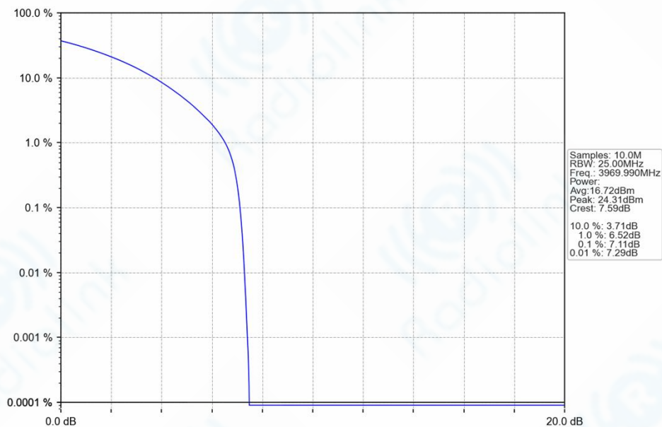
n77a_30kHz_SISO_NTNV_20MHz_CP-OFDM_64_QAM_3969.99MHz_Outer_Full_Ant1
