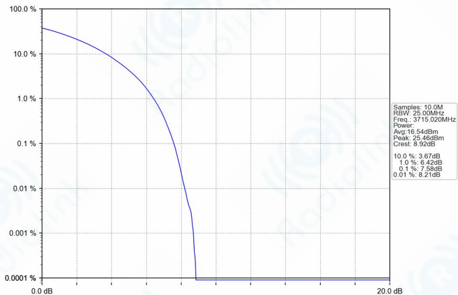
n77a_30kHz_SISO_NTNV_30MHz_CP-OFDM_64_QAM_3715.02MHz_Outer_Full_Ant1
