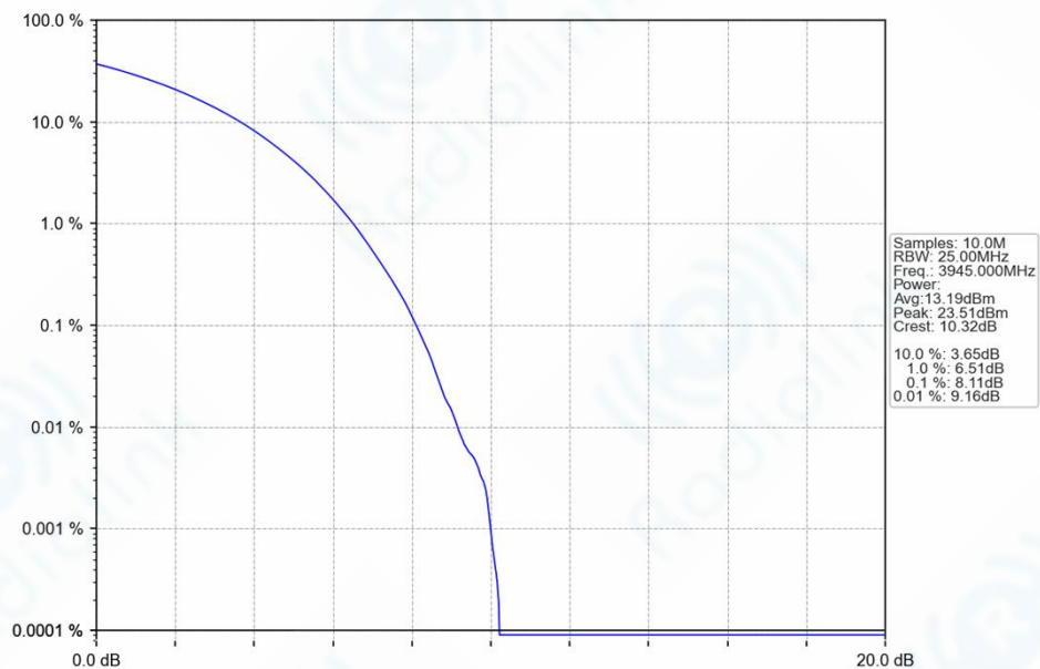
n77a_30kHz_SISO_NTNV_70MHz_CP-OFDM_QPSK_3945MHz_Outer_Full_Ant1
