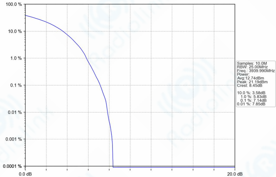
n77a_30kHz_SISO_NTNV_80MHz_DFT-s-OFDM_QPSK_3939.99MHz_Outer_Full_Ant1
