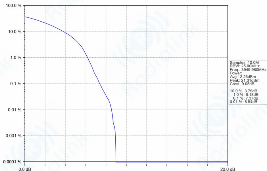
n77a_30kHz_SISO_NTNV_60MHz_DFT-s-OFDM_256_QAM_3949.98MHz_Outer_Full_Ant1
