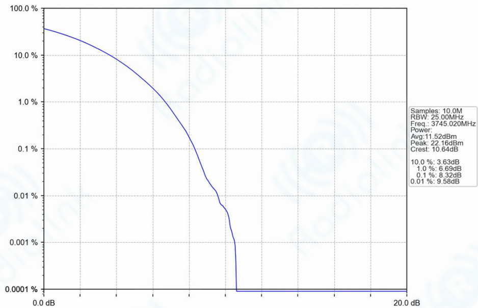
n77a_30kHz_SISO_NTNV_90MHz_CP-OFDM_64_QAM_3745.02MHz_Outer_Full_Ant1
