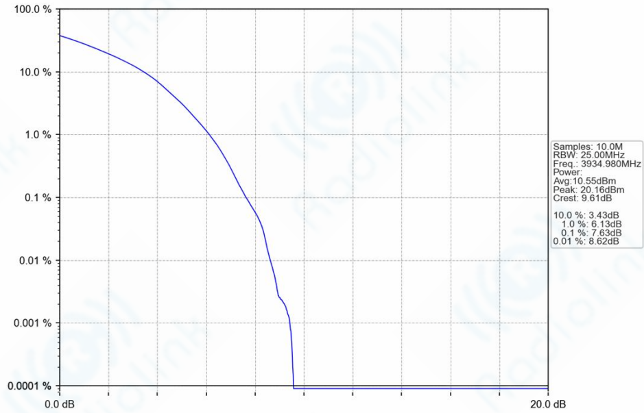
n77a_30kHz_SISO_NTNV_90MHz_DFT-s-OFDM_256_QAM_3934.98MHz_Outer_Full_Ant1
