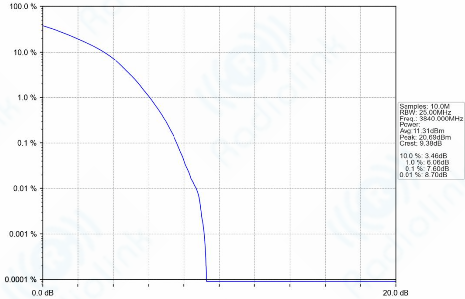
n77a_30kHz_SISO_NTNV_90MHz_DFT-s-OFDM_64_QAM_3840MHz_Outer_Full_Ant1
