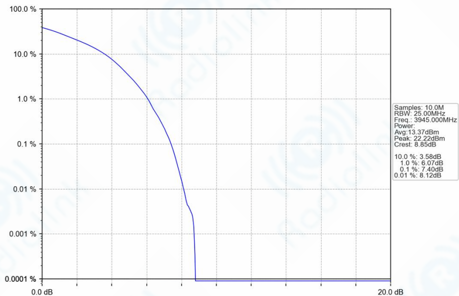
n77a_30kHz_SISO_NTNV_70MHz_DFT-s-OFDM_64_QAM_3945MHz_Outer_Full_Ant1
