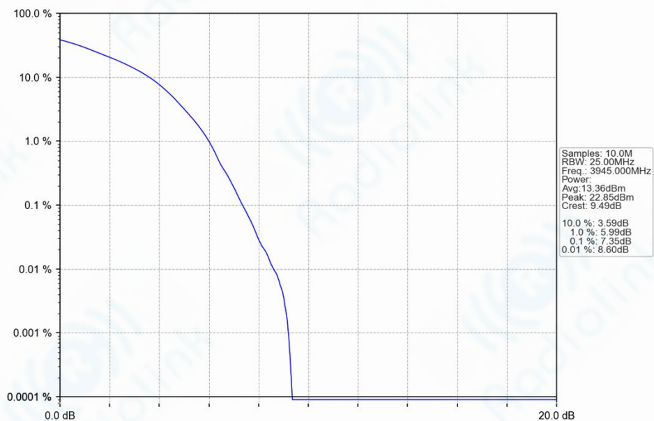
n77a_30kHz_SISO_NTNV_70MHz_DFT-s-OFDM_16_QAM_3945MHz_Outer_Full_Ant1
