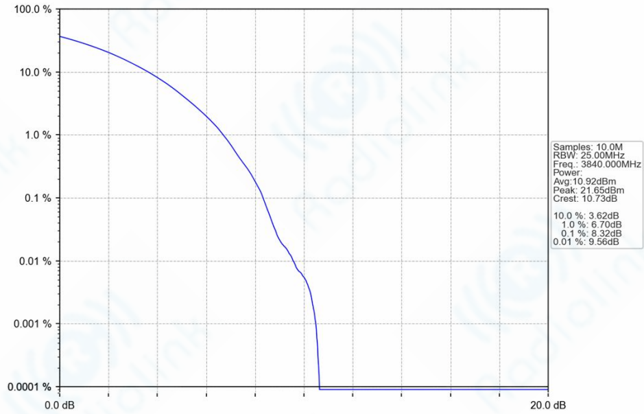
n77a_30kHz_SISO_NTNV_90MHz_CP-OFDM_64_QAM_3840MHz_Outer_Full_Ant1
