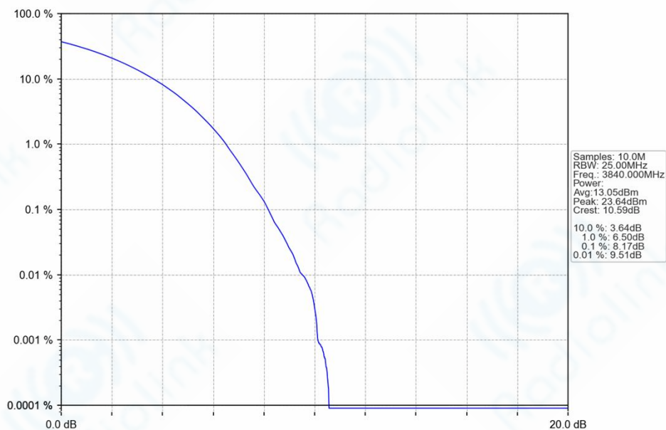
n77a_30kHz_SISO_NTNV_60MHz_CP-OFDM_64_QAM_3840MHz_Outer_Full_Ant1
