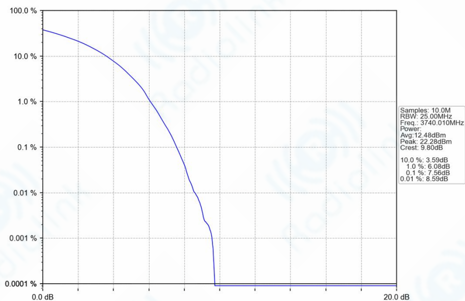
n77a_30kHz_SISO_NTNV_80MHz_DFT-s-OFDM_64_QAM_3740.01MHz_Outer_Full_Ant1
