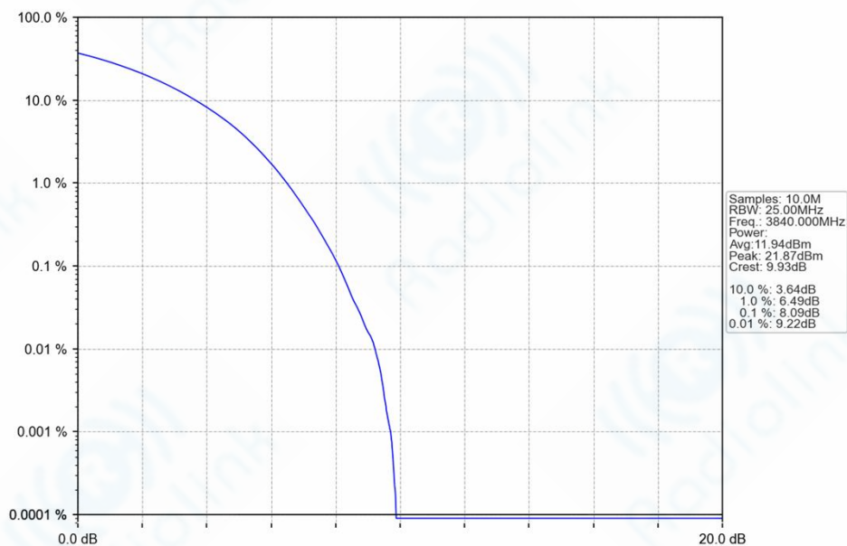
n77a_30kHz_SISO_NTNV_80MHz_CP-OFDM_QPSK_3840MHz_Outer_Full_Ant1
