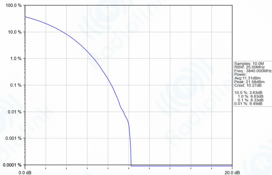
n77a_30kHz_SISO_NTNV_90MHz_CP-OFDM_16_QAM_3840MHz_Outer_Full_Ant1
