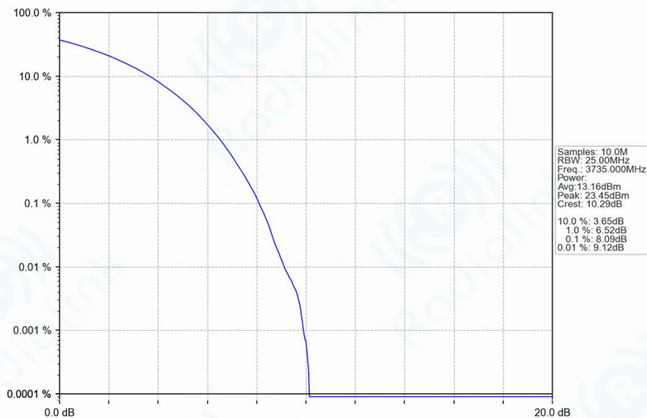
n77a_30kHz_SISO_NTNV_70MHz_CP-OFDM_QPSK_3735MHz_Outer_Full_Ant1
