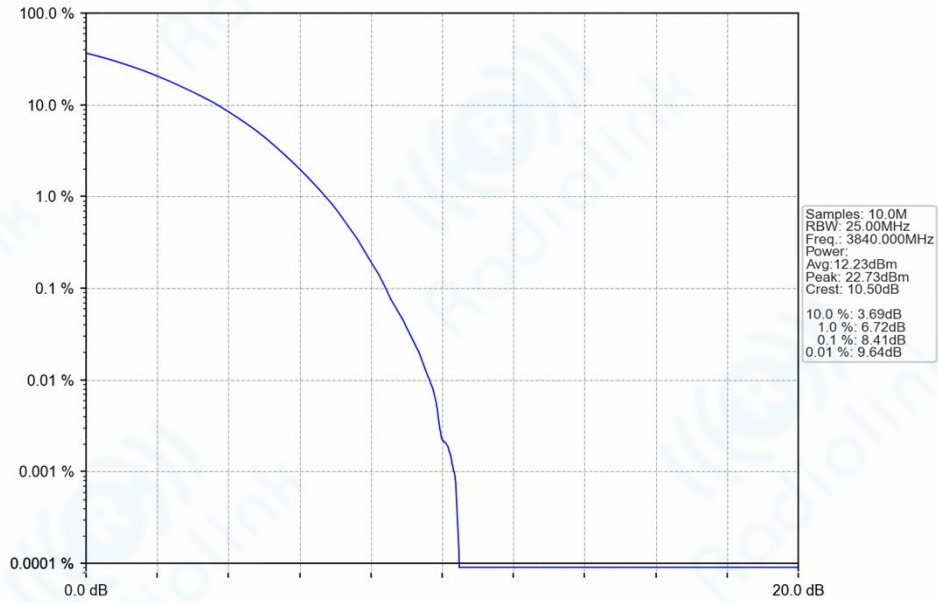
n77a_30kHz_SISO_NTNV_70MHz_CP-OFDM 64 QAM 3840MHz_Outer_Full_Ant1
