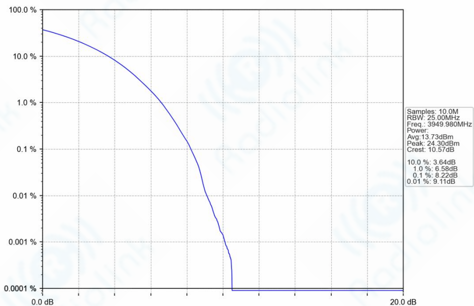
n77a_30kHz_SISO_NTNV_60MHz_CP-OFDM_16_QAM_3949.98MHz_Outer_Full_Ant1
