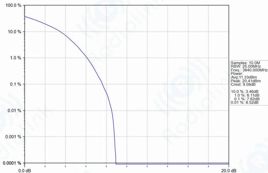
n77a_30kHz_SISO_NTNV_90MHz_DFT-s-OFDM_16_QAM_3840MHz_Outer_Full_Ant1
