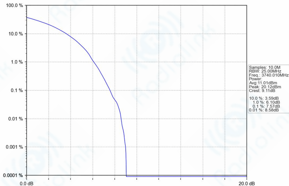
n77a_30kHz_SISO_NTNV_80MHz_DFT-s-OFDM_256_QAM_3740.01MHz_Outer_Full_Ant1
