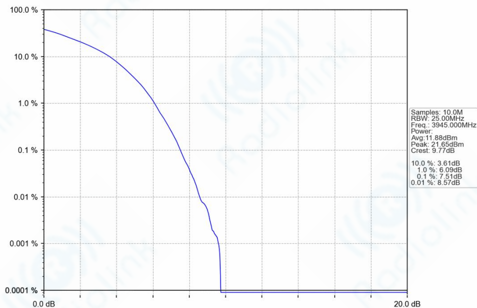
n77a_30kHz_SISO_NTNV_70MHz_DFT-s-OFDM_256_QAM_3945MHz_Outer_Full_Ant1
