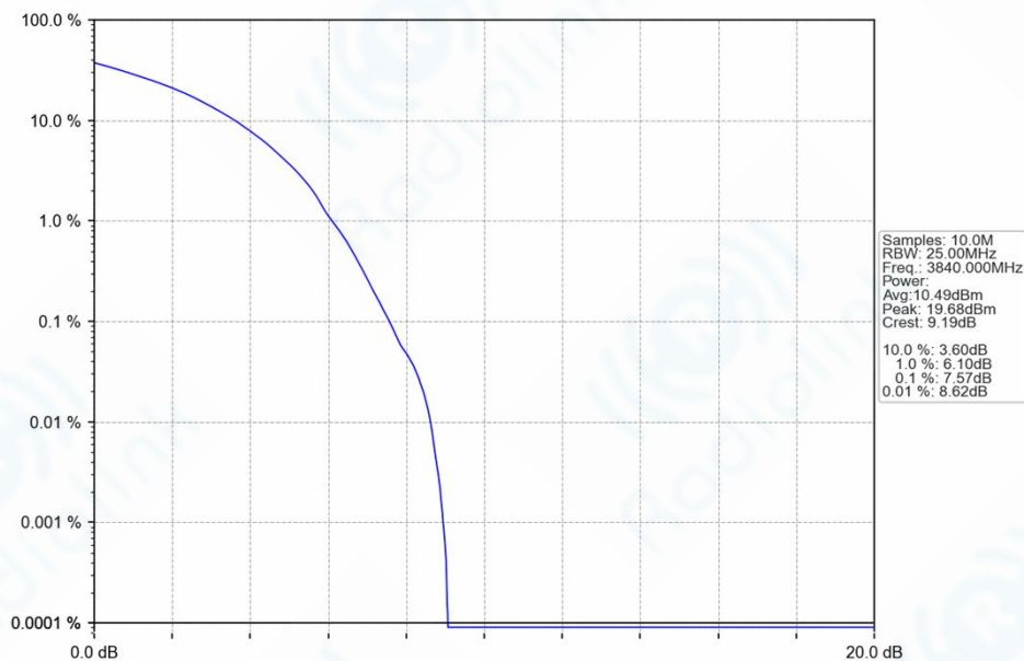
n77a_30kHz_SISO_NTNV_80MHz_DFT-s-OFDM_256_QAM_3840MHz_Outer_Full_Ant1
