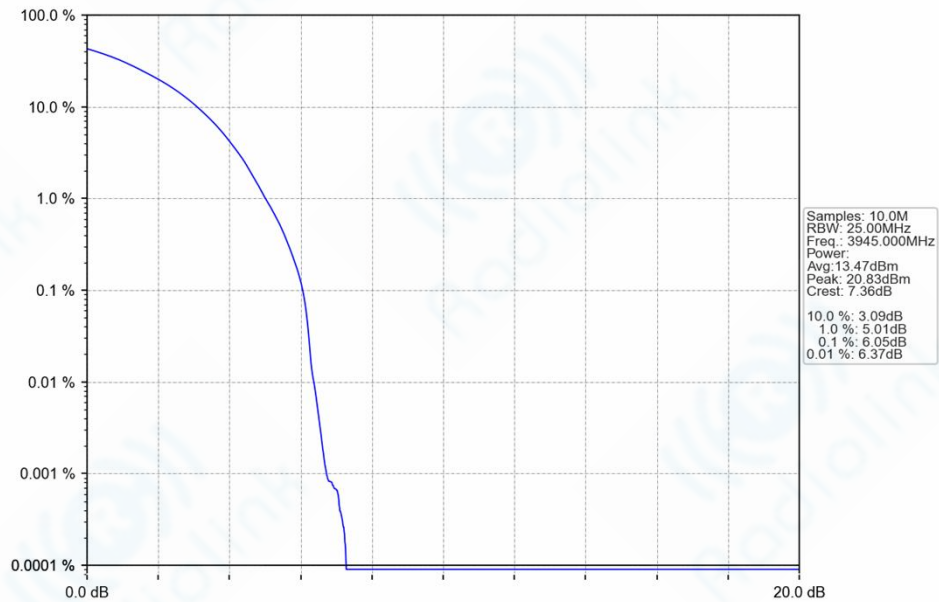
n77a_30kHz_SISO_NTNV_70MHz_DFT-s-OFDM PI/2 BPSK_3945MHz_Outer_Full_Ant1
