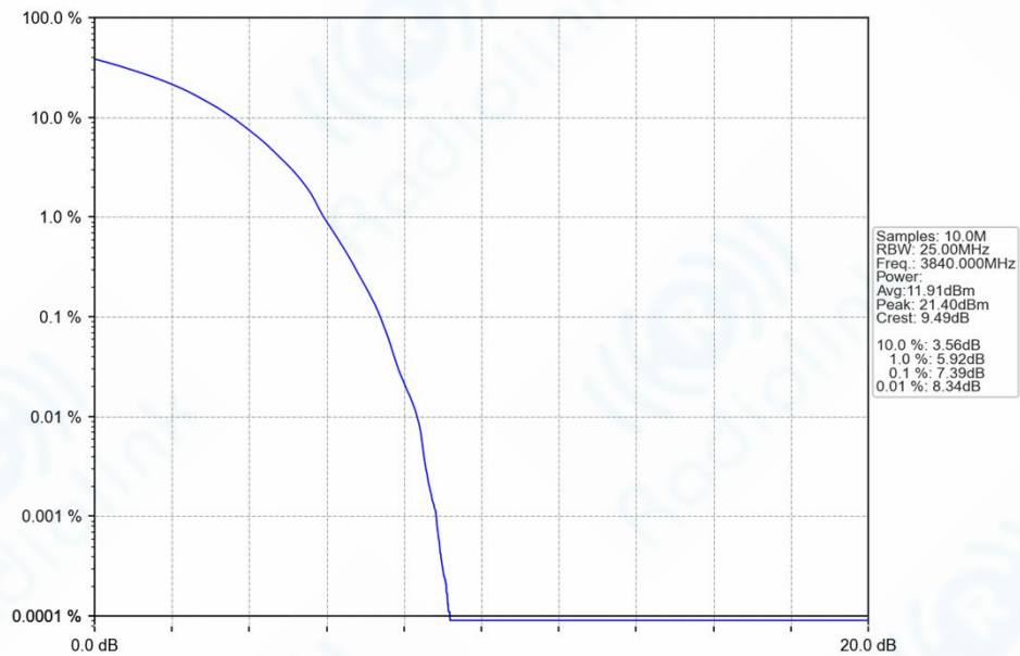
n77a_30kHz_SISO_NTNV_80MHz_DFT-s-OFDM_16_QAM_3840MHz_Outer_Full_Ant1
