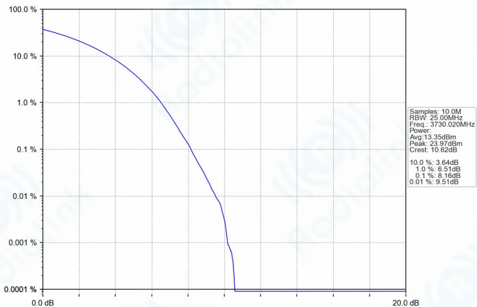
n77a_30kHz_SISO_NTNV_60MHz_CP-OFDM_64_QAM_3730.02MHz_Outer_Full_Ant1
