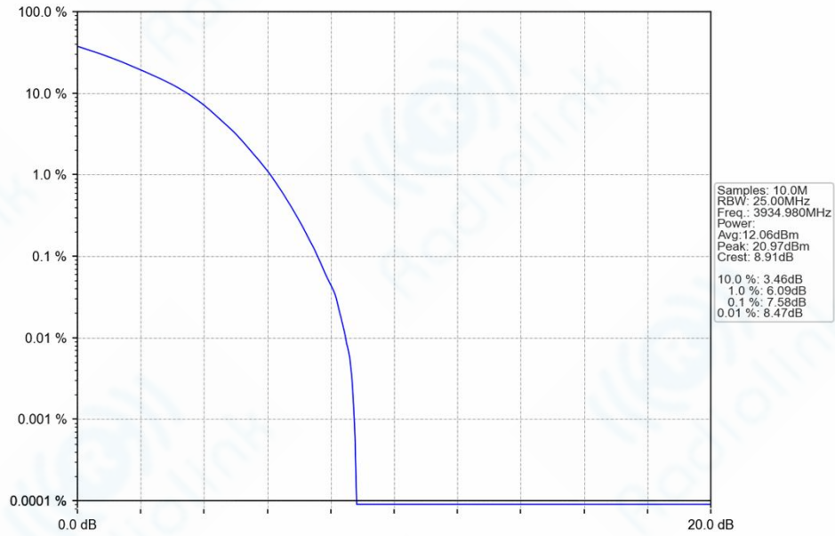
n77a_30kHz_SISO_NTNV_90MHz_DFT-s-OFDM_16_QAM_3934.98MHz_Outer_Full_Ant1
