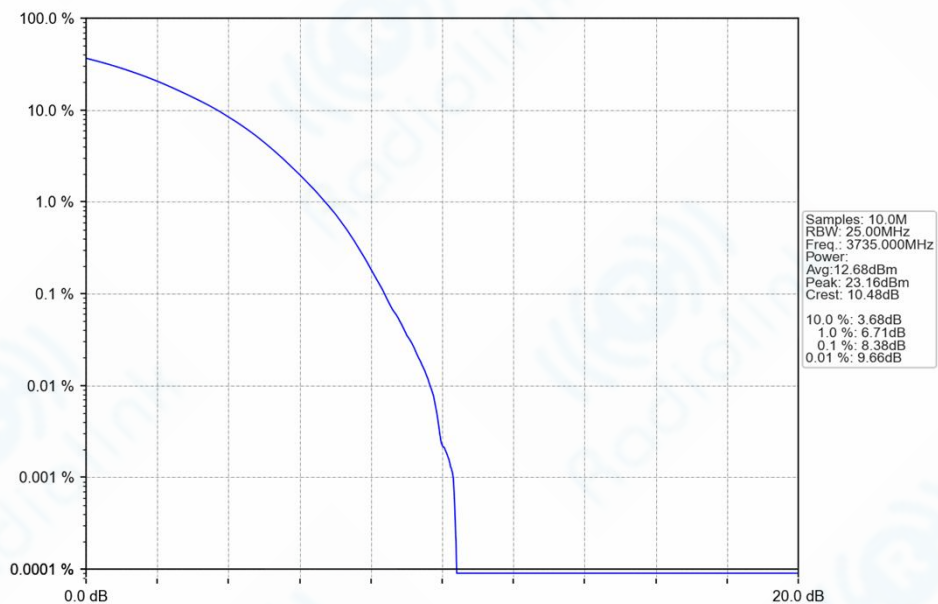
n77a_30kHz_SISO_NTNV_70MHz_CP-OFDM 64 QAM 3735MHz_Outer_Full_Ant1
