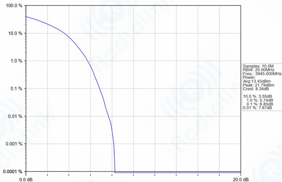
n77a_30kHz_SISO_NTNV_70MHz_DFT-s-OFDM_QPSK_3945MHz_Outer_Full_Ant1
