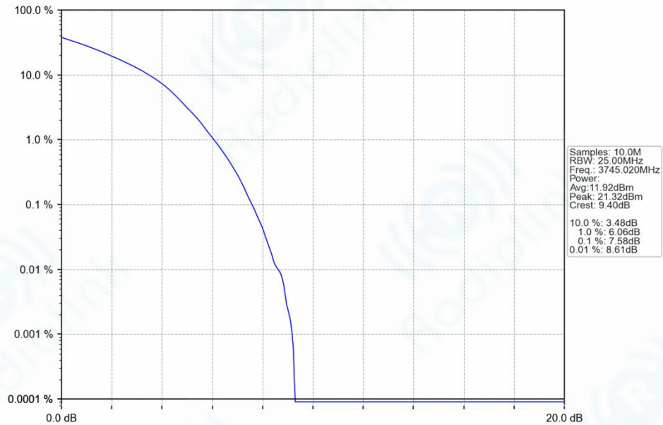
n77a_30kHz_SISO_NTNV_90MHz_DFT-s-OFDM_64_QAM_3745.02MHz_Outer_Full_Ant1
