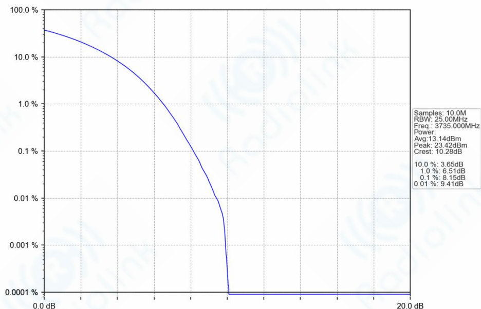
n77a_30kHz_SISO_NTNV_70MHz_CP-OFDM_16_QAM_3735MHz_Outer_Full_Ant1
