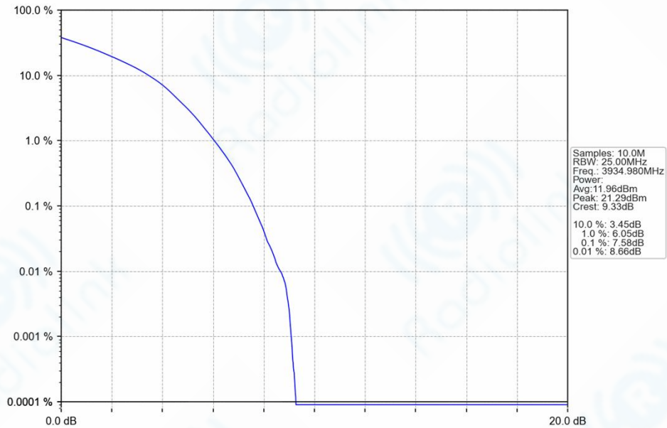
n77a_30kHz_SISO_NTNV_90MHz_DFT-s-OFDM_64_QAM_3934.98MHz_Outer_Full_Ant1
