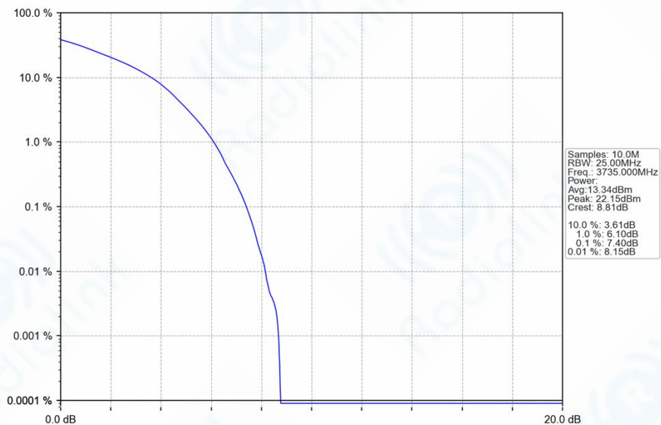
n77a_30kHz_SISO_NTNV_70MHz_DFT-s-OFDM_64_QAM_3735MHz_Outer_Full_Ant1
