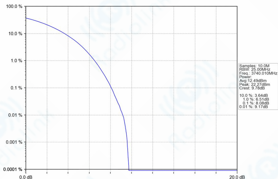
n77a_30kHz_SISO_NTNV_80MHz_CP-OFDM_QPSK_3740.01MHz_Outer_Full_Ant1
