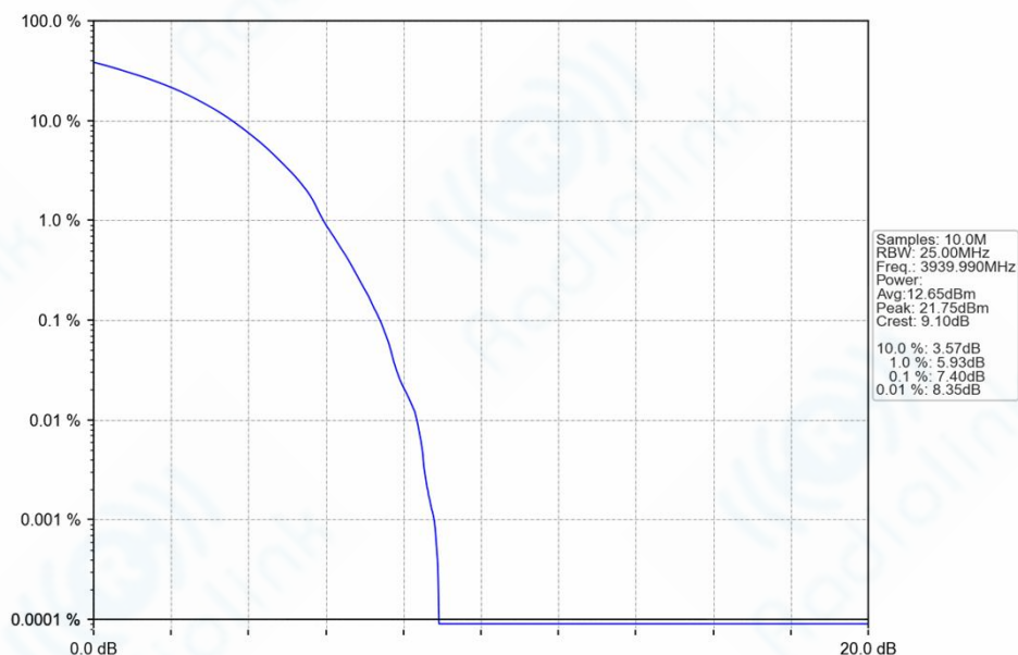
n77a_30kHz_SISO_NTNV_80MHz_DFT-s-OFDM_16_QAM_3939.99MHz_Outer_Full_Ant1
