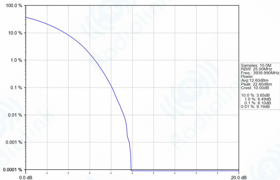
n77a_30kHz_SISO_NTNV_80MHz_CP-OFDM_QPSK_3939.99MHz_Outer_Full_Ant1
