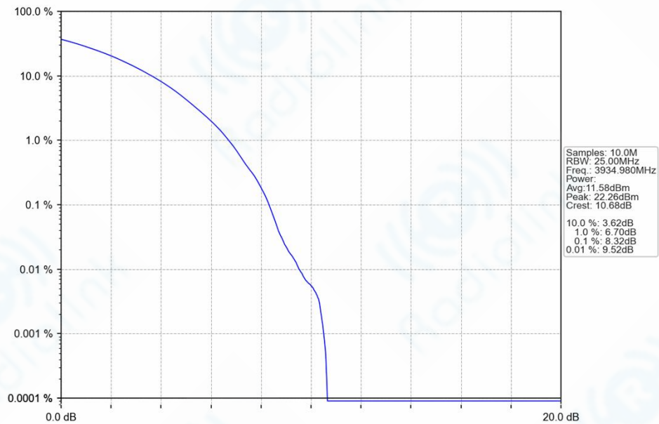
n77a_30kHz_SISO_NTNV_90MHz_CP-OFDM_64_QAM_3934.98MHz_Outer_Full_Ant1
