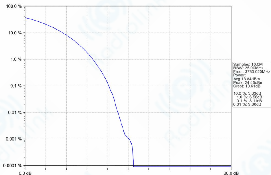
n77a_30kHz_SISO_NTNV_60MHz_CP-OFDM_QPSK_3730.02MHz_Outer_Full_Ant1
