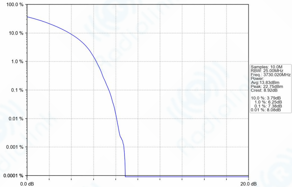
n77a_30kHz_SISO_NTNV_60MHz_DFT-s-OFDM_64_QAM_3730.02MHz_Outer_Full_Ant1
