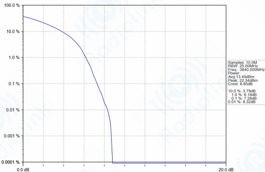
n77a_30kHz_SISO_NTNV_60MHz_DFT-s-OFDM_16_QAM_3840MHz_Outer_Full_Ant1
