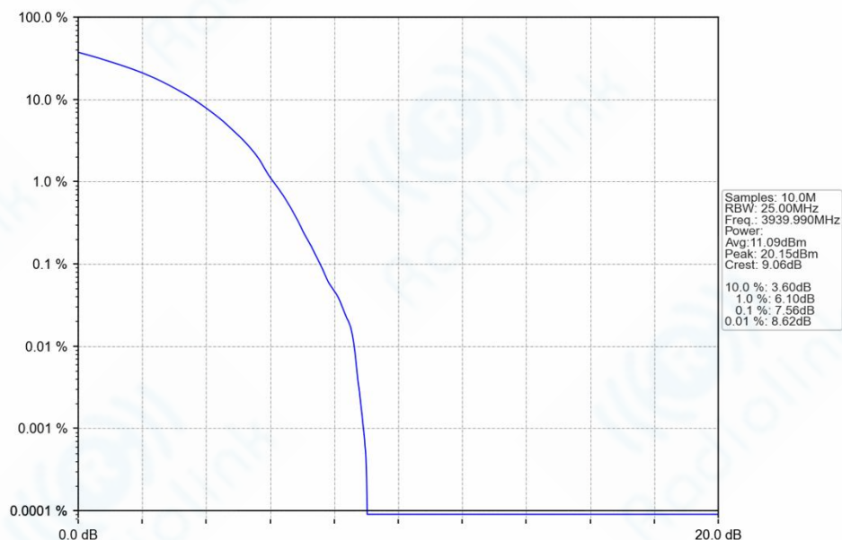
n77a_30kHz_SISO_NTNV_80MHz_DFT-s-OFDM_256_QAM_3939.99MHz_Outer_Full_Ant1
