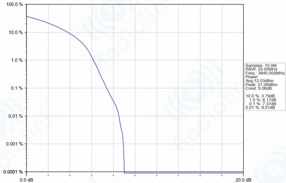
n77a_30kHz_SISO_NTNV_60MHz_DFT-s-OFDM_256_QAM_3840MHz_Outer_Full_Ant1
