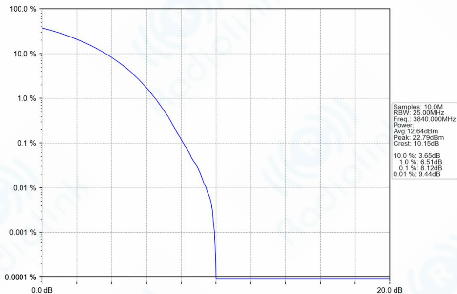
n77a_30kHz_SISO_NTNV_70MHz_CP-OFDM_16_QAM_3840MHz_Outer_Full_Ant1
