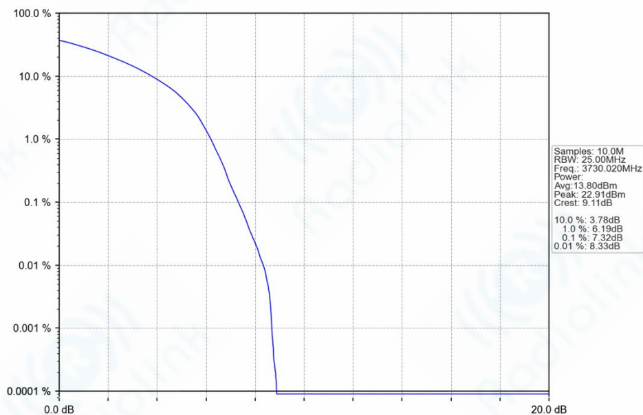
n77a_30kHz_SISO_NTNV_60MHz_DFT-s-OFDM_16_QAM_3730.02MHz_Outer_Full_Ant1
