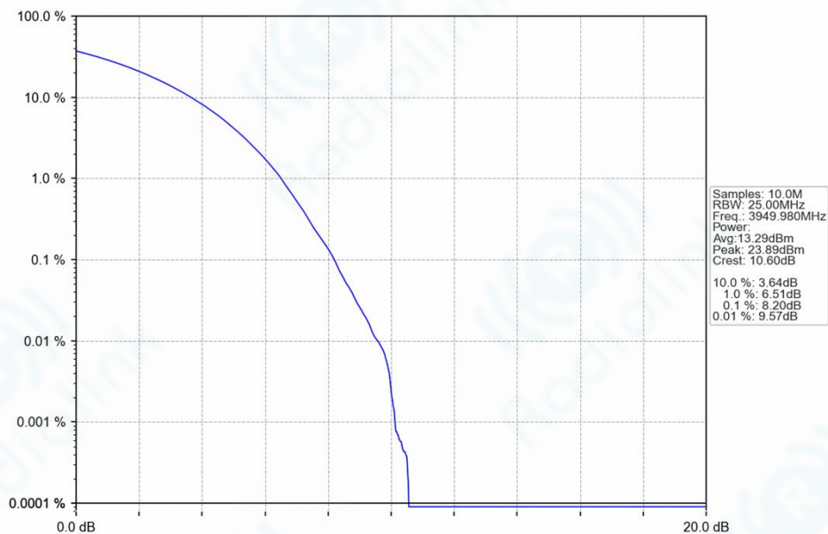
n77a_30kHz_SISO_NTNV_60MHz_CP-OFDM_64_QAM_3949.98MHz_Outer_Full_Ant1
