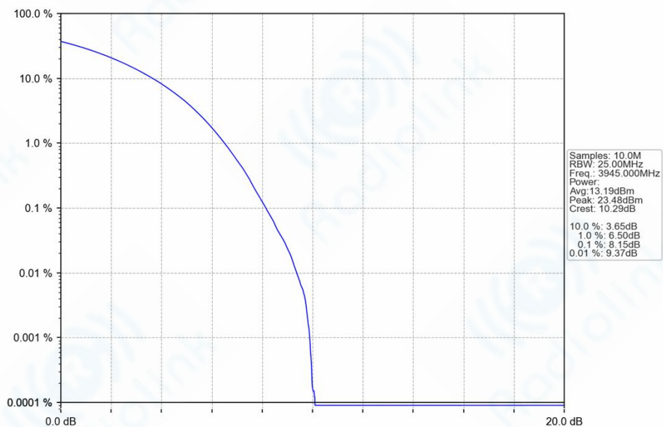
n77a_30kHz_SISO_NTNV_70MHz_CP-OFDM 16 QAM 3945MHz_Outer_Full_Ant1
