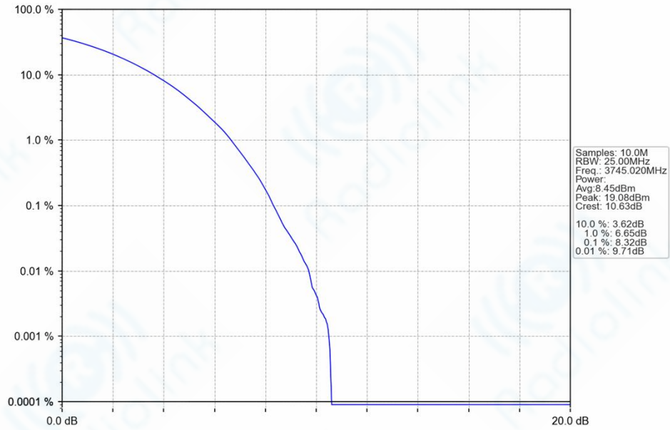
n77a_30kHz_SISO_NTNV_90MHz_CP-OFDM_256_QAM_3745.02MHz_Outer_Full_Ant1
