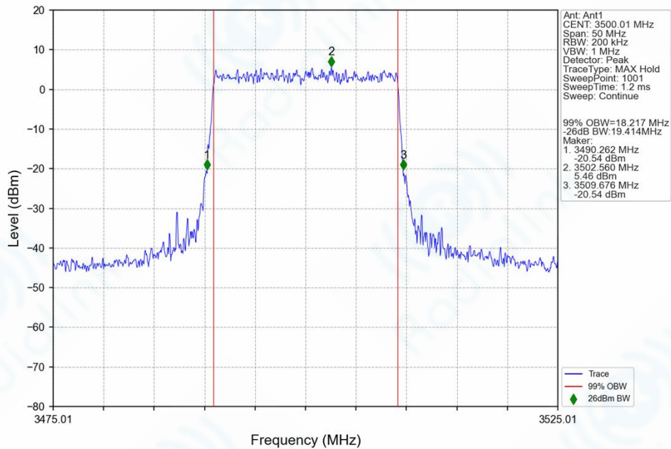
n77d_30kHz_SISO_NTNV_20MHz_CP-OFDM_256_QAM_3500.01MHz_Outer_Full_Ant1
