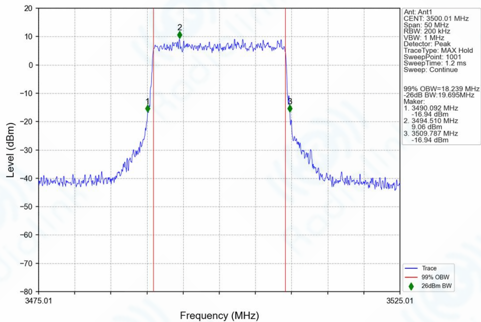
n77d_30kHz_SISO_NTNV_20MHz_CP-OFDM_16_QAM_3500.01MHz_Outer_Full_Ant1
