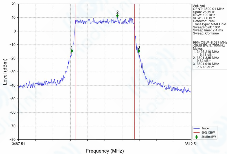
n77d_30kHz_SISO_NTNV_10MHz_DFT-s-OFDM_16_QAM_3500.01MHz_Outer_Full_Ant1
