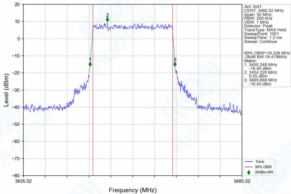
n77d_30kHz_SISO_NTNV_20MHz_CP-OFDM_64 QAM_3460.02MHz_Outer_Full_Ant1
