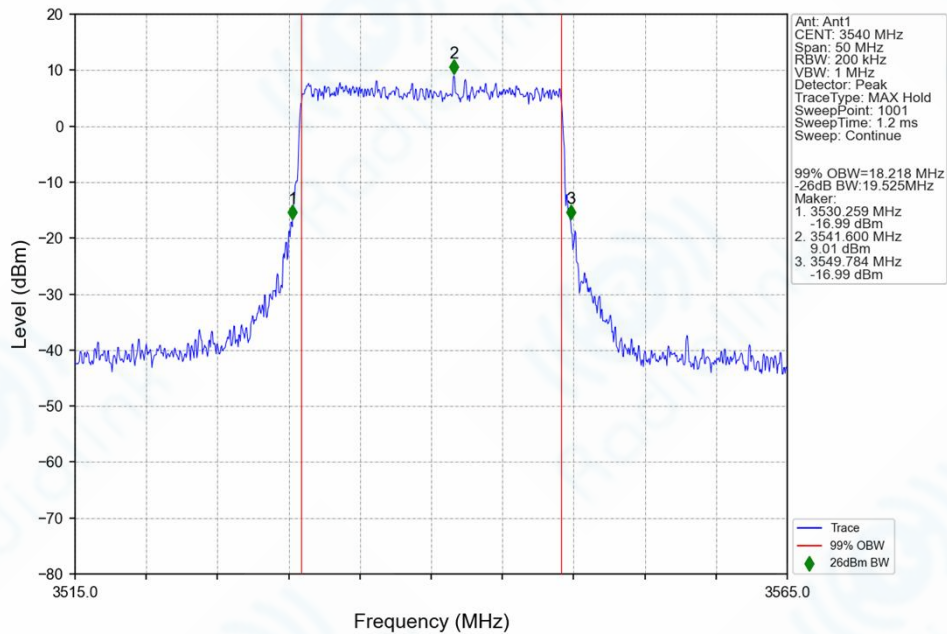
n77d_30kHz_SISO_NTNV_20MHz_CP-OFDM_QPSK_3540MHz_Outer_Full_Ant1
