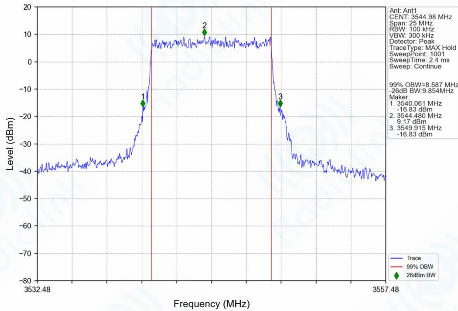
n77d_30kHz_SISO_NTNV_10MHz_DFT-s-OFDM_64_QAM_3544.98MHz_Outer_Full_Ant1
