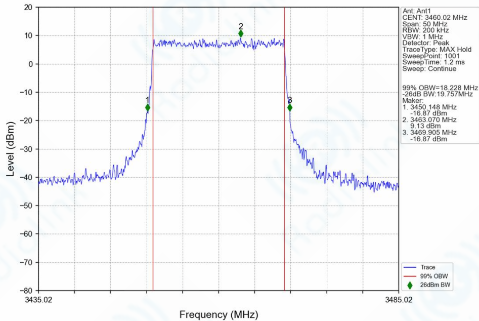
n77d_30kHz_SISO_NTNV_20MHz_CP-OFDM_QPSK_3460.02MHz_Outer_Full_Ant1
