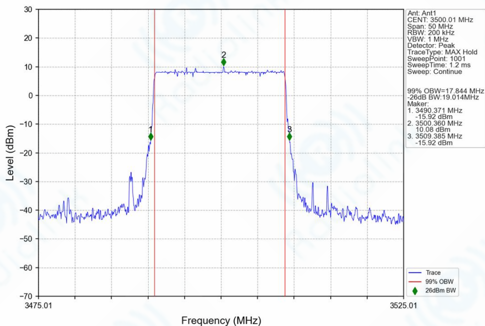
n77d_30kHz_SISO_NTNV_20MHz_DFT-s-OFDM_16_QAM_3500.01MHz_Outer_Full_Ant1
