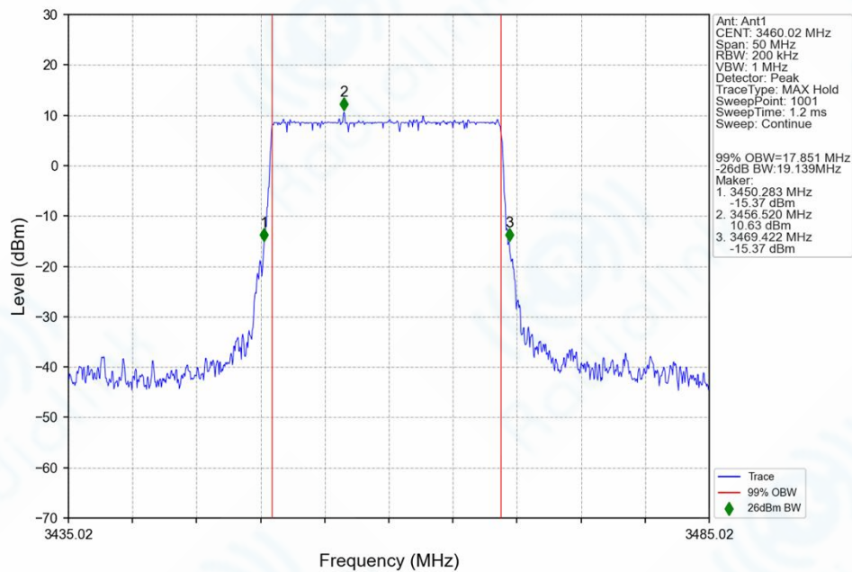
n77d_30kHz_SISO_NTNV_20MHz_DFT-s-OFDM_64_QAM_3460.02MHz_Outer_Full_Ant1
