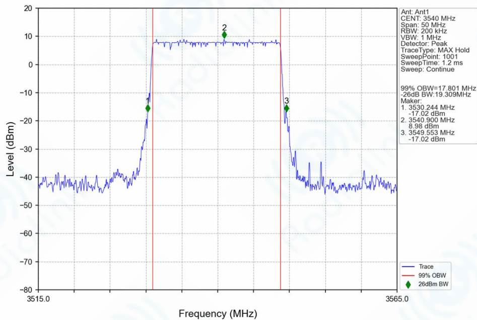
n77d_30kHz_SISO_NTNV_20MHz_DFT-s-OFDM_QPSK_3540MHz_Outer_Full_Ant1
