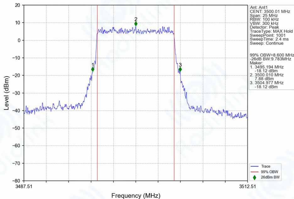
n77d_30kHz_SISO_NTNV_10MHz_DFT-s-OFDM_256_QAM_3500.01MHz_Outer_Full_Ant1
