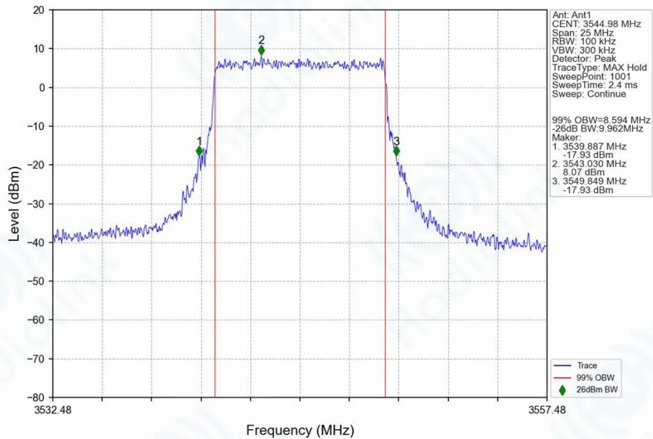
n77d_30kHz_SISO_NTNV_10MHz_CP-OFDM_QPSK_3544.98MHz_Outer_Full_Ant1
