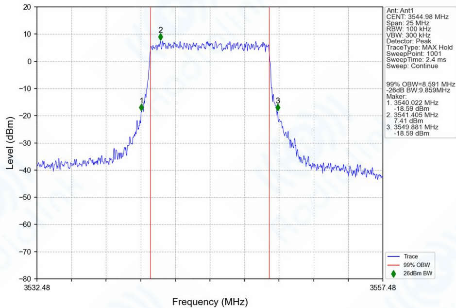
n77d_30kHz_SISO_NTNV_10MHz_CP-OFDM_64_QAM_3544.98MHz_Outer_Full_Ant1
