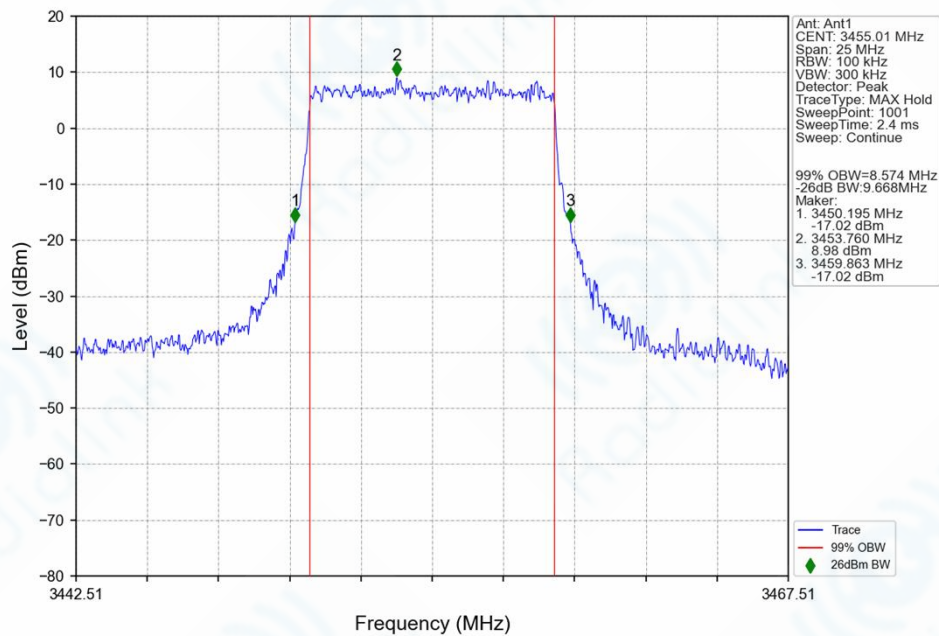
n77d_30kHz_SISO_NTNV_10MHz_CP-OFDM_QPSK_3455.01MHz_Outer_Full_Ant1
