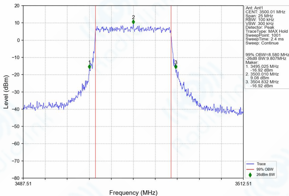
n77d_30kHz_SISO_NTNV_10MHz_CP-OFDM_16_QAM_3500.01MHz_Outer_Full_Ant1
