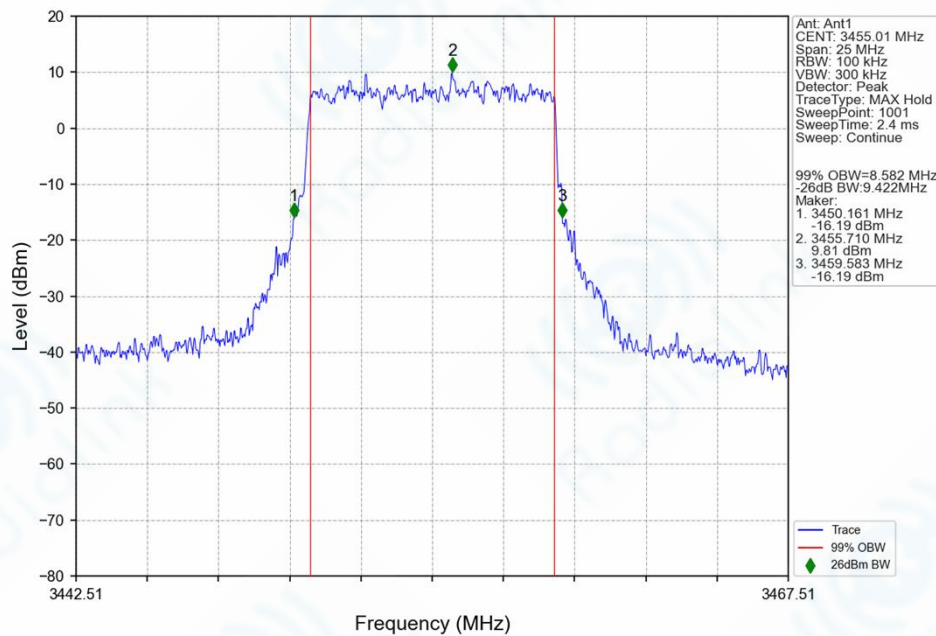
n77d_30kHz_SISO_NTNV_10MHz_CP-OFDM_64 QAM_3455.01MHz_Outer_Full_Ant1
