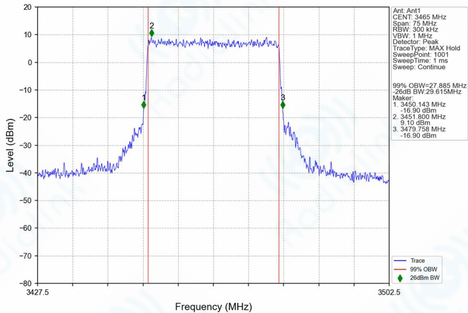
n77d_30kHz_SISO_NTNV_30MHz_CP-OFDM_QPSK_3465MHz_Outer_Full_Ant1
