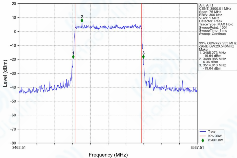
n77d_30kHz_SISO_NTNV_30MHz_CP-OFDM_256_QAM_3500.01MHz_Outer_Full_Ant1
