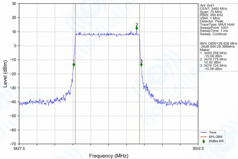
n77d_30kHz_SISO_NTNV_30MHz_DFT-s-OFDM_64_QAM_3465MHz_Outer_Full_Ant1
