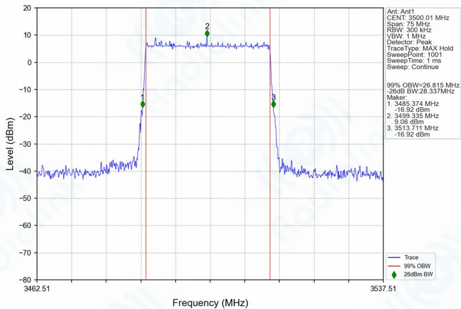
n77d_30kHz_SISO_NTNV_30MHz_DFT-s-OFDM_256_QAM_3500.01MHz_Outer_Full_Ant1
