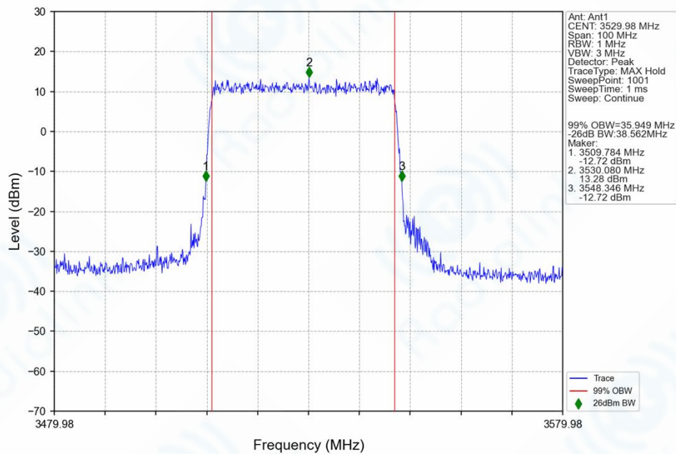
n77d_30kHz_SISO_NTNV_40MHz_DFT-s-OFDM_64_QAM_3529.98MHz_Outer_Full_Ant1
