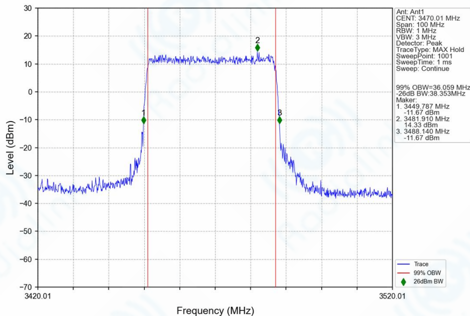
n77d_30kHz_SISO_NTNV_40MHz_DFT-s-OFDM_64_QAM_3470.01MHz_Outer_Full_Ant1
