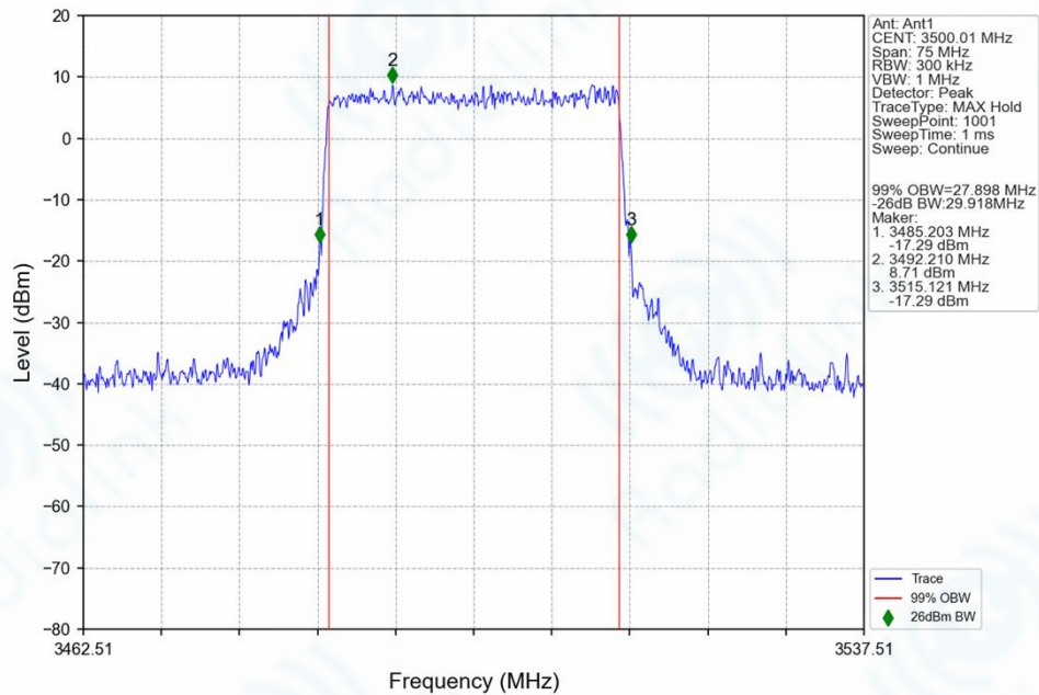
n77d_30kHz_SISO_NTNV_30MHz_CP-OFDM_16_QAM_3500.01MHz_Outer_Full_Ant1
