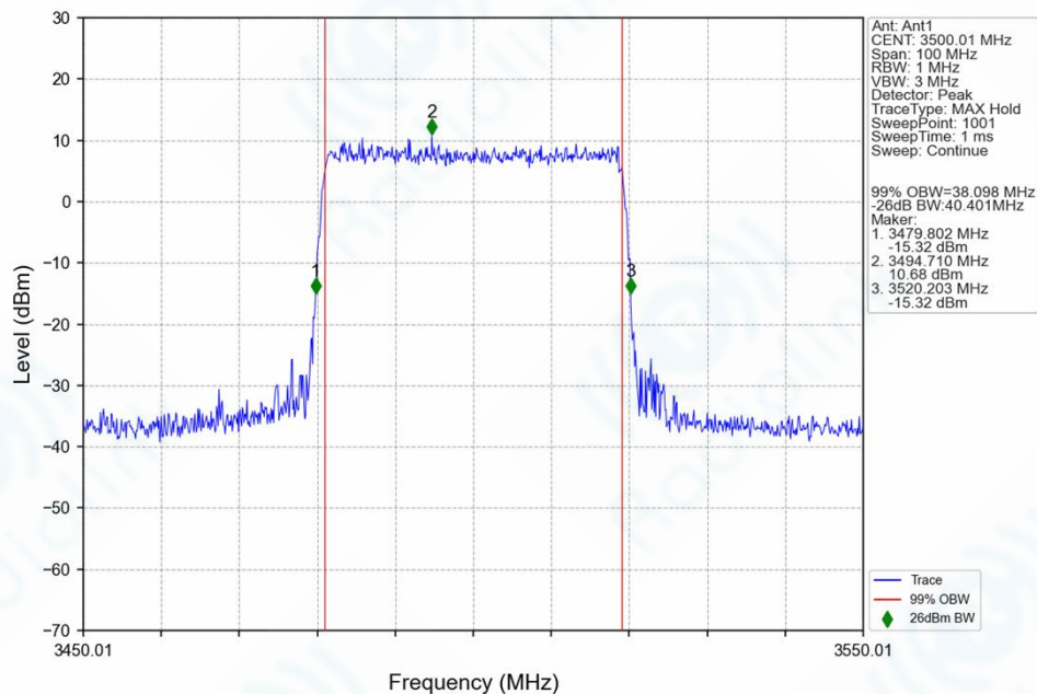
n77d_30kHz_SISO_NTNV_40MHz_CP-OFDM_256_QAM_3500.01MHz_Outer_Full_Ant1
