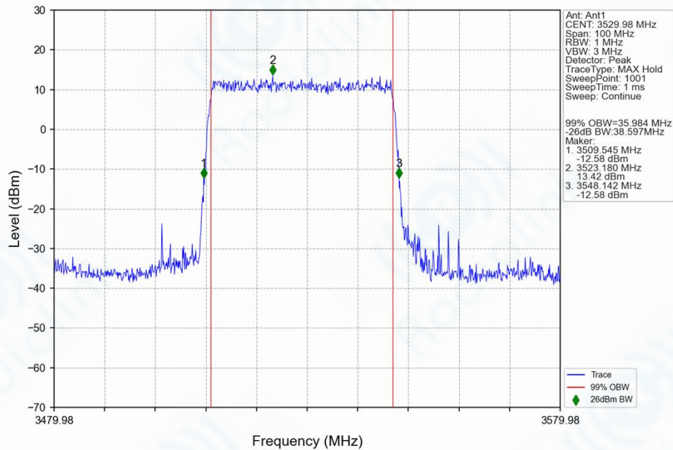
n77d_30kHz_SISO_NTNV_40MHz_DFT-s-OFDM_QPSK_3529.98MHz_Outer_Full_Ant1
