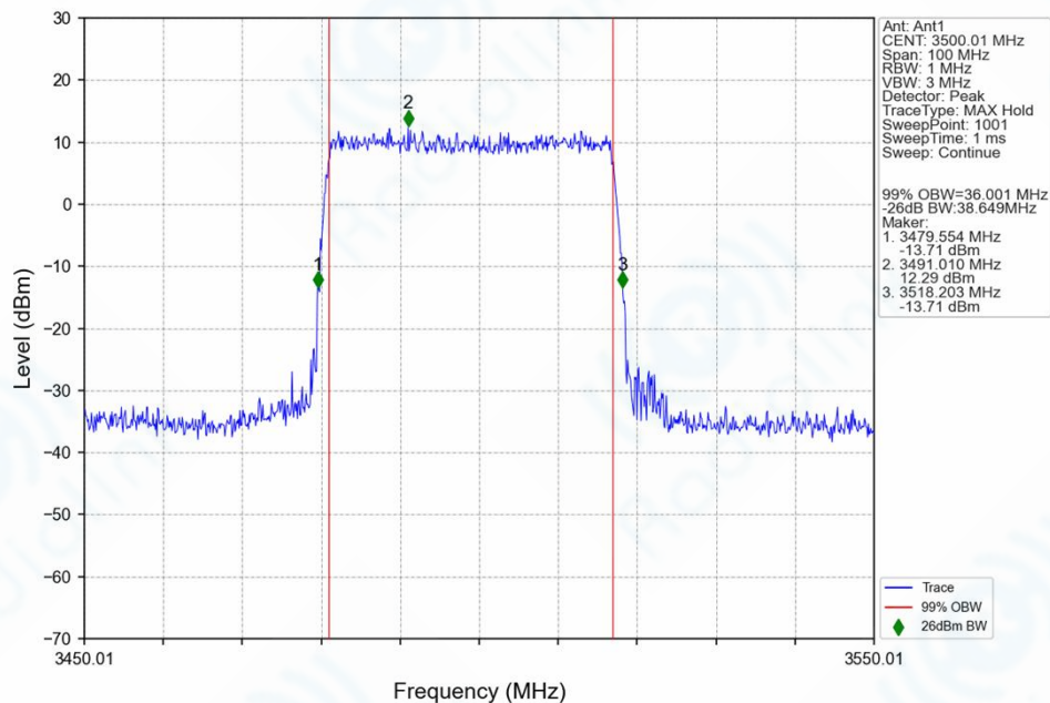
n77d_30kHz_SISO_NTNV_40MHz_DFT-s-OFDM_256_QAM_3500.01MHz_Outer_Full_Ant1
