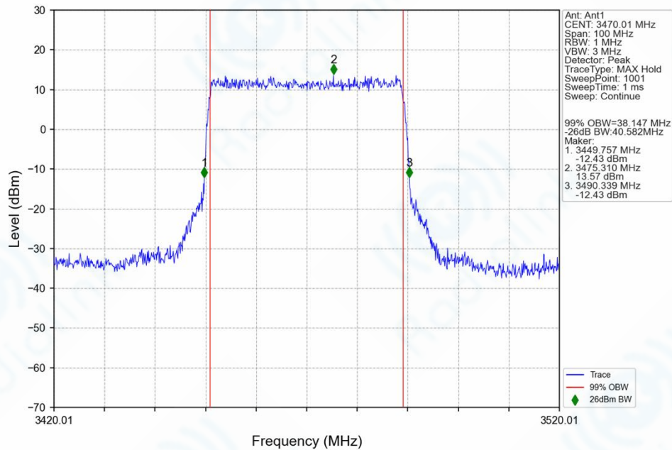
n77d_30kHz_SISO_NTNV_40MHz_CP-OFDM_QPSK_3470.01MHz_Outer_Full_Ant1
