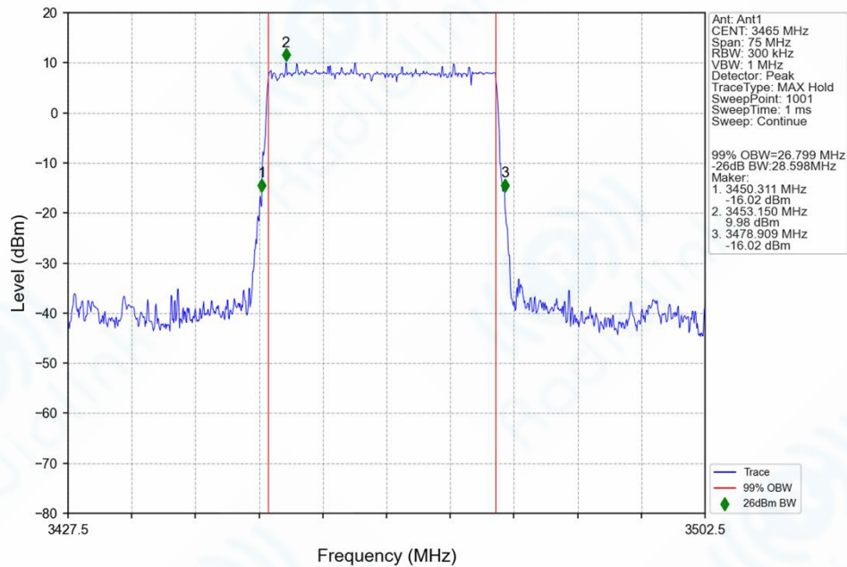
n77d_30kHz_SISO_NTNV_30MHz_DFT-s-OFDM QPSK_3465MHz_Outer_Full_Ant1
