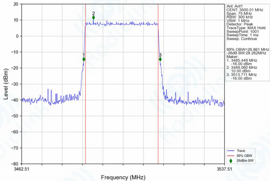
n77d_30kHz_SISO_NTNV_30MHz_DFT-s-OFDM_16_QAM_3500.01MHz_Outer_Full_Ant1
