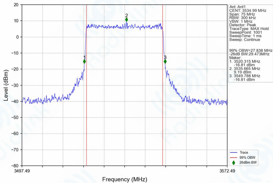
n77d_30kHz_SISO_NTNV_30MHz_CP-OFDM_QPSK_3534.99MHz_Outer_Full_Ant1
