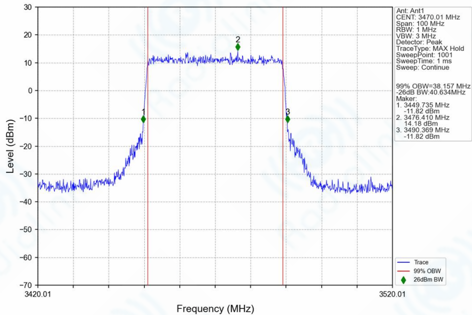
n77d_30kHz_SISO_NTNV_40MHz_CP-OFDM_64 QAM_3470.01MHz_Outer_Full_Ant1
