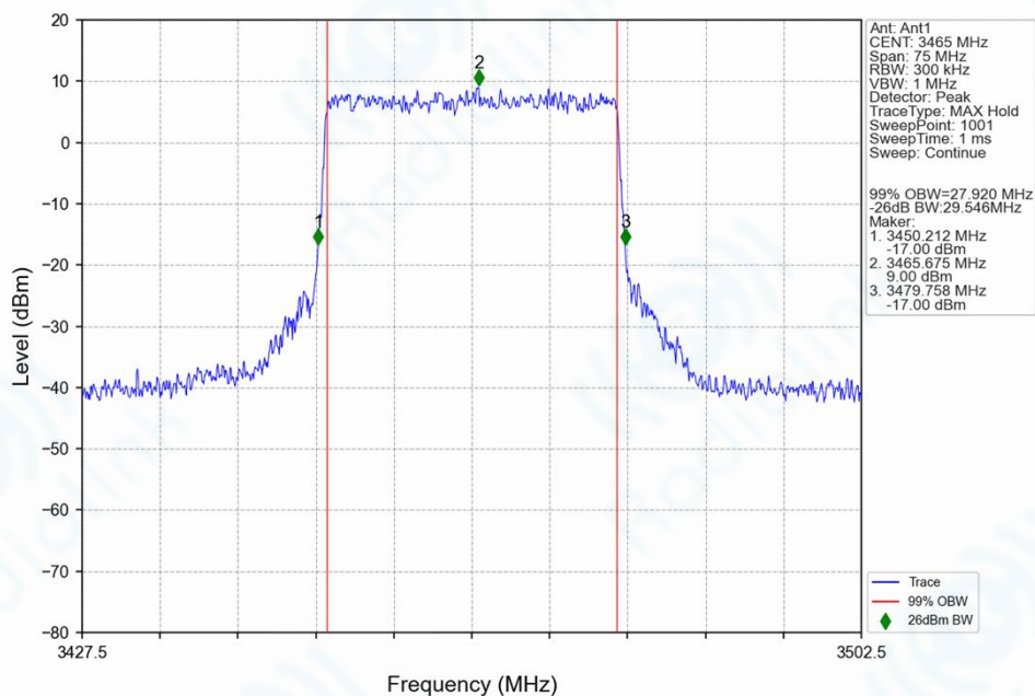
n77d_30kHz_SISO_NTNV_30MHz_CP-OFDM_64 QAM_3465MHz_Outer_Full_Ant1
