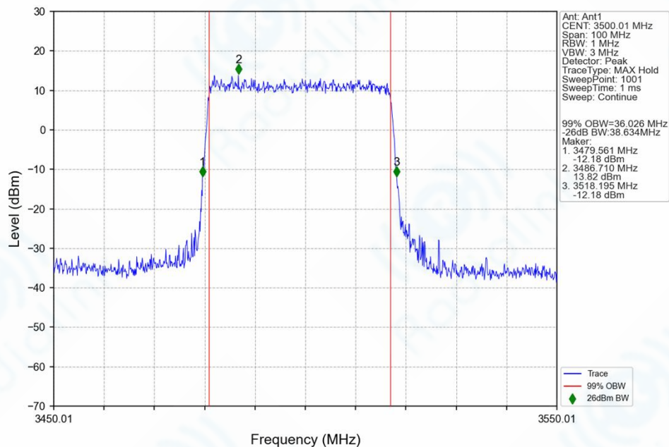
n77d_30kHz_SISO_NTNV_40MHz_DFT-s-OFDM_16_QAM_3500.01MHz_Outer_Full_Ant1
