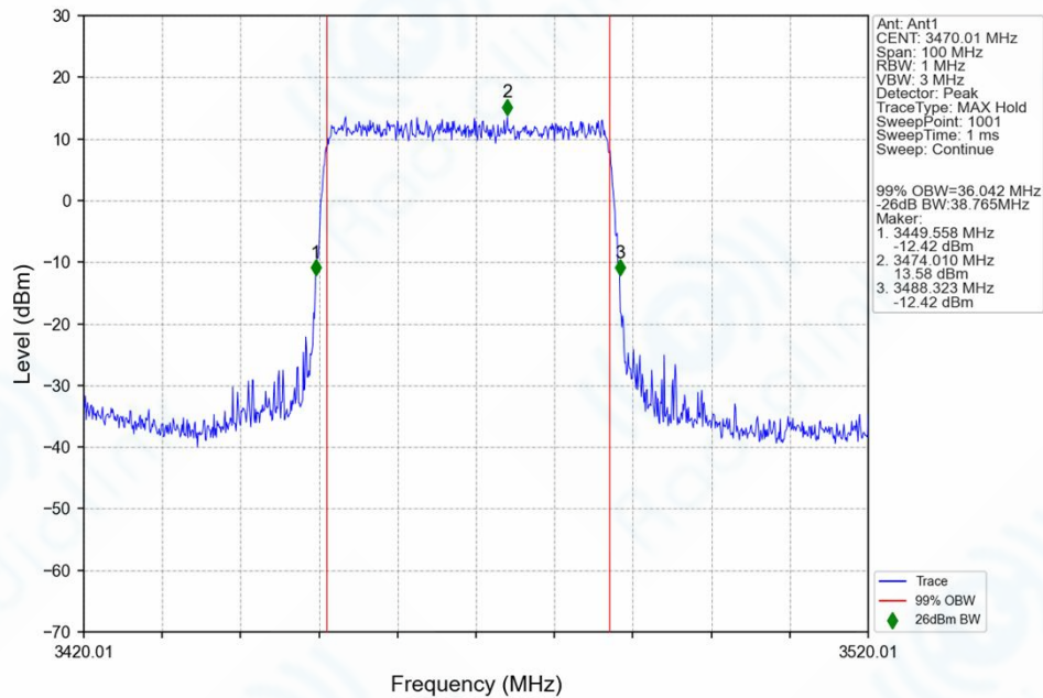
n77d_30kHz_SISO_NTNV_40MHz_DFT-s-OFDM_QPSK_3470.01MHz_Outer_Full_Ant1
