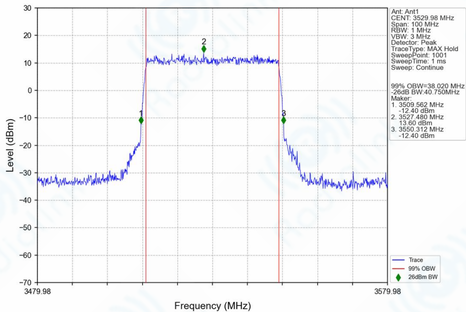
n77d_30kHz_SISO_NTNV_40MHz_CP-OFDM_QPSK_3529.98MHz_Outer_Full_Ant1
