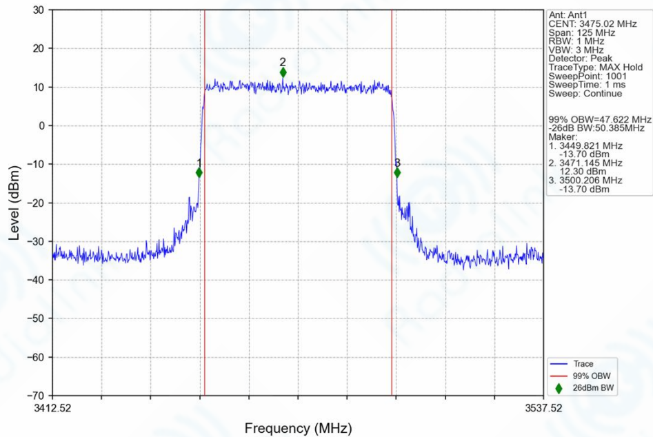
n77d_30kHz_SISO_NTNV_50MHz_CP-OFDM 64 QAM 3475.02MHz_Outer_Full_Ant1
