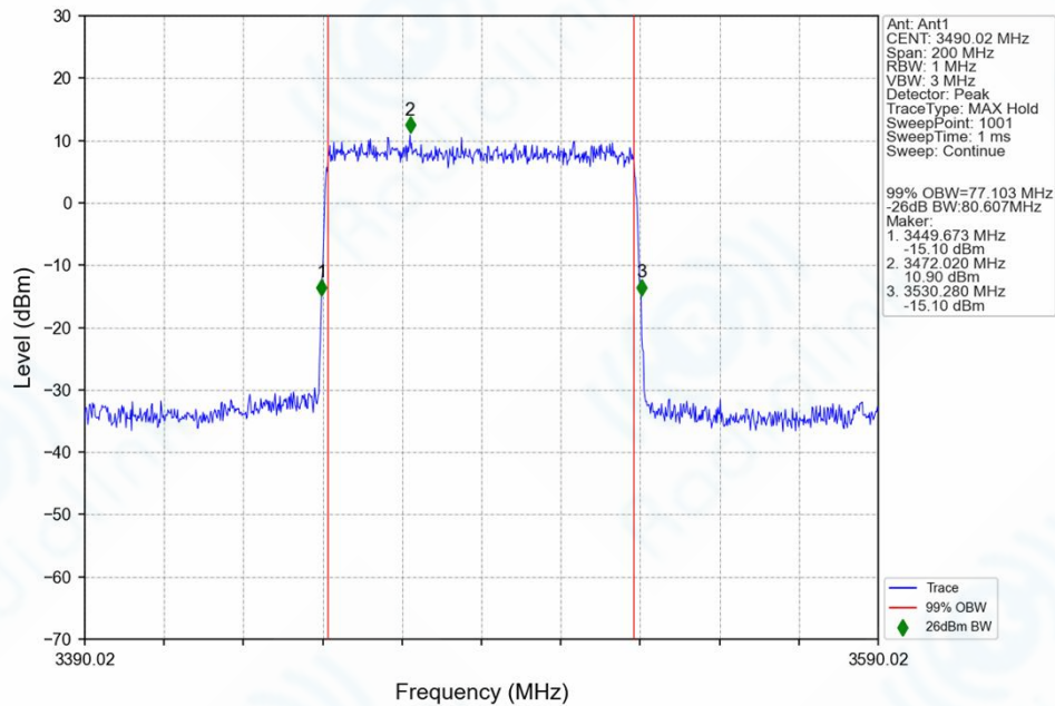
n77d_30kHz_SISO_NTNV_80MHz_DFT-s-OFDM_64_QAM_3490.02MHz_Outer_Full_Ant1
