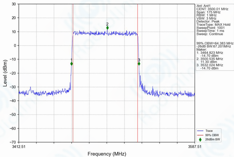
n77d_30kHz_SISO_NTNV_70MHz_DFT-s-OFDM_16_QAM_3500.01MHz_Outer_Full_Ant1
