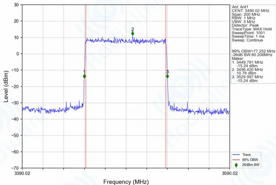
n77d_30kHz_SISO_NTNV_80MHz_DFT-s-OFDM QPSK_3490.02MHz_Outer_Full_Ant1
