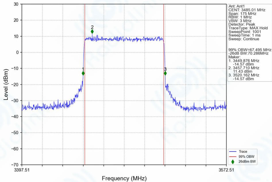
n77d_30kHz_SISO_NTNV_70MHz_CP-OFDM_64_QAM_3485.01MHz_Outer_Full_Ant1
