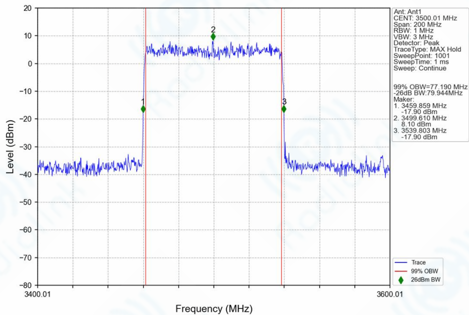
n77d_30kHz_SISO_NTNV_80MHz_DFT-s-OFDM_256_QAM_3500.01MHz_Outer_Full_Ant1
