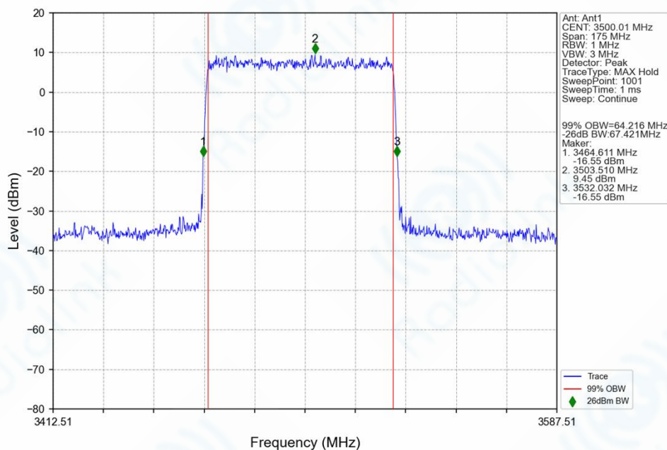
n77d_30kHz_SISO_NTNV_70MHz_DFT-s-OFDM_256_QAM_3500.01MHz_Outer_Full_Ant1
