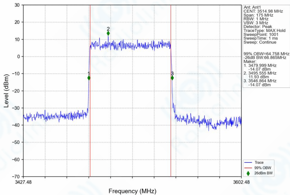
n77d_30kHz_SISO_NTNV_70MHz_DFT-s-OFDM_64_QAM_3514.98MHz_Outer_Full_Ant1
