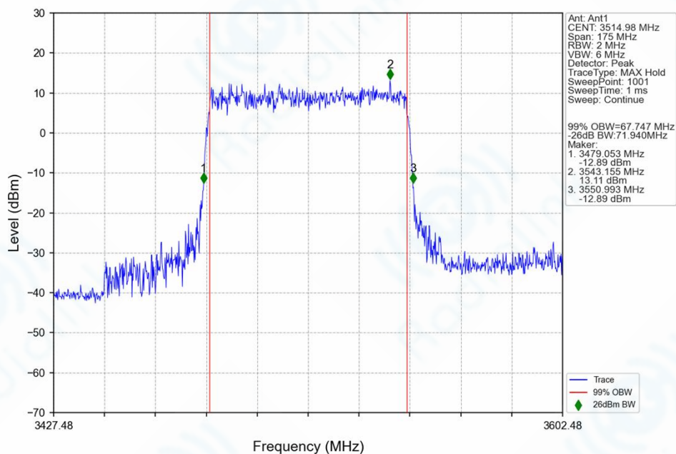
n77d_30kHz_SISO_NTNV_70MHz_CP-OFDM_64_QAM_3514.98MHz_Outer_Full_Ant1
