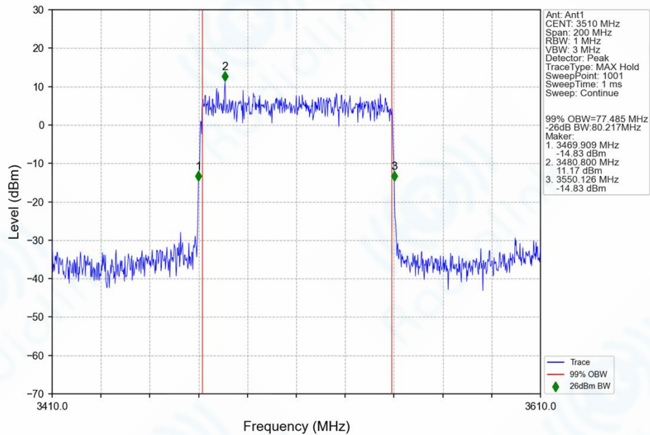
n77d_30kHz_SISO_NTNV_80MHz_CP-OFDM_QPSK_3510MHz_Outer_Full_Ant1
