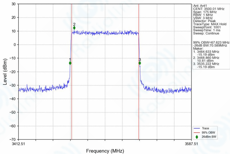
n77d_30kHz_SISO_NTNV_70MHz_CP-OFDM_16_QAM_3500.01MHz_Outer_Full_Ant1
