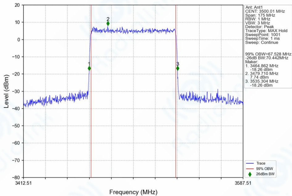
n77d_30kHz_SISO_NTNV_70MHz_CP-OFDM_256_QAM_3500.01MHz_Outer_Full_Ant1
