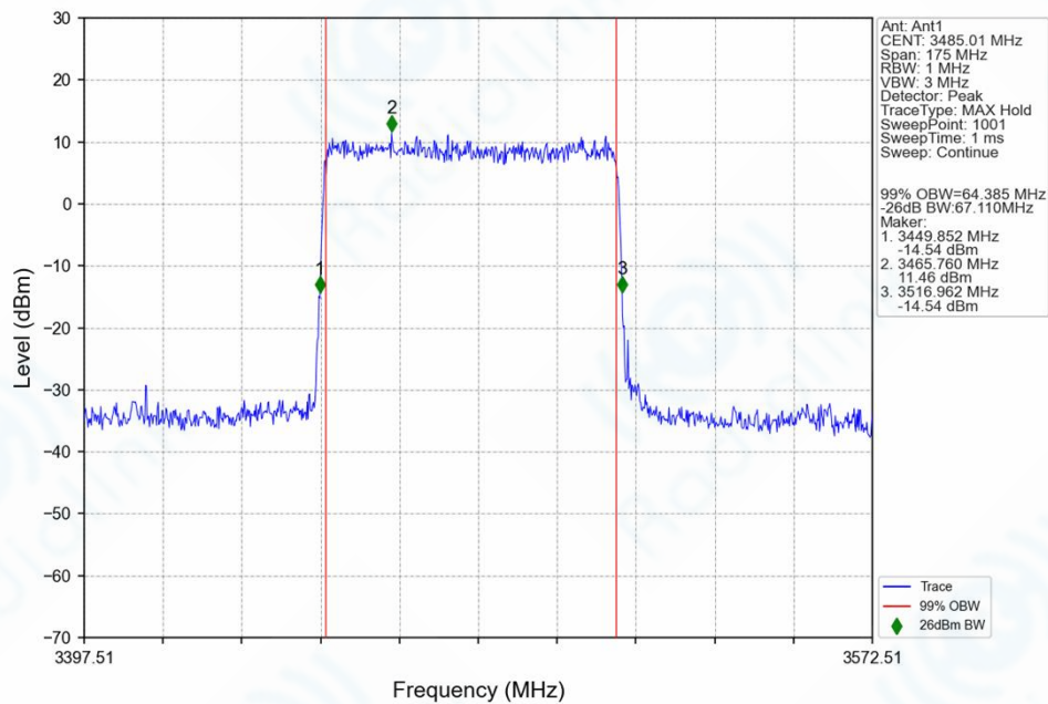
n77d_30kHz_SISO_NTNV_70MHz_DFT-s-OFDM_64_QAM_3485.01MHz_Outer_Full_Ant1
