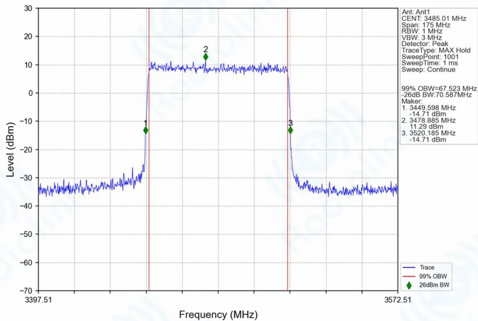
n77d_30kHz_SISO_NTNV_70MHz_CP-OFDM_QPSK_3485.01MHz_Outer_Full_Ant1
