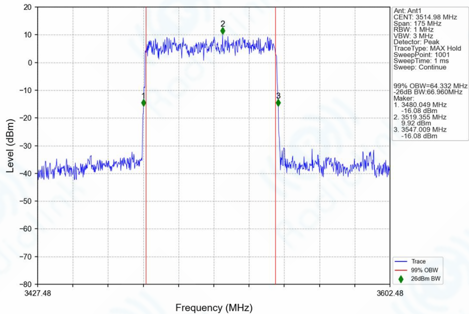
n77d_30kHz_SISO_NTNV_70MHz_DFT-s-OFDM_QPSK_3514.98MHz_Outer_Full_Ant1
