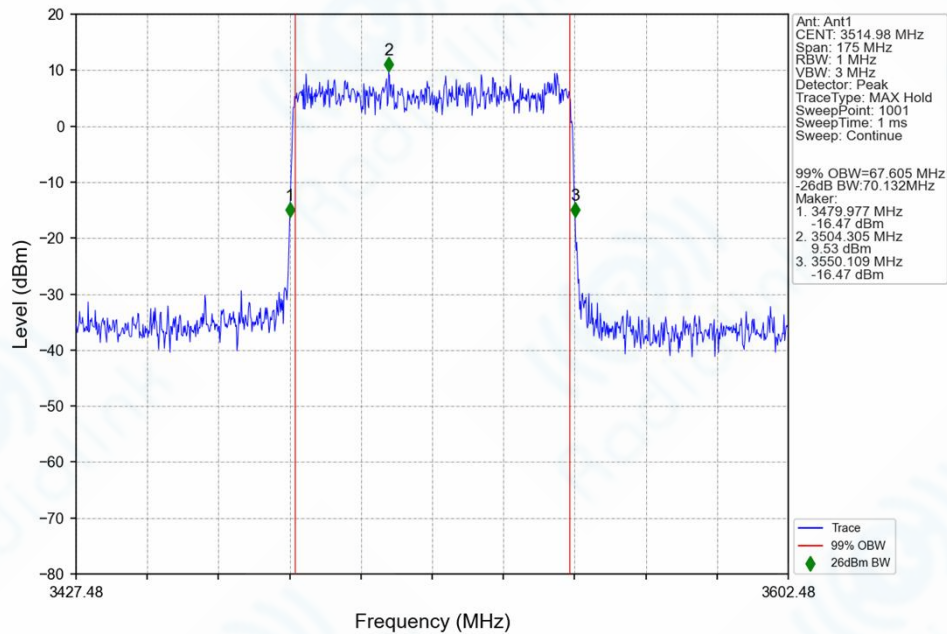
n77d_30kHz_SISO_NTNV_70MHz_CP-OFDM_QPSK_3514.98MHz_Outer_Full_Ant1
