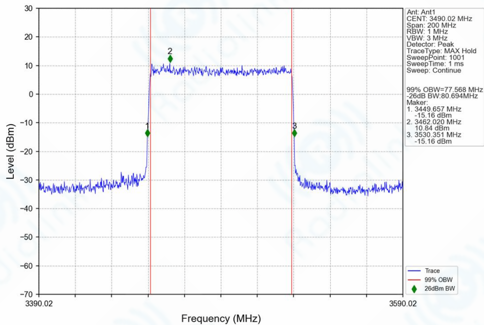
n77d_30kHz_SISO_NTNV_80MHz_CP-OFDM_QPSK_3490.02MHz_Outer_Full_Ant1
