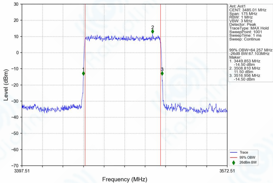
n77d_30kHz_SISO_NTNV_70MHz_DFT-s-OFDM QPSK_3485.01MHz_Outer_Full_Ant1
