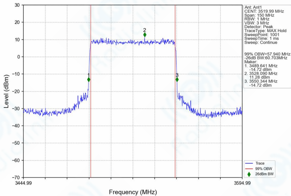
n77d_30kHz_SISO_NTNV_60MHz_CP-OFDM_64_QAM_3519.99MHz_Outer_Full_Ant1
