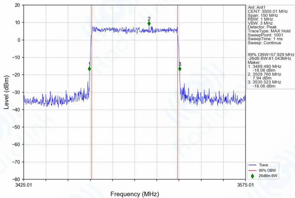
n77d_30kHz_SISO_NTNV_60MHz_CP-OFDM_256_QAM_3500.01MHz_Outer_Full_Ant1
