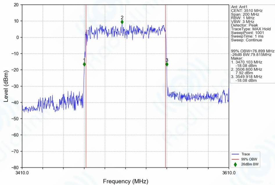
n77d_30kHz_SISO_NTNV_80MHz_DFT-s-OFDM_64_QAM_3510MHz_Outer_Full_Ant1
