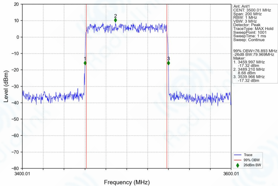
n77d_30kHz_SISO_NTNV_80MHz_DFT-s-OFDM_16_QAM_3500.01MHz_Outer_Full_Ant1
