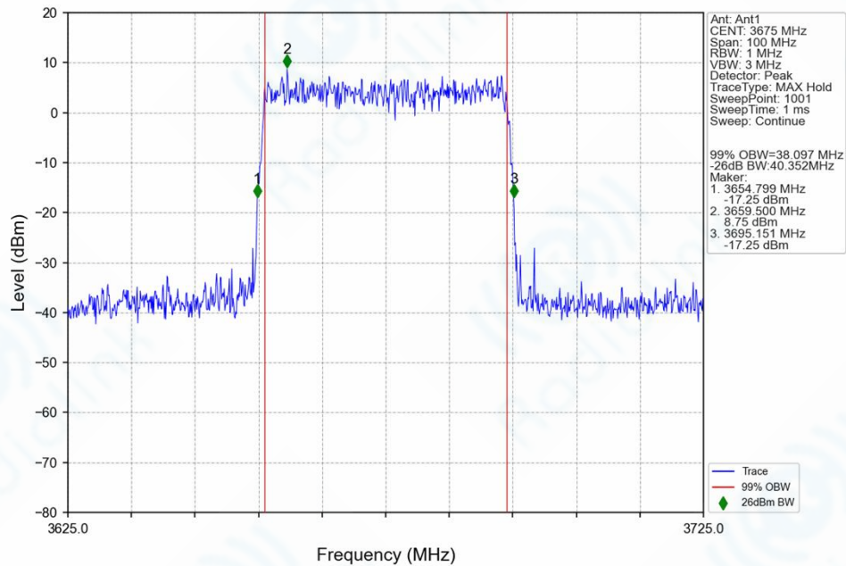
n77g_30kHz_SISO_NTNV_40MHz_CP-OFDM_256_QAM_3675MHz_Outer_Full_Ant1
