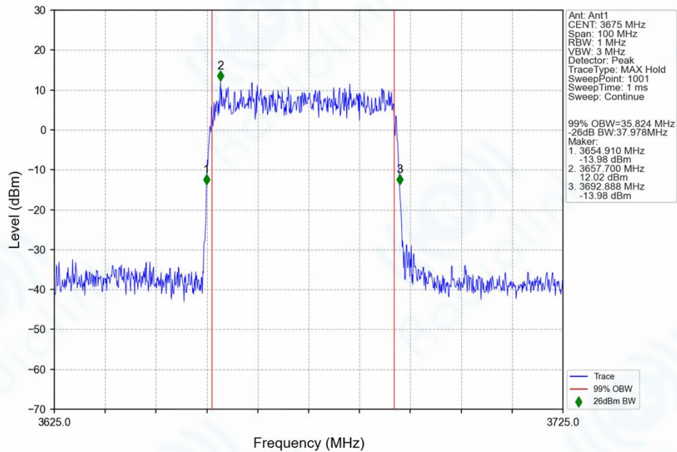
n77g_30kHz_SISO_NTNV_40MHz_DFT-s-OFDM_16_QAM_3675MHz_Outer_Full_Ant1
