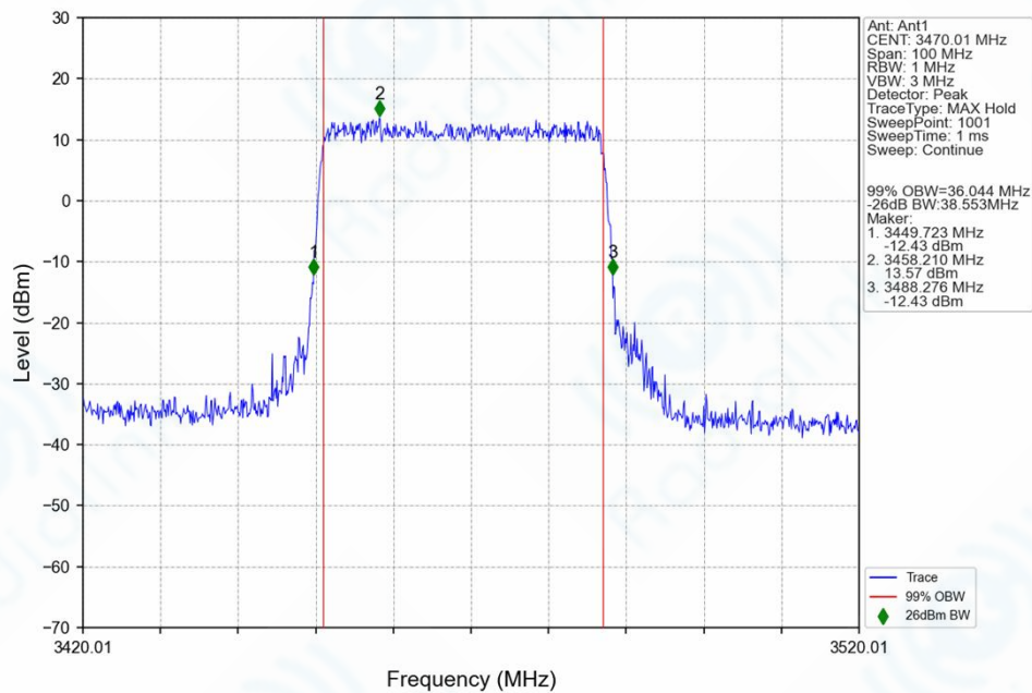
n77g_30kHz_SISO_NTNV_40MHz_DFT-s-OFDM_64_QAM_3470.01MHz_Outer_Full_Ant1
