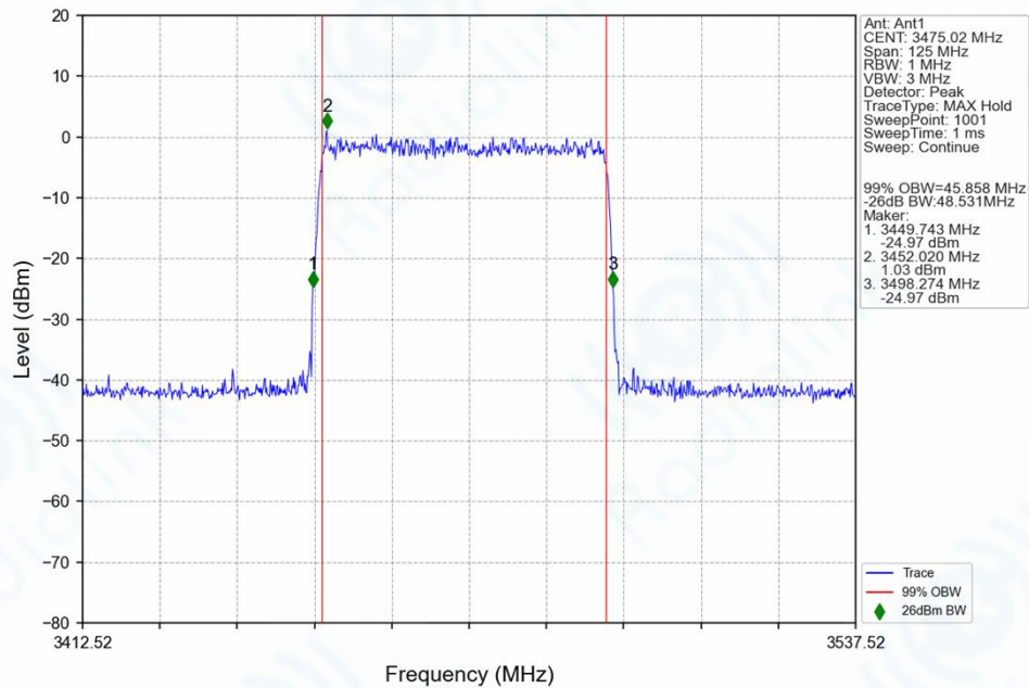
n77g_30kHz_SISO_NTNV_50MHz_DFT-s-OFDM QPSK_3475.02MHz_Outer_Full_Ant1
