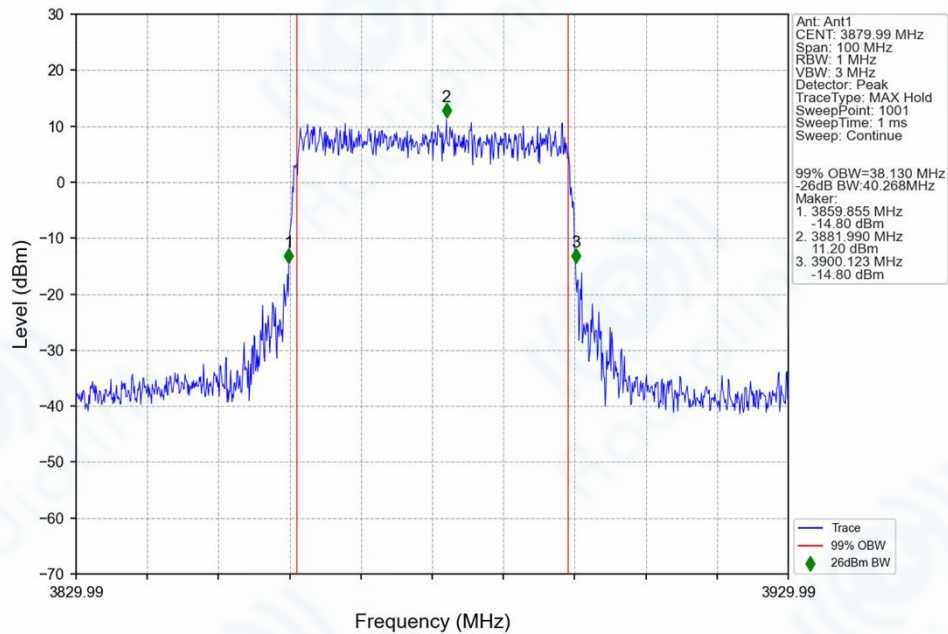
n77g_30kHz_SISO_NTNV_40MHz_CP-OFDM_64_QAM_3879.99MHz_Outer_Full_Ant1
