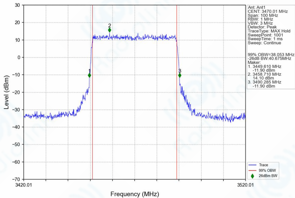
n77g_30kHz_SISO_NTNV_40MHz_CP-OFDM_QPSK_3470.01MHz_Outer_Full_Ant1
