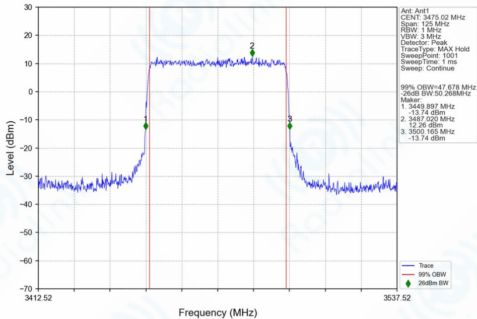
n77g_30kHz_SISO_NTNV_50MHz_CP-OFDM_QPSK_3475.02MHz_Outer_Full_Ant1
