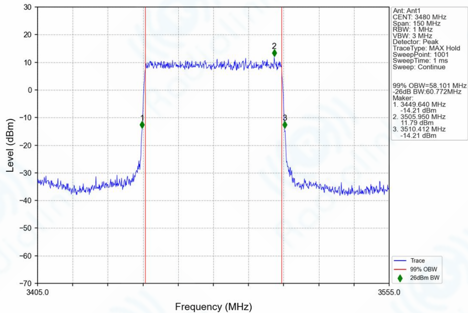
n77g_30kHz_SISO_NTNV_60MHz_DFT-s-OFDM QPSK_3480MHz_Outer_Full_Ant1
