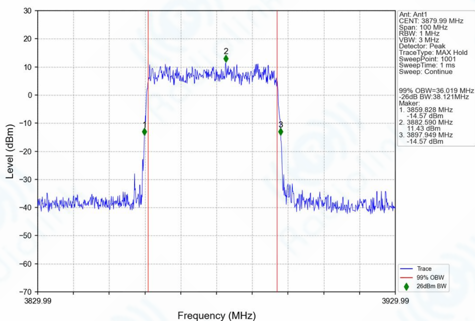
n77g 30kHz SISO NTNV 40MHz DFT-s-OFDM QPSK 3879.99MHz Outer Full Ant1
