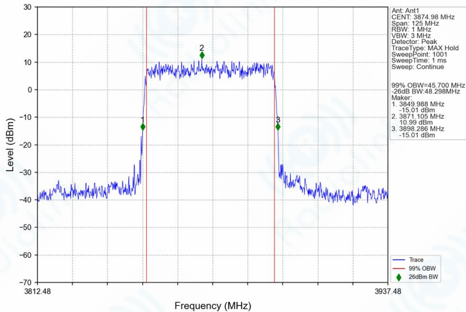
n77g_30kHz_SISO_NTNV_50MHz_DFT-s-OFDM_QPSK_3874.98MHz_Outer_Full_Ant1
