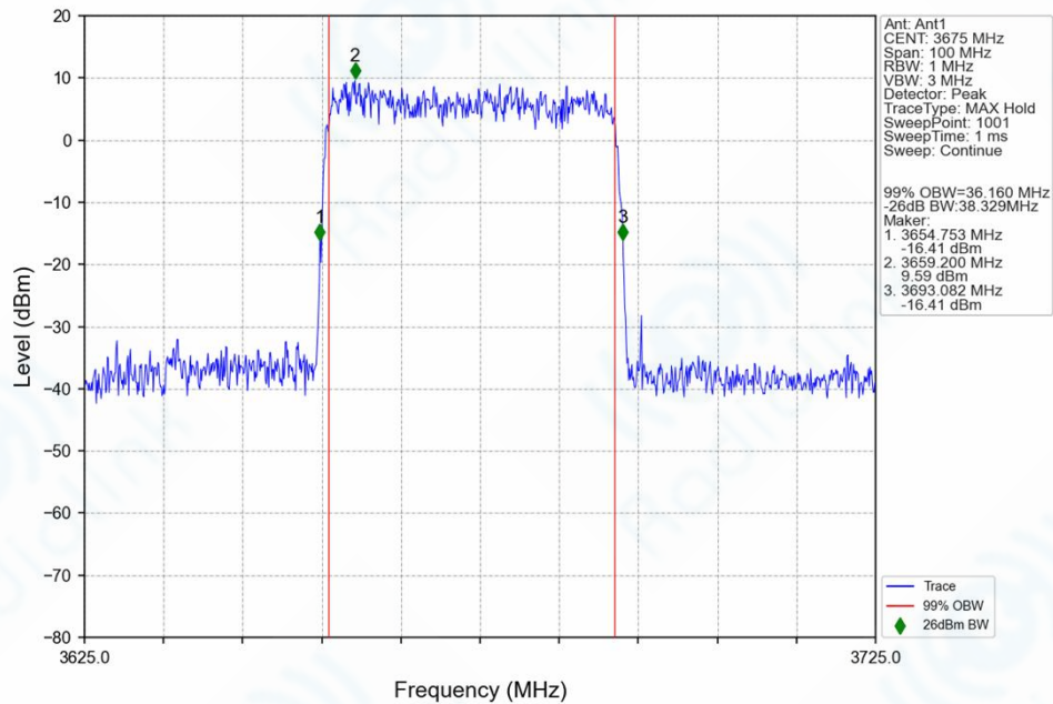
n77g_30kHz_SISO_NTNV_40MHz_DFT-s-OFDM_256_QAM_3675MHz_Outer_Full_Ant1
