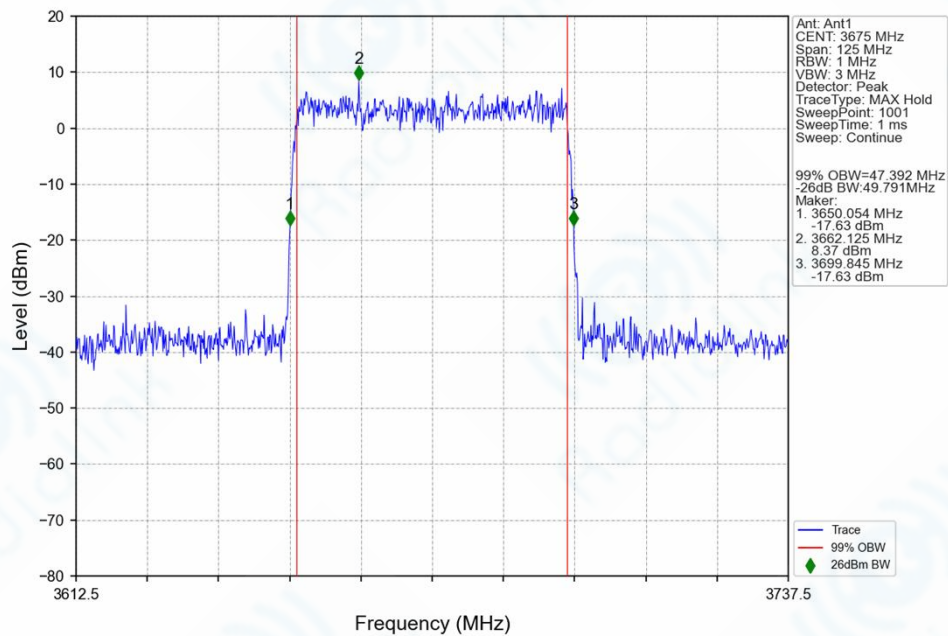
n77g_30kHz_SISO_NTNV_50MHz_CP-OFDM_256_QAM_3675MHz_Outer_Full_Ant1
