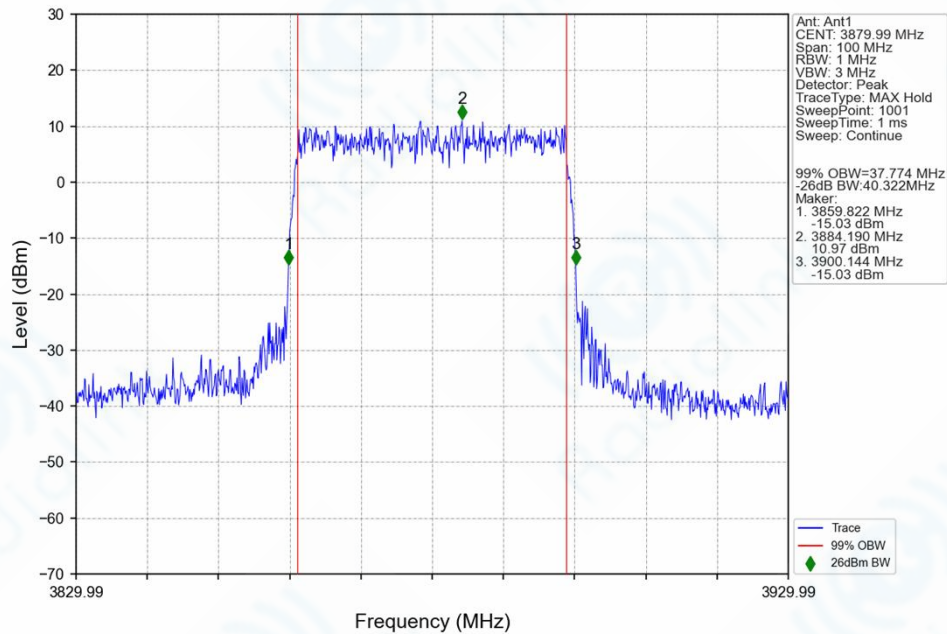
n77g_30kHz_SISO_NTNV_40MHz_CP-OFDM_QPSK_3879.99MHz_Outer_Full_Ant1
