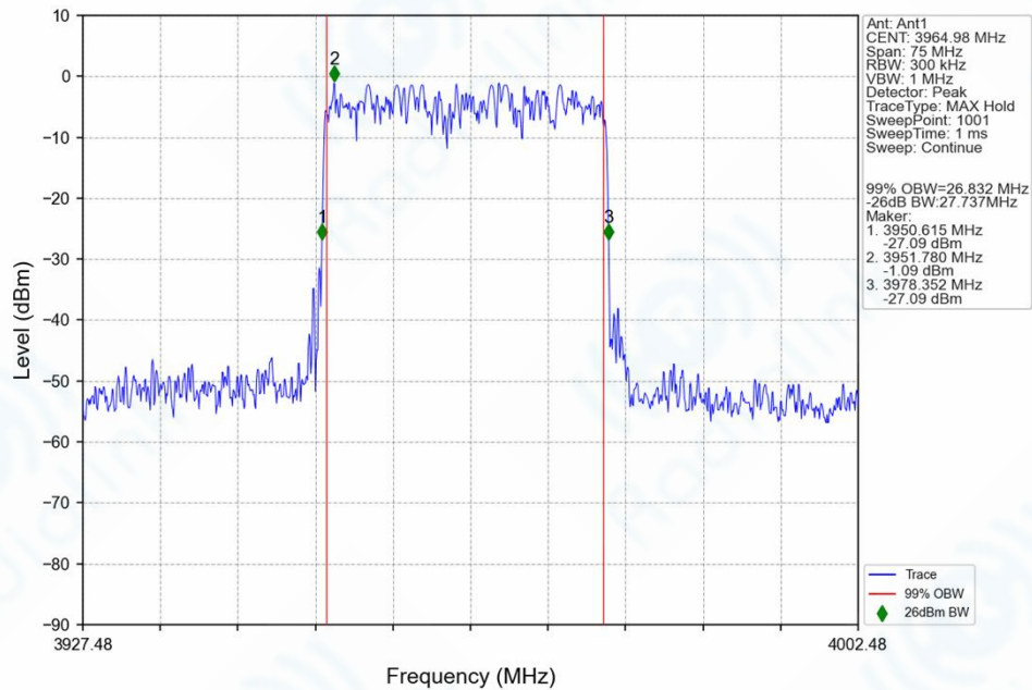
n77h_30kHz_SISO_NTNV_30MHz_DFT-s-OFDM_QPSK_3964.98MHz_Outer_Full_Ant1
