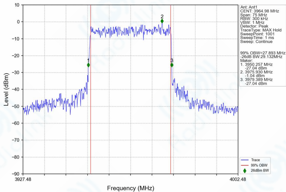
n77h_30kHz_SISO_NTNV_30MHz_CP-OFDM_QPSK_3964.98MHz_Outer_Full_Ant1
