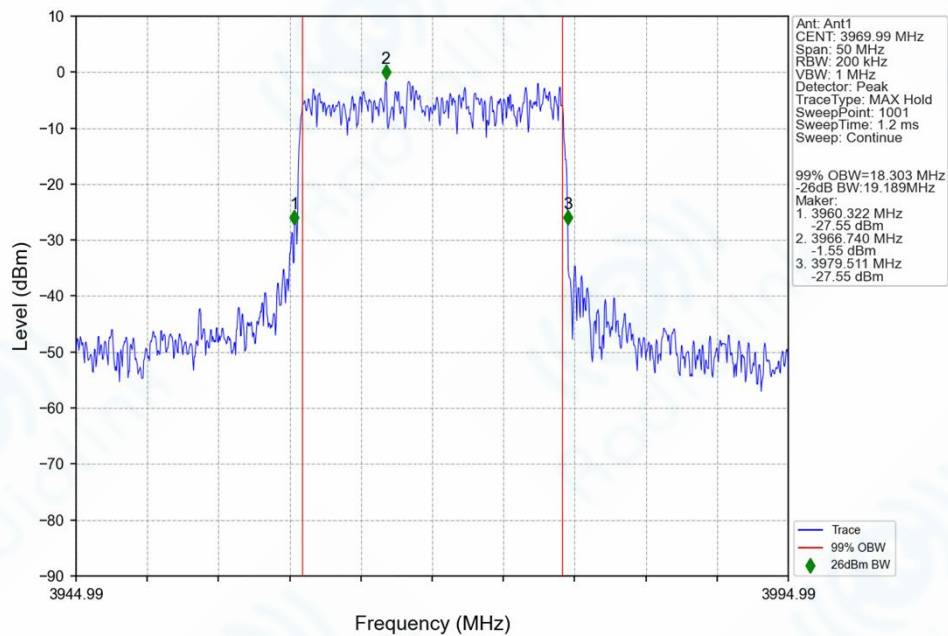
n77h_30kHz_SISO_NTNV_20MHz_CP-OFDM_64_QAM_3969.99MHz_Outer_Full_Ant1
