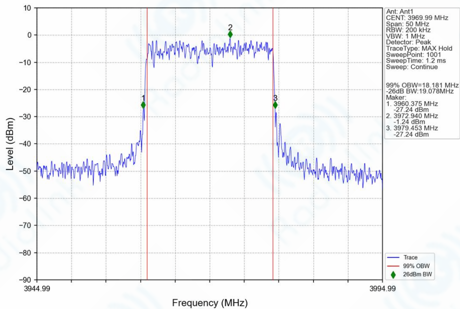
n77h_30kHz_SISO_NTNV_20MHz_CP-OFDM_QPSK_3969.99MHz_Outer_Full_Ant1
