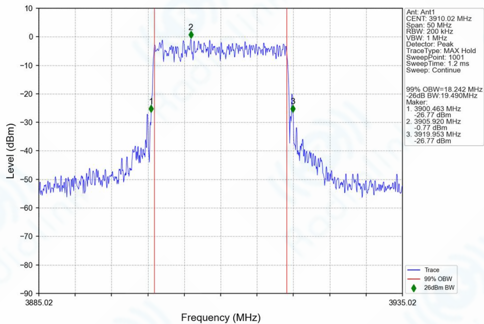
n77h_30kHz_SISO_NTNV_20MHz_CP-OFDM_64_QAM_3910.02MHz_Outer_Full_Ant1
