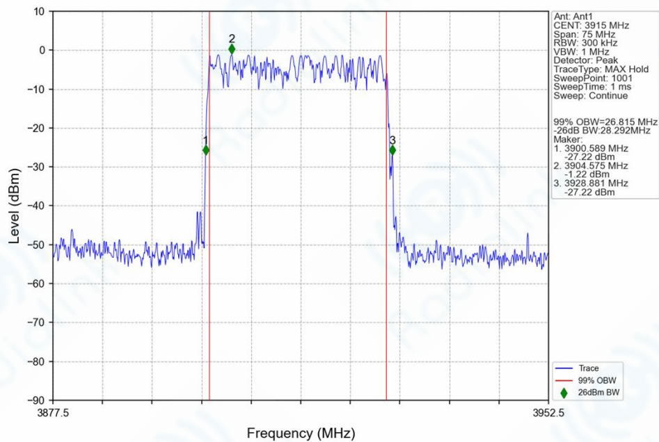
n77h_30kHz_SISO_NTNV_30MHz_DFT-s-OFDM QPSK_3915MHz_Outer_Full_Ant1
