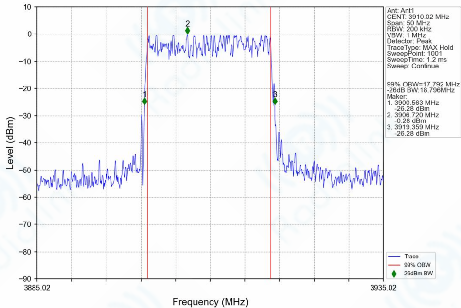
n77h_30kHz_SISO_NTNV_20MHz_DFT-s-OFDM_64_QAM_3910.02MHz_Outer_Full_Ant1
