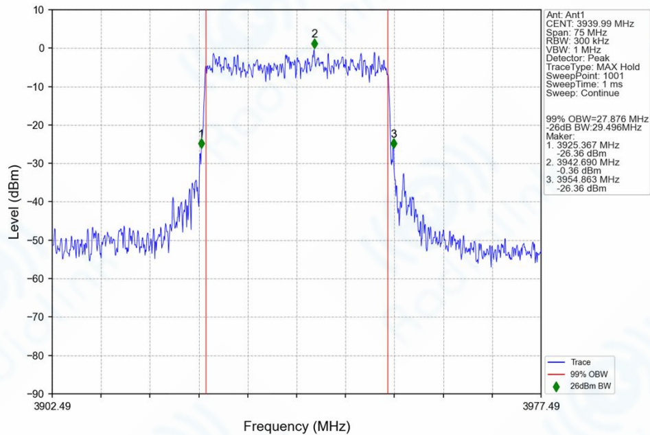
n77h_30kHz_SISO_NTNV_30MHz_CP-OFDM_16_QAM_3939.99MHz_Outer_Full_Ant1
