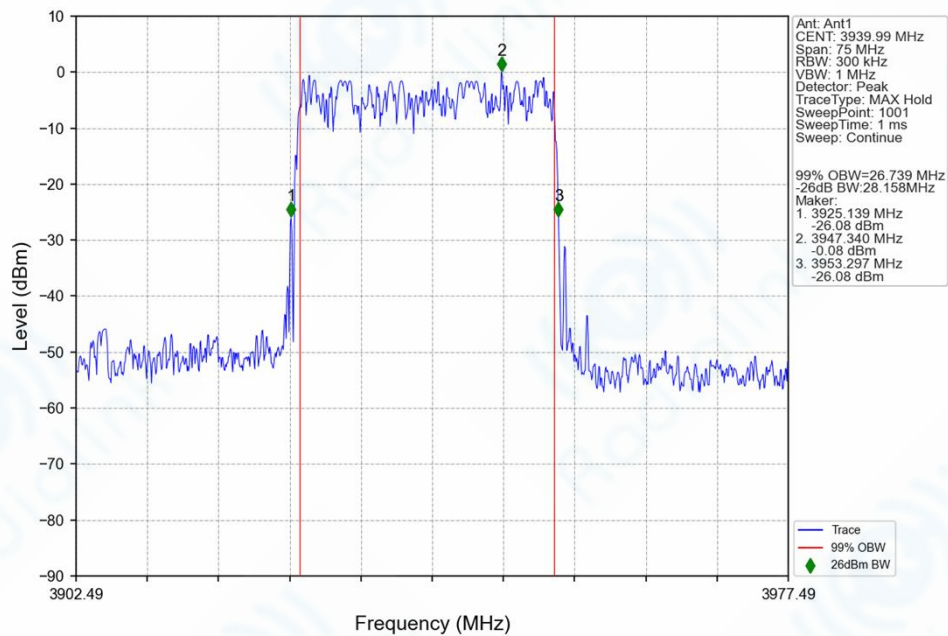
n77h_30kHz_SISO_NTNV_30MHz_DFT-s-OFDM_16_QAM_3939.99MHz_Outer_Full_Ant1
