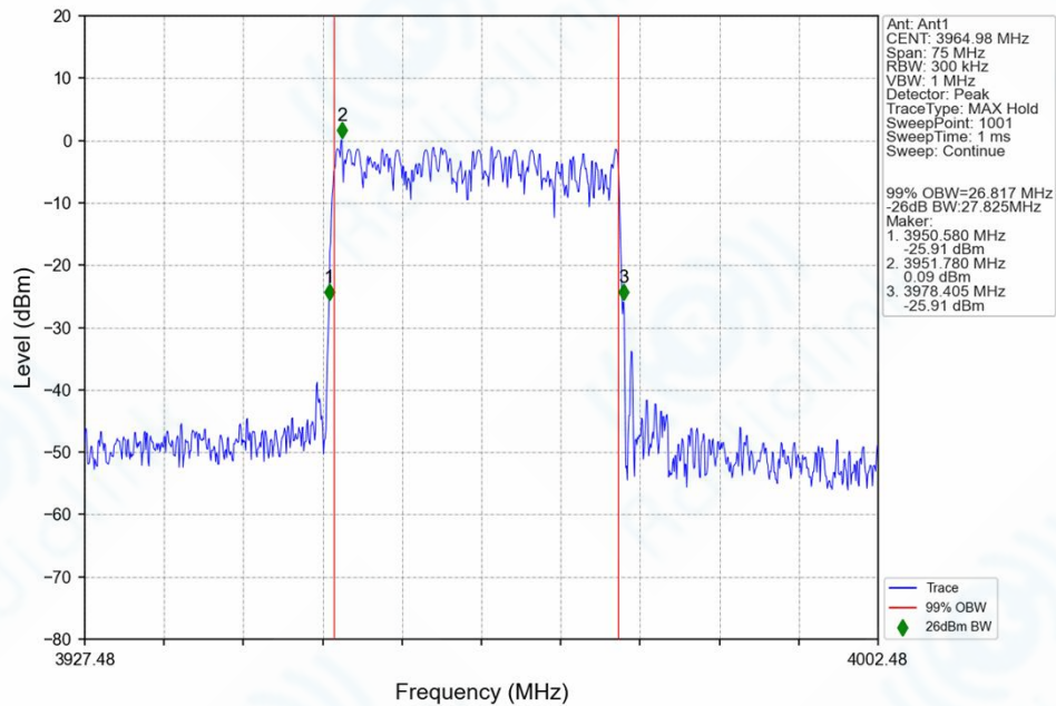
n77h_30kHz_SISO_NTNV_30MHz_DFT-s-OFDM_64_QAM_3964.98MHz_Outer_Full_Ant1
