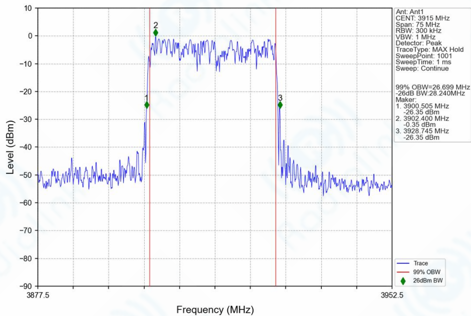
n77h_30kHz_SISO_NTNV_30MHz_DFT-s-OFDM_64_QAM_3915MHz_Outer_Full_Ant1
