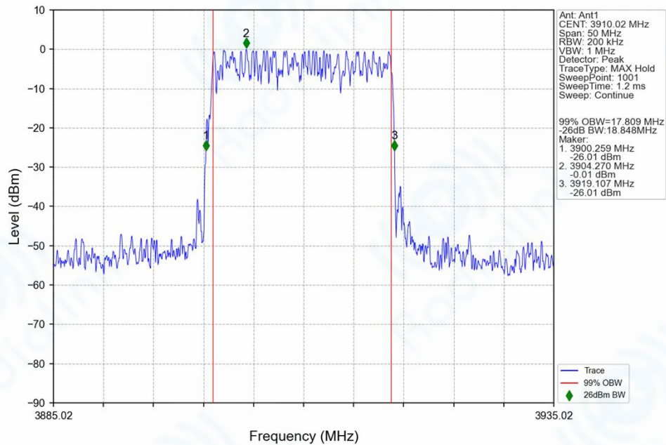
n77h_30kHz_SISO_NTNV_20MHz_DFT-s-OFDM QPSK_3910.02MHz_Outer_Full_Ant1
