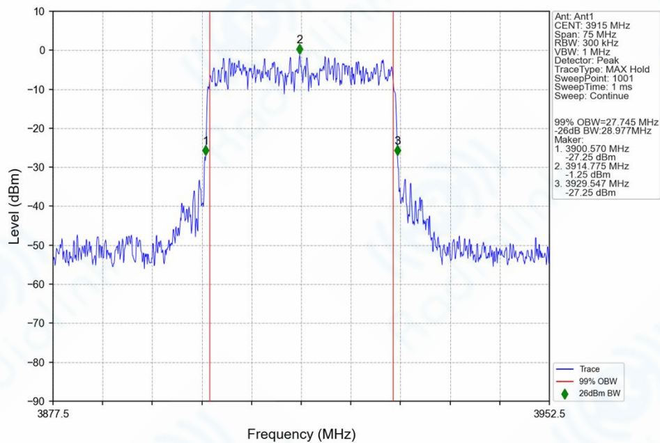
n77h_30kHz_SISO_NTNV_30MHz_CP-OFDM_QPSK_3915MHz_Outer_Full_Ant1
