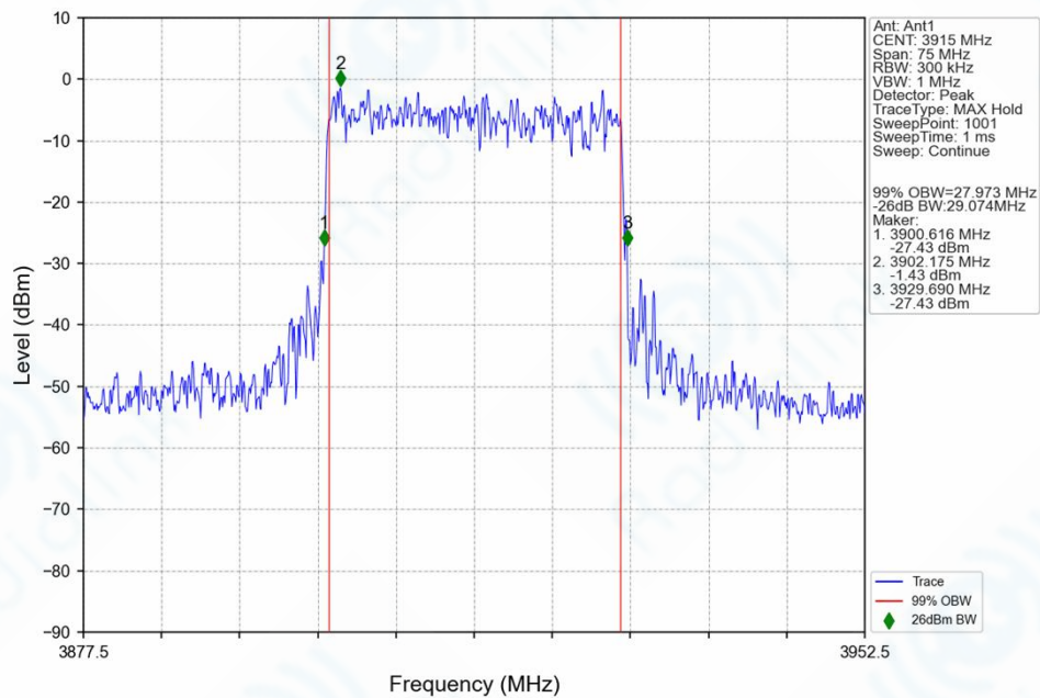
n77h_30kHz_SISO_NTNV_30MHz_CP-OFDM 64 QAM_3915MHz_Outer_Full_Ant1
