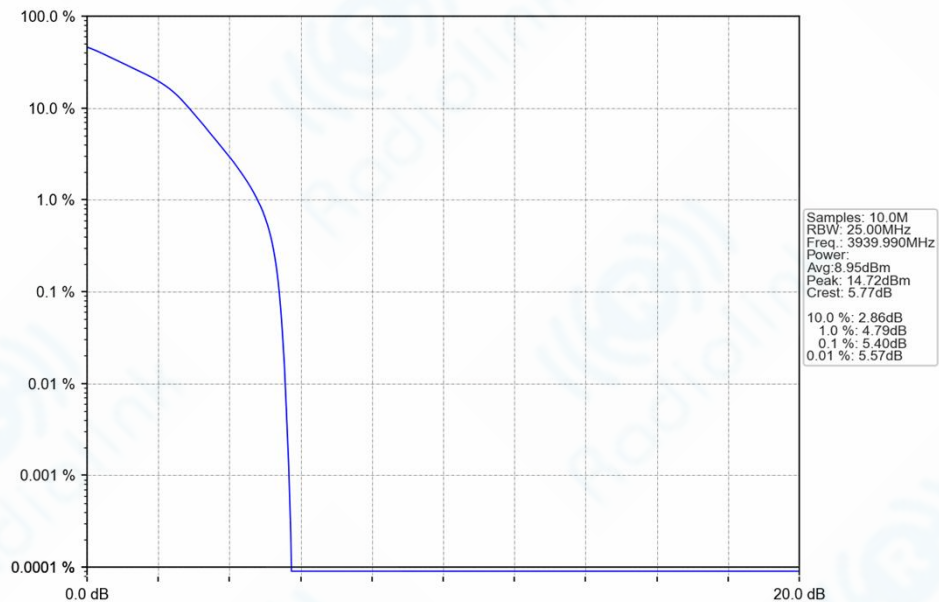
n77h_30kHz_SISO_NTNV_20MHz_DFT-s-OFDM_16_QAM_3939.99MHz_Outer_Full_Ant1
