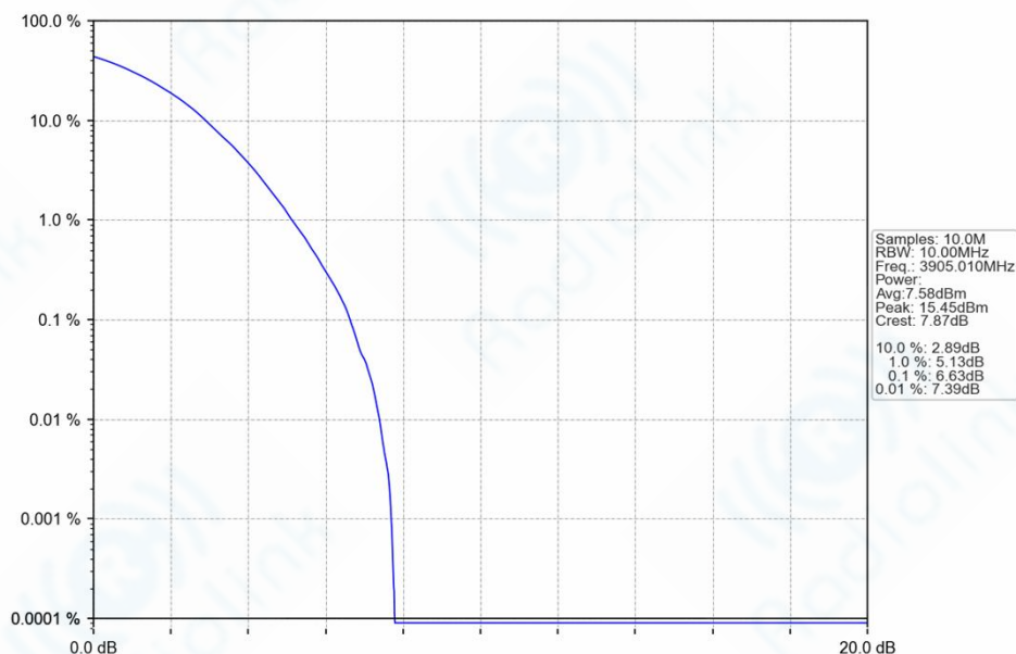
n77h_30kHz_SISO_NTNV_10MHz_DFT-s-OFDM_256_QAM_3905.01MHz_Outer_Full_Ant1
