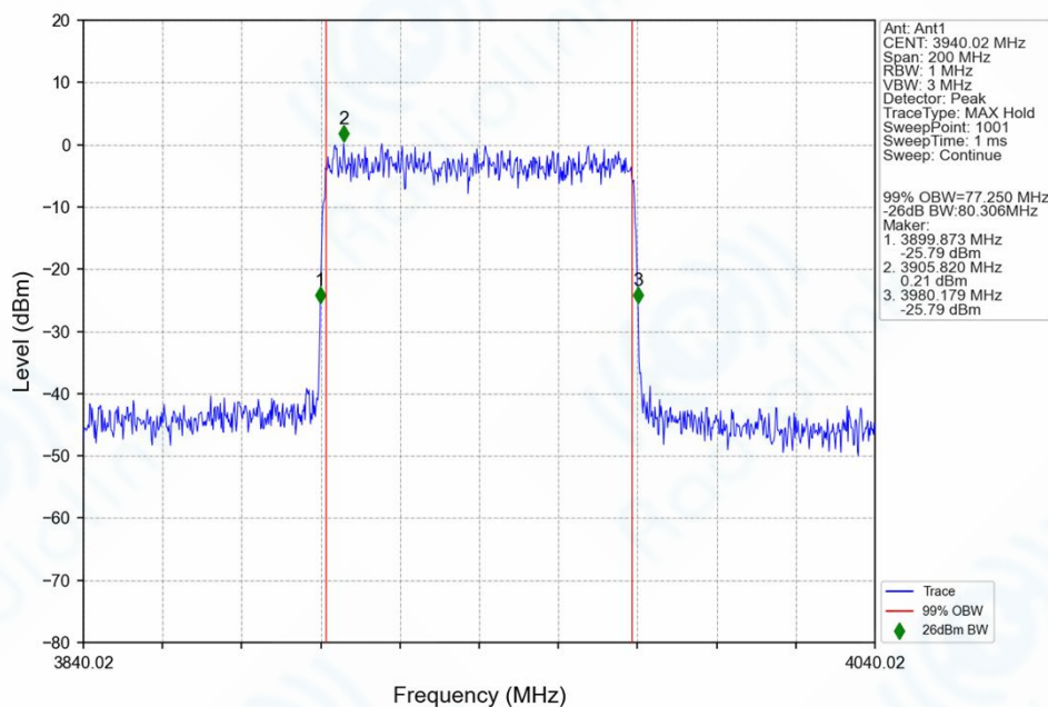
n77h_30kHz_SISO_NTNV_80MHz_CP-OFDM_QPSK_3940.02MHz_Outer_Full_Ant1
