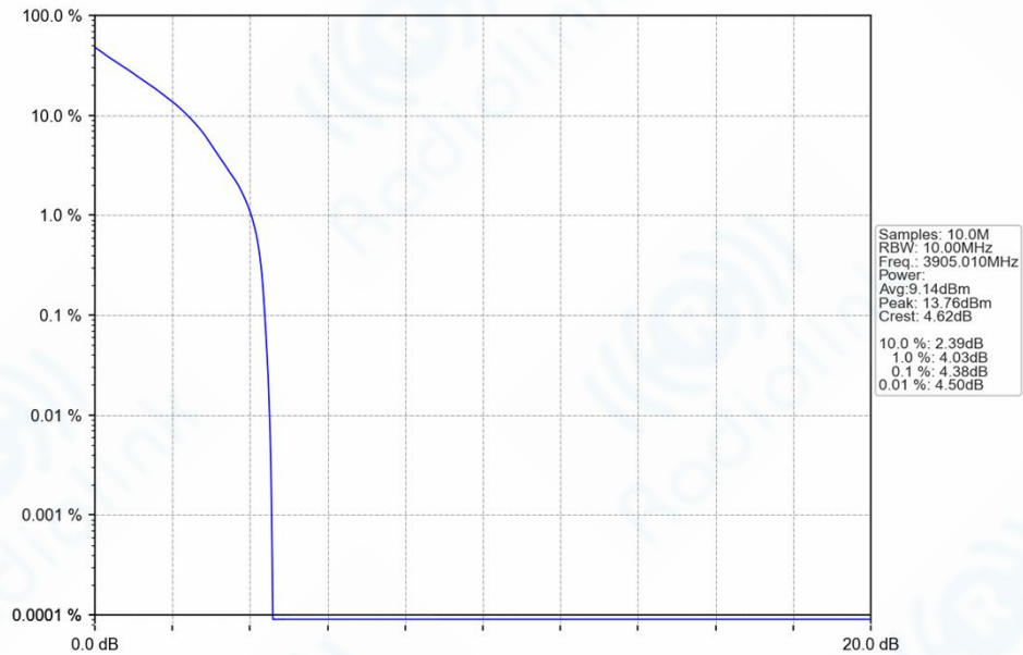
n77h_30kHz_SISO_NTNV_10MHz_DFT-s-OFDM QPSK_3905.01MHz_Outer_Full_Ant1
