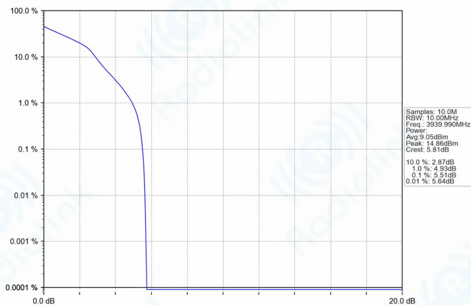
n77h_30kHz_SISO_NTNV_10MHz_DFT-s-OFDM_16_QAM_3939.99MHz_Outer_Full_Ant1
