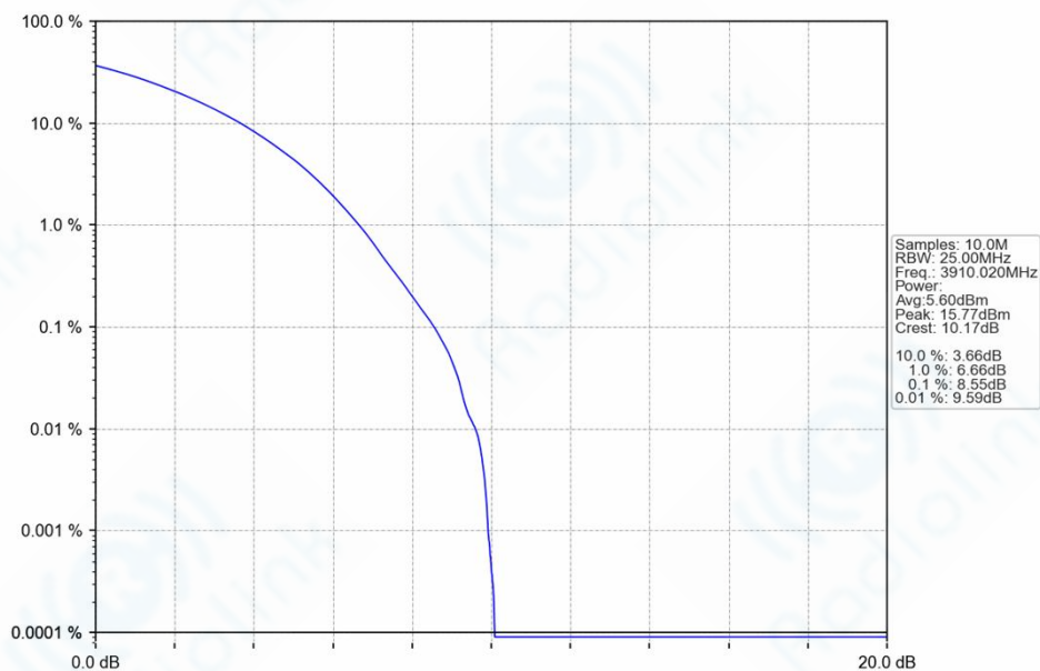
n77h_30kHz_SISO_NTNV_20MHz_CP-OFDM_256_QAM_3910.02MHz_Outer_Full_Ant1
