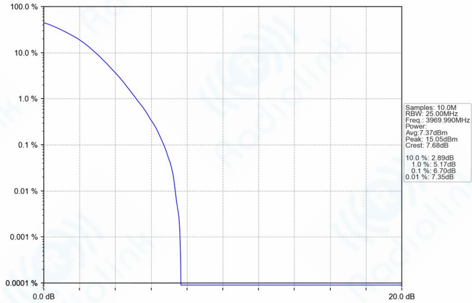
n77h_30kHz_SISO_NTNV_20MHz_DFT-s-OFDM_256_QAM_3969.99MHz_Outer_Full_Ant1
