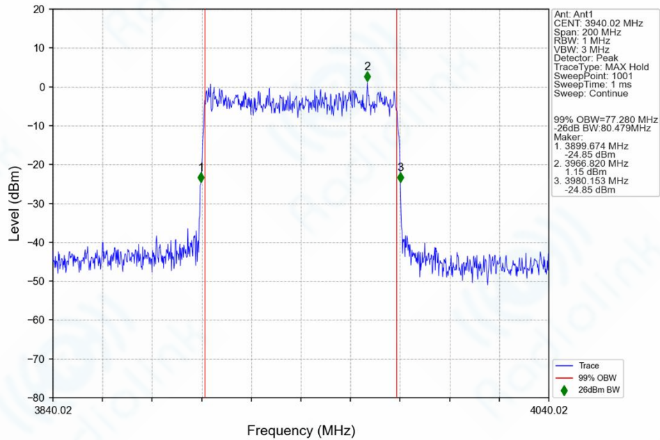
n77h_30kHz_SISO_NTNV_80MHz_CP-OFDM_64_QAM_3940.02MHz_Outer_Full_Ant1
