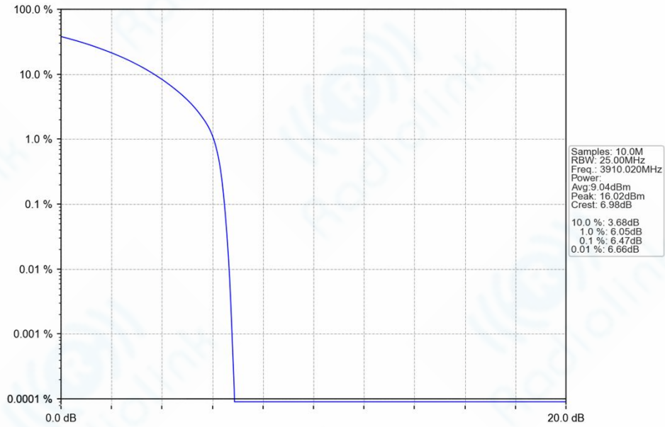
n77h_30kHz_SISO_NTNV_20MHz_CP-OFDM_16_QAM_3910.02MHz_Outer_Full_Ant1
