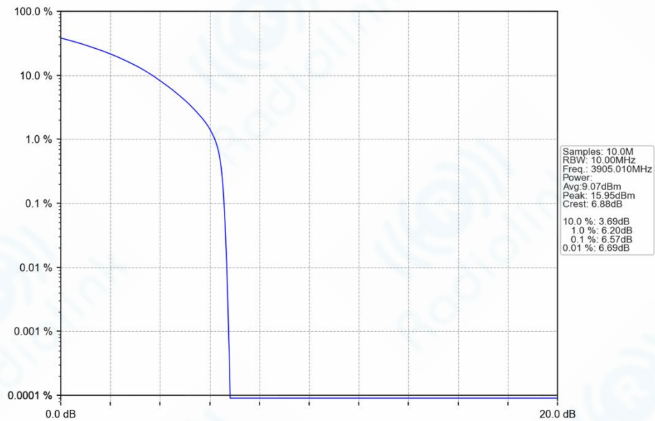
n77h_30kHz_SISO_NTNV_10MHz_CP-OFDM_QPSK_3905.01MHz_Outer_Full_Ant1
