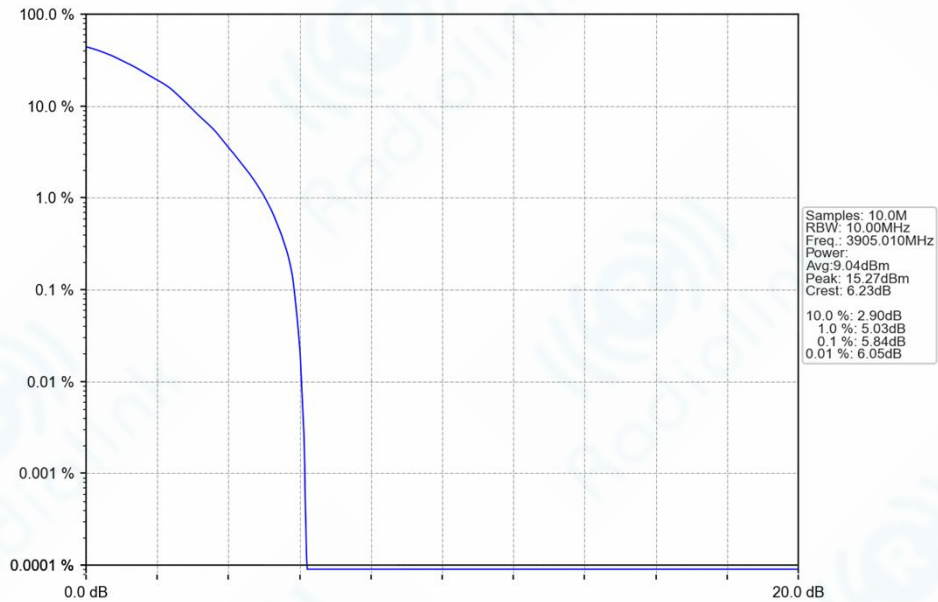
n77h_30kHz_SISO_NTNV_10MHz_DFT-s-OFDM_64_QAM_3905.01MHz_Outer_Full_Ant1
