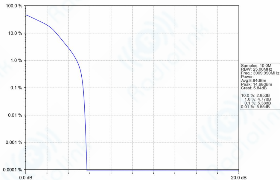
n77h_30kHz_SISO_NTNV_20MHz_DFT-s-OFDM_16_QAM_3969.99MHz_Outer_Full_Ant1
