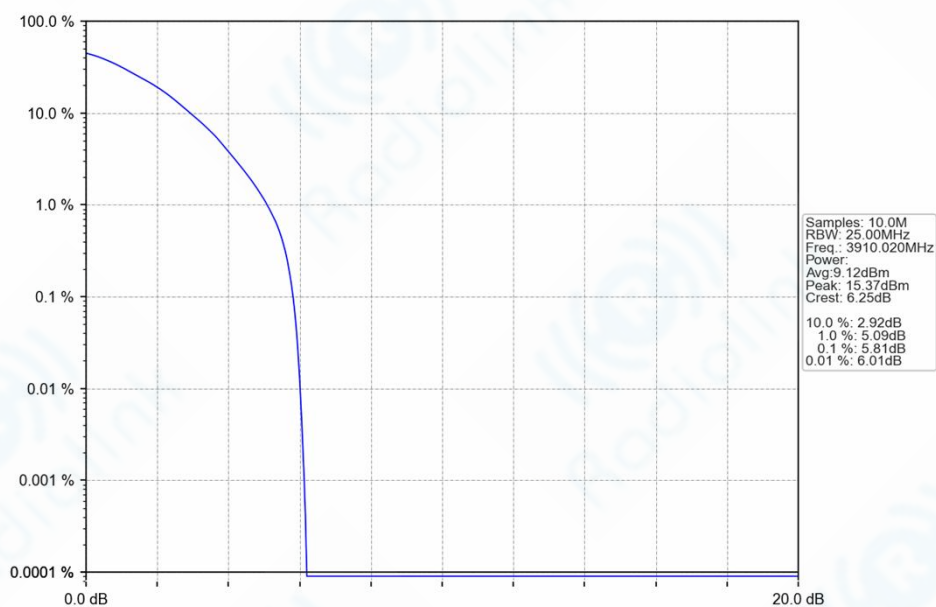
n77h_30kHz_SISO_NTNV_20MHz_DFT-s-OFDM_64_QAM_3910.02MHz_Outer_Full_Ant1
