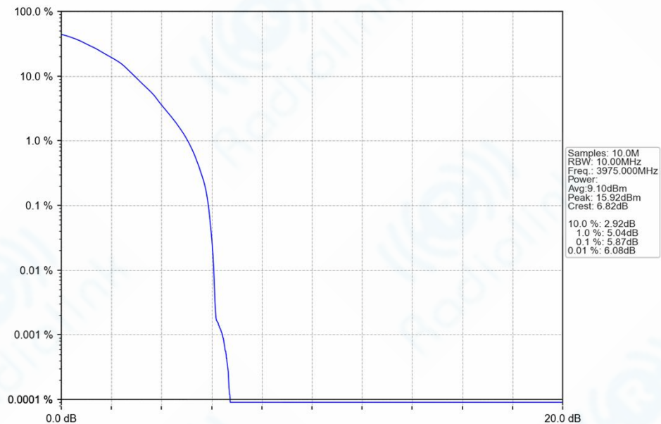
n77h_30kHz_SISO_NTNV_10MHz_DFT-s-OFDM_64_QAM_3975MHz_Outer_Full_Ant1
