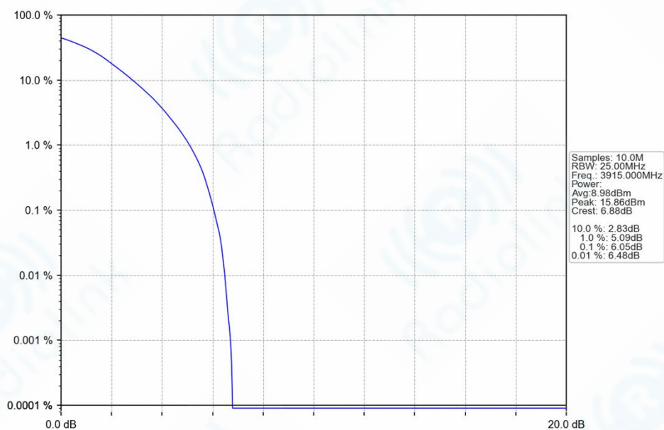
n77h_30kHz_SISO_NTNV_30MHz_DFT-s-OFDM_64_QAM_3915MHz_Outer_Full_Ant1
