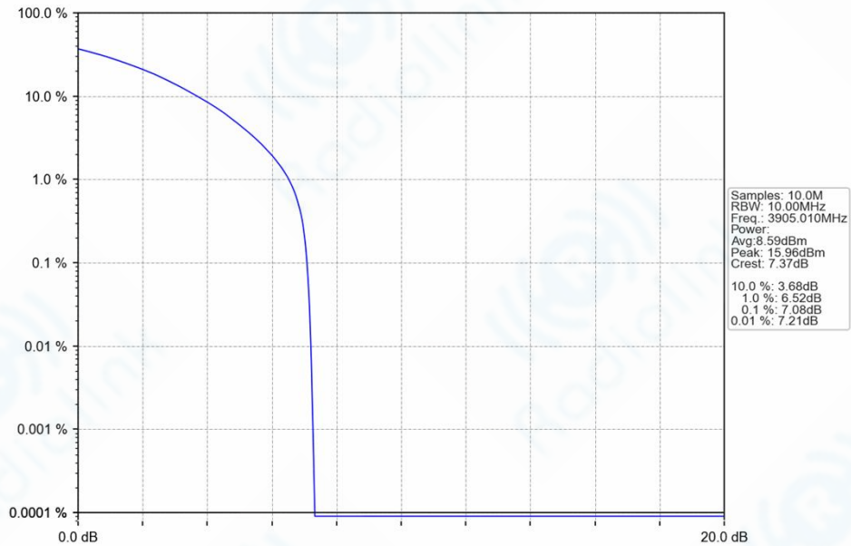
n77h_30kHz_SISO_NTNV_10MHz_CP-OFDM_64_QAM_3905.01MHz_Outer_Full_Ant1
