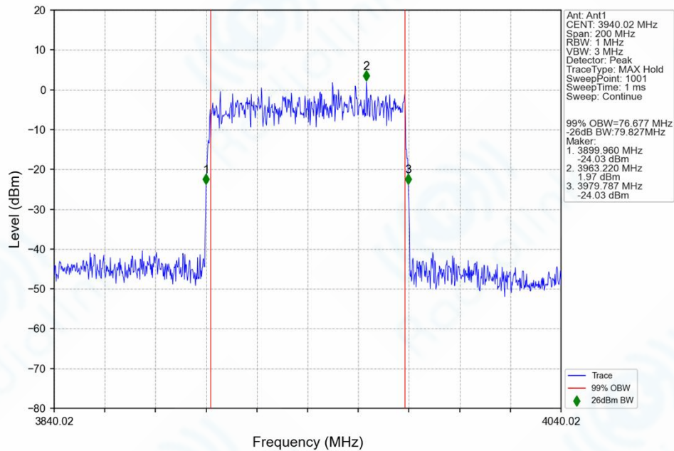
n77h_30kHz_SISO_NTNV_80MHz_DFT-s-OFDM_64_QAM_3940.02MHz_Outer_Full_Ant1
