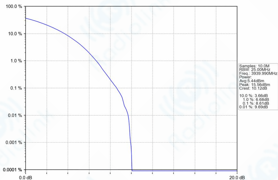
n77h_30kHz_SISO_NTNV_20MHz_CP-OFDM_256_QAM_3939.99MHz_Outer_Full_Ant1
