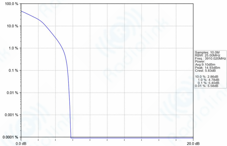
n77h_30kHz_SISO_NTNV_20MHz_DFT-s-OFDM_16_QAM_3910.02MHz_Outer_Full_Ant1
