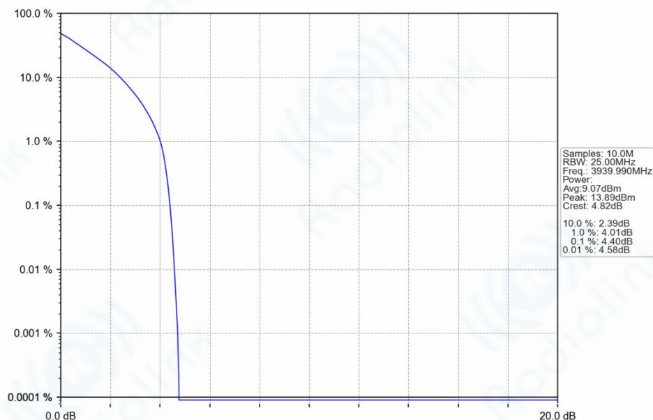
n77h_30kHz_SISO_NTNV_20MHz_DFT-s-OFDM_QPSK_3939.99MHz_Outer_Full_Ant1
