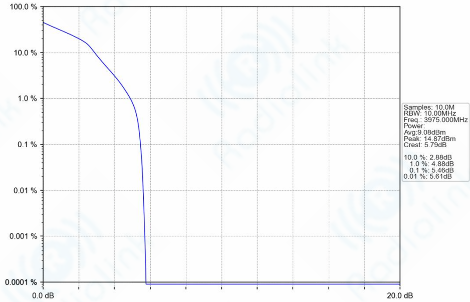
n77h_30kHz_SISO_NTNV_10MHz_DFT-s-OFDM_16_QAM_3975MHz_Outer_Full_Ant1
