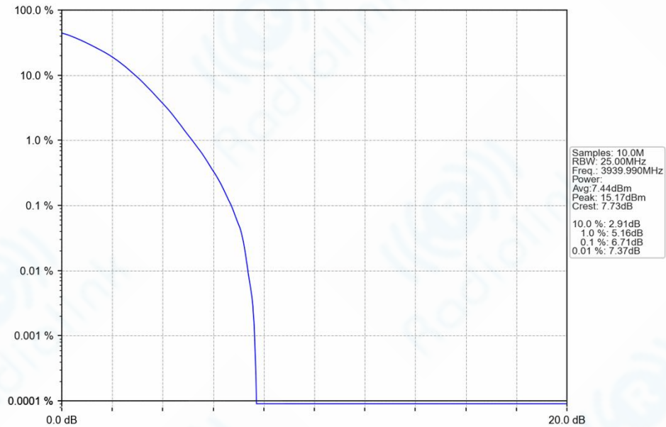
n77h_30kHz_SISO_NTNV_20MHz_DFT-s-OFDM_256_QAM_3939.99MHz_Outer_Full_Ant1
