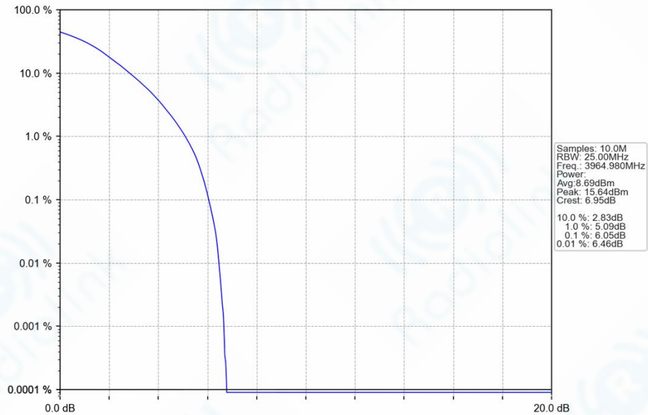
n77h_30kHz_SISO_NTNV_30MHz_DFT-s-OFDM_64_QAM_3964.98MHz_Outer_Full_Ant1
