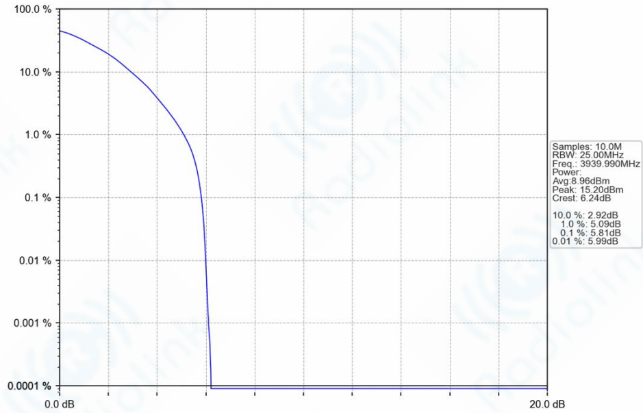
n77h_30kHz_SISO_NTNV_20MHz_DFT-s-OFDM_64_QAM_3939.99MHz_Outer_Full_Ant1
