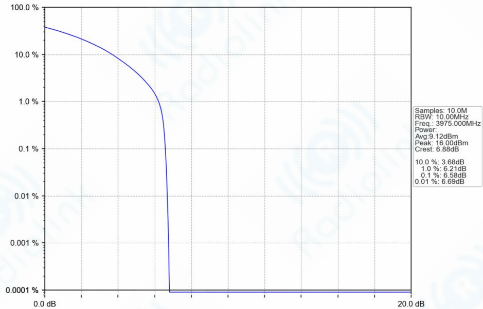
n77h_30kHz_SISO_NTNV_10MHz_CP-OFDM_QPSK_3975MHz_Outer_Full_Ant1
