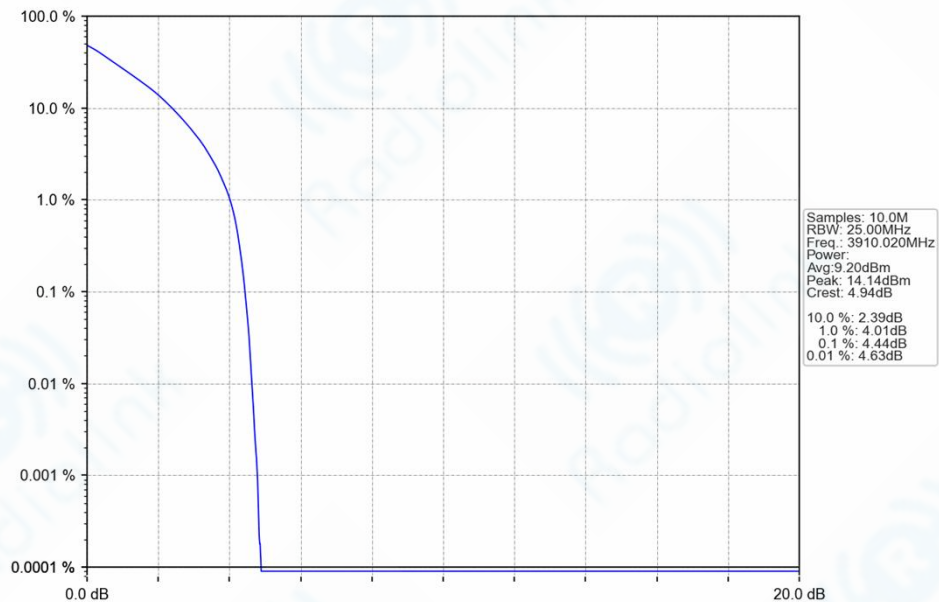
n77h_30kHz_SISO_NTNV_20MHz_DFT-s-OFDM_QPSK_3910.02MHz_Outer_Full_Ant1
