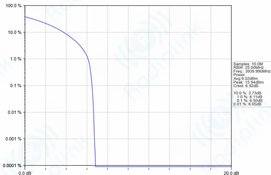
n77h_30kHz_SISO_NTNV_20MHz_CP-OFDM_QPSK_3939.99MHz_Outer_Full_Ant1
