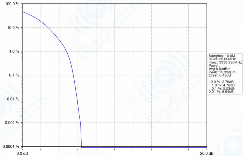
n77h_30kHz_SISO_NTNV_30MHz_DFT-s-OFDM_16_QAM_3939.99MHz_Outer_Full_Ant1
