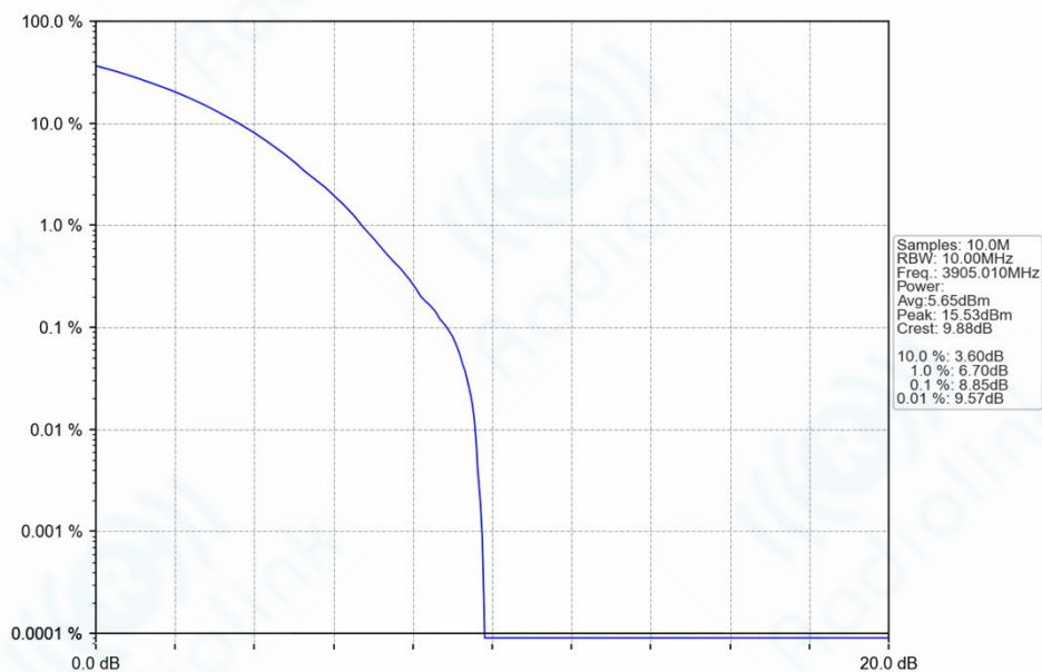
n77h_30kHz_SISO_NTNV_10MHz_CP-OFDM_256_QAM_3905.01MHz_Outer_Full_Ant1
