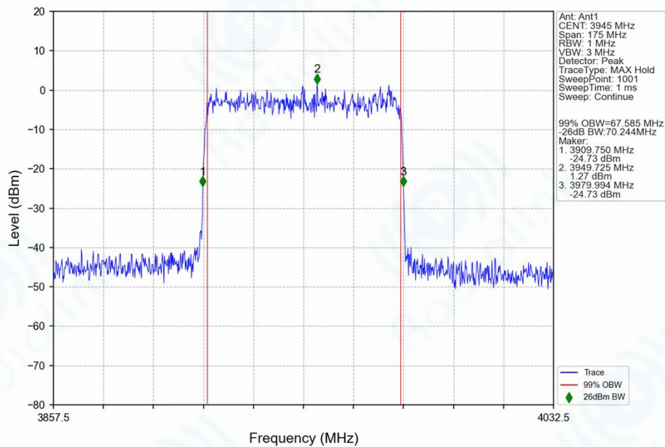
n77h_30kHz_SISO_NTNV_70MHz_CP-OFDM_QPSK_3945MHz_Outer_Full_Ant1
