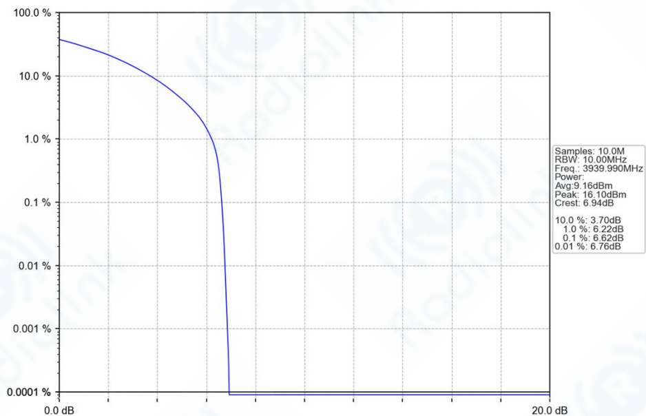
n77h_30kHz_SISO_NTNV_10MHz_CP-OFDM_16_QAM_3939.99MHz_Outer_Full_Ant1
