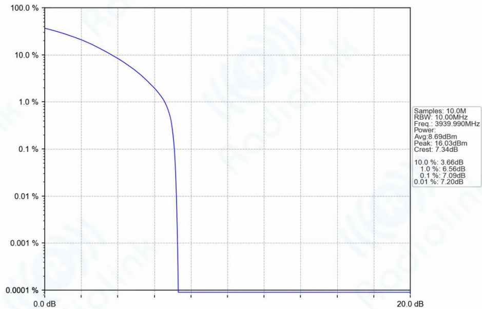
n77h_30kHz_SISO_NTNV_10MHz_CP-OFDM_64_QAM_3939.99MHz_Outer_Full_Ant1
