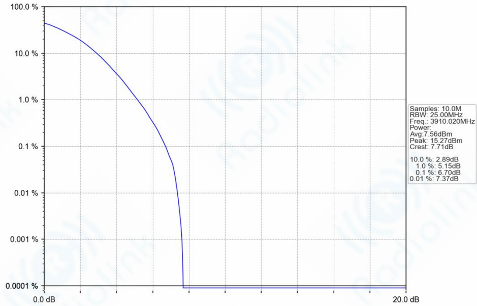
n77h_30kHz_SISO_NTNV_20MHz_DFT-s-OFDM_256_QAM_3910.02MHz_Outer_Full_Ant1
