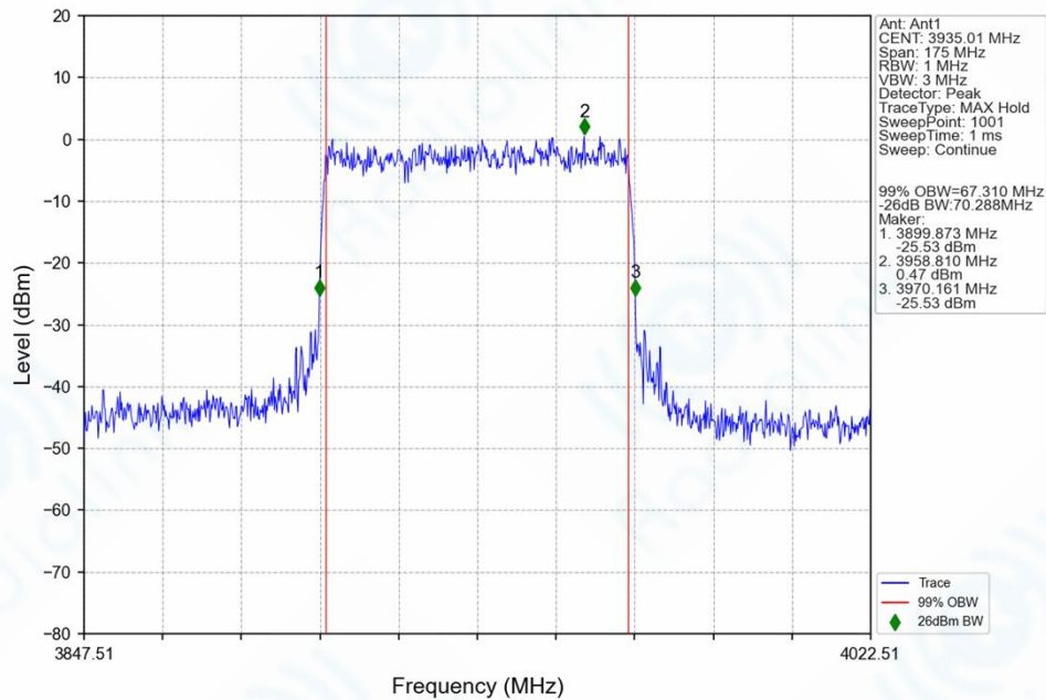
n77h_30kHz_SISO_NTNV_70MHz_CP-OFDM_64_QAM_3935.01MHz_Outer_Full_Ant1
