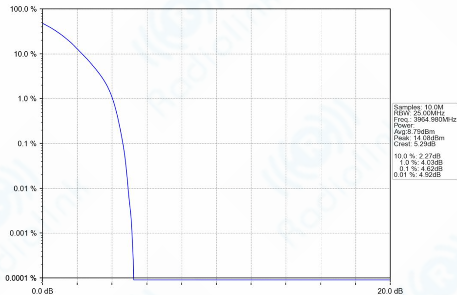
n77h_30kHz_SISO_NTNV_30MHz_DFT-s-OFDM_QPSK_3964.98MHz_Outer_Full_Ant1
