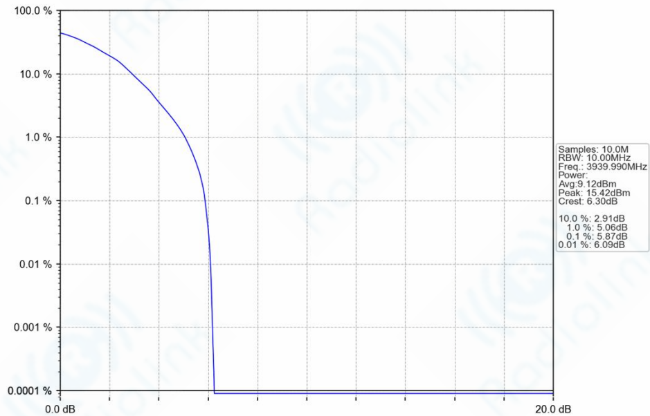
n77h_30kHz_SISO_NTNV_10MHz_DFT-s-OFDM_64_QAM_3939.99MHz_Outer_Full_Ant1
