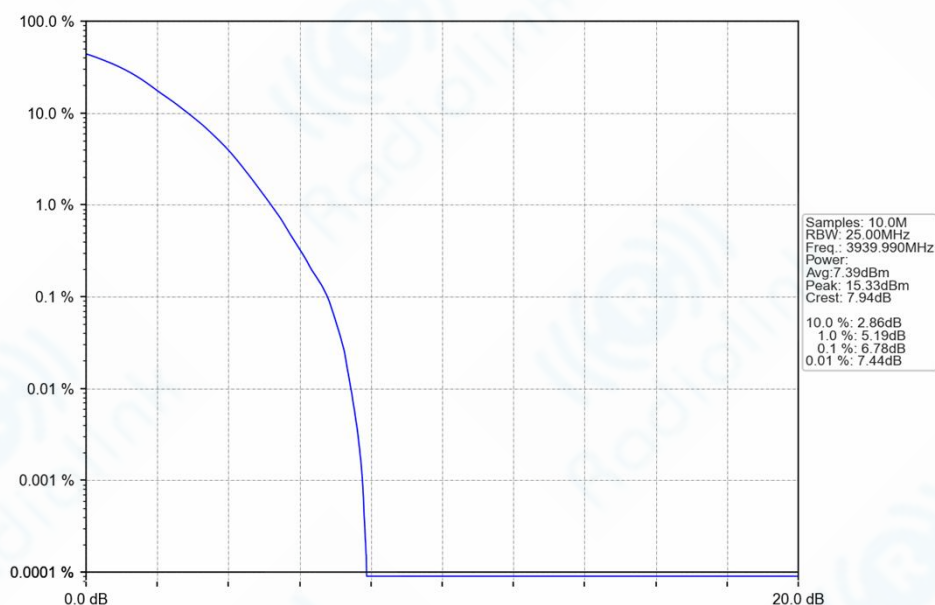
n77h_30kHz_SISO_NTNV_30MHz_DFT-s-OFDM_256_QAM_3939.99MHz_Outer_Full_Ant1
