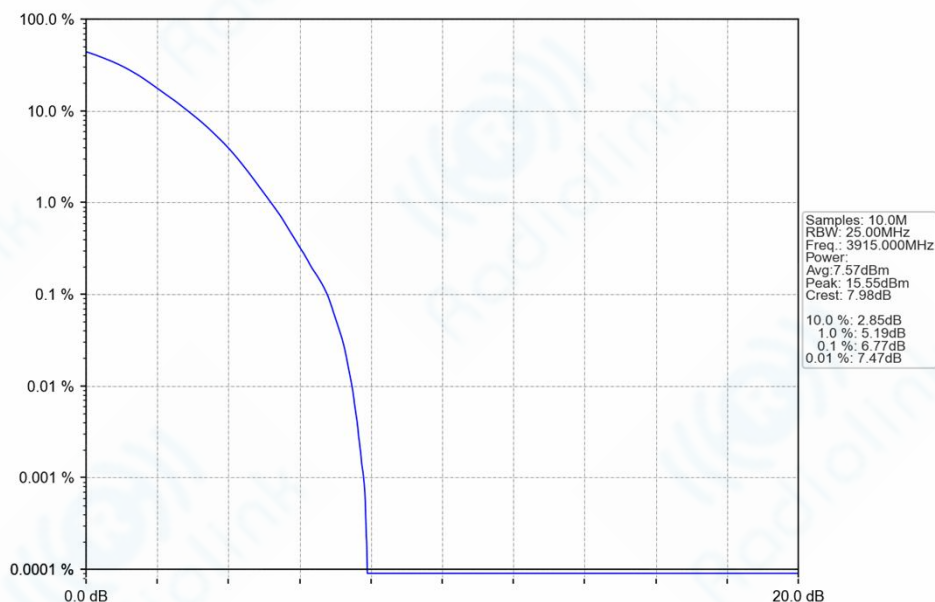
n77h_30kHz_SISO_NTNV_30MHz_DFT-s-OFDM_256_QAM_3915MHz_Outer_Full_Ant1
