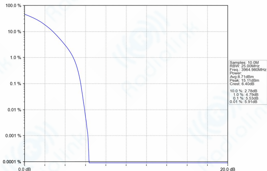
n77h_30kHz_SISO_NTNV_30MHz_DFT-s-OFDM_16_QAM_3964.98MHz_Outer_Full_Ant1
