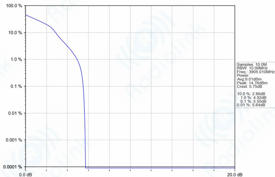
n77h_30kHz_SISO_NTNV_10MHz_DFT-s-OFDM_16_QAM_3905.01MHz_Outer_Full_Ant1
