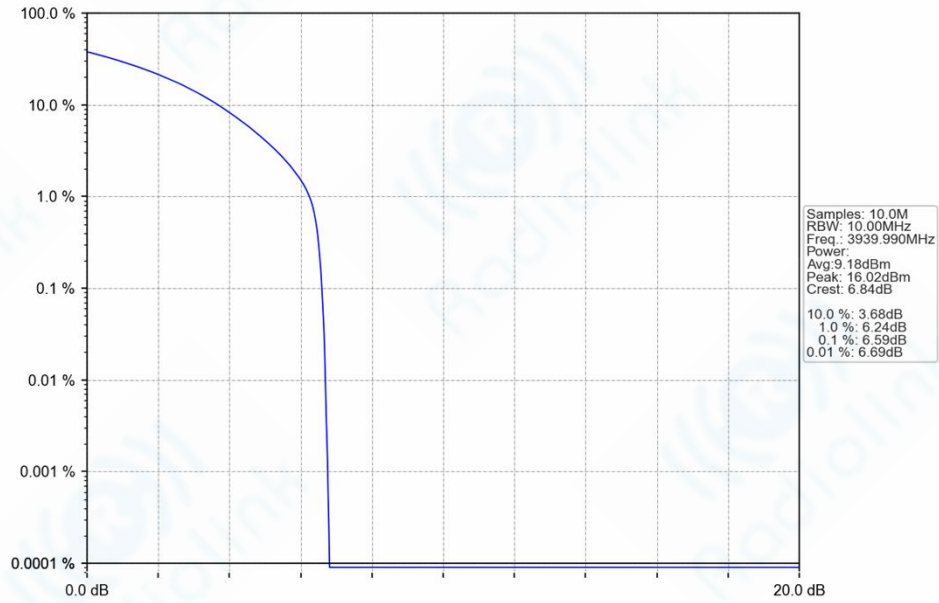
n77h_30kHz_SISO_NTNV_10MHz_CP-OFDM_QPSK_3939.99MHz_Outer_Full_Ant1
