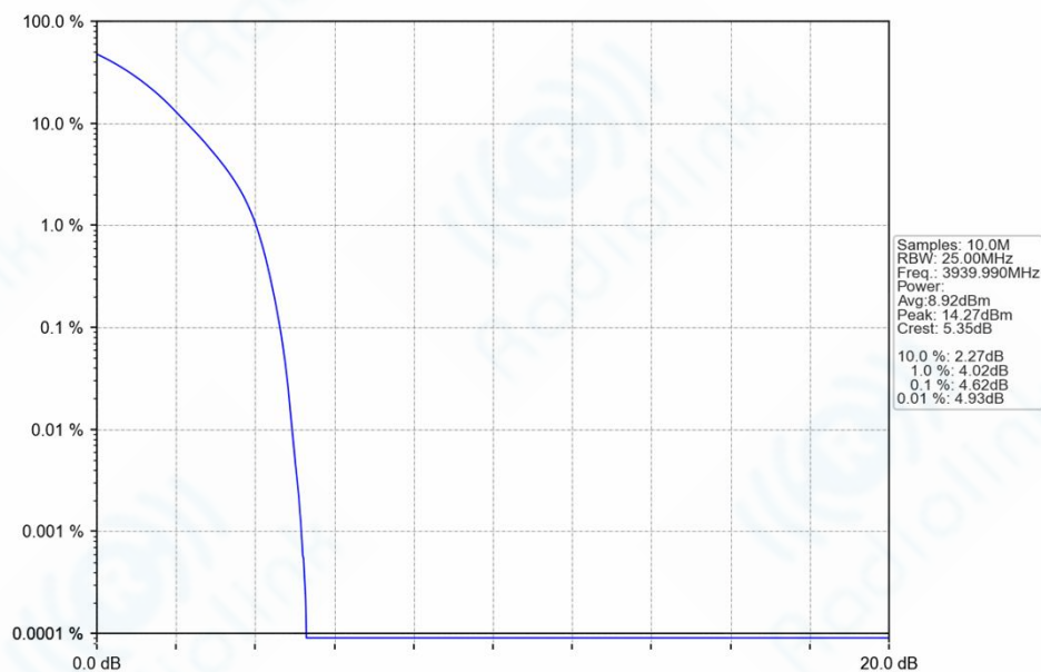
n77h_30kHz_SISO_NTNV_30MHz_DFT-s-OFDM_QPSK_3939.99MHz_Outer_Full_Ant1
