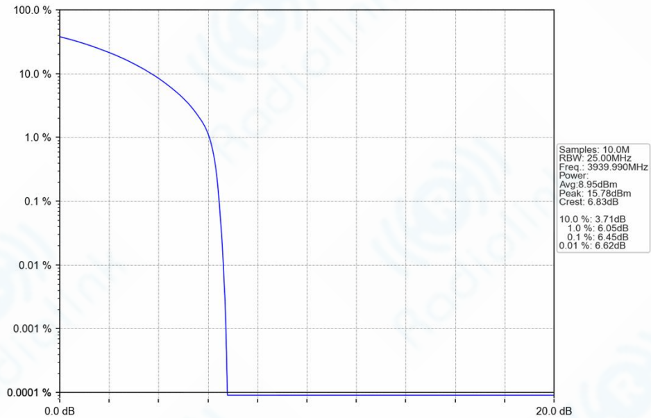
n77h_30kHz_SISO_NTNV_20MHz_CP-OFDM_16_QAM_3939.99MHz_Outer_Full_Ant1
