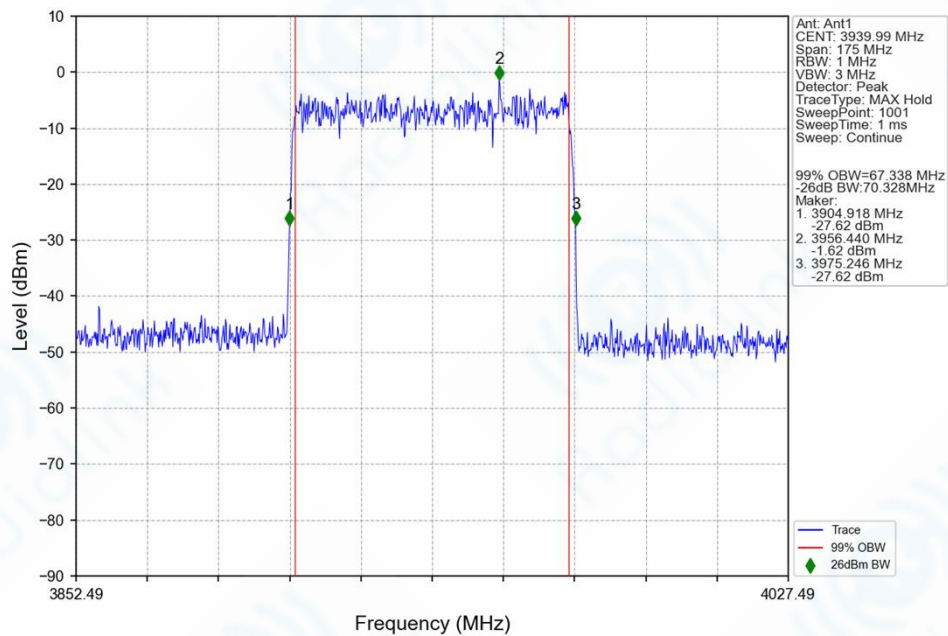
n77h_30kHz_SISO_NTNV_70MHz_CP-OFDM_256_QAM_3939.99MHz_Outer_Full_Ant1
