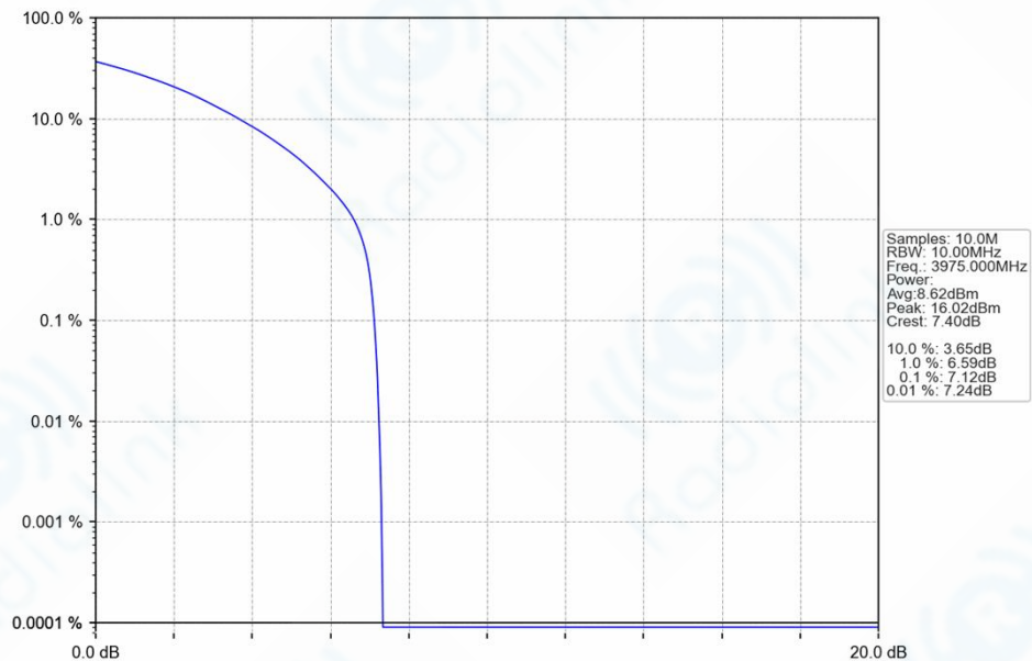
n77h_30kHz_SISO_NTNV_10MHz_CP-OFDM_64_QAM_3975MHz_Outer_Full_Ant1
