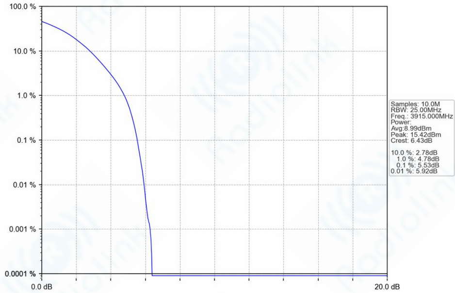
n77h_30kHz_SISO_NTNV_30MHz_DFT-s-OFDM_16_QAM_3915MHz_Outer_Full_Ant1
