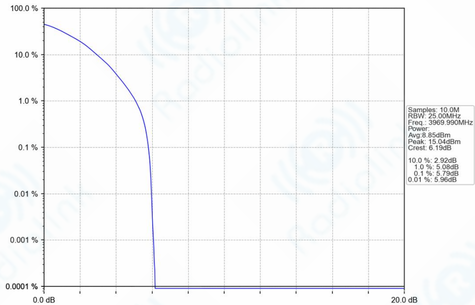
n77h_30kHz_SISO_NTNV_20MHz_DFT-s-OFDM_64_QAM_3969.99MHz_Outer_Full_Ant1
