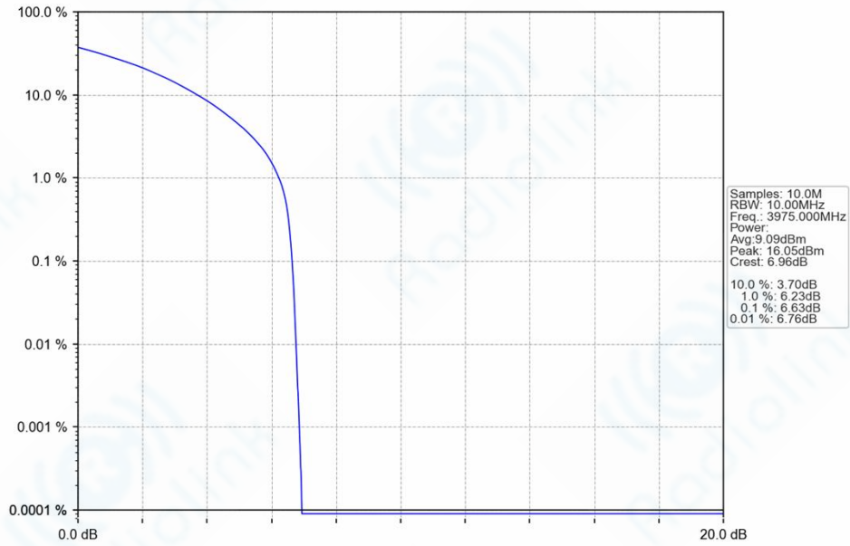
n77h_30kHz_SISO_NTNV_10MHz_CP-OFDM_16_QAM_3975MHz_Outer_Full_Ant1
