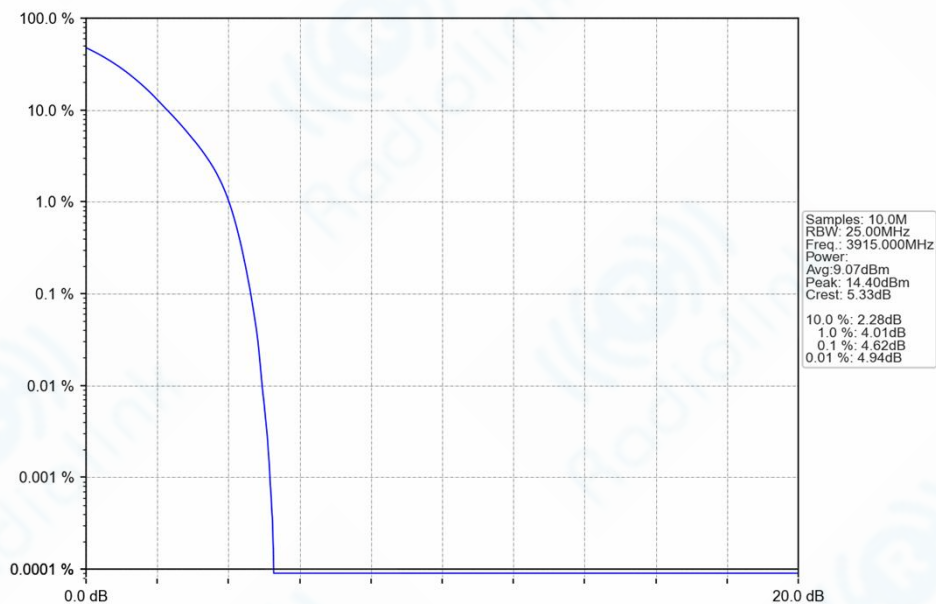
n77h_30kHz_SISO_NTNV_30MHz_DFT-s-OFDM QPSK_3915MHz_Outer_Full_Ant1
