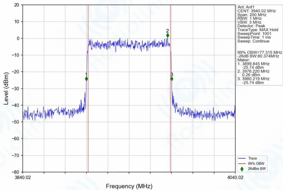
n77h_30kHz_SISO_NTNV_80MHz_CP-OFDM_64_QAM_3940.02MHz_Outer_Full_Ant1
