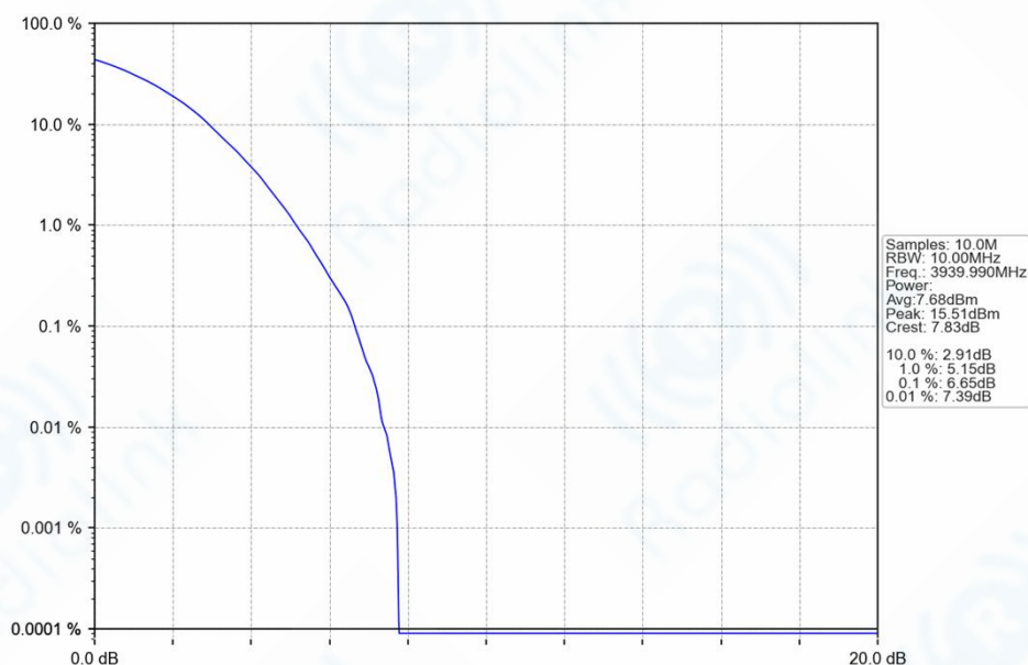
n77h_30kHz_SISO_NTNV_10MHz_DFT-s-OFDM_256_QAM_3939.99MHz_Outer_Full_Ant1
