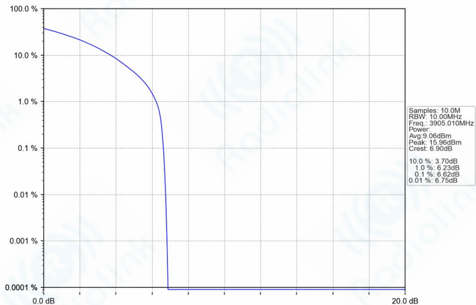
n77h_30kHz_SISO_NTNV_10MHz_CP-OFDM_16_QAM_3905.01MHz_Outer_Full_Ant1
