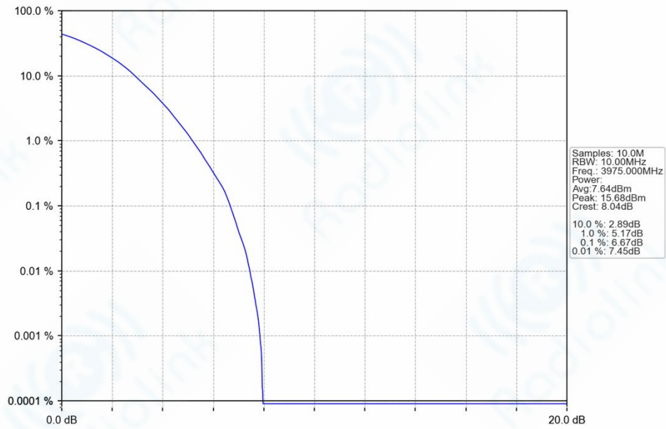
n77h_30kHz_SISO_NTNV_10MHz_DFT-s-OFDM_256_QAM_3975MHz_Outer_Full_Ant1
