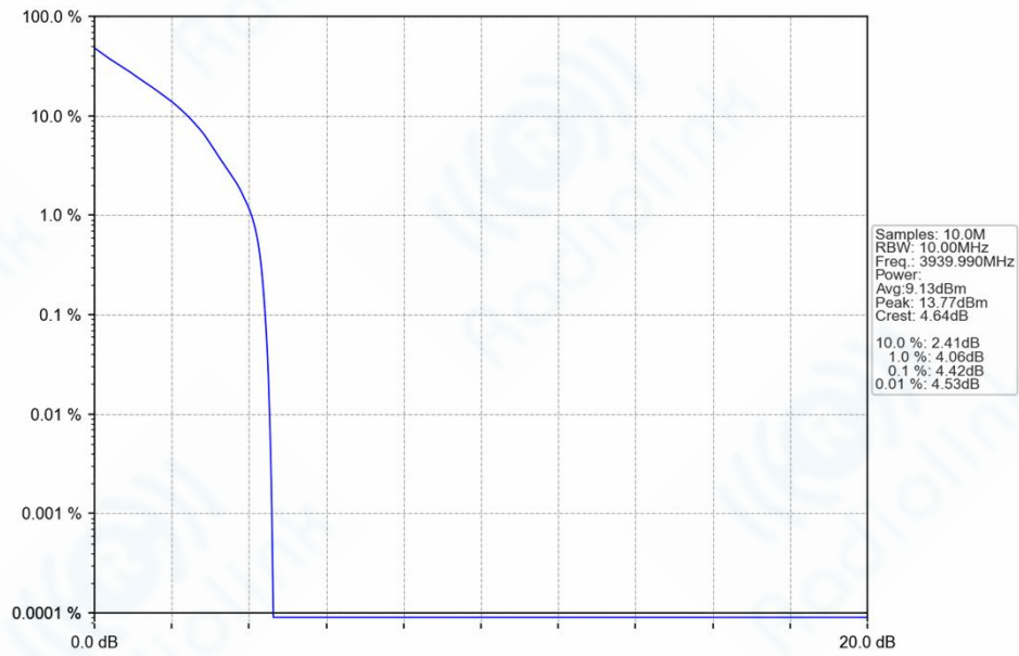
n77h_30kHz_SISO_NTNV_10MHz_DFT-s-OFDM_QPSK_3939.99MHz_Outer_Full_Ant1
