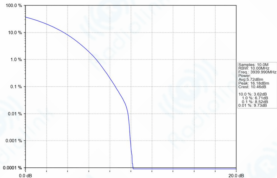
n77h_30kHz_SISO_NTNV_10MHz_CP-OFDM_256_QAM_3939.99MHz_Outer_Full_Ant1
