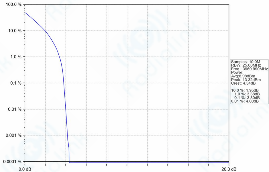
n77h_30kHz_SISO_NTNV_20MHz_DFT-s-OFDM_PI/2_BPSK_3969.99MHz_Outer_Full_Ant1
