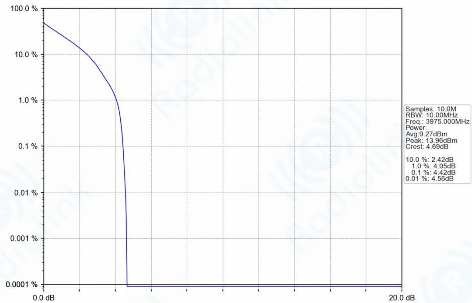
n77h_30kHz_SISO_NTNV_10MHz_DFT-s-OFDM_QPSK_3975MHz_Outer_Full_Ant1
