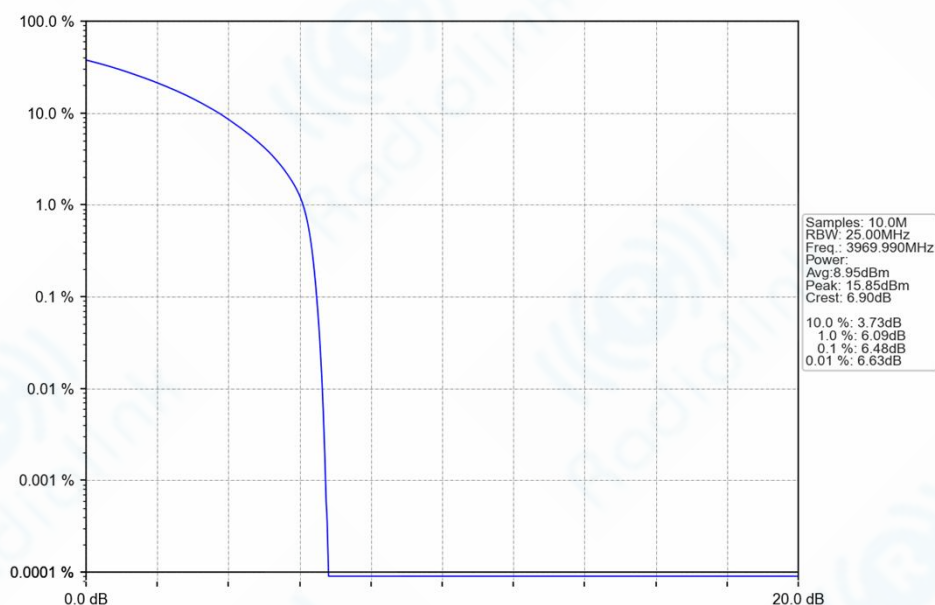
n77h_30kHz_SISO_NTNV_20MHz_CP-OFDM_QPSK_3969.99MHz_Outer_Full_Ant1
