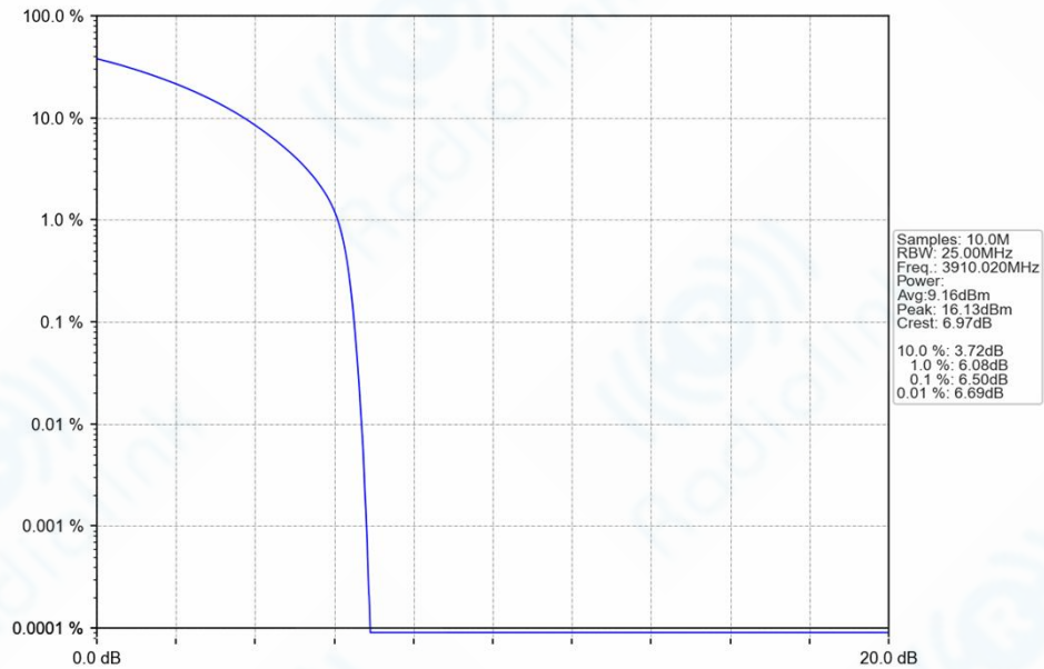
n77h_30kHz_SISO_NTNV_20MHz_CP-OFDM_QPSK_3910.02MHz_Outer_Full_Ant1
