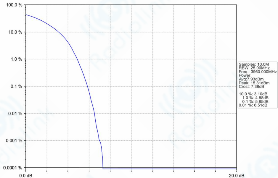
n77h_30kHz_SISO_NTNV_40MHz_DFT-s-OFDM_QPSK_3960MHz_Outer_Full_Ant1
