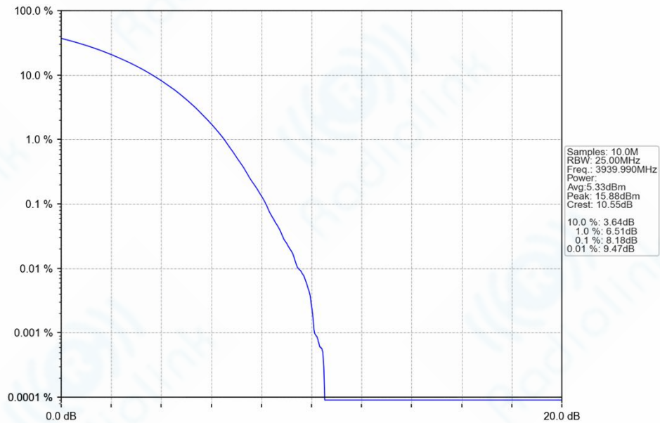
n77h_30kHz_SISO_NTNV_60MHz_CP-OFDM_64_QAM_3939.99MHz_Outer_Full_Ant1
