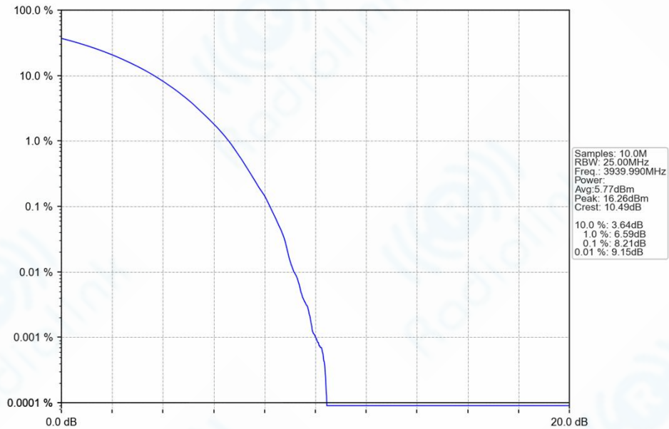
n77h_30kHz_SISO_NTNV_60MHz_CP-OFDM_16_QAM_3939.99MHz_Outer_Full_Ant1
