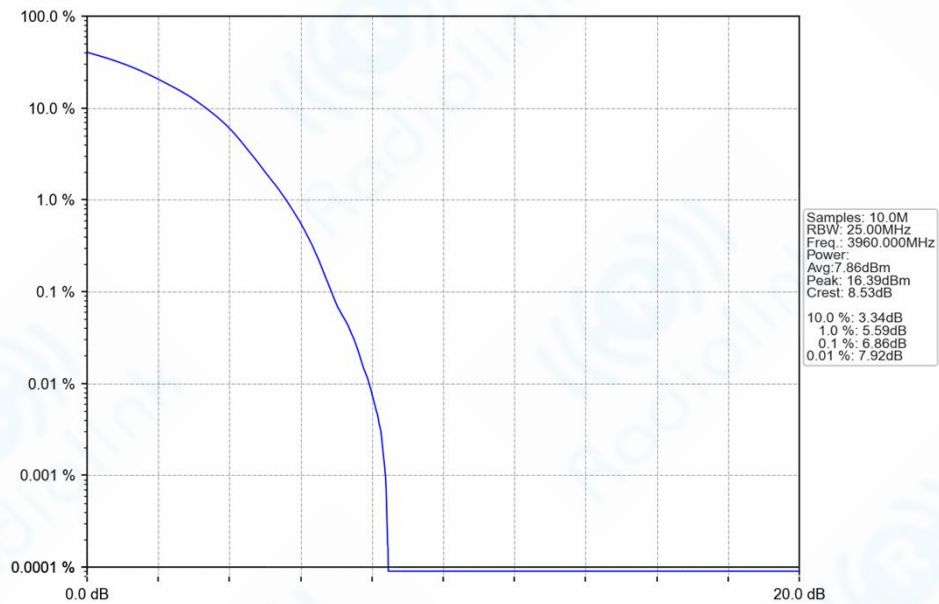
n77h_30kHz_SISO_NTNV_40MHz_DFT-s-OFDM_64_QAM_3960MHz_Outer_Full_Ant1
