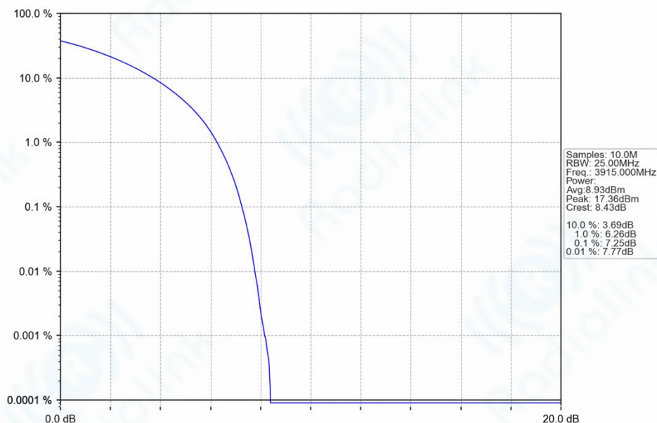
n77h_30kHz_SISO_NTNV_30MHz_CP-OFDM_16_QAM_3915MHz_Outer_Full_Ant1
