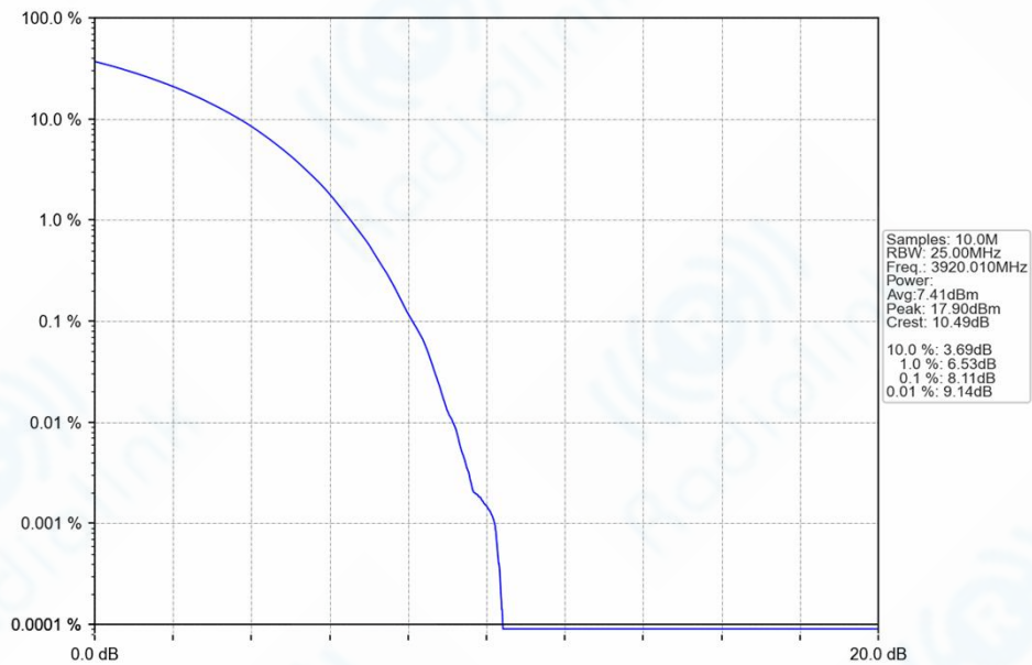
n77h_30kHz_SISO_NTNV_40MHz_CP-OFDM_64_QAM_3920.01MHz_Outer_Full_Ant1
