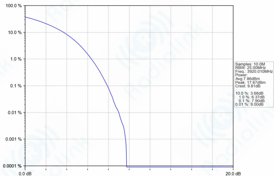
n77h_30kHz_SISO_NTNV_40MHz_CP-OFDM_16_QAM_3920.01MHz_Outer_Full_Ant1
