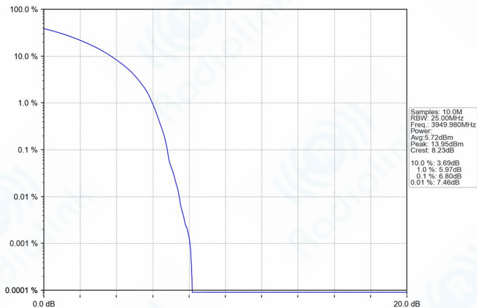
n77h_30kHz_SISO_NTNV_60MHz_DFT-s-OFDM_QPSK_3949.98MHz_Outer_Full_Ant1
