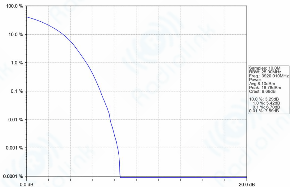
n77h_30kHz_SISO_NTNV_40MHz_DFT-s-OFDM_16_QAM_3920.01MHz_Outer_Full_Ant1
