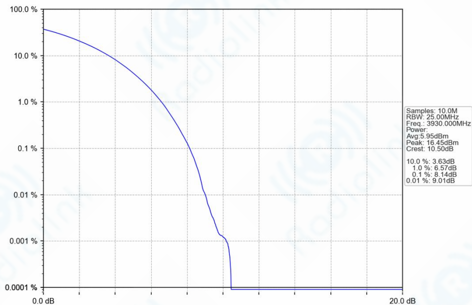
n77h_30kHz_SISO_NTNV_60MHz_CP-OFDM_QPSK_3930MHz_Outer_Full_Ant1
