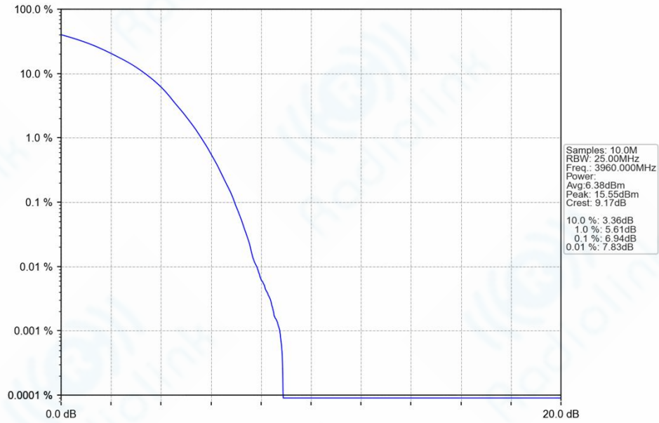
n77h_30kHz_SISO_NTNV_40MHz_DFT-s-OFDM_256_QAM_3960MHz_Outer_Full_Ant1
