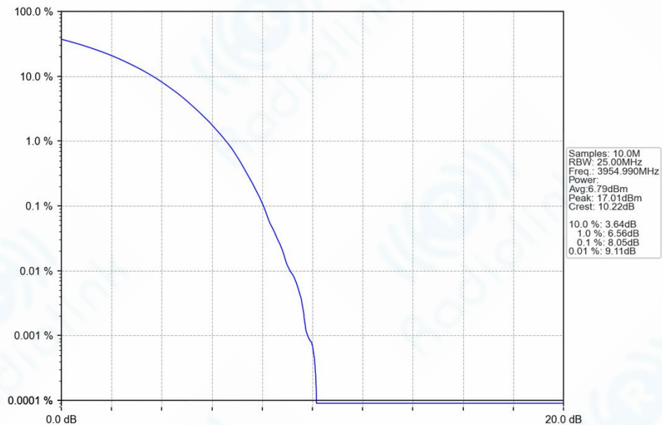
n77h_30kHz_SISO_NTNV_50MHz_CP-OFDM_QPSK_3954.99MHz_Outer_Full_Ant1
