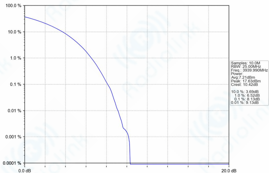
n77h_30kHz_SISO_NTNV_40MHz_CP-OFDM_64_QAM_3939.99MHz_Outer_Full_Ant1
