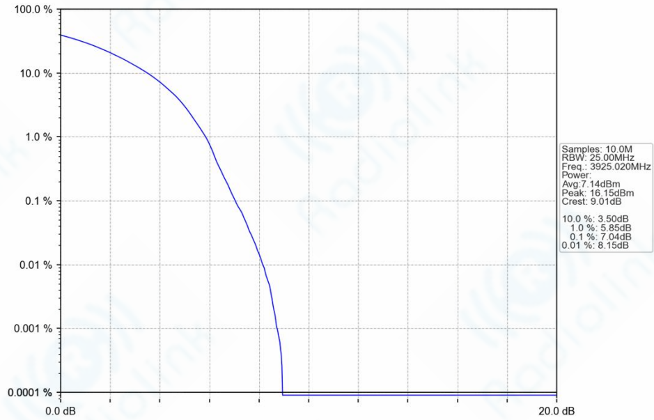
n77h_30kHz_SISO_NTNV_50MHz_DFT-s-OFDM_16_QAM_3925.02MHz_Outer_Full_Ant1
