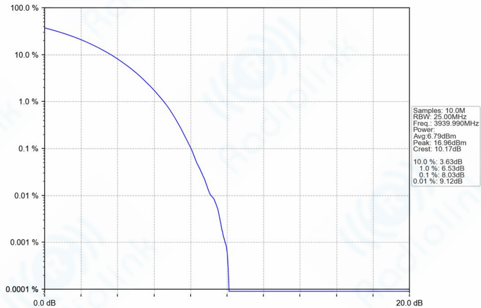
n77h_30kHz_SISO_NTNV_50MHz_CP-OFDM_QPSK_3939.99MHz_Outer_Full_Ant1
