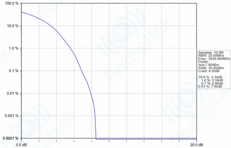
n77h_30kHz_SISO_NTNV_40MHz_DFT-s-OFDM_64_QAM_3939.99MHz_Outer_Full_Ant1
