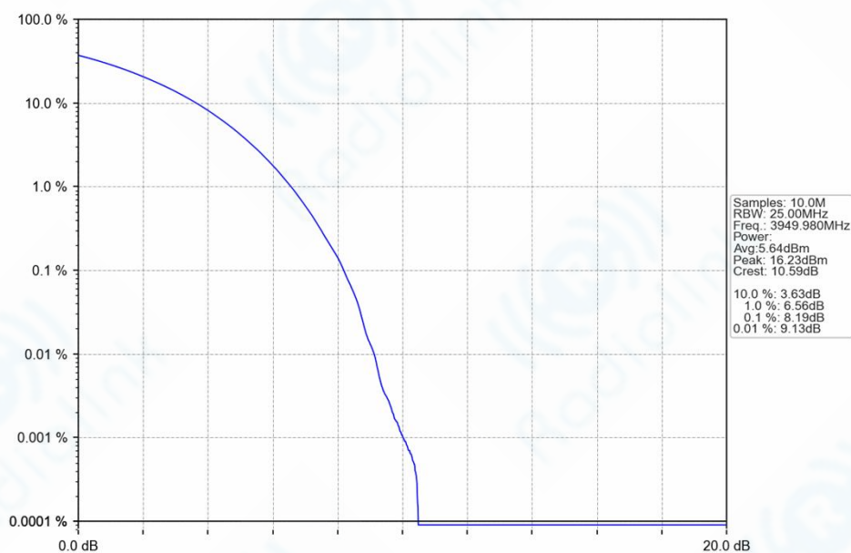
n77h_30kHz_SISO_NTNV_60MHz_CP-OFDM_QPSK_3949.98MHz_Outer_Full_Ant1
