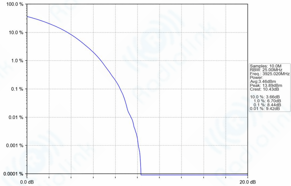
n77h_30kHz_SISO_NTNV_50MHz_CP-OFDM_256_QAM_3925.02MHz_Outer_Full_Ant1
