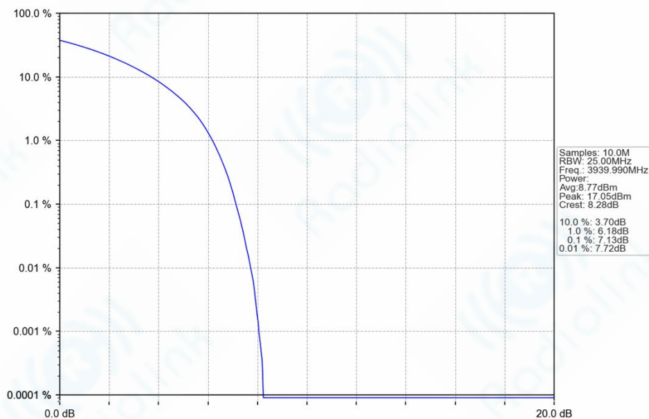
n77h_30kHz_SISO_NTNV_30MHz_CP-OFDM_QPSK_3939.99MHz_Outer_Full_Ant1
