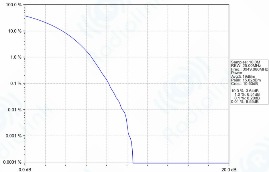
n77h_30kHz_SISO_NTNV_60MHz_CP-OFDM_64_QAM_3949.98MHz_Outer_Full_Ant1
