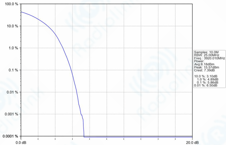
n77h_30kHz_SISO_NTNV_40MHz_DFT-s-OFDM QPSK_3920.01MHz_Outer_Full_Ant1
