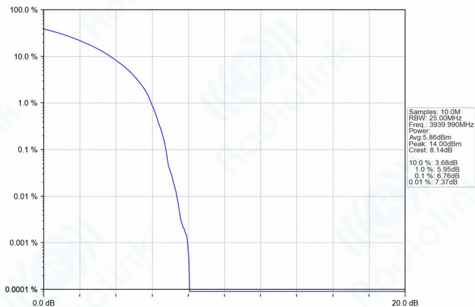
n77h_30kHz_SISO_NTNV_60MHz_DFT-s-OFDM_QPSK_3939.99MHz_Outer_Full_Ant1
