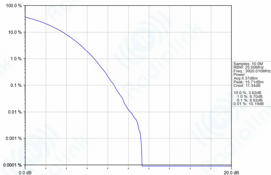
n77h_30kHz_SISO_NTNV_40MHz_CP-OFDM_256_QAM_3920.01MHz_Outer_Full_Ant1
