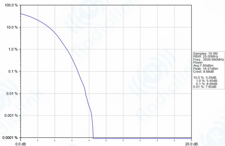
n77h_30kHz_SISO_NTNV_40MHz_DFT-s-OFDM_16_QAM_3939.99MHz_Outer_Full_Ant1
