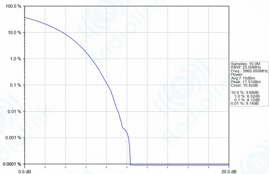
n77h_30kHz_SISO_NTNV_40MHz_CP-OFDM_64_QAM_3960MHz_Outer_Full_Ant1
