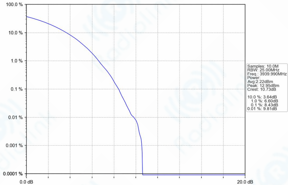
n77h_30kHz_SISO_NTNV_60MHz_CP-OFDM_256_QAM_3939.99MHz_Outer_Full_Ant1
