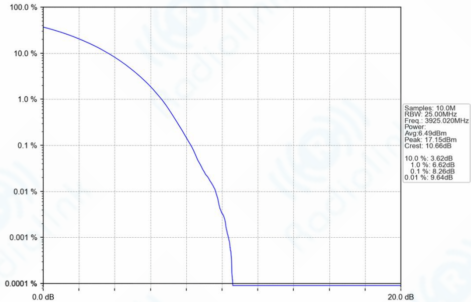
n77h_30kHz_SISO_NTNV_50MHz_CP-OFDM_64_QAM_3925.02MHz_Outer_Full_Ant1
