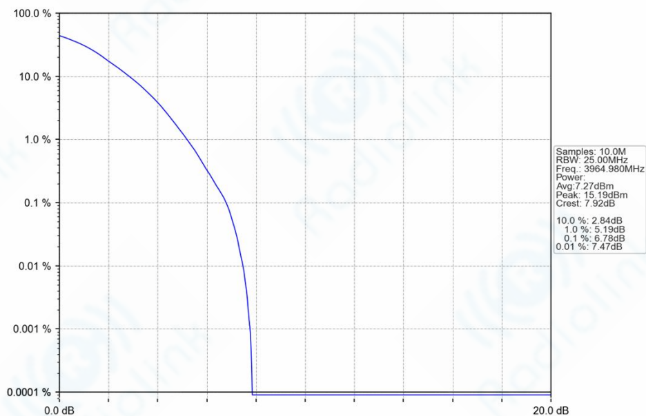
n77h_30kHz_SISO_NTNV_30MHz_DFT-s-OFDM_256_QAM_3964.98MHz_Outer_Full_Ant1
