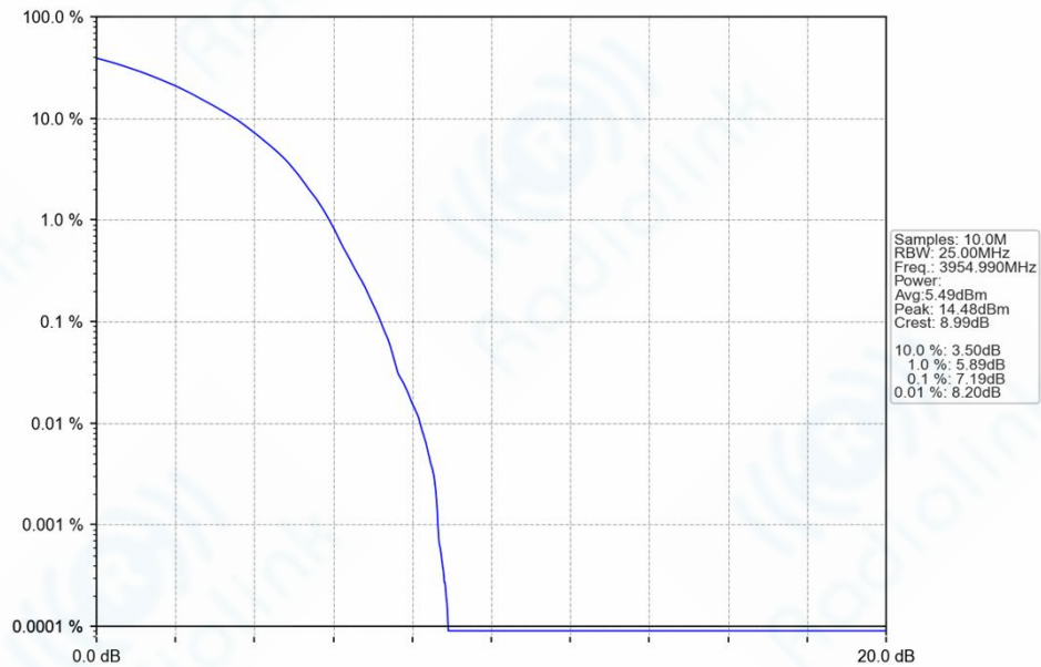
n77h_30kHz_SISO_NTNV_50MHz_DFT-s-OFDM_256_QAM_3954.99MHz_Outer_Full_Ant1
