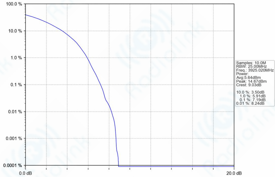
n77h_30kHz_SISO_NTNV_50MHz_DFT-s-OFDM_256_QAM_3925.02MHz_Outer_Full_Ant1
