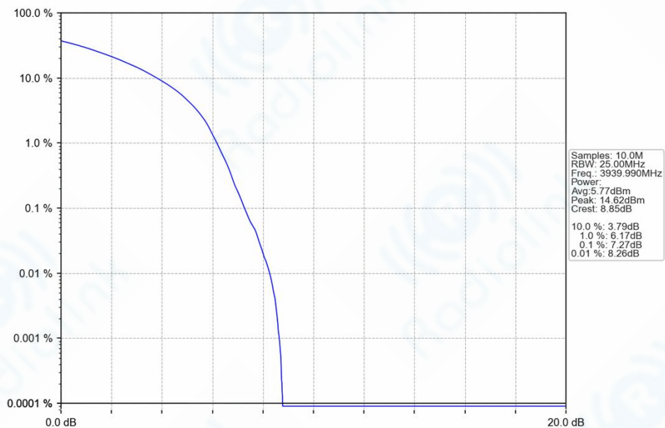
n77h_30kHz_SISO_NTNV_60MHz_DFT-s-OFDM_16_QAM_3939.99MHz_Outer_Full_Ant1
