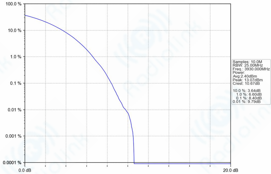
n77h_30kHz_SISO_NTNV_60MHz_CP-OFDM_256_QAM_3930MHz_Outer_Full_Ant1
