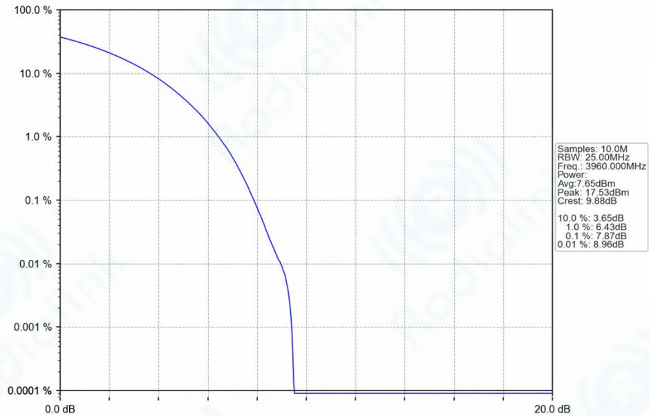
n77h_30kHz_SISO_NTNV_40MHz_CP-OFDM_QPSK_3960MHz_Outer_Full_Ant1
