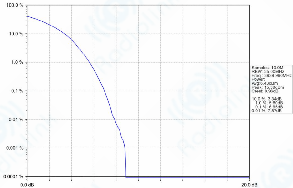
n77h_30kHz_SISO_NTNV_40MHz_DFT-s-OFDM_256_QAM_3939.99MHz_Outer_Full_Ant1
