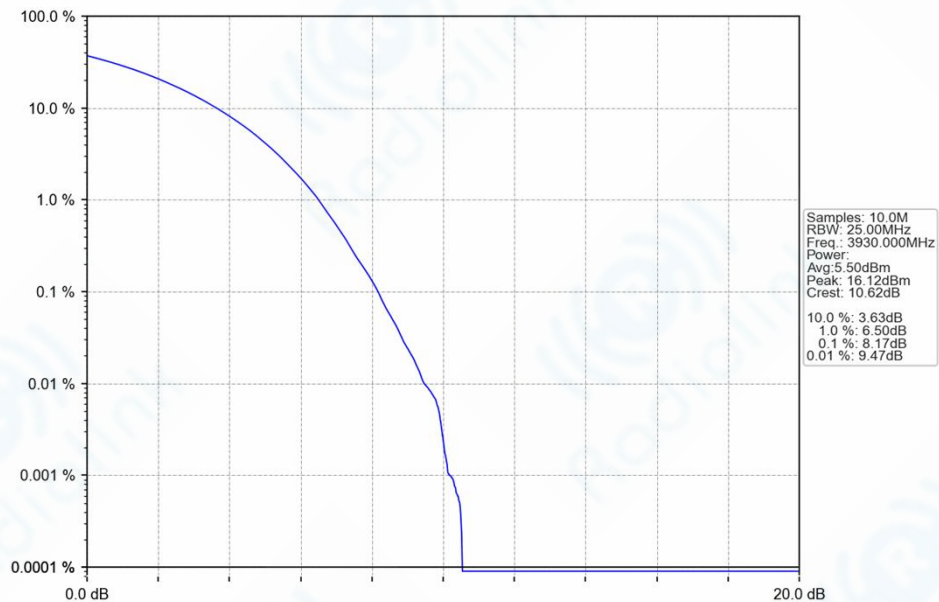
n77h_30kHz_SISO_NTNV_60MHz_CP-OFDM_64_QAM_3930MHz_Outer_Full_Ant1
