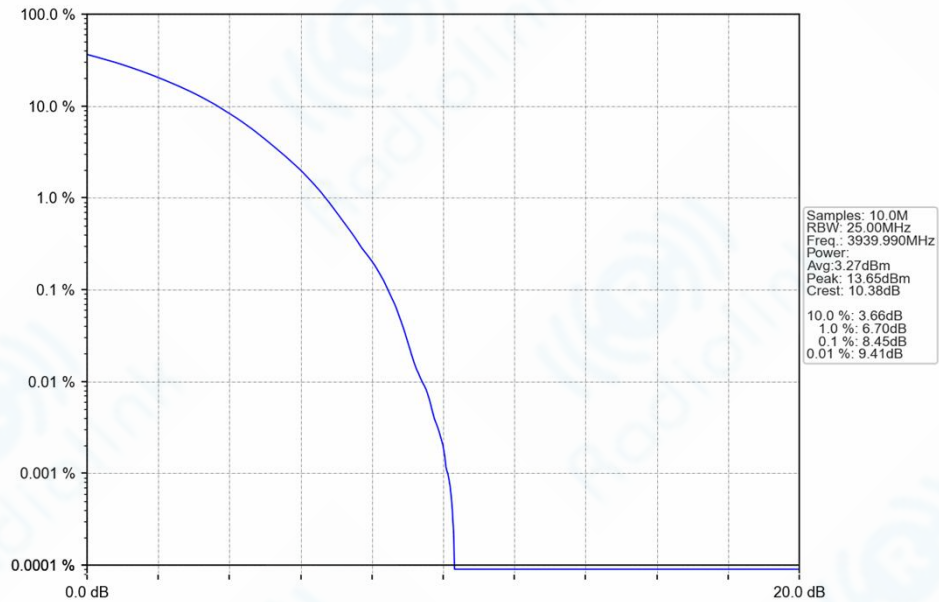
n77h_30kHz_SISO_NTNV_50MHz_CP-OFDM_256_QAM_3939.99MHz_Outer_Full_Ant1
