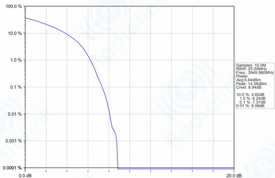
n77h_30kHz_SISO_NTNV_60MHz_DFT-s-OFDM_64_QAM_3949.98MHz_Outer_Full_Ant1
