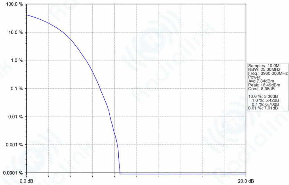
n77h_30kHz_SISO_NTNV_40MHz_DFT-s-OFDM_16_QAM_3960MHz_Outer_Full_Ant1
