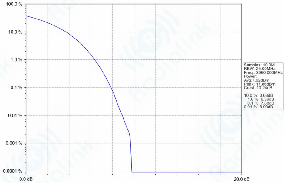
n77h_30kHz_SISO_NTNV_40MHz_CP-OFDM_16_QAM_3960MHz_Outer_Full_Ant1
