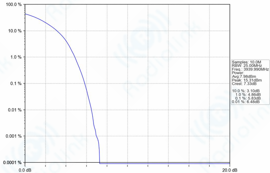
n77h_30kHz_SISO_NTNV_40MHz_DFT-s-OFDM_QPSK_3939.99MHz_Outer_Full_Ant1
