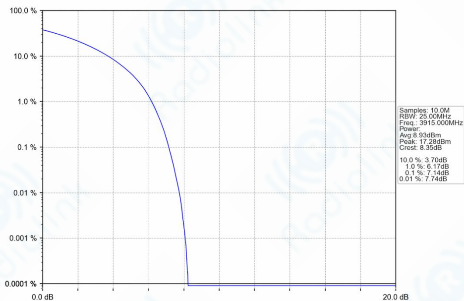
n77h_30kHz_SISO_NTNV_30MHz_CP-OFDM_QPSK_3915MHz_Outer_Full_Ant1
