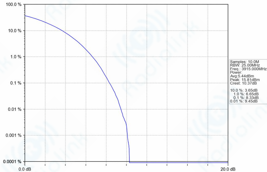
n77h_30kHz_SISO_NTNV_30MHz_CP-OFDM_256_QAM_3915MHz_Outer_Full_Ant1
