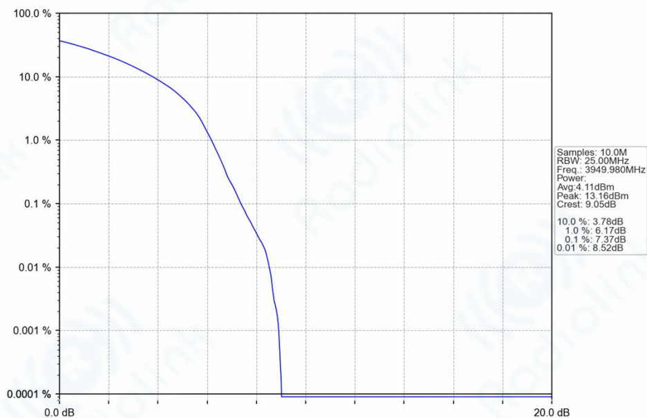
n77h_30kHz_SISO_NTNV_60MHz_DFT-s-OFDM_256_QAM_3949.98MHz_Outer_Full_Ant1
