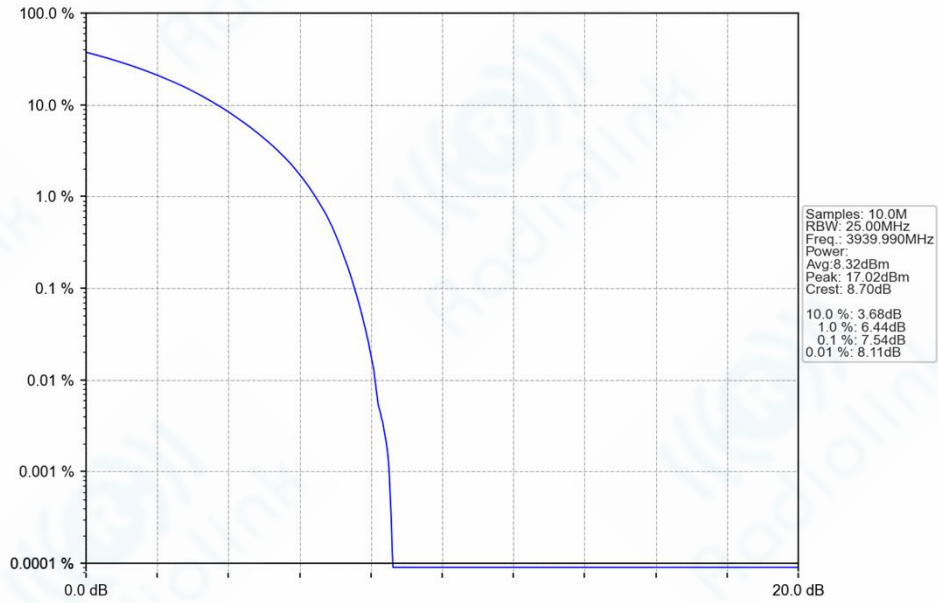
n77h_30kHz_SISO_NTNV_30MHz_CP-OFDM_64_QAM_3939.99MHz_Outer_Full_Ant1
