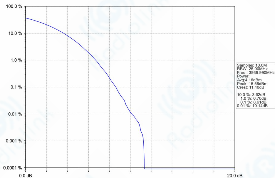
n77h_30kHz_SISO_NTNV_40MHz_CP-OFDM_256_QAM_3939.99MHz_Outer_Full_Ant1
