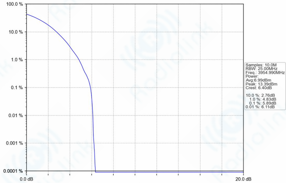
n77h_30kHz_SISO_NTNV_50MHz_DFT-s-OFDM_PI/2_BPSK_3954.99MHz_Outer_Full_Ant1
