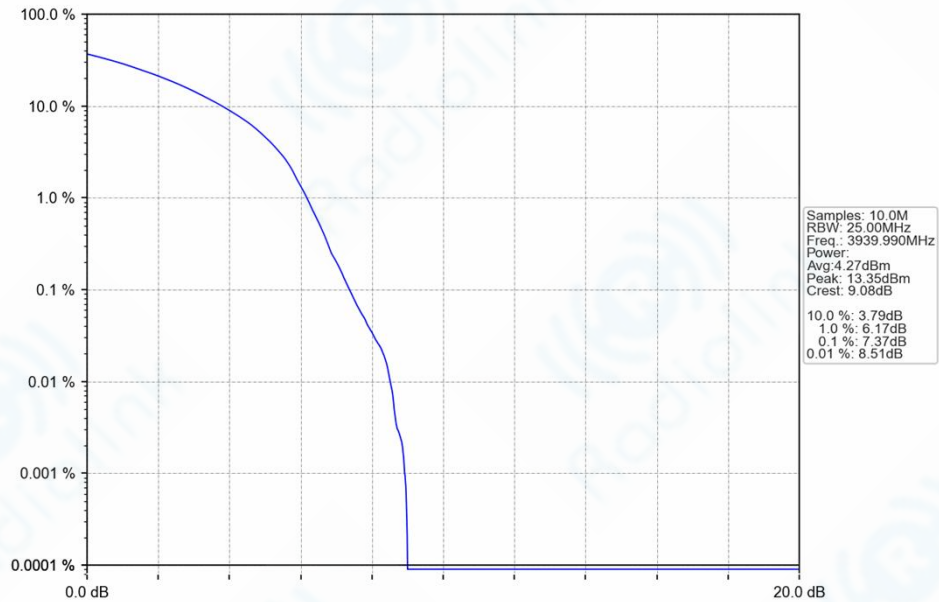
n77h_30kHz_SISO_NTNV_60MHz_DFT-s-OFDM_256_QAM_3939.99MHz_Outer_Full_Ant1
