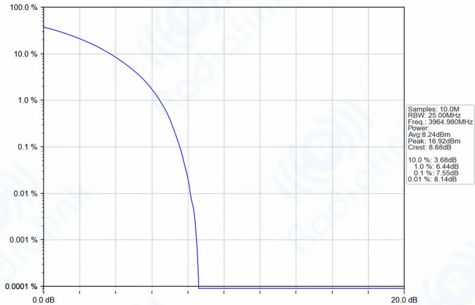
n77h_30kHz_SISO_NTNV_30MHz_CP-OFDM_64_QAM_3964.98MHz_Outer_Full_Ant1
