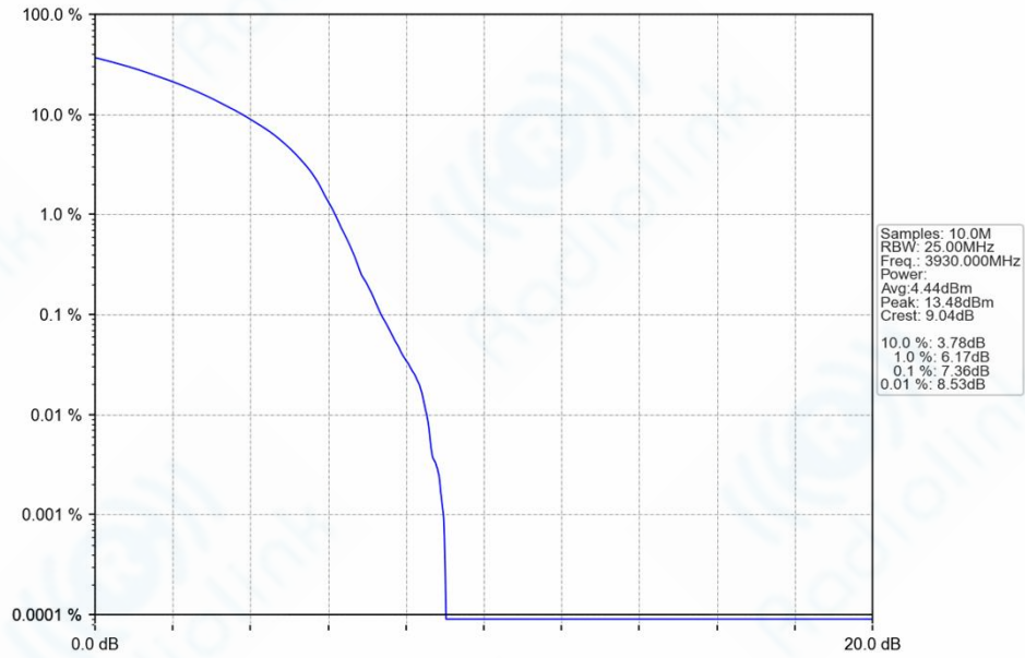
n77h_30kHz_SISO_NTNV_60MHz_DFT-s-OFDM_256_QAM_3930MHz_Outer_Full_Ant1
