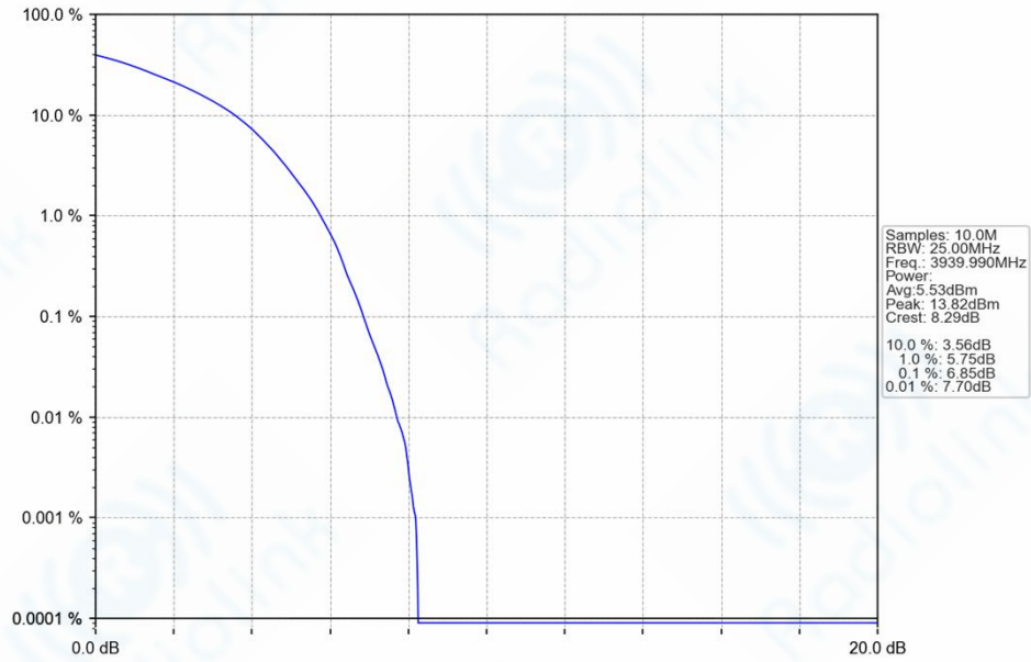
n77h_30kHz_SISO_NTNV_70MHz_DFT-s-OFDM_QPSK_3939.99MHz_Outer_Full_Ant1
