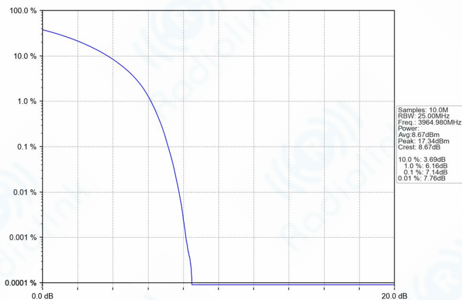
n77h_30kHz_SISO_NTNV_30MHz_CP-OFDM_QPSK_3964.98MHz_Outer_Full_Ant1
