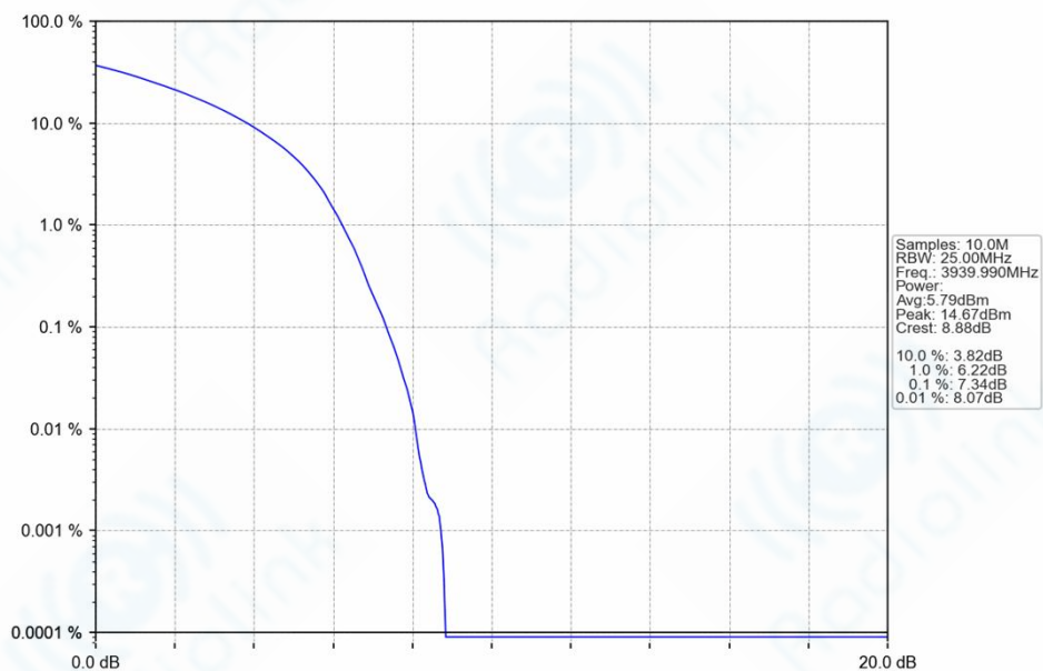
n77h_30kHz_SISO_NTNV_60MHz_DFT-s-OFDM_64_QAM_3939.99MHz_Outer_Full_Ant1
