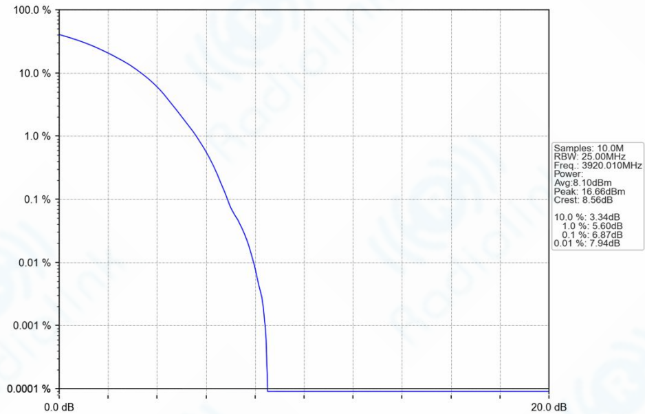
n77h_30kHz_SISO_NTNV_40MHz_DFT-s-OFDM_64_QAM_3920.01MHz_Outer_Full_Ant1
