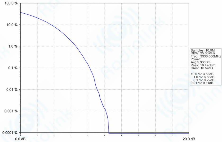
n77h_30kHz_SISO_NTNV_60MHz_CP-OFDM_16_QAM_3930MHz_Outer_Full_Ant1
