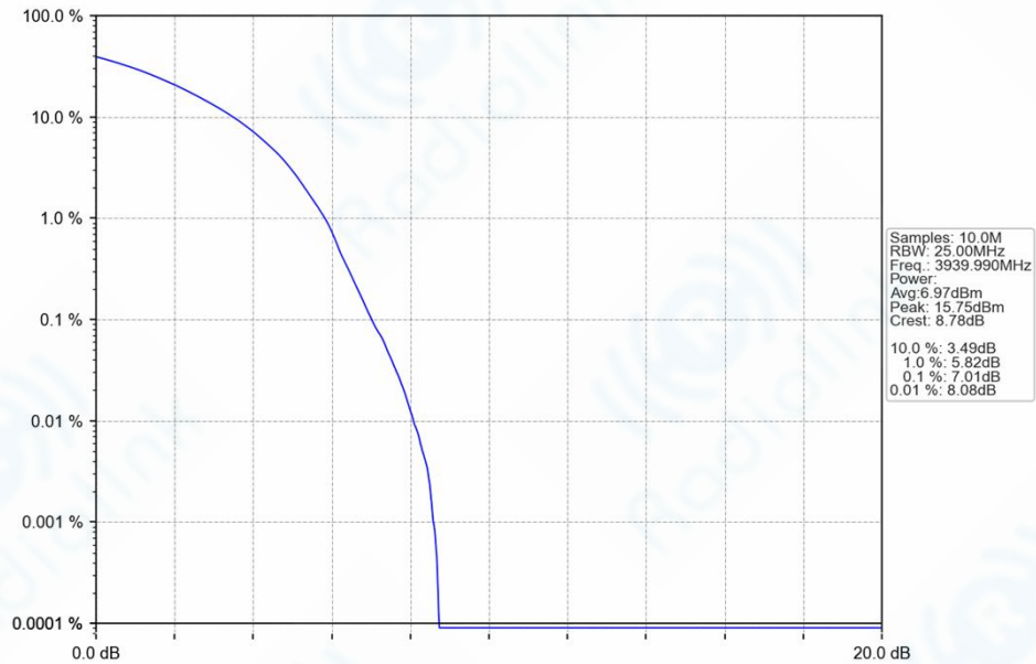
n77h_30kHz_SISO_NTNV_50MHz_DFT-s-OFDM_16_QAM_3939.99MHz_Outer_Full_Ant1
