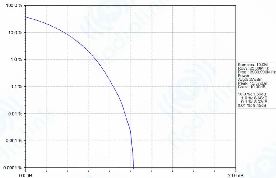
n77h_30kHz_SISO_NTNV_30MHz_CP-OFDM_256_QAM_3939.99MHz_Outer_Full_Ant1
