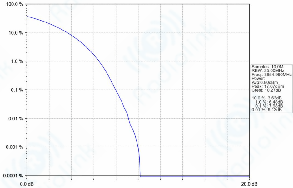
n77h_30kHz_SISO_NTNV_50MHz_CP-OFDM_16_QAM_3954.99MHz_Outer_Full_Ant1
