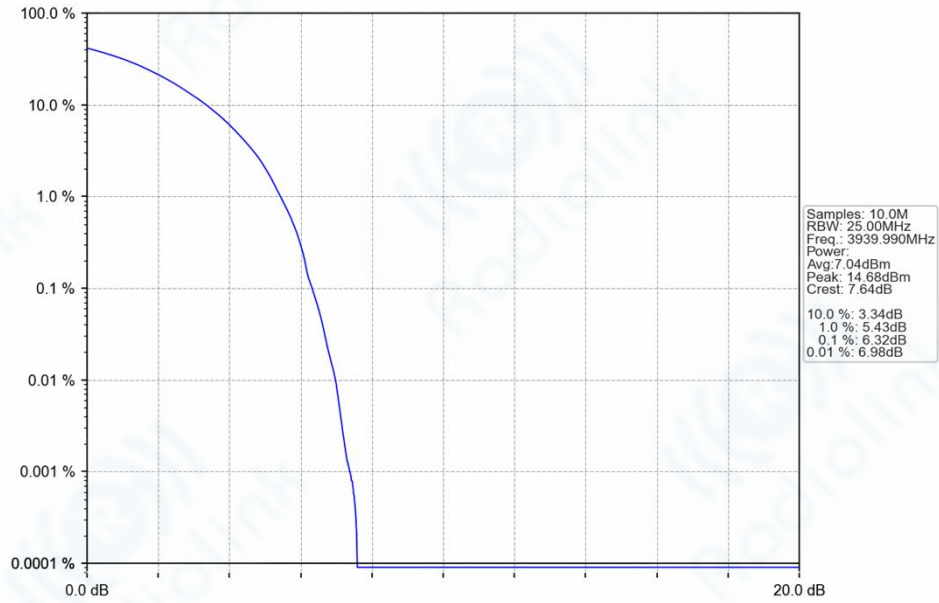
n77h_30kHz_SISO_NTNV_50MHz_DFT-s-OFDM_QPSK_3939.99MHz_Outer_Full_Ant1
