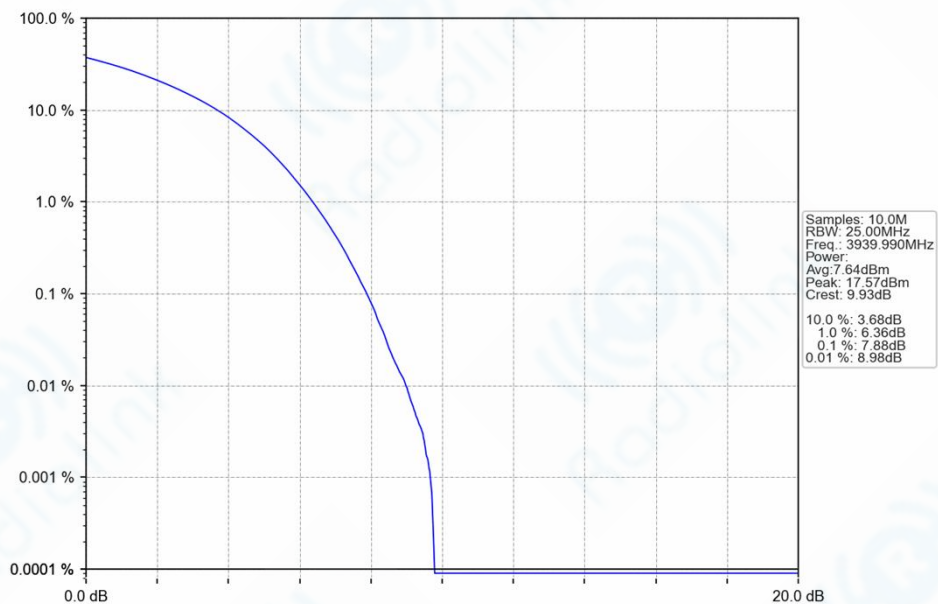
n77h_30kHz_SISO_NTNV_40MHz_CP-OFDM_16_QAM_3939.99MHz_Outer_Full_Ant1
