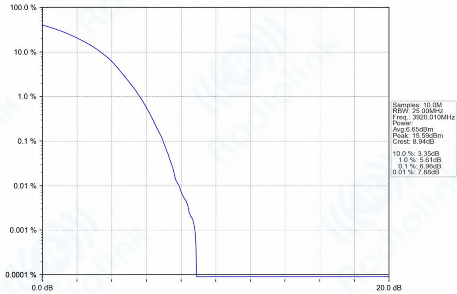
n77h_30kHz_SISO_NTNV_40MHz_DFT-s-OFDM_256_QAM_3920.01MHz_Outer_Full_Ant1
