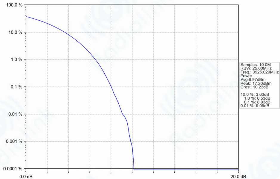
n77h_30kHz_SISO_NTNV_50MHz_CP-OFDM_QPSK_3925.02MHz_Outer_Full_Ant1
