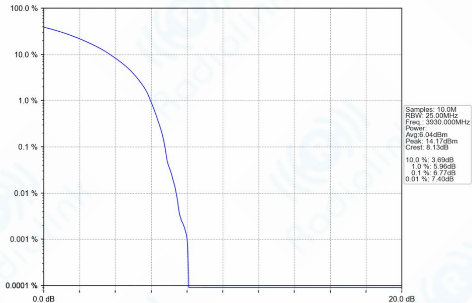
n77h_30kHz_SISO_NTNV_60MHz_DFT-s-OFDM QPSK_3930MHz_Outer_Full_Ant1
