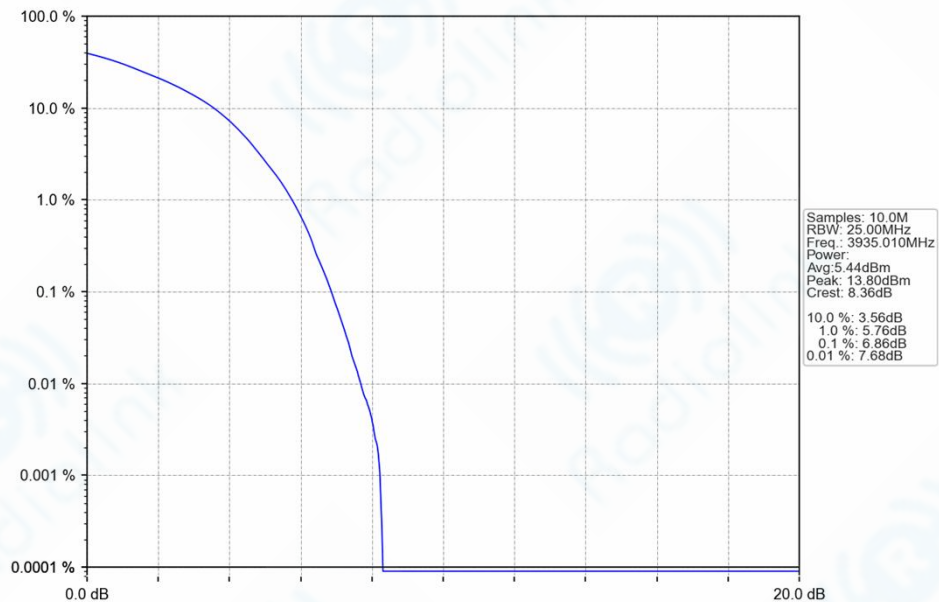
n77h_30kHz_SISO_NTNV_70MHz_DFT-s-OFDM QPSK_3935.01MHz_Outer_Full_Ant1
