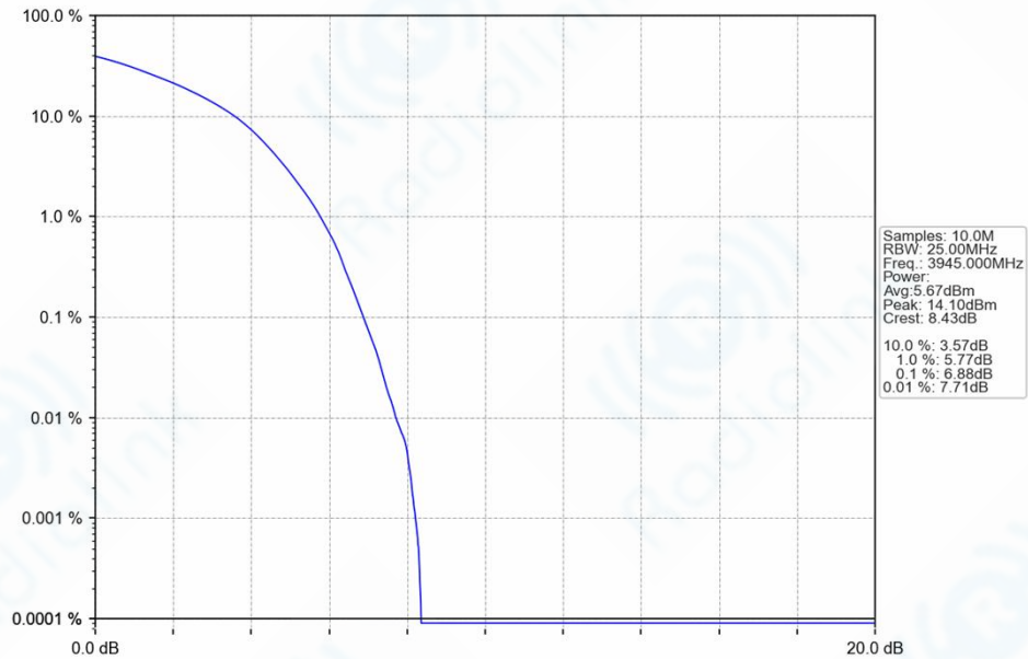
n77h_30kHz_SISO_NTNV_70MHz_DFT-s-OFDM_QPSK_3945MHz_Outer_Full_Ant1
