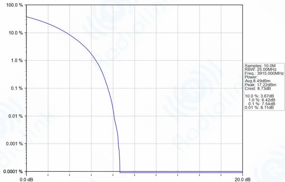
n77h_30kHz_SISO_NTNV_30MHz_CP-OFDM_64_QAM_3915MHz_Outer_Full_Ant1
