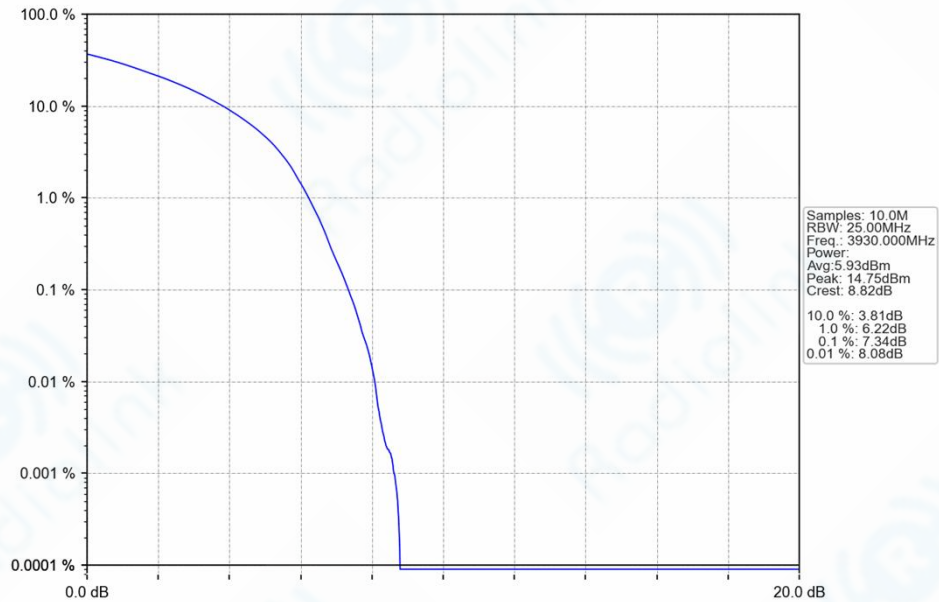
n77h_30kHz_SISO_NTNV_60MHz_DFT-s-OFDM_64_QAM_3930MHz_Outer_Full_Ant1
