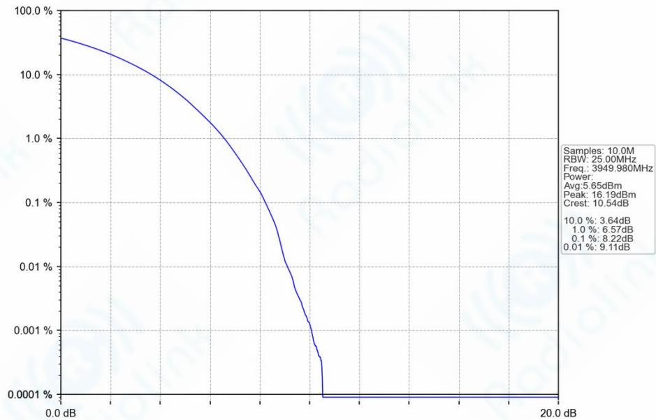
n77h_30kHz_SISO_NTNV_60MHz_CP-OFDM_16_QAM_3949.98MHz_Outer_Full_Ant1
