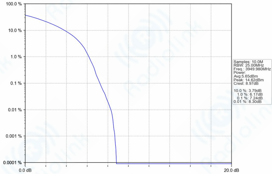
n77h_30kHz_SISO_NTNV_60MHz_DFT-s-OFDM_16_QAM_3949.98MHz_Outer_Full_Ant1
