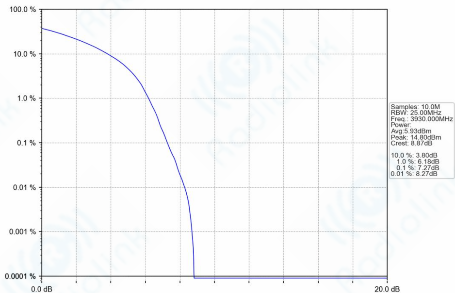
n77h_30kHz_SISO_NTNV_60MHz_DFT-s-OFDM_16_QAM_3930MHz_Outer_Full_Ant1
