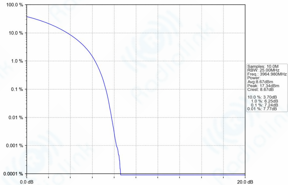
n77h_30kHz_SISO_NTNV_30MHz_CP-OFDM_16_QAM_3964.98MHz_Outer_Full_Ant1
