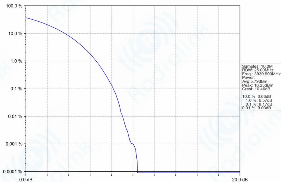
n77h_30kHz_SISO_NTNV_60MHz_CP-OFDM_QPSK_3939.99MHz_Outer_Full_Ant1
