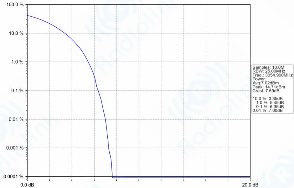
n77h_30kHz_SISO_NTNV_50MHz_DFT-s-OFDM_QPSK_3954.99MHz_Outer_Full_Ant1
