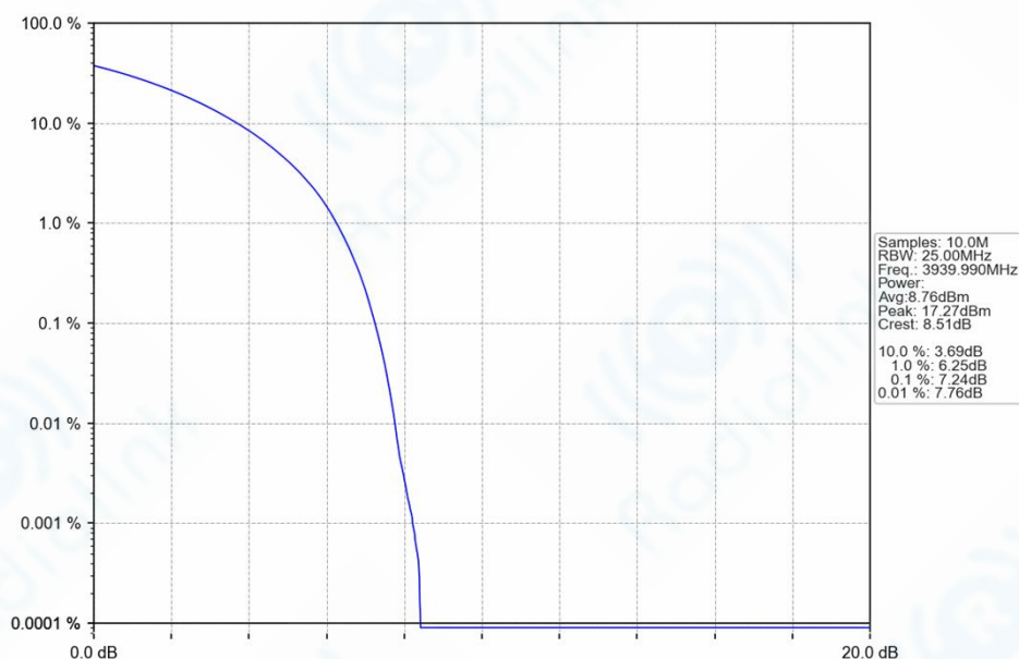
n77h_30kHz_SISO_NTNV_30MHz_CP-OFDM_16_QAM_3939.99MHz_Outer_Full_Ant1
