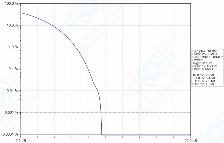
n77h_30kHz_SISO_NTNV_40MHz_CP-OFDM_QPSK_3920.01MHz_Outer_Full_Ant1
