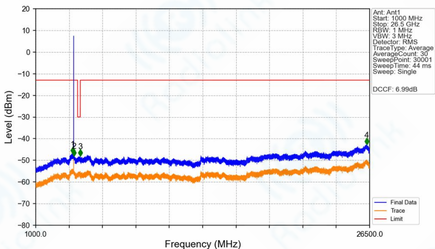
n77h_30kHz_SISO_NTNV_10MHz_DFT-s-OFDM_QPSK_3905.01MHz_Edge_1RB_Left_Ant1
