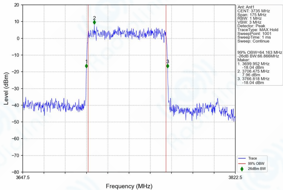
n78a_30kHz_SISO_NTNV_70MHz_DFT-s-OFDM QPSK_3735MHz_Outer_Full_Ant1
