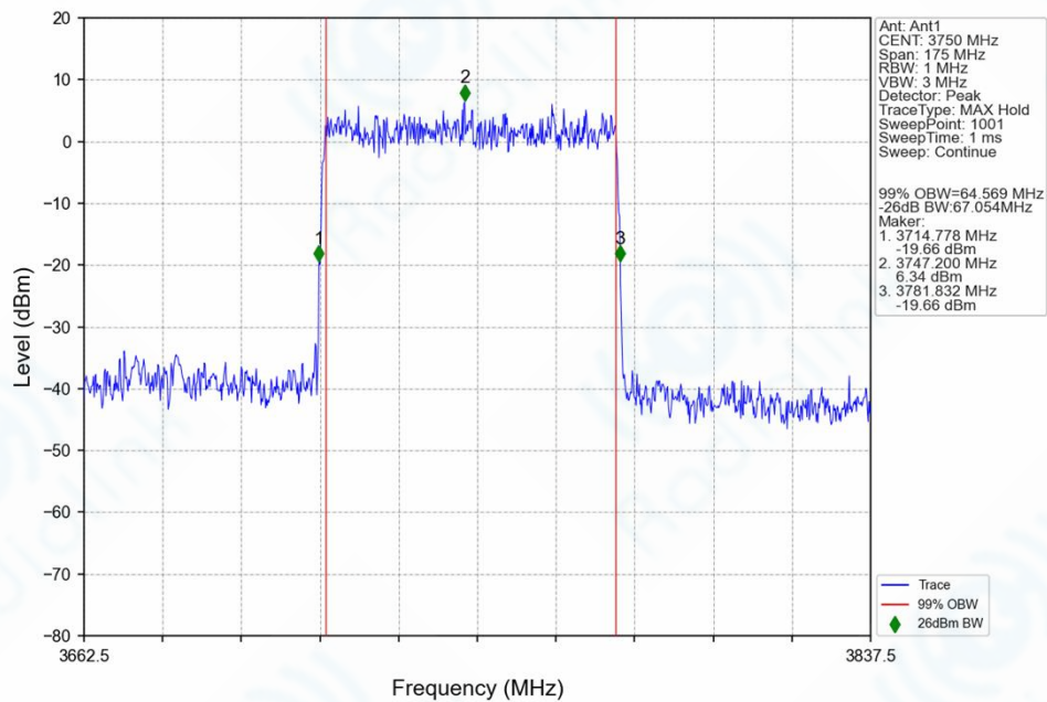
n78a_30kHz_SISO_NTNV_70MHz_DFT-s-OFDM_256_QAM_3750MHz_Outer_Full_Ant1
