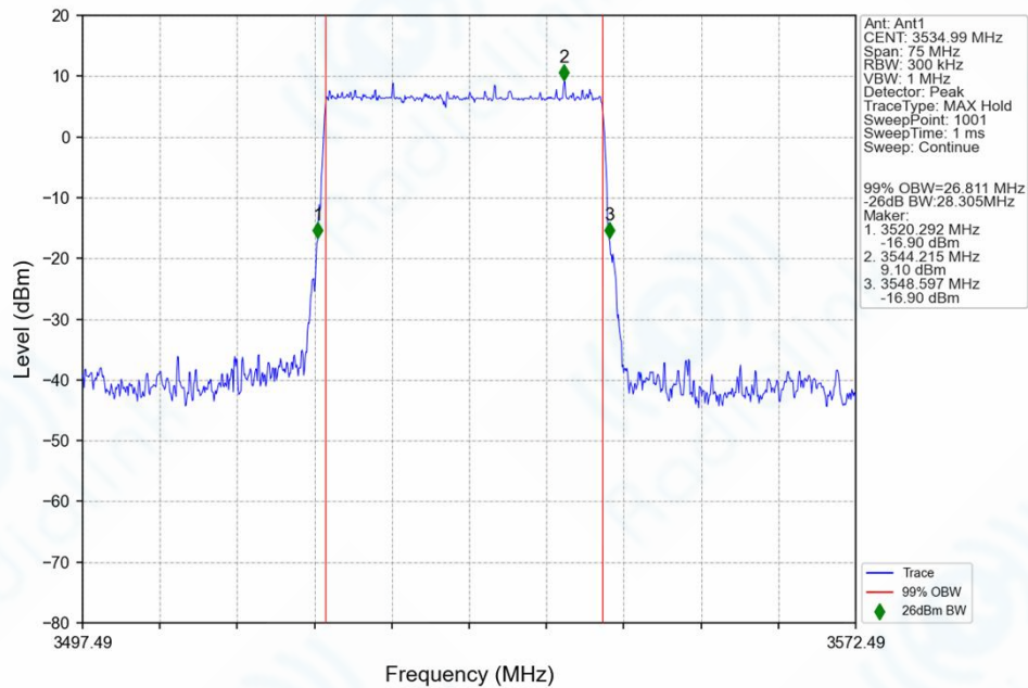
n78e_30kHz_SISO_NTNV_30MHz_DFT-s-OFDM_QPSK_3534.99MHz_Outer_Full_Ant1
