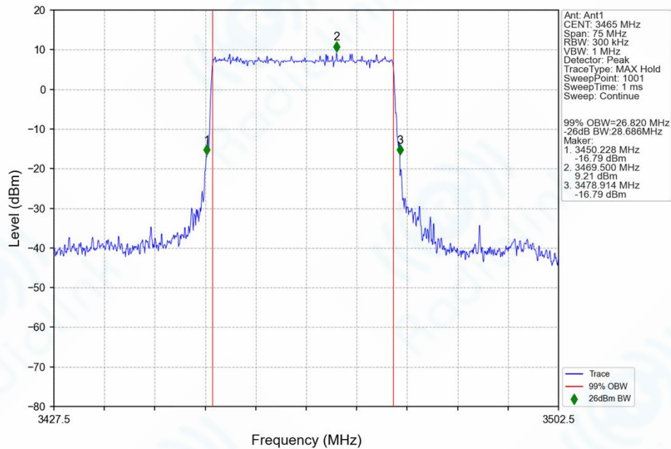
n78e_30kHz_SISO_NTNV_30MHz_DFT-s-OFDM_64_QAM_3465MHz_Outer_Full_Ant1
