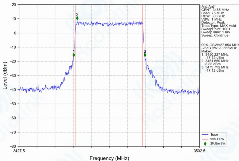
n78e_30kHz_SISO_NTNV_30MHz_CP-OFDM_QPSK_3465MHz_Outer_Full_Ant1
