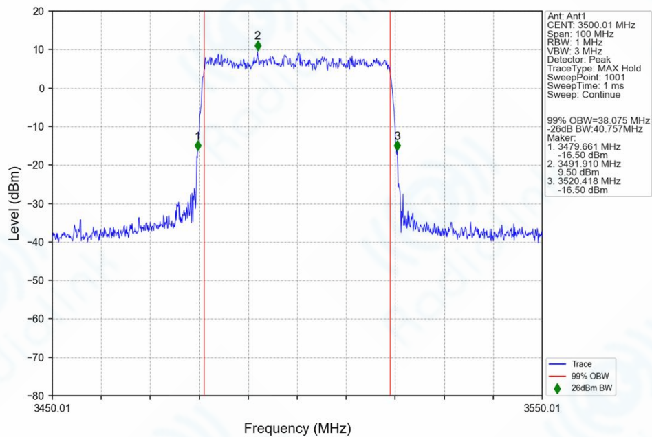
n78e_30kHz_SISO_NTNV_40MHz_CP-OFDM_256_QAM_3500.01MHz_Outer_Full_Ant1
