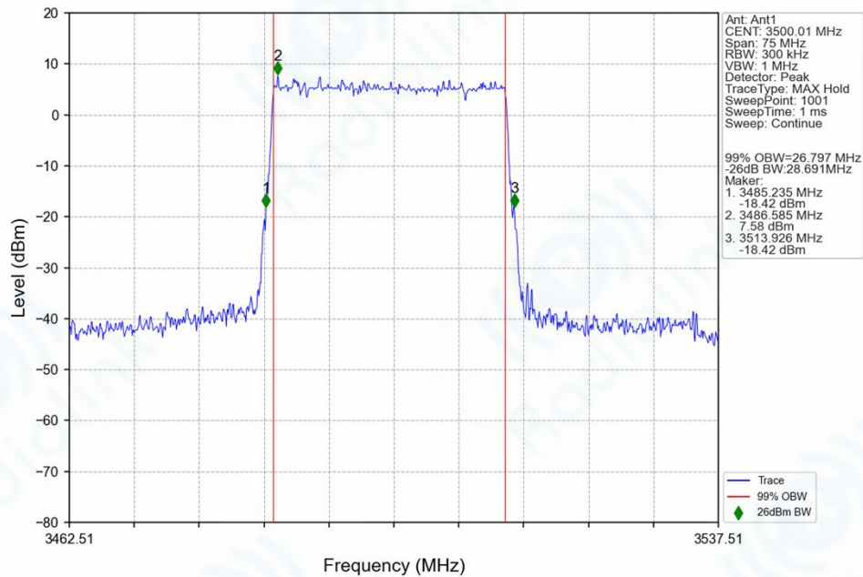
n78e_30kHz_SISO_NTNV_30MHz_DFT-s-OFDM_256_QAM_3500.01MHz_Outer_Full_Ant1
