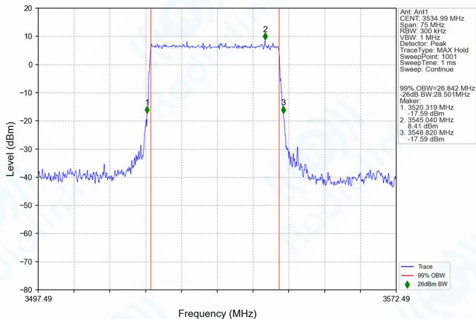
n78e_30kHz_SISO_NTNV_30MHz_DFT-s-OFDM_64_QAM_3534.99MHz_Outer_Full_Ant1
