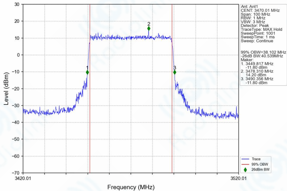
n78e_30kHz_SISO_NTNV_40MHz_CP-OFDM_64_QAM_3470.01MHz_Outer_Full_Ant1
