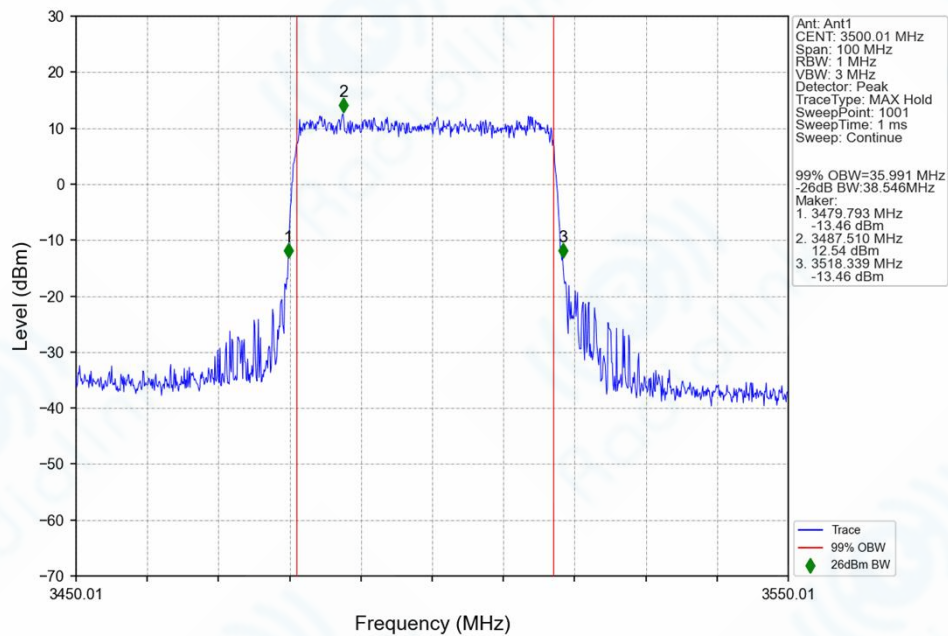
n78e_30kHz_SISO_NTNV_40MHz_DFT-s-OFDM_16_QAM_3500.01MHz_Outer_Full_Ant1
