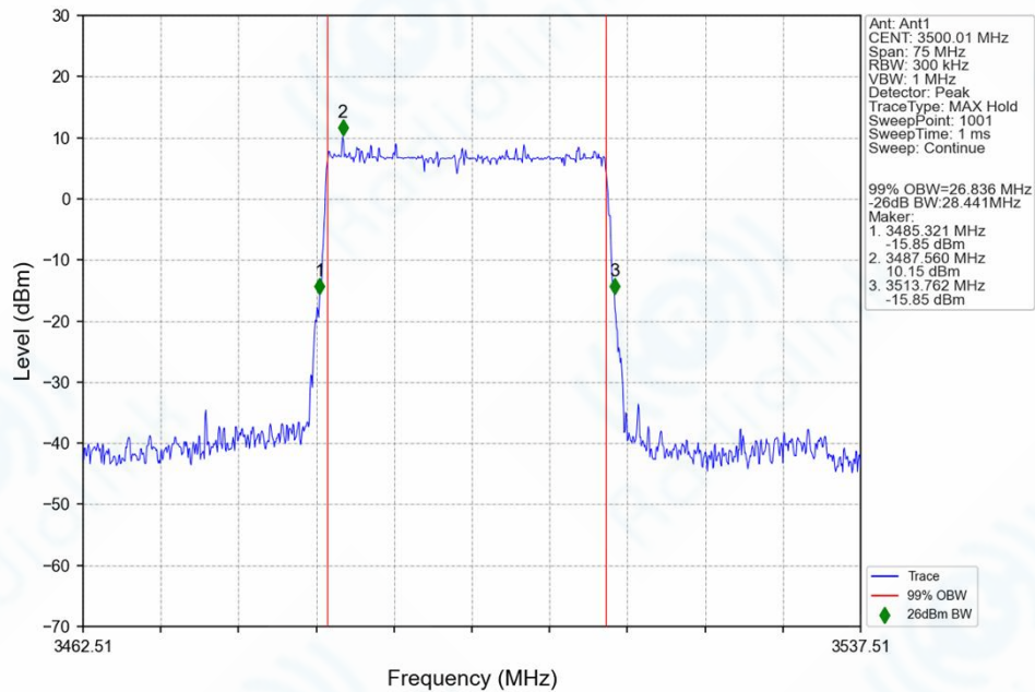
n78e_30kHz_SISO_NTNV_30MHz_DFT-s-OFDM_16_QAM_3500.01MHz_Outer_Full_Ant1
