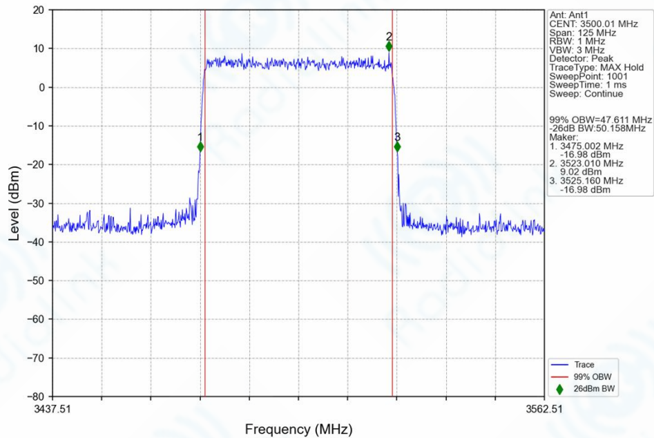
n78e_30kHz_SISO_NTNV_50MHz_CP-OFDM_256_QAM_3500.01MHz_Outer_Full_Ant1
