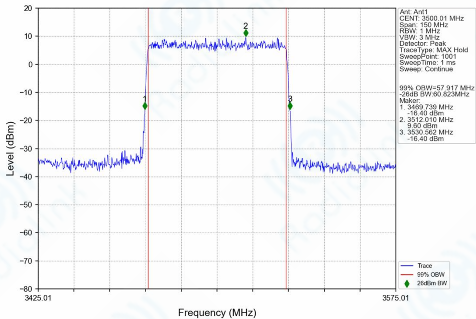
n78e_30kHz_SISO_NTNV_60MHz_DFT-s-OFDM_256_QAM_3500.01MHz_Outer_Full_Ant1
