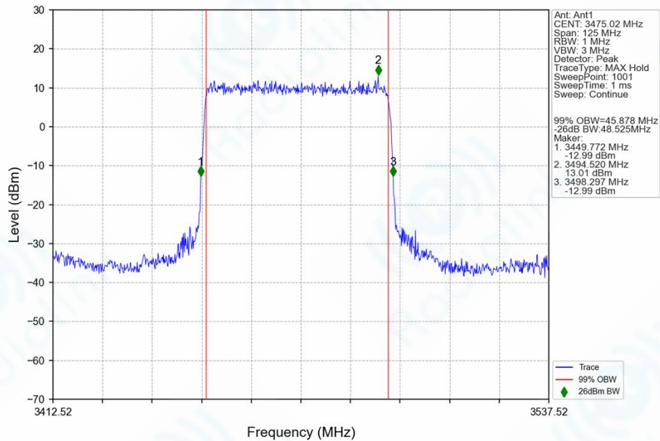
n78e_30kHz_SISO_NTNV_50MHz_DFT-s-OFDM QPSK_3475.02MHz_Outer_Full_Ant1
