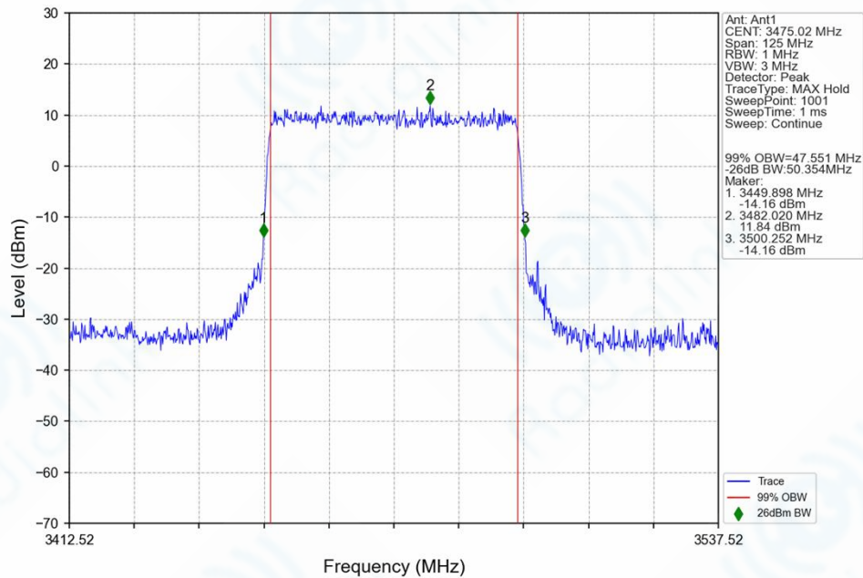
n78e_30kHz_SISO_NTNV_50MHz_CP-OFDM_64 QAM_3475.02MHz_Outer_Full_Ant1
