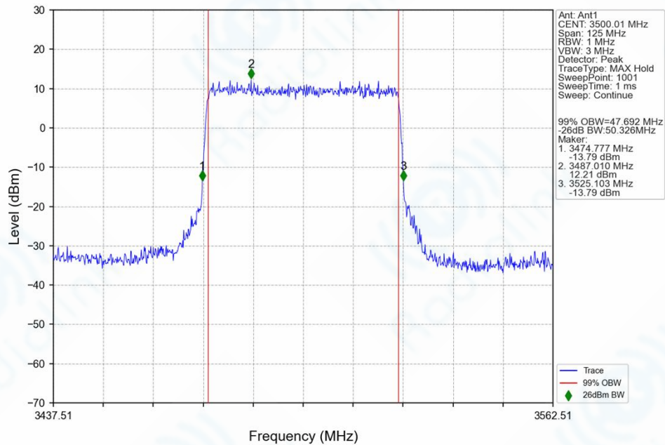
n78e_30kHz_SISO_NTNV_50MHz_CP-OFDM_16_QAM_3500.01MHz_Outer_Full_Ant1
