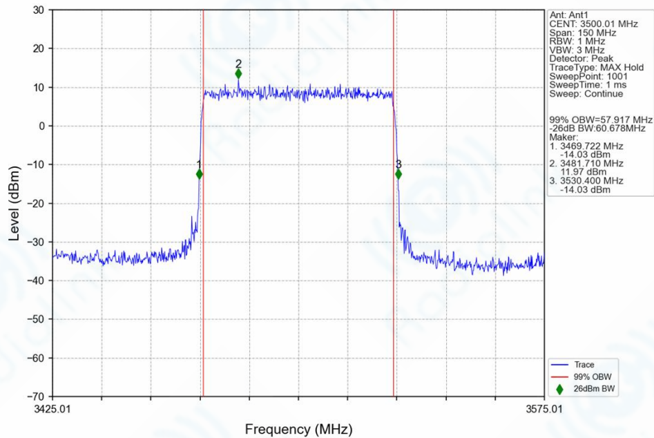
n78e_30kHz_SISO_NTNV_60MHz_DFT-s-OFDM_16_QAM_3500.01MHz_Outer_Full_Ant1
