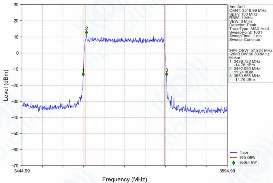
n78e_30kHz_SISO_NTNV_60MHz_DFT-s-OFDM_64_QAM_3519.99MHz_Outer_Full_Ant1
