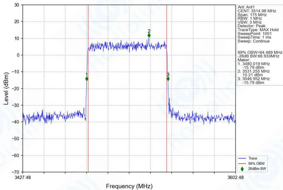
n78e_30kHz_SISO_NTNV_70MHz_DFT-s-OFDM_64_QAM_3514.98MHz_Outer_Full_Ant1
