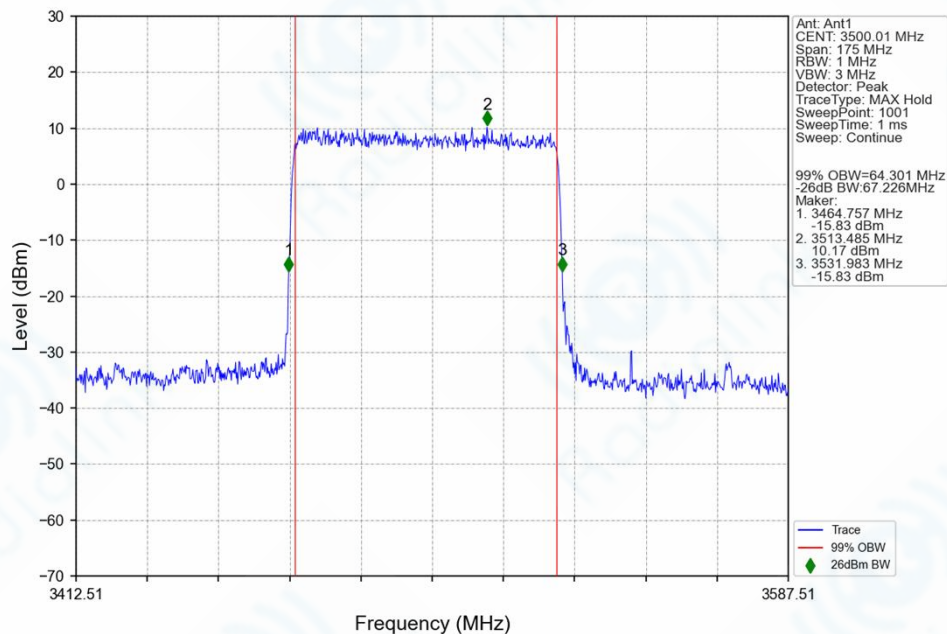
n78e_30kHz_SISO_NTNV_70MHz_DFT-s-OFDM_16_QAM_3500.01MHz_Outer_Full_Ant1
