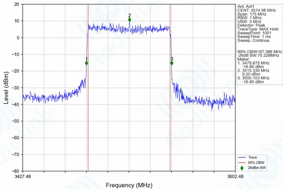
n78e_30kHz_SISO_NTNV_70MHz_CP-OFDM_64_QAM_3514.98MHz_Outer_Full_Ant1
