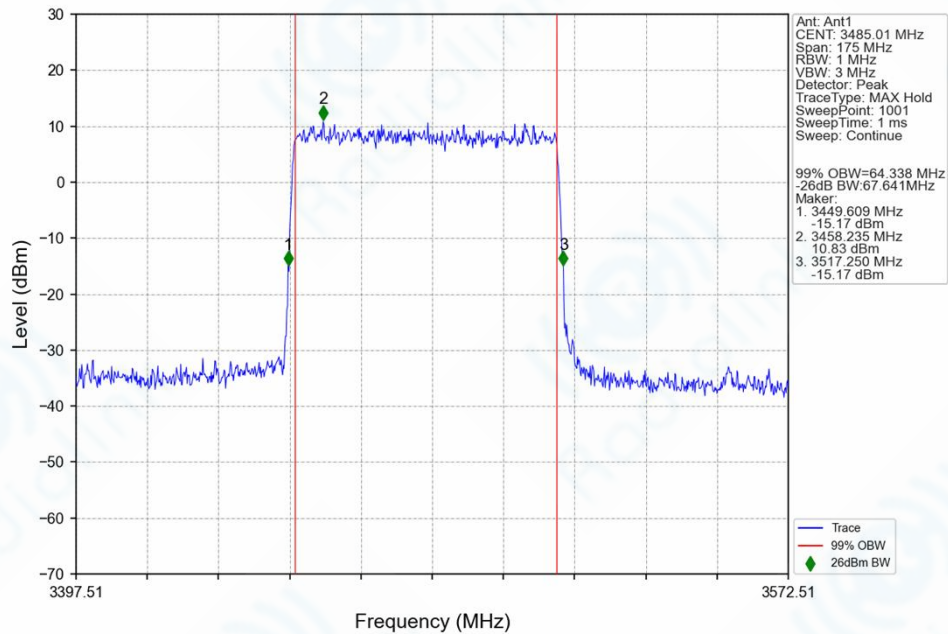
n78e_30kHz_SISO_NTNV_70MHz_DFT-s-OFDM_64_QAM_3485.01MHz_Outer_Full_Ant1
