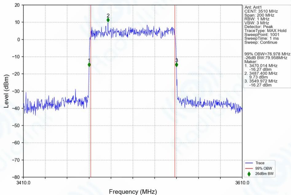
n78e_30kHz_SISO_NTNV_80MHz_DFT-s-OFDM_64_QAM_3510MHz_Outer_Full_Ant1
