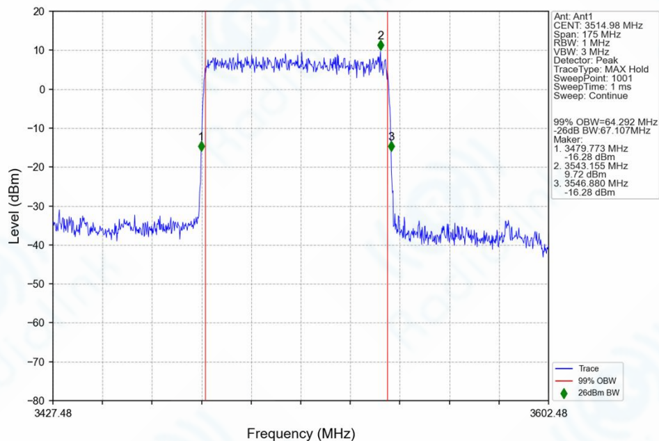
n78e_30kHz_SISO_NTNV_70MHz_DFT-s-OFDM_QPSK_3514.98MHz_Outer_Full_Ant1
