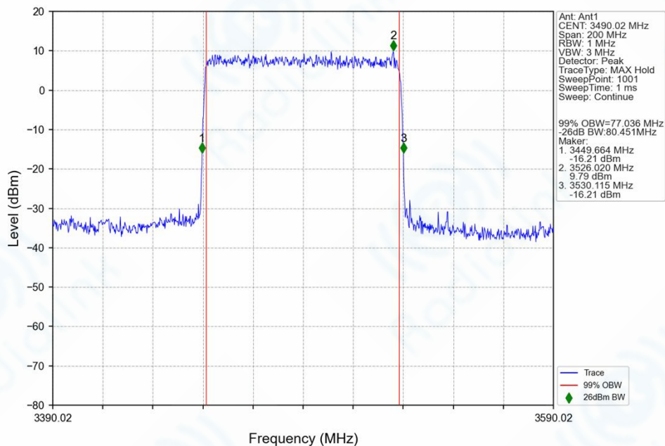
n78e_30kHz_SISO_NTNV_80MHz_DFT-s-OFDM QPSK_3490.02MHz_Outer_Full_Ant1
