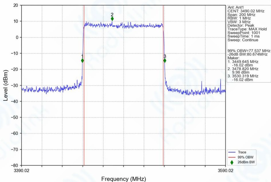
n78e_30kHz_SISO_NTNV_80MHz_CP-OFDM_QPSK_3490.02MHz_Outer_Full_Ant1
