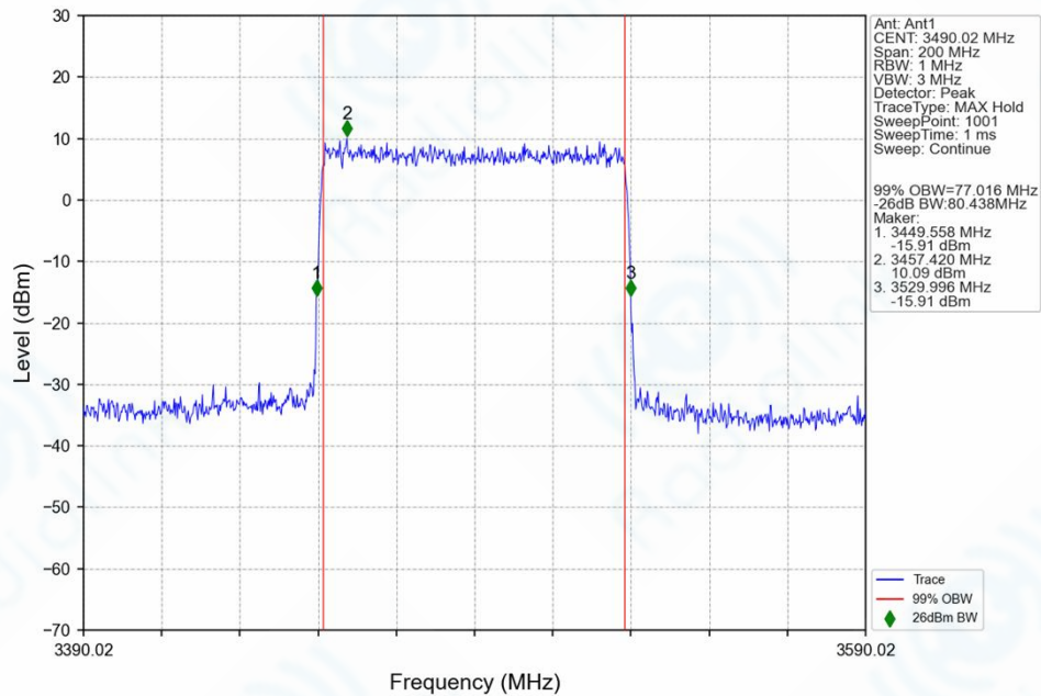
n78e_30kHz_SISO_NTNV_80MHz_DFT-s-OFDM_64_QAM_3490.02MHz_Outer_Full_Ant1
