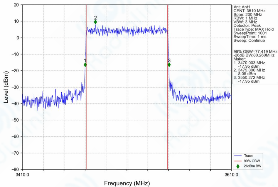
n78e_30kHz_SISO_NTNV_80MHz_CP-OFDM 64 QAM_3510MHz_Outer_Full_Ant1
