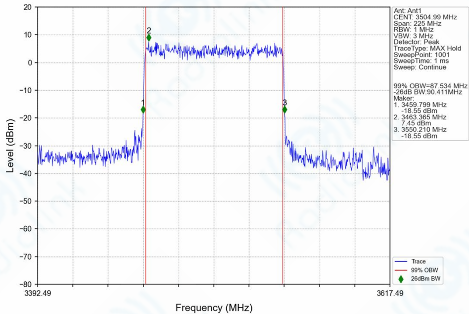
n78e_30kHz_SISO_NTNV_90MHz_CP-OFDM_64_QAM_3504.99MHz_Outer_Full_Ant1
