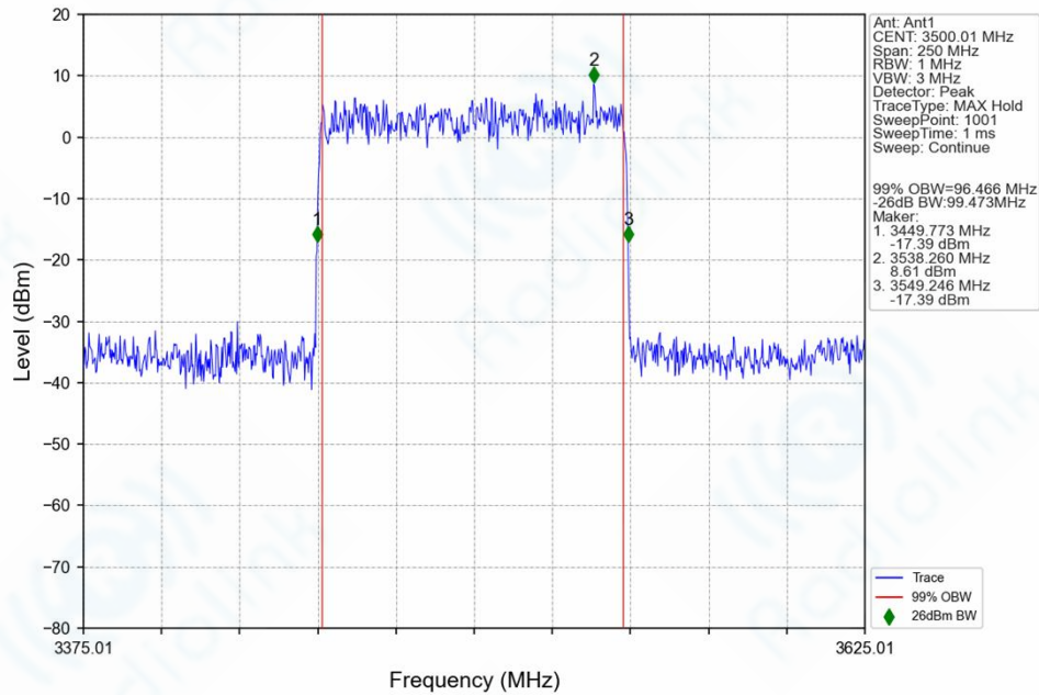
n78e_30kHz_SISO_NTNV_100MHz_DFT-s-OFDM_64_QAM_3500.01MHz_Outer_Full_Ant1
