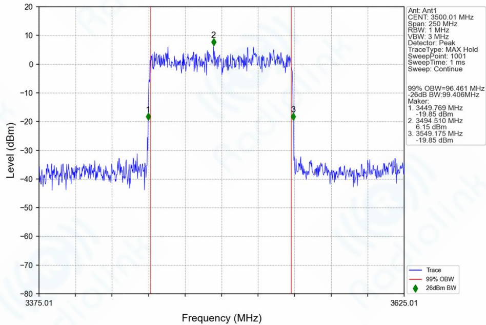
n78e_30kHz_SISO_NTNV_100MHz_CP-OFDM_QPSK_3500.01MHz_Outer_Full_Ant1
