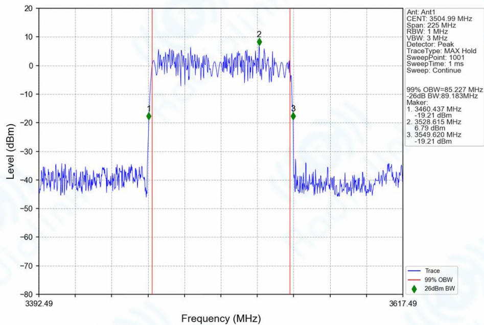
n78e_30kHz_SISO_NTNV_90MHz_DFT-s-OFDM_QPSK_3504.99MHz_Outer_Full_Ant1
