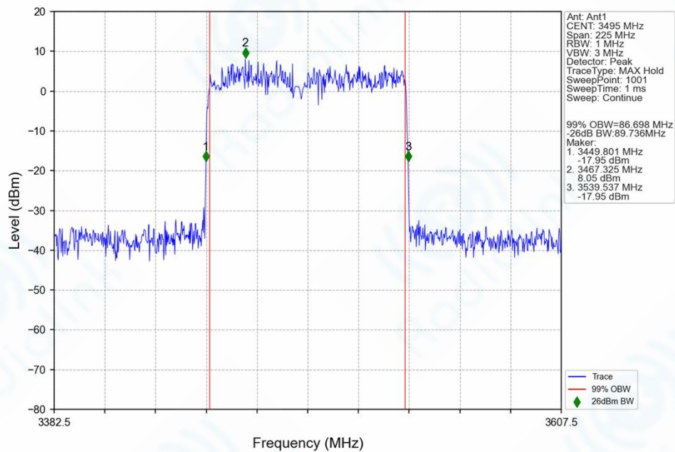
n78e_30kHz_SISO_NTNV_90MHz_DFT-s-OFDM_64_QAM_3495MHz_Outer_Full_Ant1
