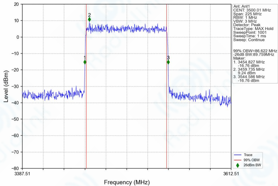
n78e_30kHz_SISO_NTNV_90MHz_DFT-s-OFDM_16_QAM_3500.01MHz_Outer_Full_Ant1
