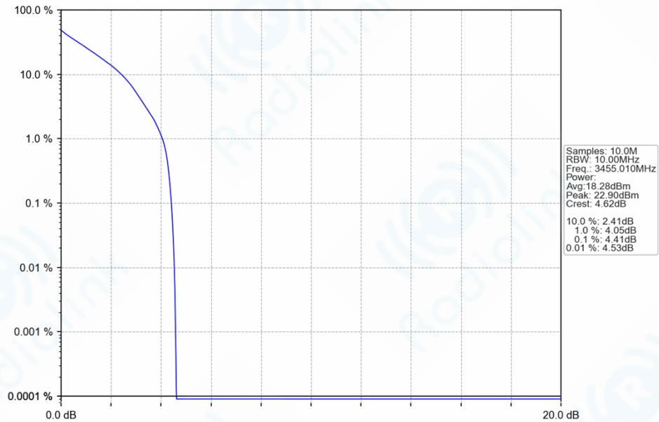
n78e_30kHz_SISO_NTNV_10MHz_DFT-s-OFDM_QPSK_3455.01MHz_Outer_Full_Ant1
