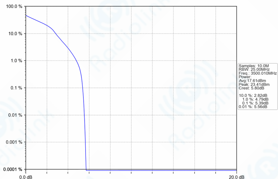
n78e_30kHz_SISO_NTNV_20MHz_DFT-s-OFDM_16_QAM_3500.01MHz_Outer_Full_Ant1
