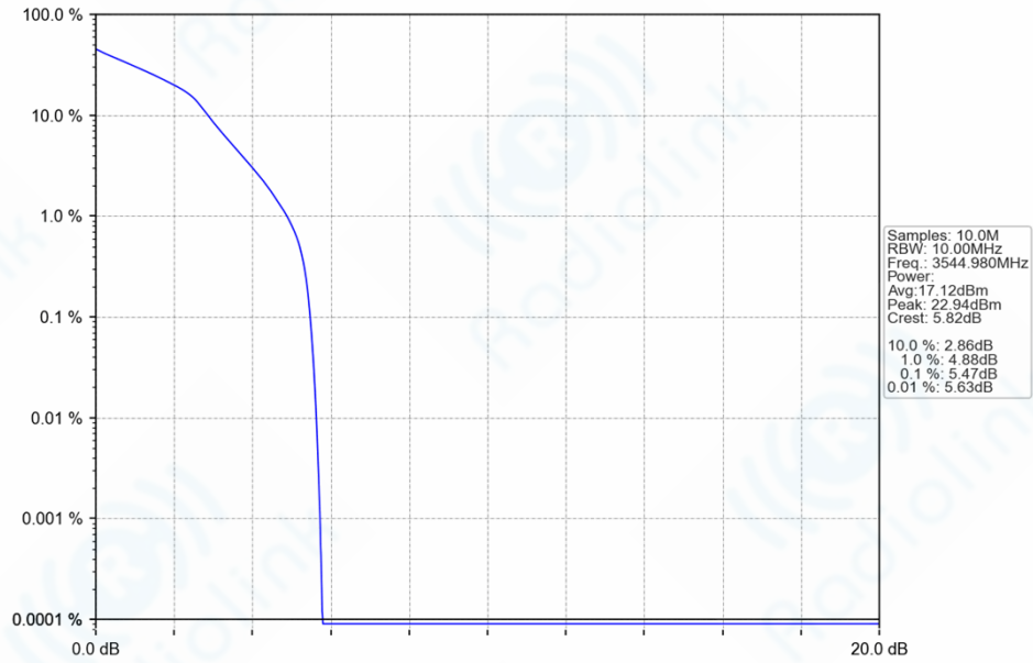
n78e_30kHz_SISO_NTNV_10MHz_DFT-s-OFDM_16_QAM_3544.98MHz_Outer_Full_Ant1
