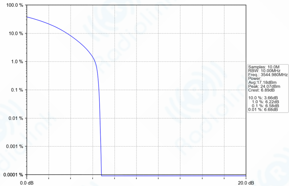
n78e_30kHz_SISO_NTNV_10MHz_CP-OFDM_QPSK_3544.98MHz_Outer_Full_Ant1
