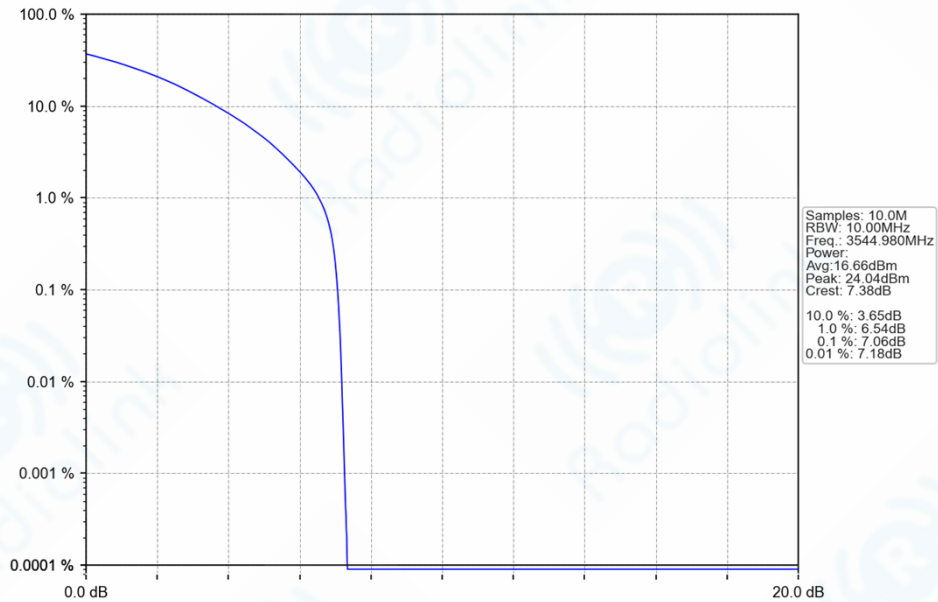
n78e_30kHz_SISO_NTNV_10MHz_CP-OFDM_64_QAM_3544.98MHz_Outer_Full_Ant1
