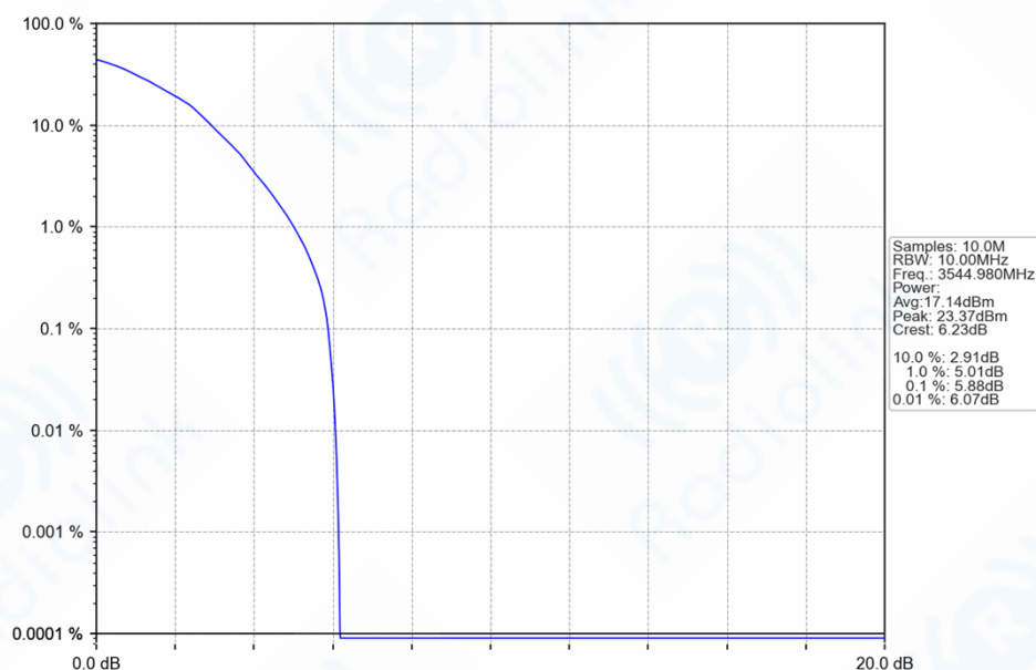
n78e_30kHz_SISO_NTNV_10MHz_DFT-s-OFDM_64_QAM_3544.98MHz_Outer_Full_Ant1
