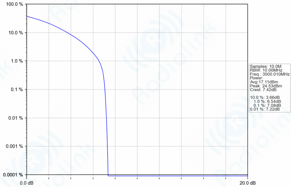
n78e_30kHz_SISO_NTNV_10MHz_CP-OFDM_64_QAM_3500.01MHz_Outer_Full_Ant1
