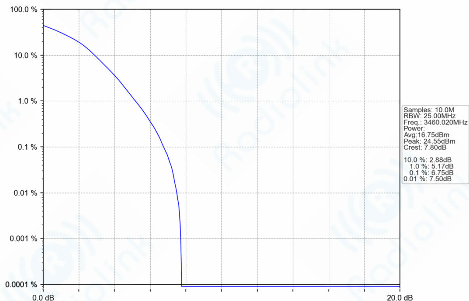
n78e_30kHz_SISO_NTNV_20MHz_DFT-s-OFDM_256_QAM_3460.02MHz_Outer_Full_Ant1
