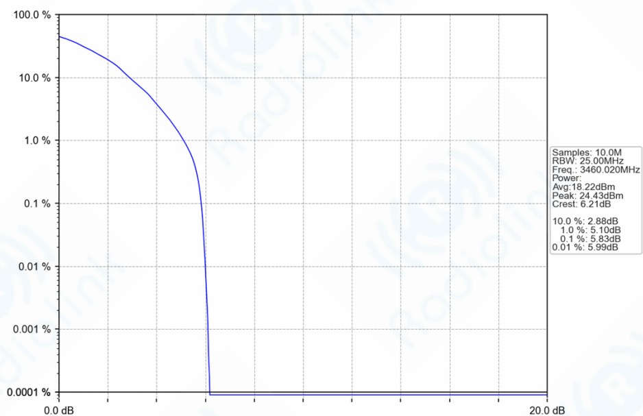
n78e_30kHz_SISO_NTNV_20MHz_DFT-s-OFDM_64_QAM_3460.02MHz_Outer_Full_Ant1
