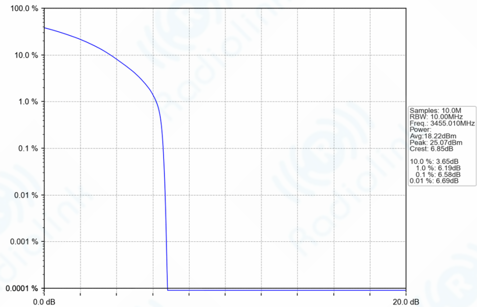
n78e_30kHz_SISO_NTNV_10MHz_CP-OFDM_QPSK_3455.01MHz_Outer_Full_Ant1
