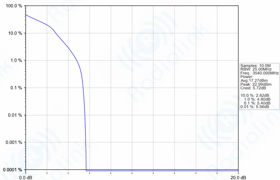
n78e_30kHz_SISO_NTNV_20MHz_DFT-s-OFDM_16_QAM_3540MHz_Outer_Full_Ant1
