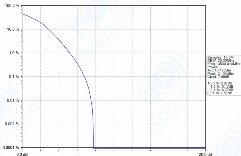
n78e_30kHz_SISO_NTNV_20MHz_DFT-s-OFDM_256_QAM_3500.01MHz_Outer_Full_Ant1
