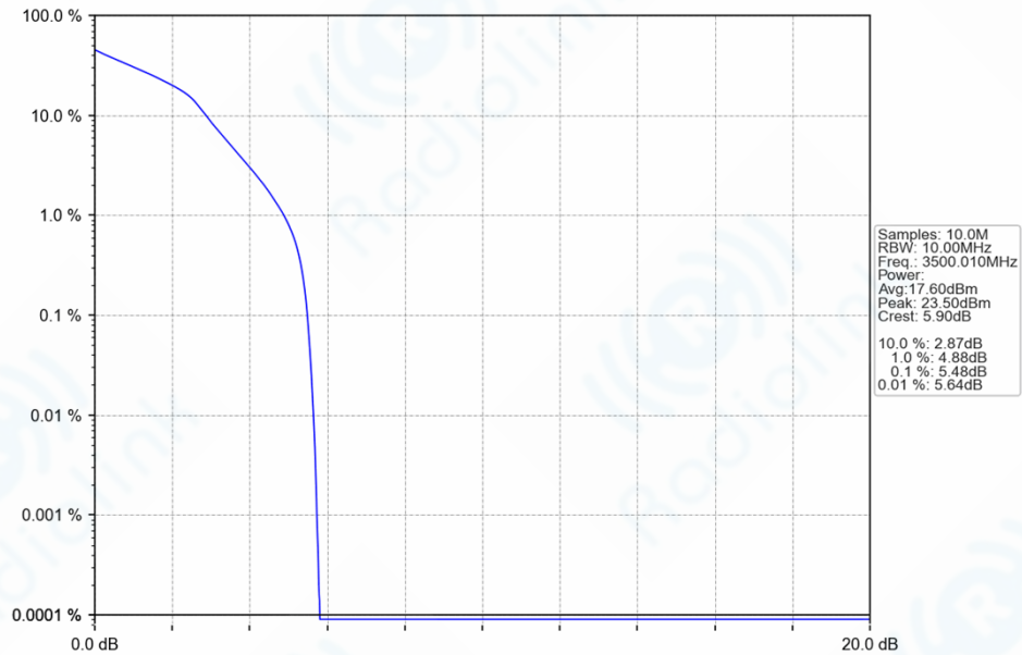
n78e_30kHz_SISO_NTNV_10MHz_DFT-s-OFDM_16_QAM_3500.01MHz_Outer_Full_Ant1
