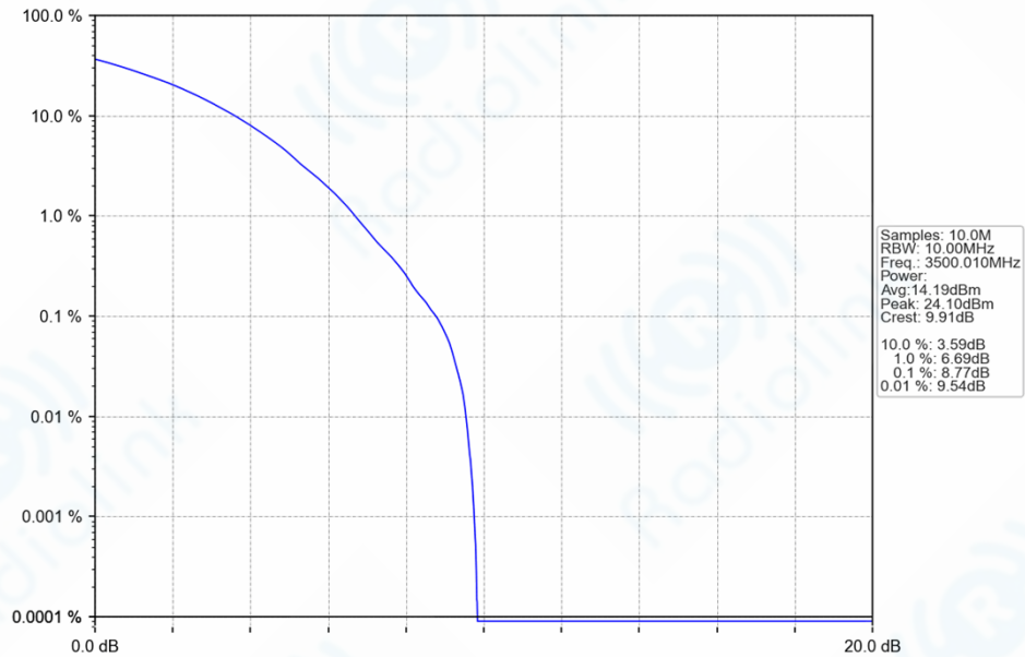
n78e_30kHz_SISO_NTNV_10MHz_CP-OFDM_256_QAM_3500.01MHz_Outer_Full_Ant1
