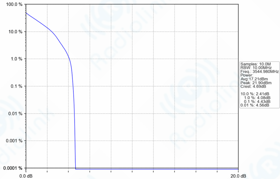
n78e_30kHz_SISO_NTNV_10MHz_DFT-s-OFDM_QPSK_3544.98MHz_Outer_Full_Ant1
