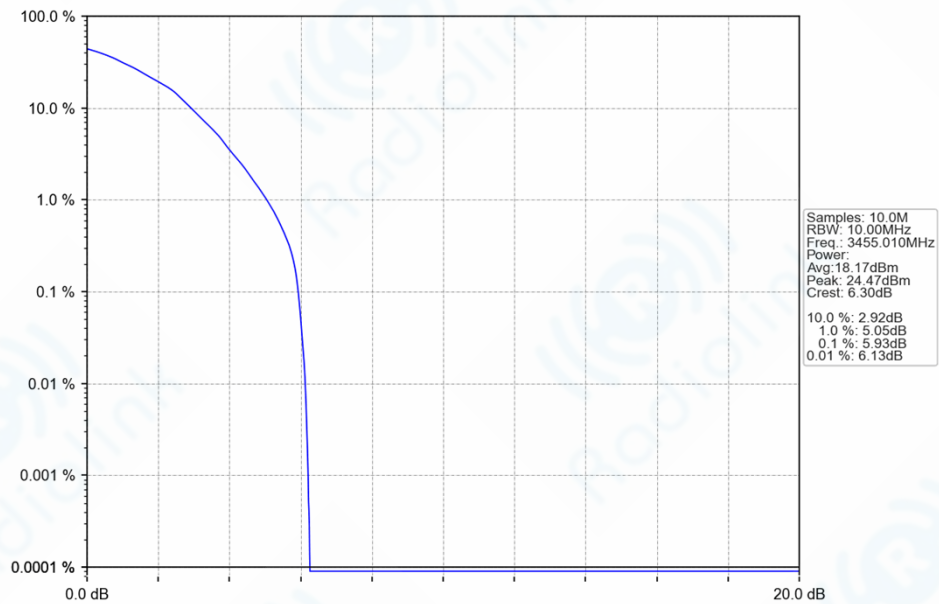
n78e_30kHz_SISO_NTNV_10MHz_DFT-s-OFDM_64_QAM_3455.01MHz_Outer_Full_Ant1
