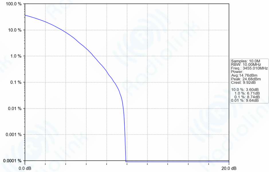
n78e_30kHz_SISO_NTNV_10MHz_CP-OFDM_256_QAM_3455.01MHz_Outer_Full_Ant1
