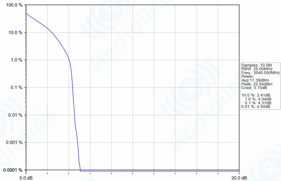
n78e_30kHz_SISO_NTNV_20MHz_DFT-s-OFDM_QPSK_3540MHz_Outer_Full_Ant1
