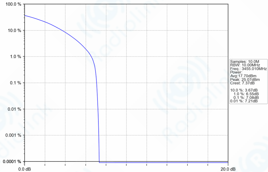
n78e_30kHz_SISO_NTNV_10MHz_CP-OFDM_64_QAM_3455.01MHz_Outer_Full_Ant1
