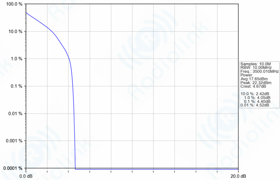
n78e_30kHz_SISO_NTNV_10MHz_DFT-s-OFDM_QPSK_3500.01MHz_Outer_Full_Ant1
