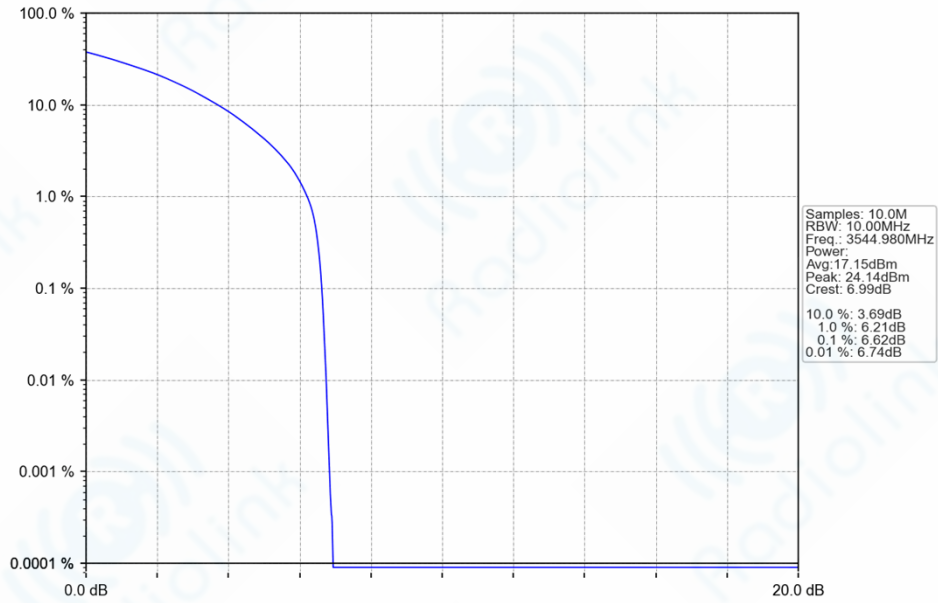
n78e_30kHz_SISO_NTNV_10MHz_CP-OFDM_16_QAM_3544.98MHz_Outer_Full_Ant1
