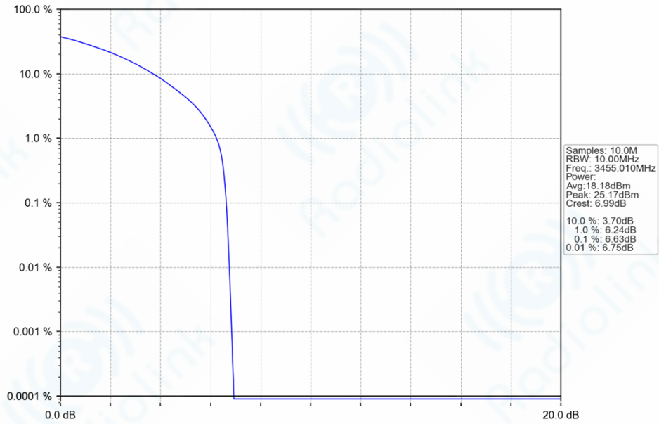
n78e_30kHz_SISO_NTNV_10MHz_CP-OFDM_16_QAM_3455.01MHz_Outer_Full_Ant1
