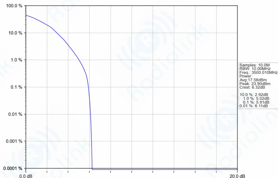
n78e_30kHz_SISO_NTNV_10MHz_DFT-s-OFDM_64_QAM_3500.01MHz_Outer_Full_Ant1
