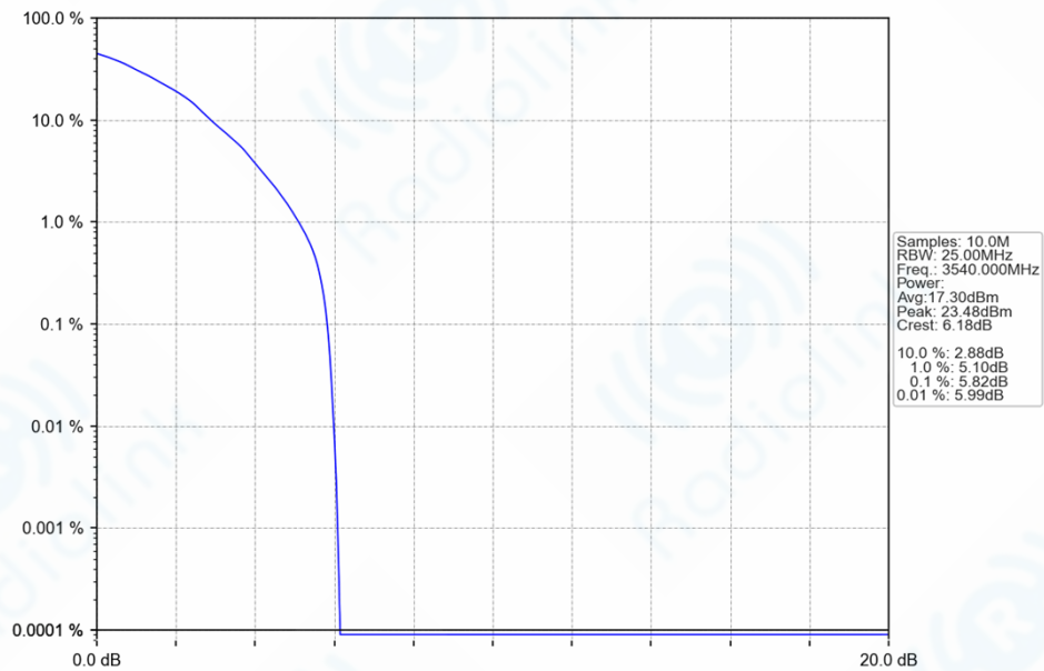
n78e_30kHz_SISO_NTNV_20MHz_DFT-s-OFDM_64_QAM_3540MHz_Outer_Full_Ant1
