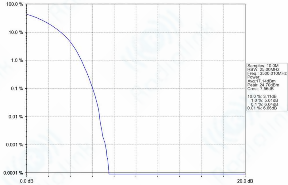
n78e_30kHz_SISO_NTNV_40MHz_DFT-s-OFDM_QPSK_3500.01MHz_Outer_Full_Ant1
