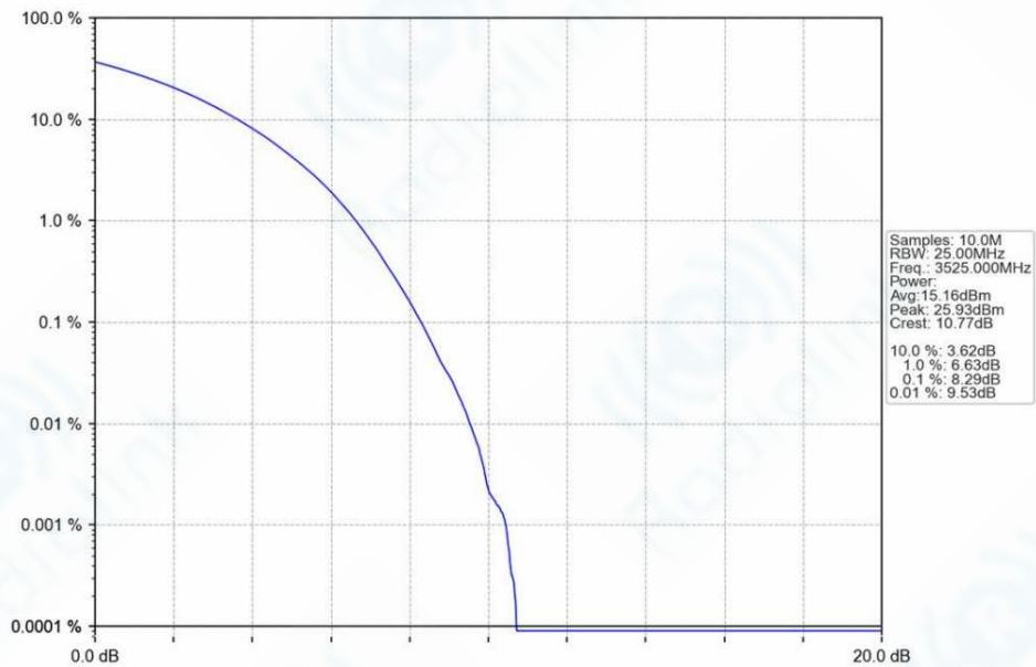
n78e_30kHz_SISO_NTNV_50MHz_CP-OFDM_64_QAM_3525MHz_Outer_Full_Ant1
