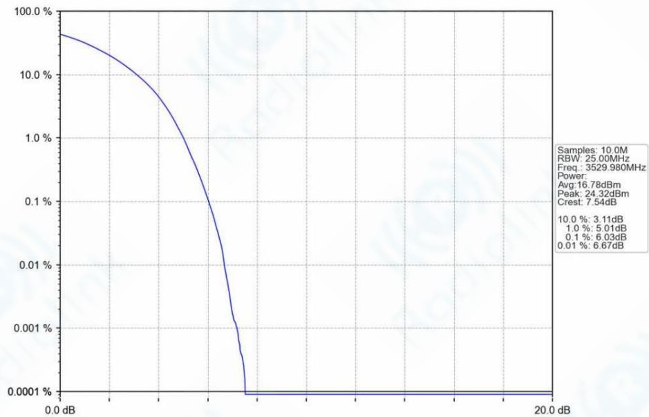
n78e_30kHz_SISO_NTNV_40MHz_DFT-s-OFDM_QPSK_3529.98MHz_Outer_Full_Ant1
