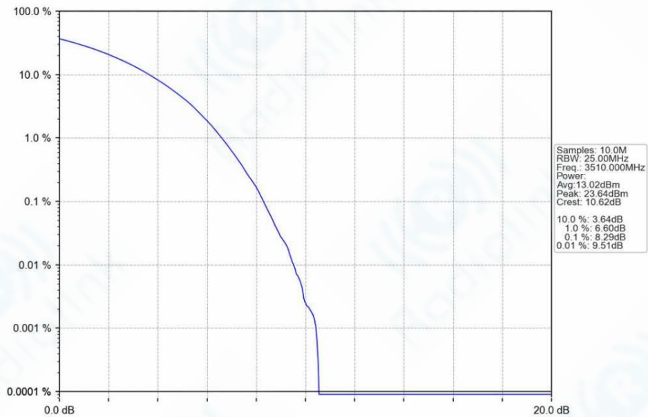
n78e_30kHz_SISO_NTNV_80MHz_CP-OFDM_64_QAM_3510MHz_Outer_Full_Ant1
