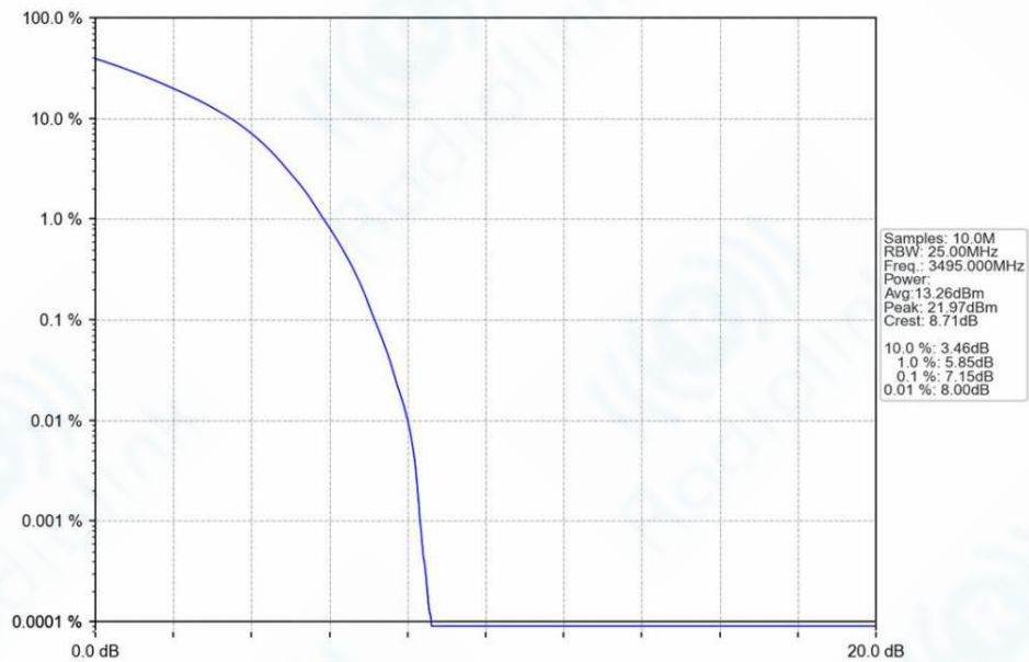
n78e_30kHz_SISO_NTNV_90MHz_DFT-s-OFDM QPSK_3495MHz_Outer_Full_Ant1
