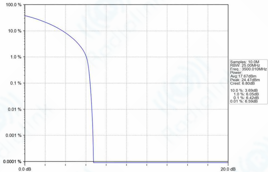
n78e_30kHz_SISO_NTNV_20MHz_CP-OFDM_16_QAM_3500.01MHz_Outer_Full_Ant1
