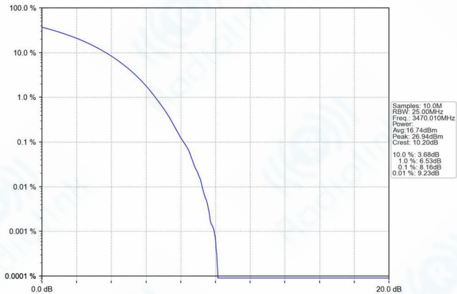
n78e_30kHz_SISO_NTNV_40MHz_CP-OFDM_64_QAM_3470.01MHz_Outer_Full_Ant1
