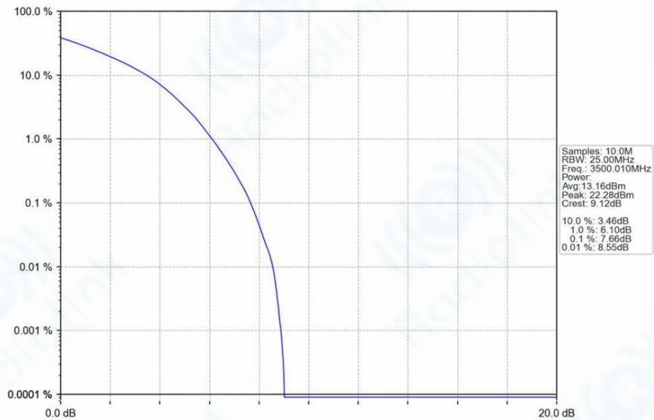
n78e_30kHz_SISO_NTNV_90MHz_DFT-s-OFDM_16_QAM_3500.01MHz_Outer_Full_Ant1
