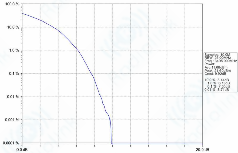
n78e_30kHz_SISO_NTNV_90MHz_DFT-s-OFDM_256_QAM_3495MHz_Outer_Full_Ant1
