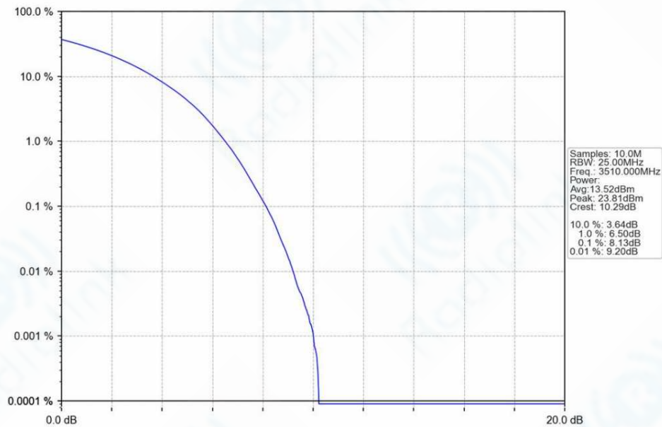
n78e_30kHz_SISO_NTNV_80MHz_CP-OFDM_QPSK_3510MHz_Outer_Full_Ant1
