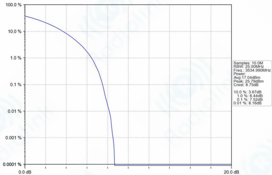
n78e_30kHz_SISO_NTNV_30MHz_CP-OFDM_64_QAM_3534.99MHz_Outer_Full_Ant1
