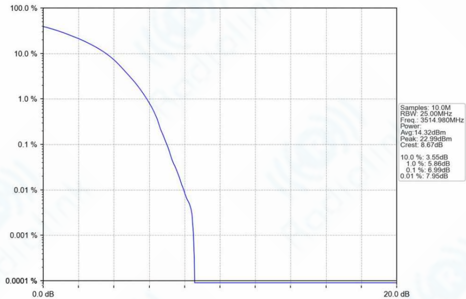
n78e_30kHz_SISO_NTNV_70MHz_DFT-s-OFDM_QPSK_3514.98MHz_Outer_Full_Ant1
