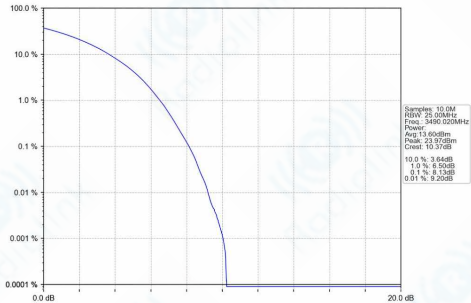
n78e_30kHz_SISO_NTNV_80MHz_CP-OFDM_QPSK_3490.02MHz_Outer_Full_Ant1
