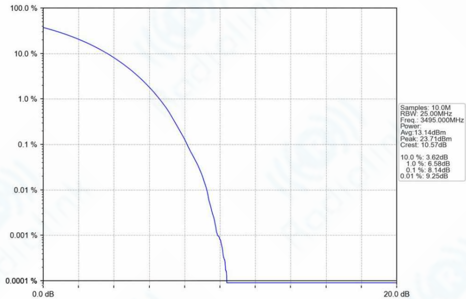
n78e_30kHz_SISO_NTNV_90MHz_CP-OFDM_QPSK_3495MHz_Outer_Full_Ant1
