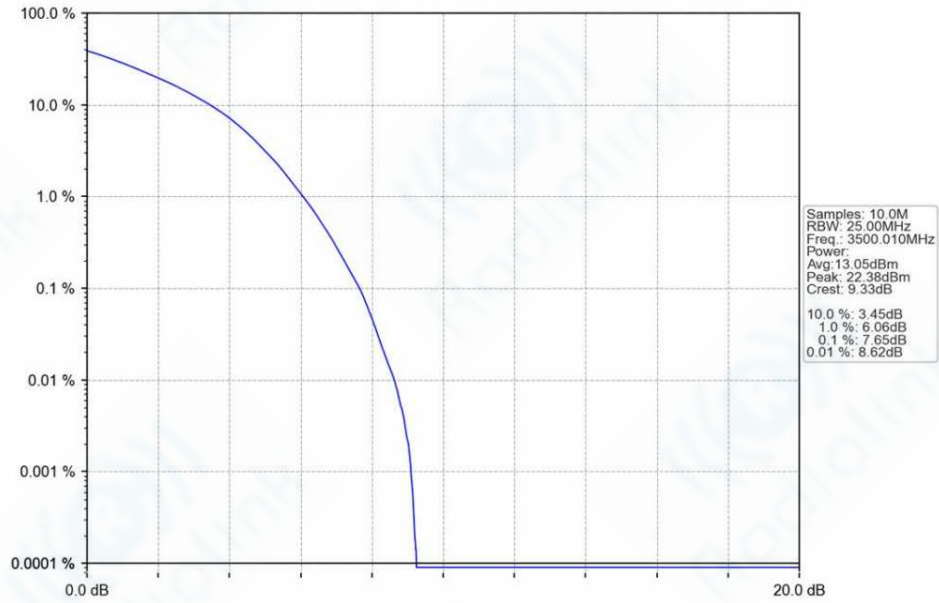
n78e_30kHz_SISO_NTNV_90MHz_DFT-s-OFDM_64_QAM_3500.01MHz_Outer_Full_Ant1
