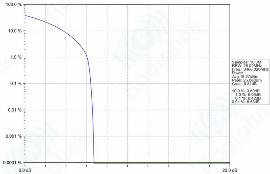
n78e_30kHz_SISO_NTNV_20MHz_CP-OFDM_16_QAM_3460.02MHz_Outer_Full_Ant1
