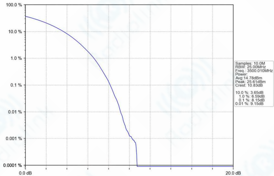
n78e_30kHz_SISO_NTNV_60MHz_CP-OFDM_16_QAM_3500.01MHz_Outer_Full_Ant1
