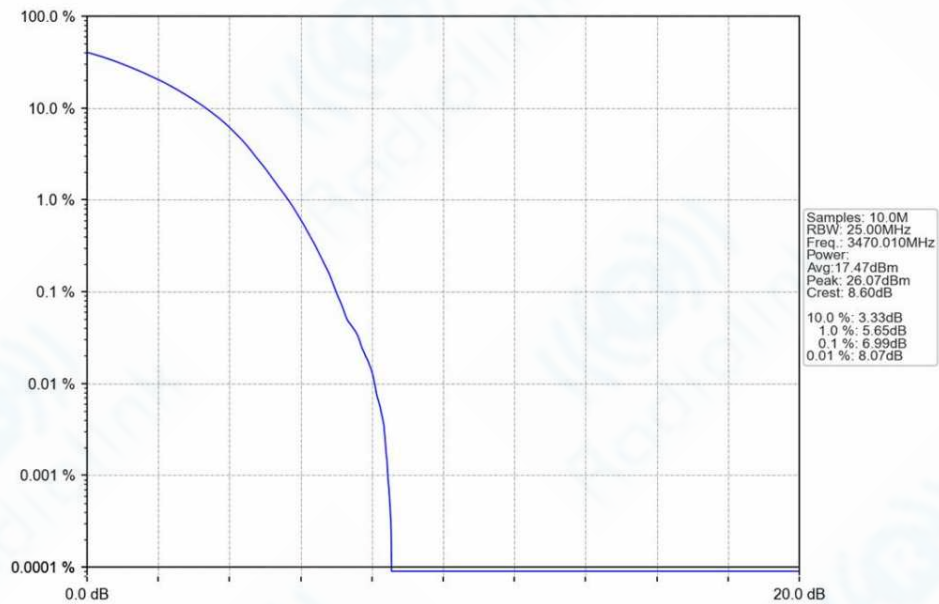
n78e_30kHz_SISO_NTNV_40MHz_DFT-s-OFDM_64_QAM_3470.01MHz_Outer_Full_Ant1
