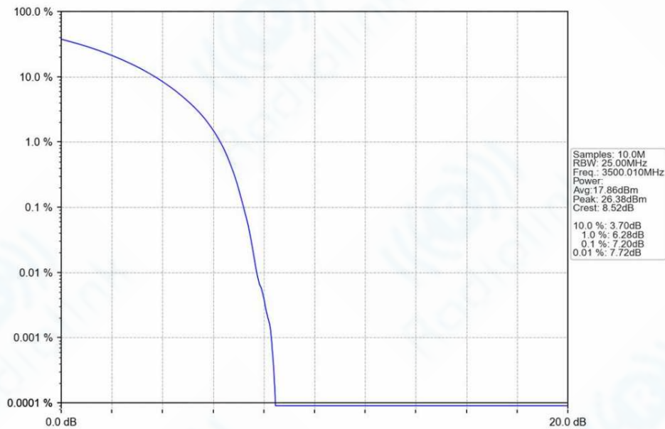
n78e_30kHz_SISO_NTNV_30MHz_CP-OFDM_16_QAM_3500.01MHz_Outer_Full_Ant1
