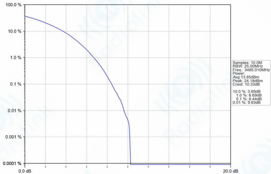
n78e_30kHz_SISO_NTNV_70MHz_CP-OFDM_64_QAM_3485.01MHz_Outer_Full_Ant1
