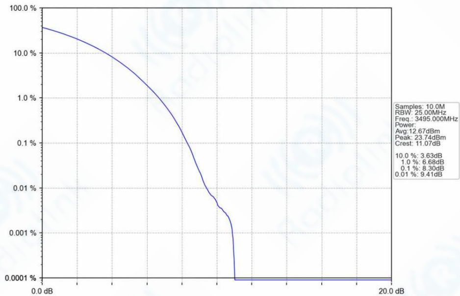
n78e_30kHz_SISO_NTNV_90MHz_CP-OFDM_64_QAM_3495MHz_Outer_Full_Ant1
