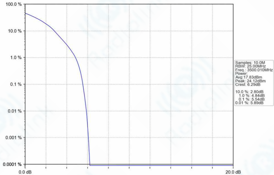
n78e_30kHz_SISO_NTNV_30MHz_DFT-s-OFDM_16_QAM_3500.01MHz_Outer_Full_Ant1
