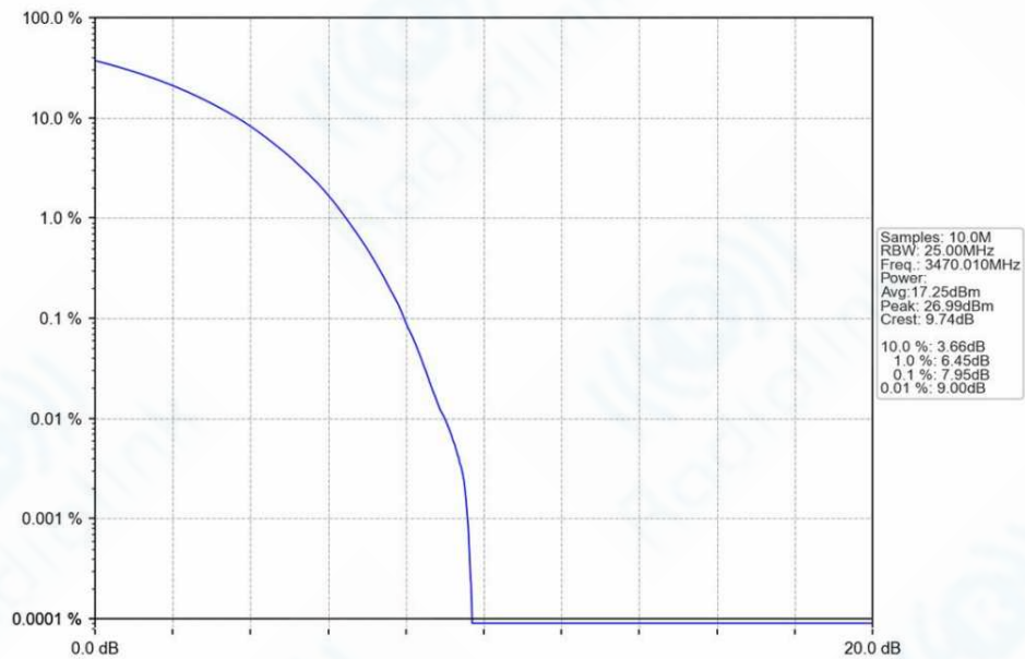
n78e_30kHz_SISO_NTNV_40MHz_CP-OFDM_QPSK_3470.01MHz_Outer_Full_Ant1
