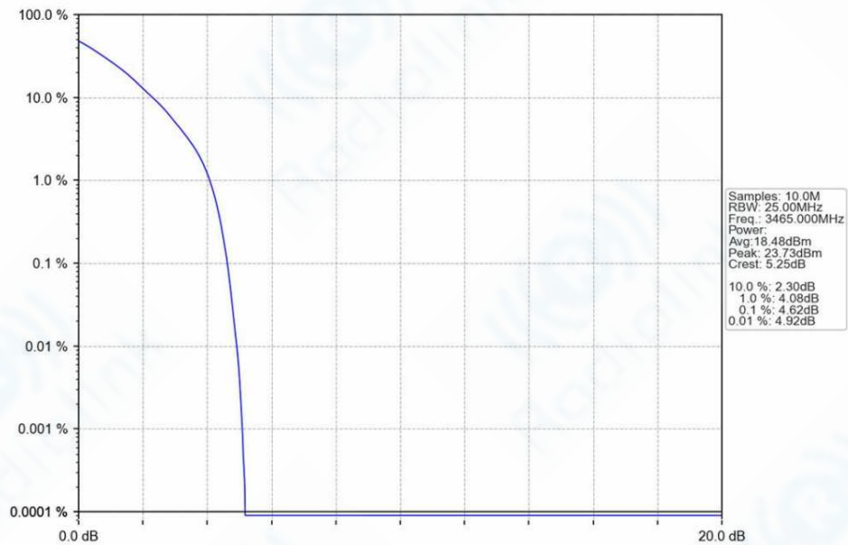
n78e_30kHz_SISO_NTNV_30MHz_DFT-s-OFDM QPSK_3465MHz_Outer_Full_Ant1
