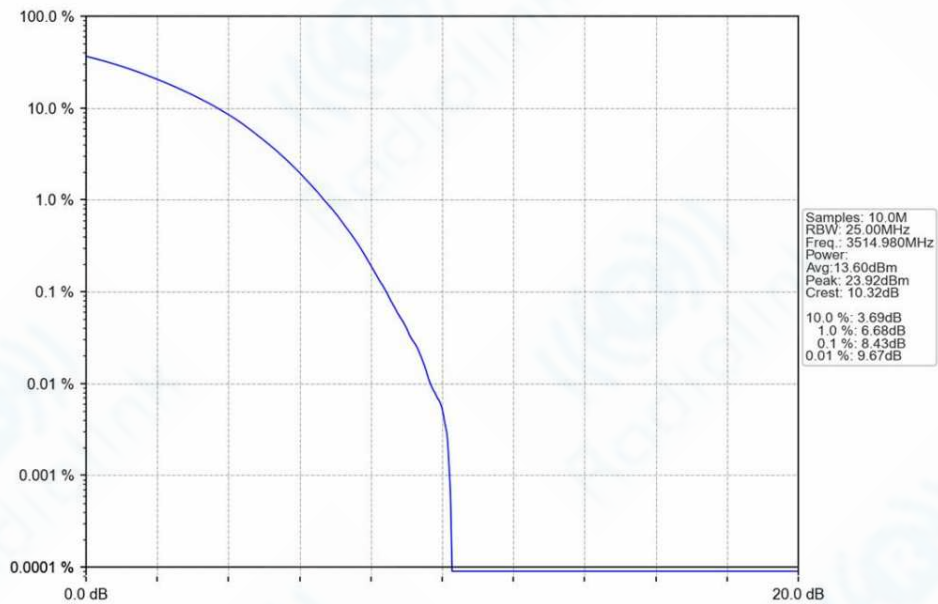
n78e_30kHz_SISO_NTNV_70MHz_CP-OFDM_64_QAM_3514.98MHz_Outer_Full_Ant1
