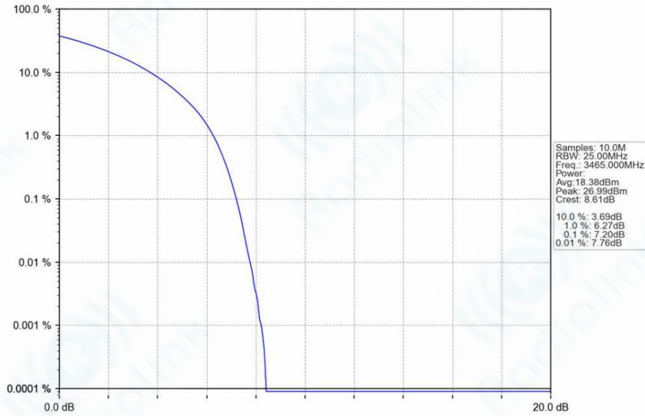
n78e_30kHz_SISO_NTNV_30MHz_CP-OFDM_16_QAM_3465MHz_Outer_Full_Ant1
