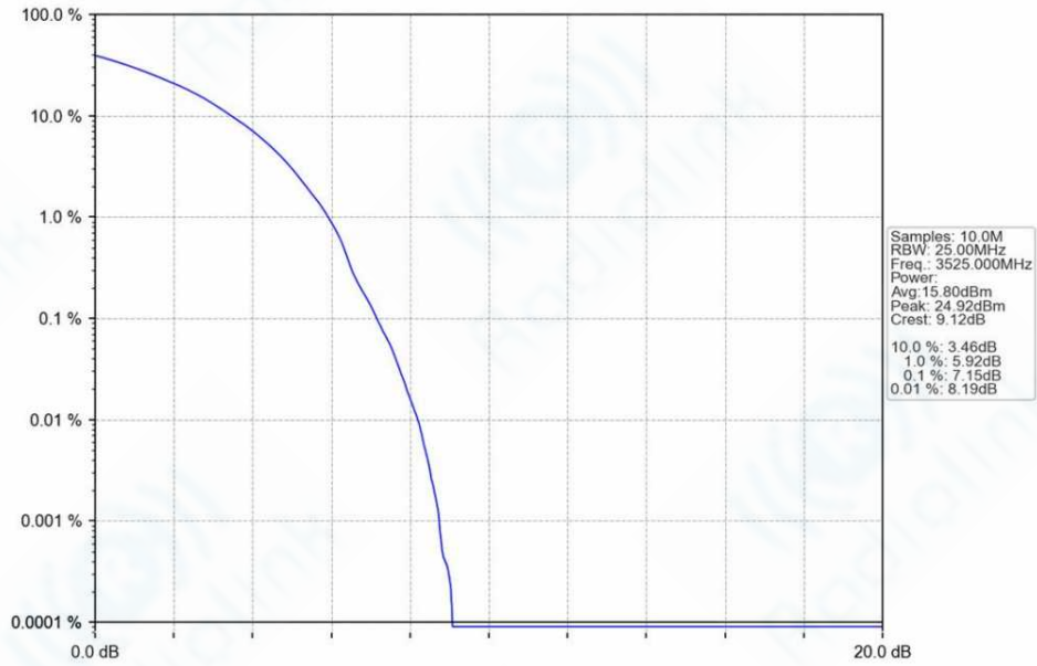
n78e_30kHz_SISO_NTNV_50MHz_DFT-s-OFDM_16_QAM_3525MHz_Outer_Full_Ant1
