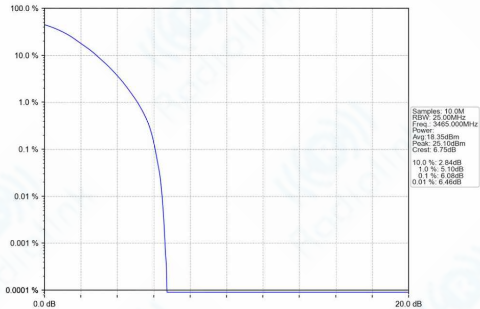
n78e_30kHz_SISO_NTNV_30MHz_DFT-s-OFDM_64_QAM_3465MHz_Outer_Full_Ant1
