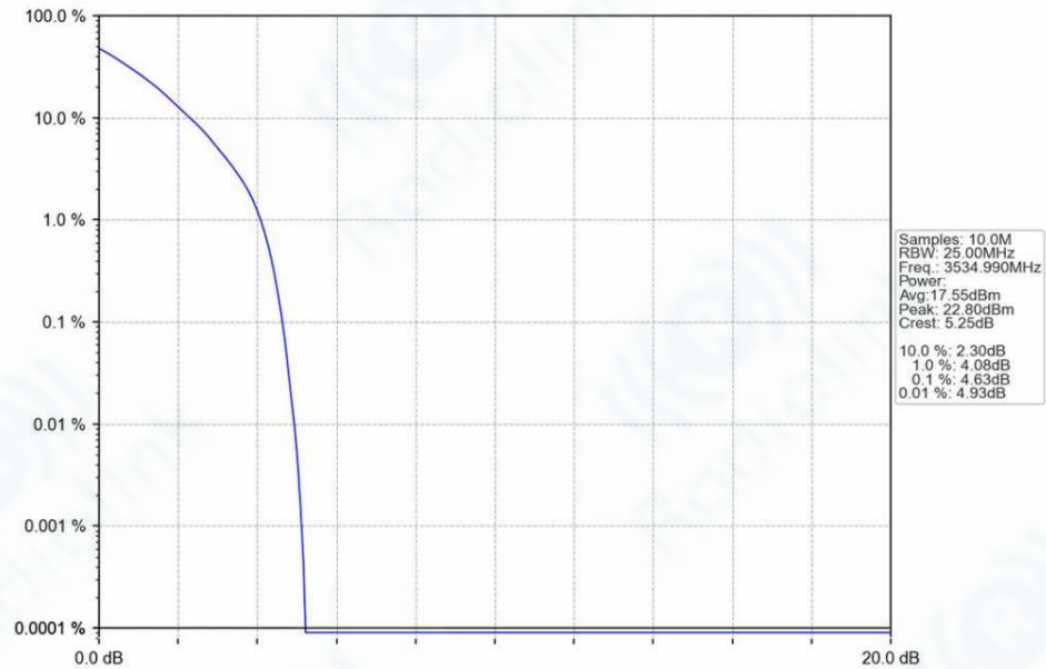
n78e_30kHz_SISO_NTNV_30MHz_DFT-s-OFDM_QPSK_3534.99MHz_Outer_Full_Ant1
