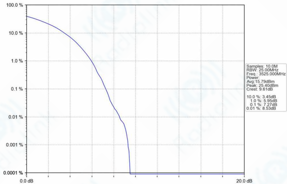
n78e_30kHz_SISO_NTNV_50MHz_DFT-s-OFDM_64_QAM_3525MHz_Outer_Full_Ant1
