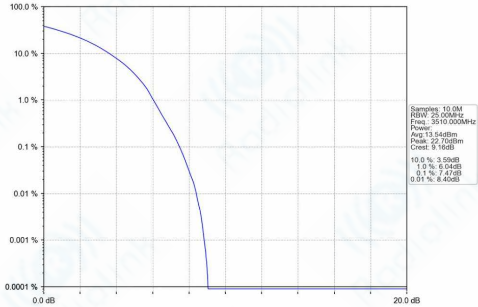
n78e_30kHz_SISO_NTNV_80MHz_DFT-s-OFDM_16_QAM_3510MHz_Outer_Full_Ant1
