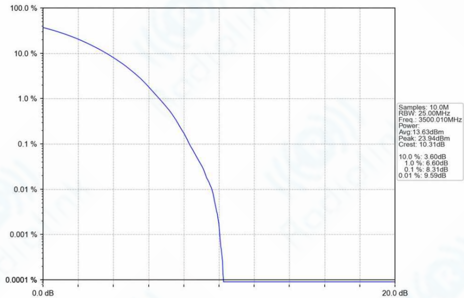
n78e_30kHz_SISO_NTNV_80MHz_CP-OFDM_16_QAM_3500.01MHz_Outer_Full_Ant1
