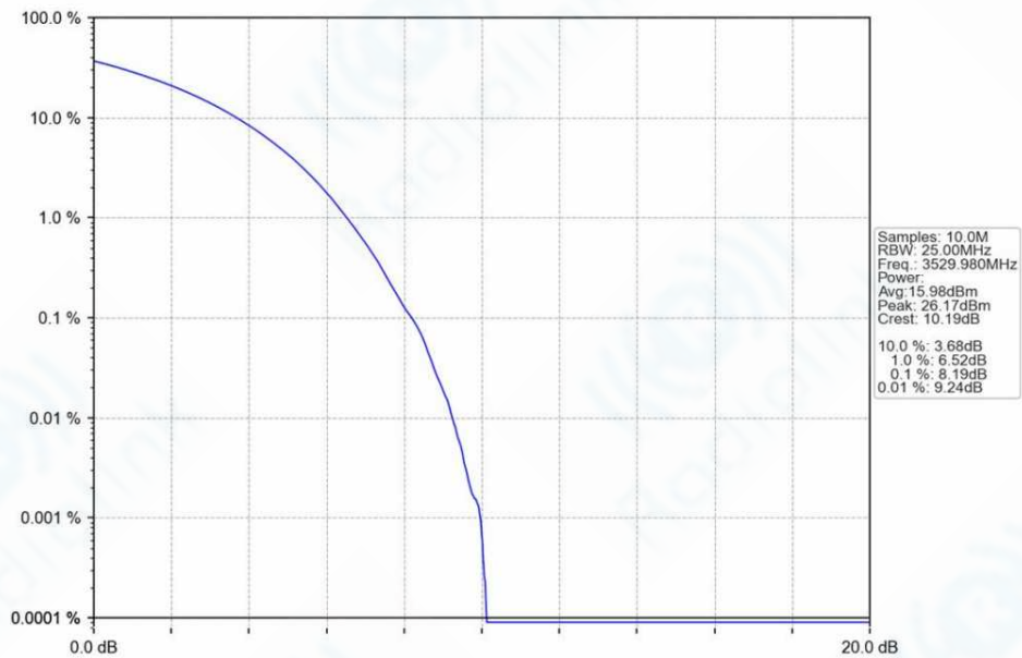
n78e_30kHz_SISO_NTNV_40MHz_CP-OFDM_64_QAM_3529.98MHz_Outer_Full_Ant1
