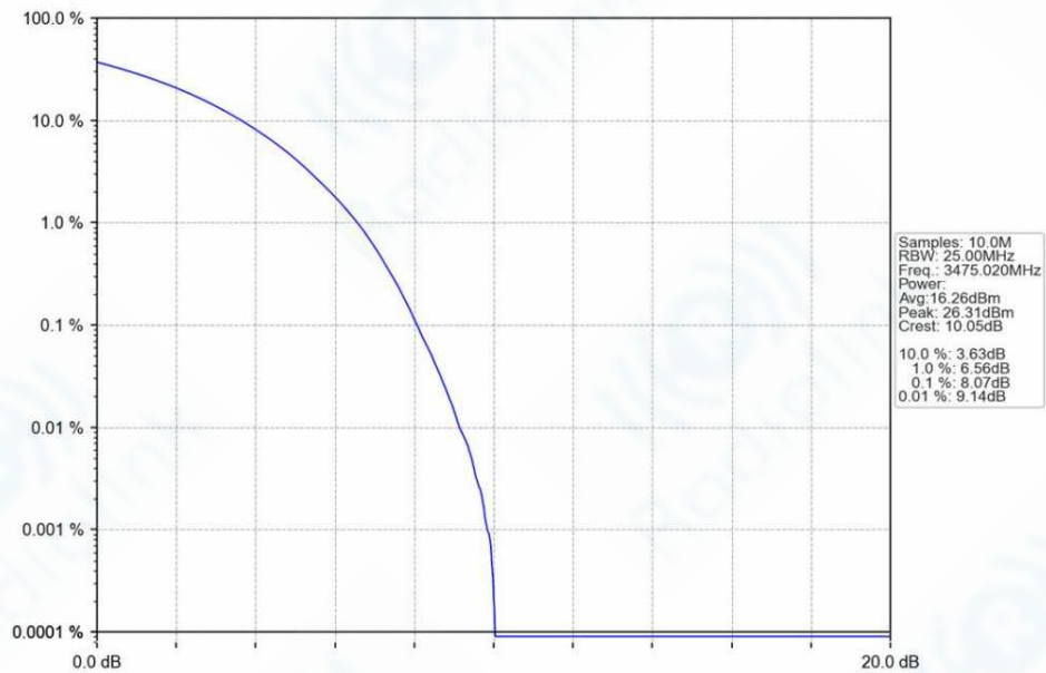
n78e_30kHz_SISO_NTNV_50MHz_CP-OFDM_QPSK_3475.02MHz_Outer_Full_Ant1
