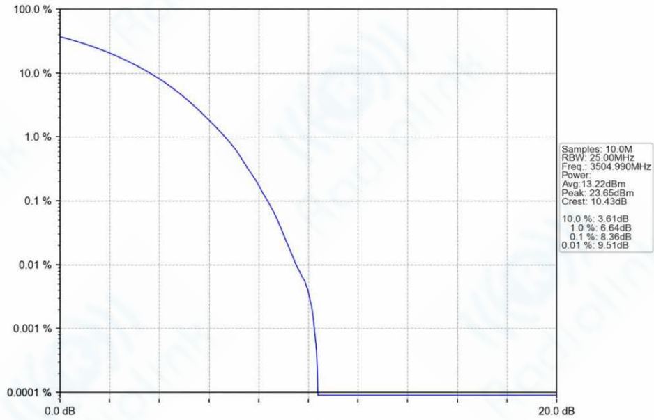
n78e_30kHz_SISO_NTNV_90MHz_CP-OFDM_16_QAM_3504.99MHz_Outer_Full_Ant1
