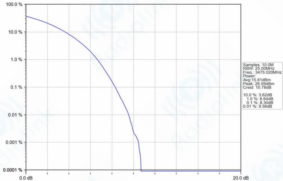
n78e_30kHz_SISO_NTNV_50MHz_CP-OFDM_64_QAM_3475.02MHz_Outer_Full_Ant1
