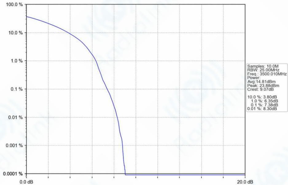
n78e_30kHz_SISO_NTNV_60MHz_DFT-s-OFDM_16_QAM_3500.01MHz_Outer_Full_Ant1
