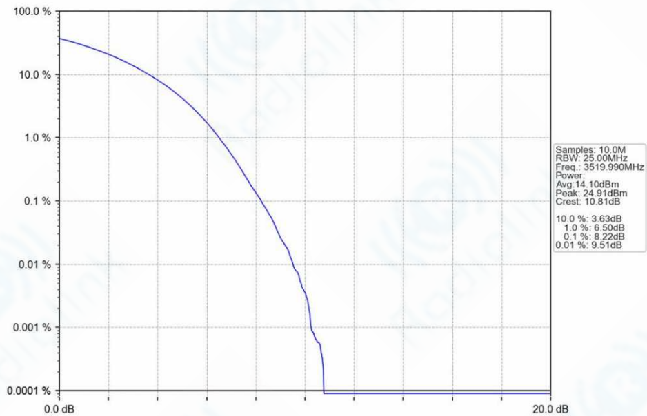
n78e_30kHz_SISO_NTNV_60MHz_CP-OFDM_64_QAM_3519.99MHz_Outer_Full_Ant1
