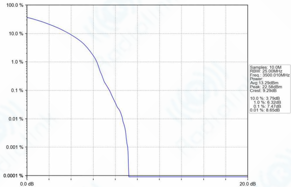
n78e_30kHz_SISO_NTNV_60MHz_DFT-s-OFDM_256_QAM_3500.01MHz_Outer_Full_Ant1
