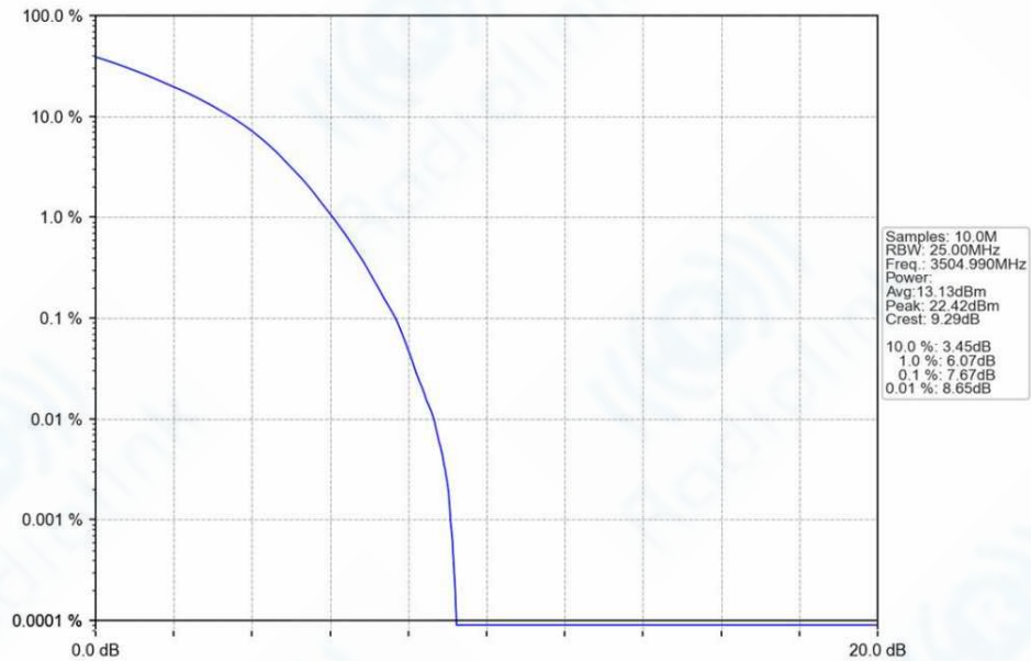
n78e_30kHz_SISO_NTNV_90MHz_DFT-s-OFDM_64_QAM_3504.99MHz_Outer_Full_Ant1
