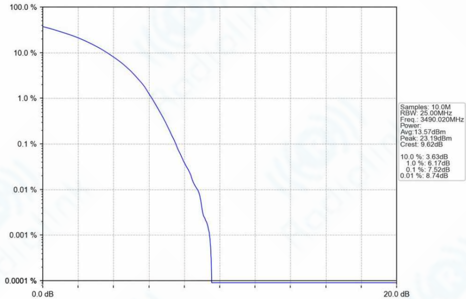
n78e_30kHz_SISO_NTNV_80MHz_DFT-s-OFDM_64_QAM_3490.02MHz_Outer_Full_Ant1
