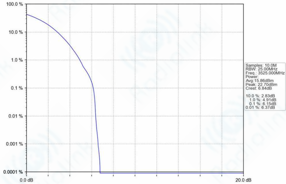
n78e_30kHz_SISO_NTNV_50MHz_DFT-s-OFDM_PI/2_BPSK_3525MHz_Outer_Full_Ant1
