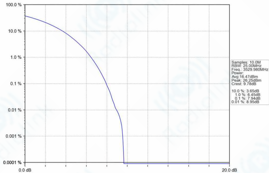
n78e_30kHz_SISO_NTNV_40MHz_CP-OFDM_QPSK_3529.98MHz_Outer_Full_Ant1
