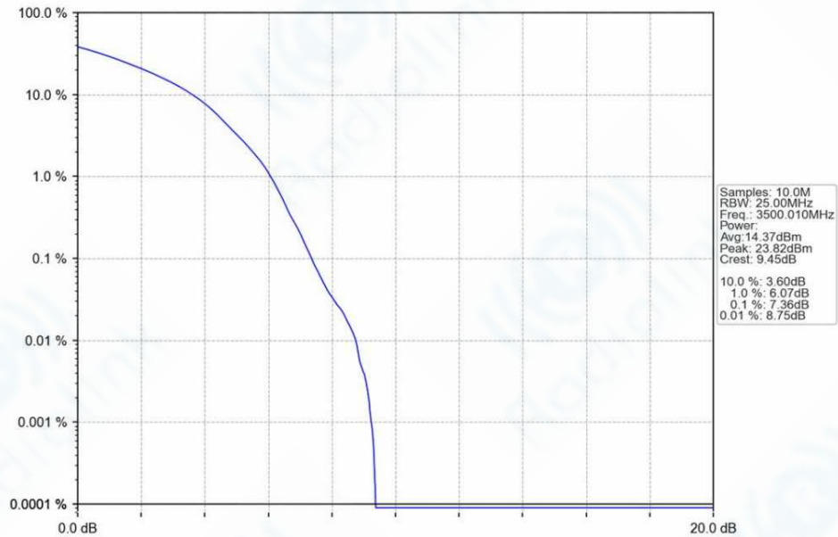
n78e_30kHz_SISO_NTNV_70MHz_DFT-s-OFDM_16_QAM_3500.01MHz_Outer_Full_Ant1
