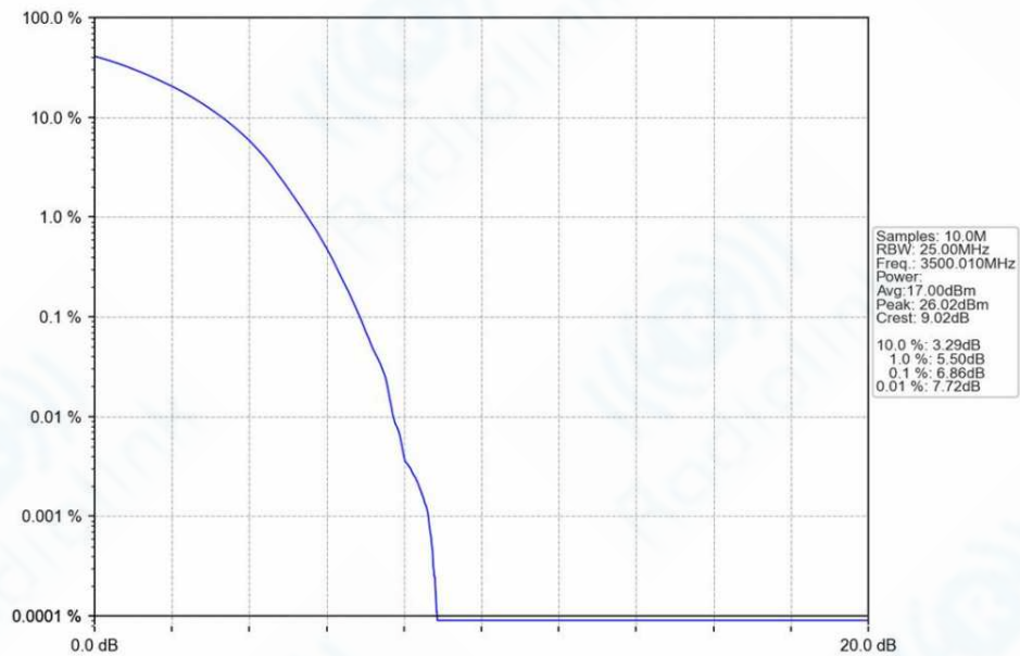
n78e_30kHz_SISO_NTNV_40MHz_DFT-s-OFDM_16_QAM_3500.01MHz_Outer_Full_Ant1
