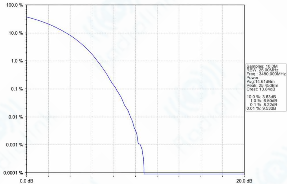
n78e_30kHz_SISO_NTNV_60MHz_CP-OFDM_64_QAM_3480MHz_Outer_Full_Ant1
