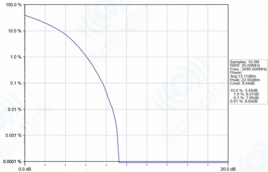
n78e_30kHz_SISO_NTNV_90MHz_DFT-s-OFDM_64_QAM_3495MHz_Outer_Full_Ant1
