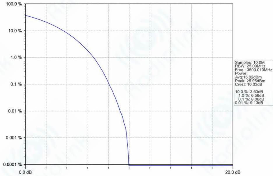
n78e_30kHz_SISO_NTNV_50MHz_CP-OFDM_QPSK_3500.01MHz_Outer_Full_Ant1
