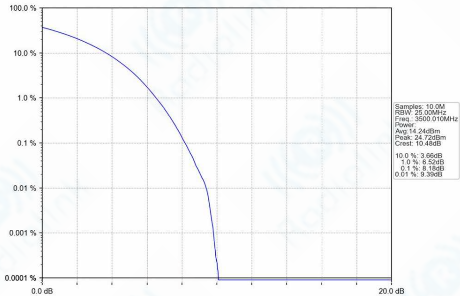
n78e_30kHz_SISO_NTNV_70MHz_CP-OFDM_16_QAM_3500.01MHz_Outer_Full_Ant1
