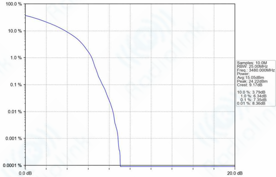
n78e_30kHz_SISO_NTNV_60MHz_DFT-s-OFDM_16_QAM_3480MHz_Outer_Full_Ant1
