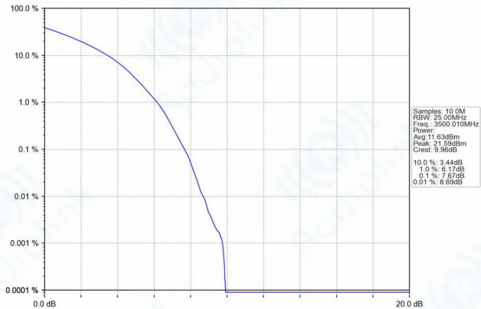
n78e_30kHz_SISO_NTNV_90MHz_DFT-s-OFDM_256_QAM_3500.01MHz_Outer_Full_Ant1
