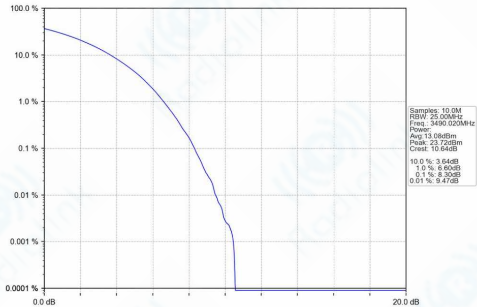
n78e_30kHz_SISO_NTNV_80MHz_CP-OFDM_64_QAM_3490.02MHz_Outer_Full_Ant1
