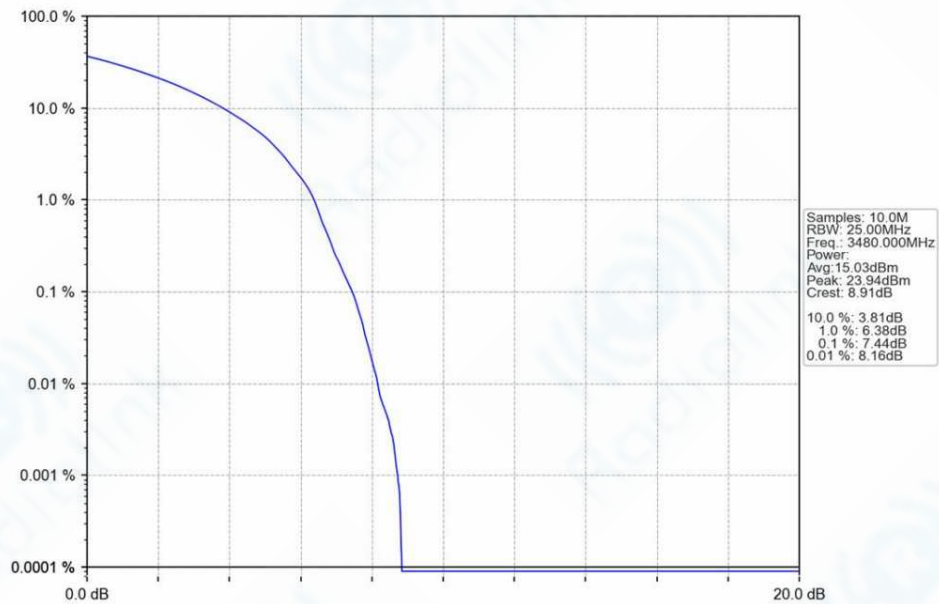
n78e_30kHz_SISO_NTNV_60MHz_DFT-s-OFDM_64_QAM_3480MHz_Outer_Full_Ant1
