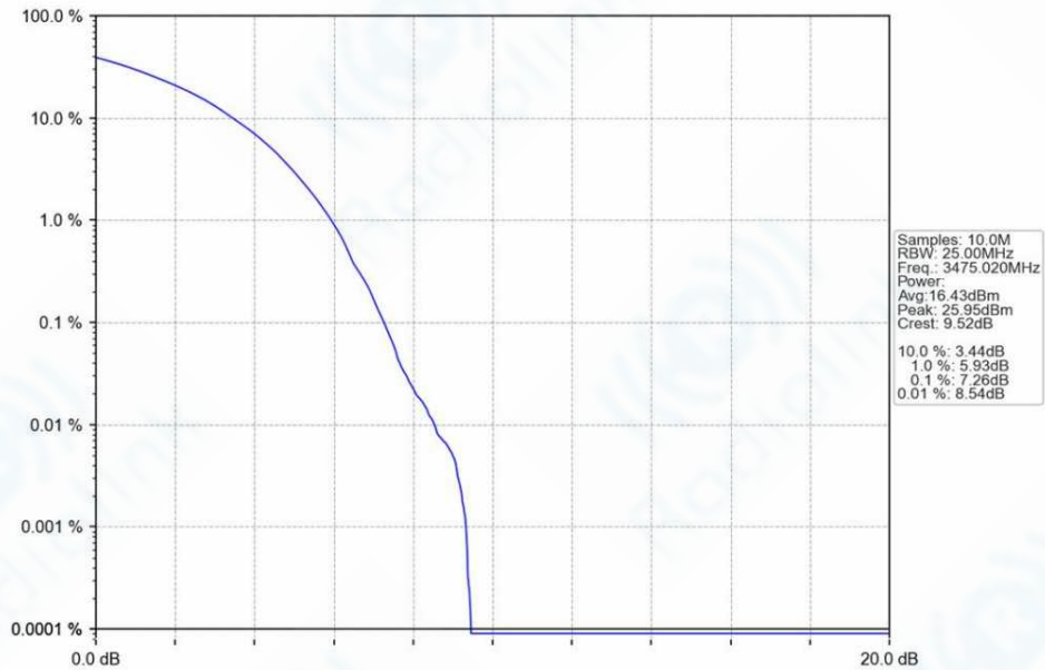
n78e_30kHz_SISO_NTNV_50MHz_DFT-s-OFDM_64_QAM_3475.02MHz_Outer_Full_Ant1
