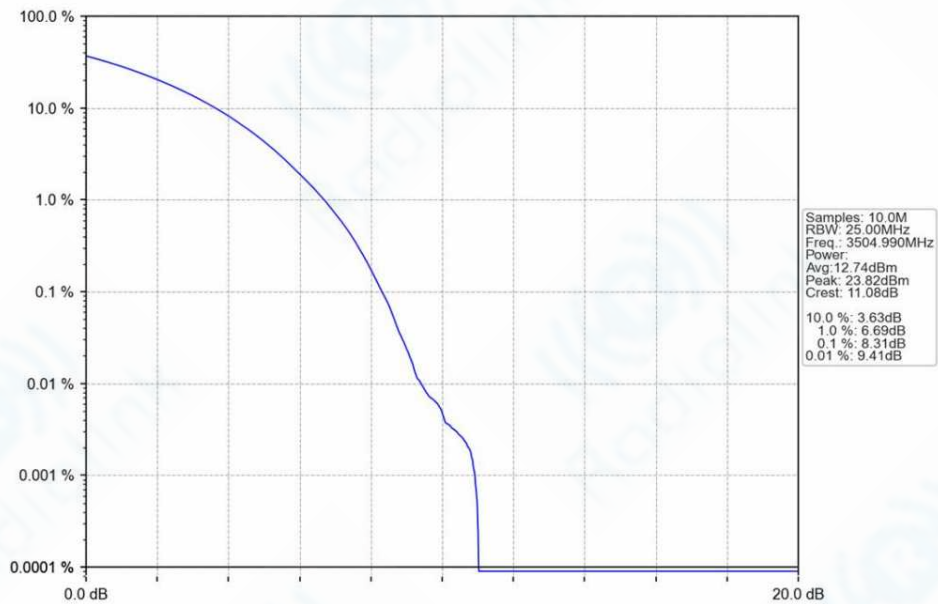
n78e_30kHz_SISO_NTNV_90MHz_CP-OFDM_64_QAM_3504.99MHz_Outer_Full_Ant1
