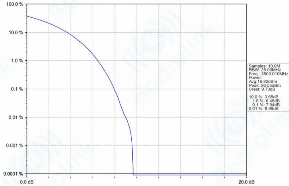
n78e_30kHz_SISO_NTNV_40MHz_CP-OFDM_QPSK_3500.01MHz_Outer_Full_Ant1
