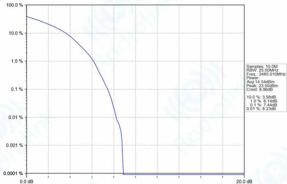
n78e_30kHz_SISO_NTNV_70MHz_DFT-s-OFDM_64_QAM_3485.01MHz_Outer_Full_Ant1
