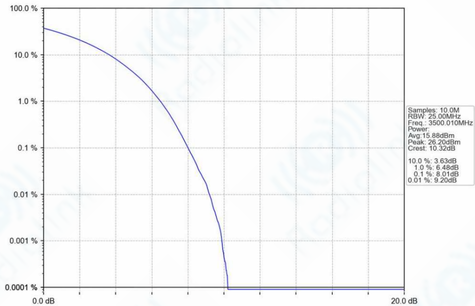
n78e_30kHz_SISO_NTNV_50MHz_CP-OFDM_16_QAM_3500.01MHz_Outer_Full_Ant1
