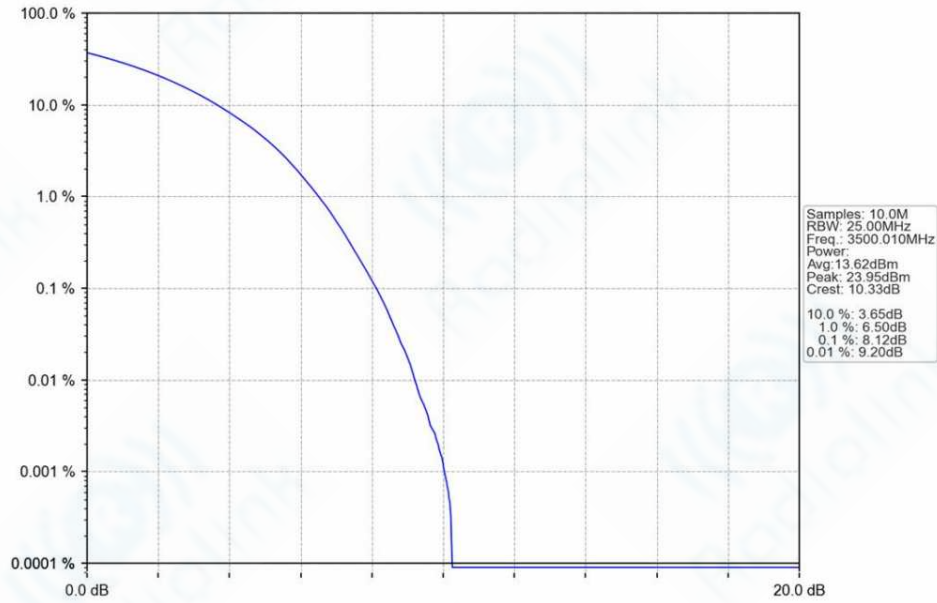
n78e_30kHz_SISO_NTNV_80MHz_CP-OFDM_QPSK_3500.01MHz_Outer_Full_Ant1
