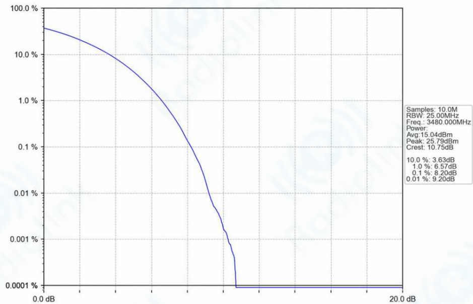
n78e_30kHz_SISO_NTNV_60MHz_CP-OFDM_QPSK_3480MHz_Outer_Full_Ant1
