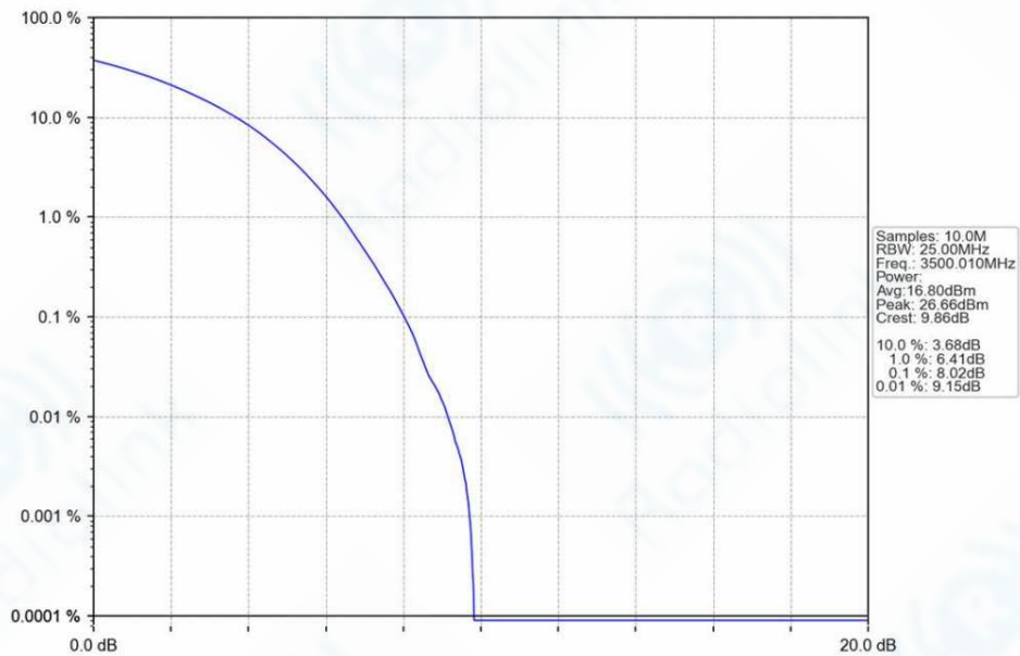
n78e_30kHz_SISO_NTNV_40MHz_CP-OFDM_16_QAM_3500.01MHz_Outer_Full_Ant1
