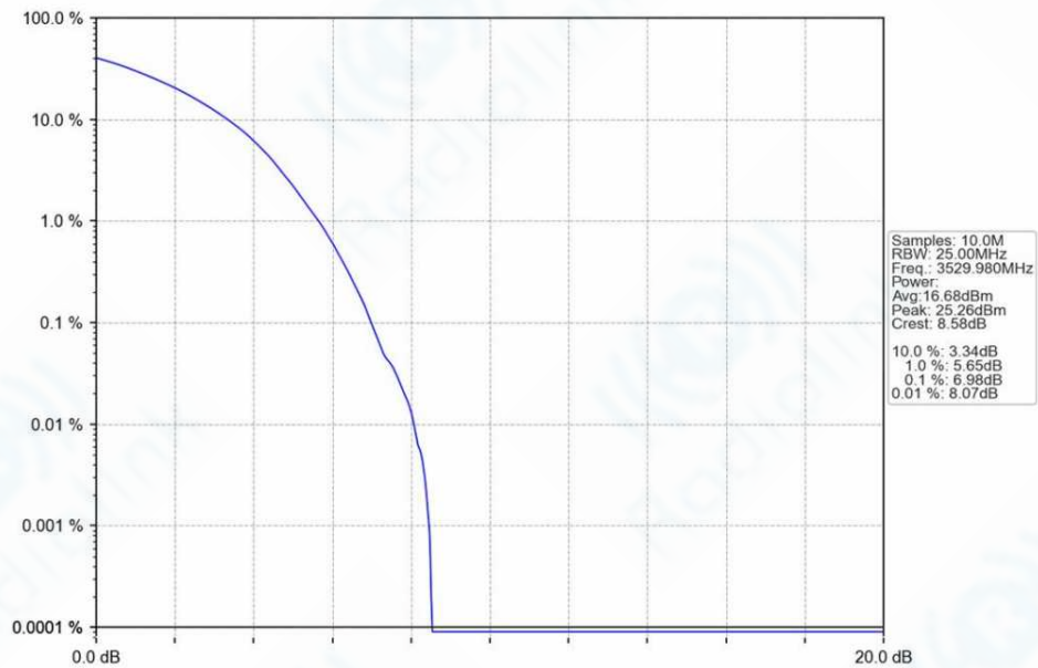
n78e_30kHz_SISO_NTNV_40MHz_DFT-s-OFDM_64_QAM_3529.98MHz_Outer_Full_Ant1
