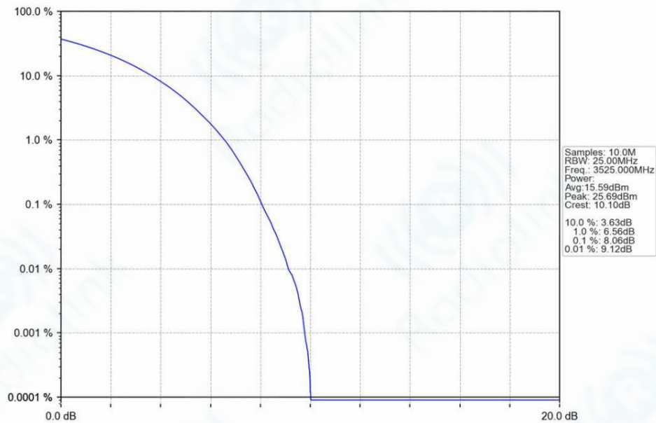
n78e_30kHz_SISO_NTNV_50MHz_CP-OFDM_QPSK_3525MHz_Outer_Full_Ant1
