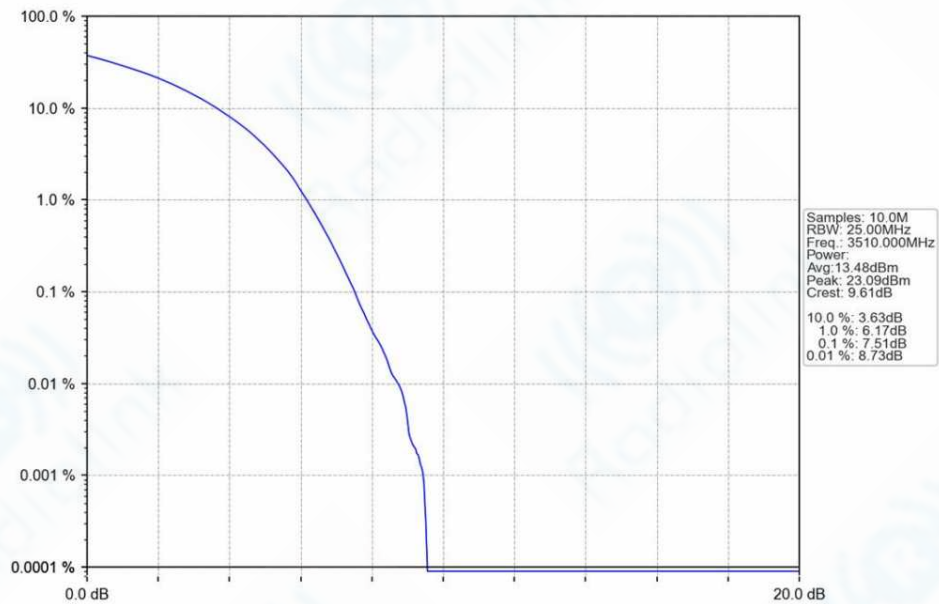
n78e_30kHz_SISO_NTNV_80MHz_DFT-s-OFDM_64_QAM_3510MHz_Outer_Full_Ant1
