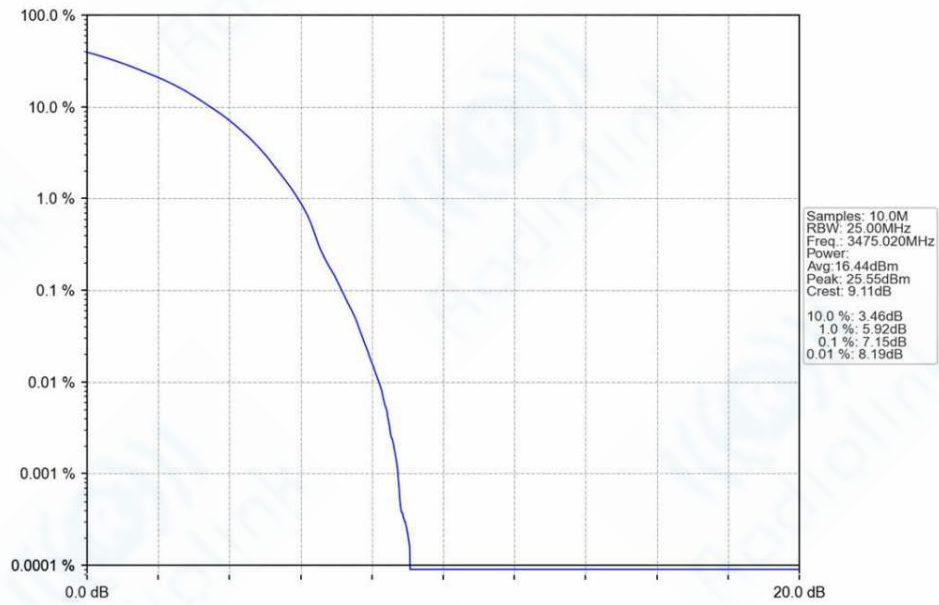
n78e_30kHz_SISO_NTNV_50MHz_DFT-s-OFDM_16_QAM_3475.02MHz_Outer_Full_Ant1
