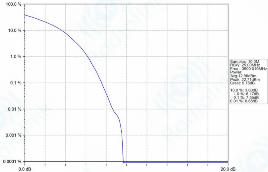
n78e_30kHz_SISO_NTNV_70MHz_DFT-s-OFDM_256_QAM_3500.01MHz_Outer_Full_Ant1
