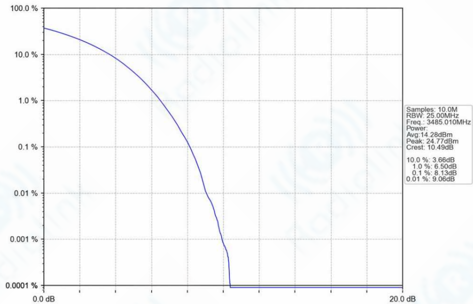
n78e_30kHz_SISO_NTNV_70MHz_CP-OFDM_QPSK_3485.01MHz_Outer_Full_Ant1
