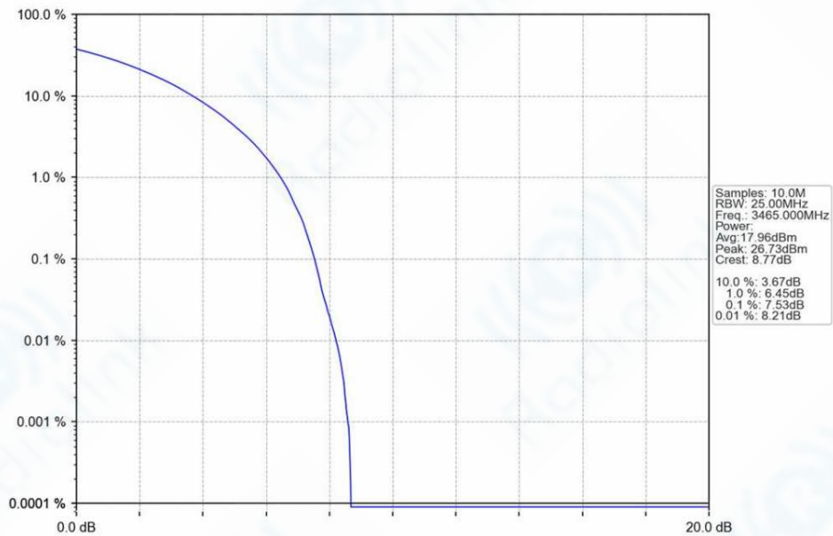
n78e_30kHz_SISO_NTNV_30MHz_CP-OFDM_64_QAM_3465MHz_Outer_Full_Ant1
