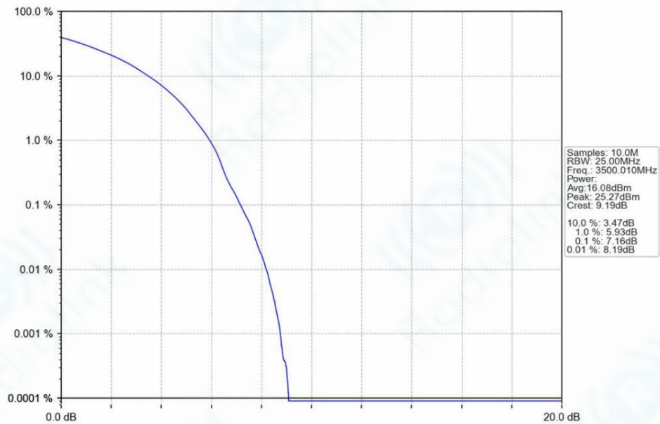
n78e_30kHz_SISO_NTNV_50MHz_DFT-s-OFDM_16_QAM_3500.01MHz_Outer_Full_Ant1
