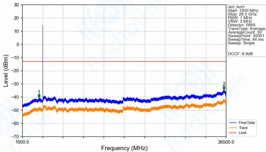
n78e_30kHz_SISO_NTNV_20MHz_DFT-s-OFDM_PI/2_BPSK_3540MHz_Edge_1RB_Right_Ant1
