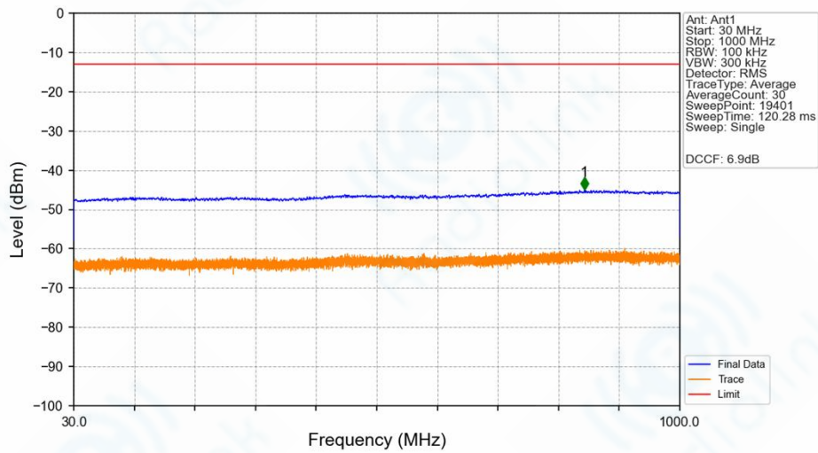
n78e_30kHz_SISO_NTNV_20MHz_DFT-s-OFDM_PI/2_BPSK_3540MHz_Edge_1RB_Right_Ant1
