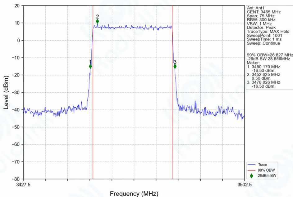
n78f_30kHz_SISO_NTNV_30MHz_DFT-s-OFDM_QPSK_3465MHz_Outer_Full_Ant1
