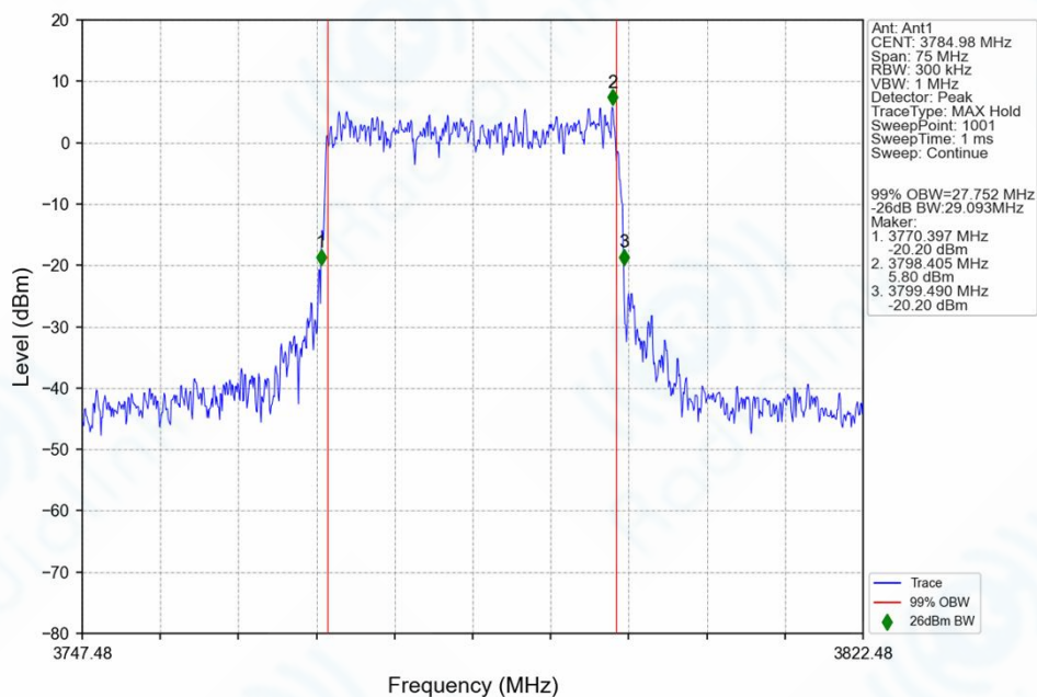
n78f_30kHz_SISO_NTNV_30MHz_CP-OFDM QPSK 3784.98MHz_Outer_Full_Ant1
