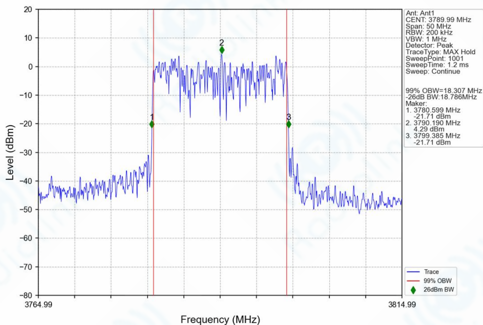
n78f_30kHz_SISO_NTNV_20MHz_CP-OFDM_64_QAM_3789.99MHz_Outer_Full_Ant1
