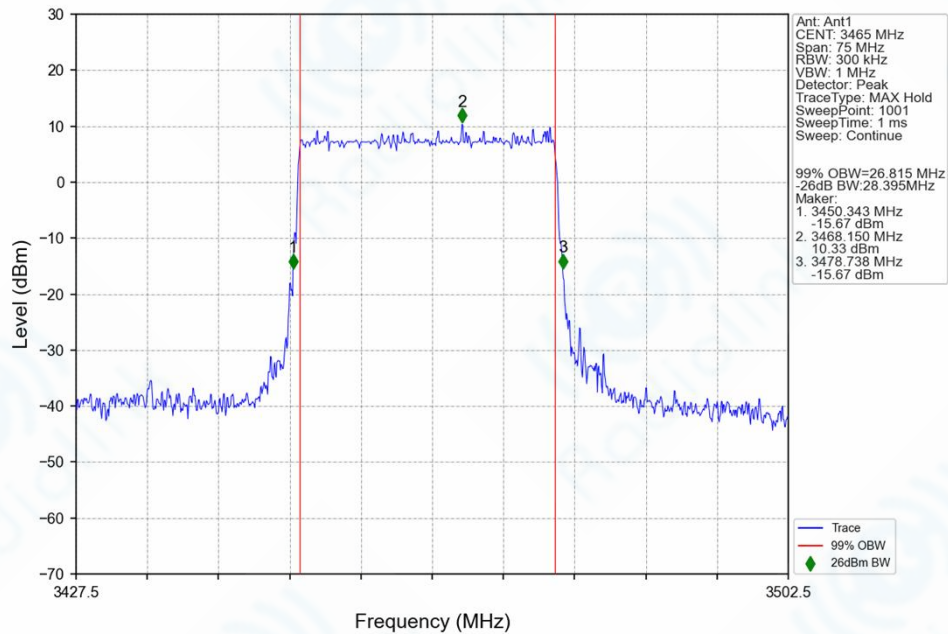
n78f_30kHz_SISO_NTNV_30MHz_DFT-s-OFDM_64_QAM_3465MHz_Outer_Full_Ant1
