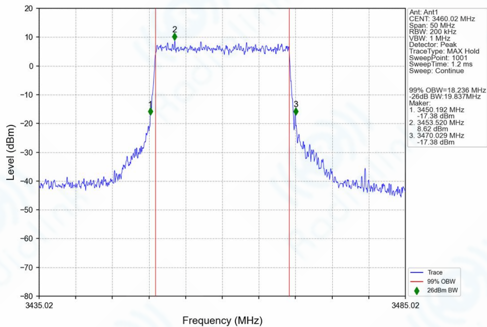
n78f_30kHz_SISO_NTNV_20MHz_CP-OFDM_64_QAM_3460.02MHz_Outer_Full_Ant1
