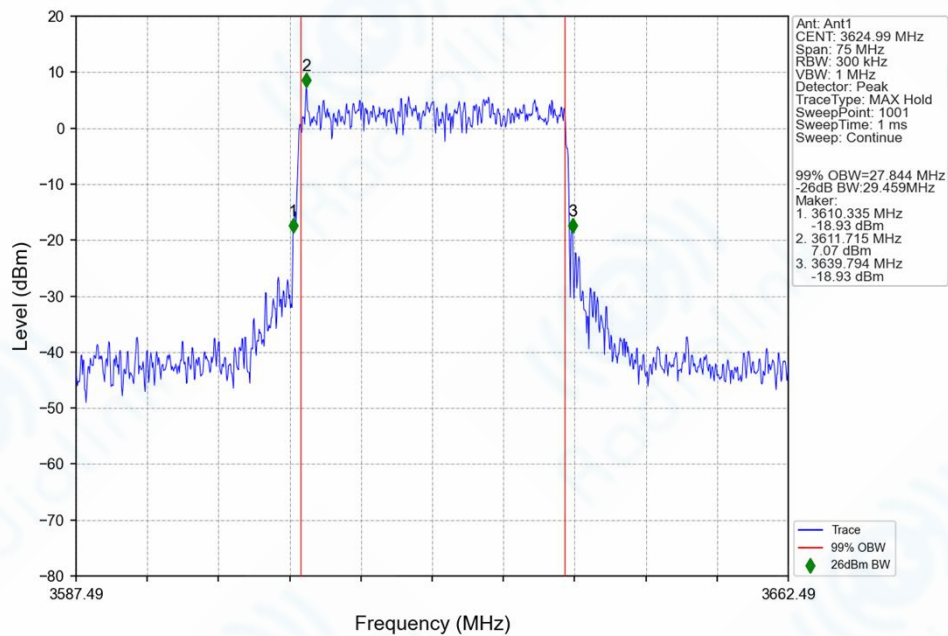
n78f_30kHz_SISO_NTNV_30MHz_CP-OFDM_16_QAM_3624.99MHz_Outer_Full_Ant1
