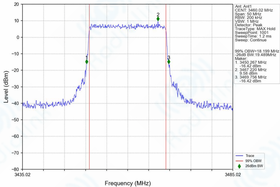
n78f_30kHz_SISO_NTNV_20MHz_CP-OFDM QPSK_3460.02MHz_Outer_Full_Ant1
