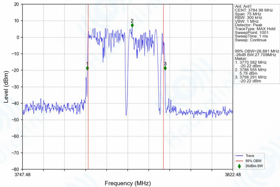
n78f_30kHz_SISO_NTNV_30MHz_DFT-s-OFDM_64_QAM_3784.98MHz_Outer_Full_Ant1
