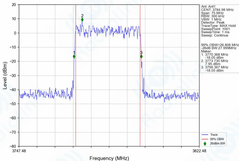
n78f_30kHz_SISO_NTNV_30MHz_DFT-s-OFDM_QPSK_3784.98MHz_Outer_Full_Ant1
