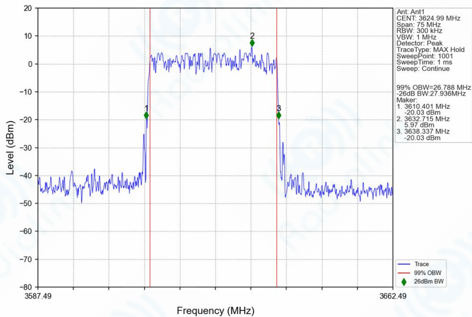
n78f_30kHz_SISO_NTNV_30MHz_DFT-s-OFDM_256_QAM_3624.99MHz_Outer_Full_Ant1
