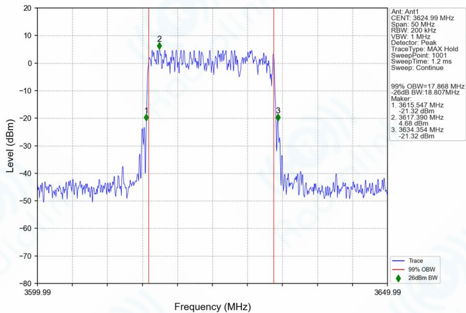
n78f_30kHz_SISO_NTNV_20MHz_DFT-s-OFDM_256_QAM_3624.99MHz_Outer_Full_Ant1
