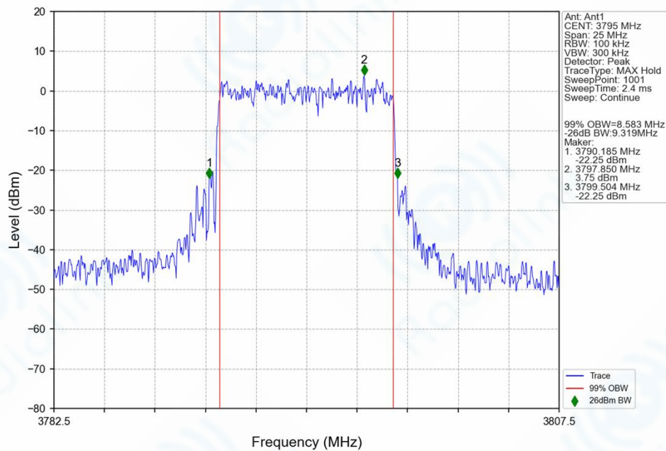
n78f_30kHz_SISO_NTNV_10MHz_CP-OFDM_64_QAM_3795MHz_Outer_Full_Ant1
