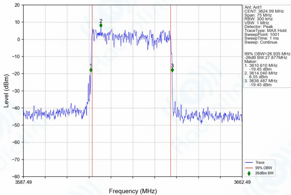
n78f_30kHz_SISO_NTNV_30MHz_DFT-s-OFDM_16_QAM_3624.99MHz_Outer_Full_Ant1
