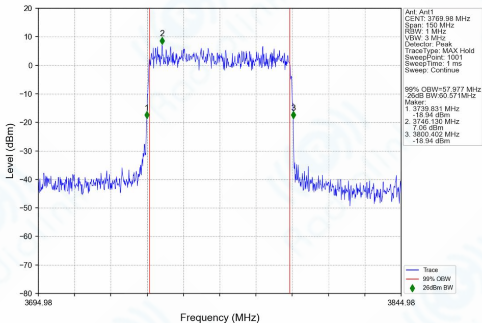
n78f_30kHz_SISO_NTNV_60MHz_DFT-s-OFDM_QPSK_3769.98MHz_Outer_Full_Ant1
