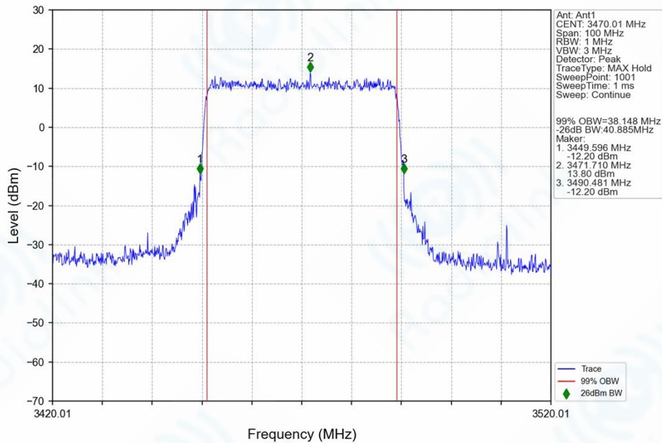
n78f_30kHz_SISO_NTNV_40MHz_CP-OFDM QPSK_3470.01MHz_Outer_Full_Ant1
