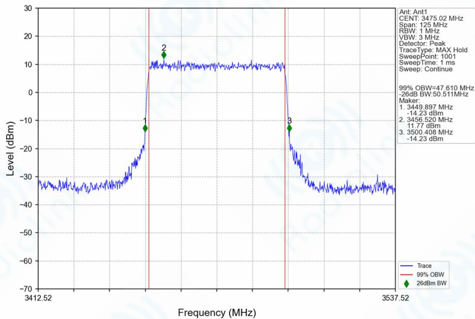
n78f_30kHz_SISO_NTNV_50MHz_CP-OFDM_64_QAM_3475.02MHz_Outer_Full_Ant1
