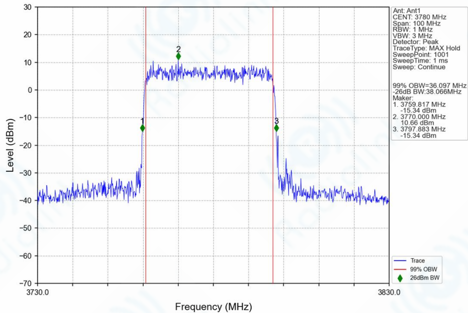
n78f_30kHz_SISO_NTNV_40MHz_DFT-s-OFDM_64_QAM_3780MHz_Outer_Full_Ant1
