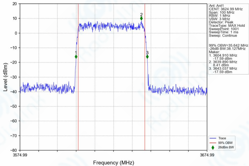
n78f_30kHz_SISO_NTNV_40MHz_DFT-s-OFDM 256 QAM_3624.99MHz_Outer_Full_Ant1
