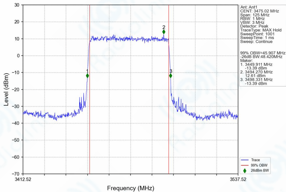
n78f_30kHz_SISO_NTNV_50MHz_DFT-s-OFDM_QPSK_3475.02MHz_Outer_Full_Ant1
