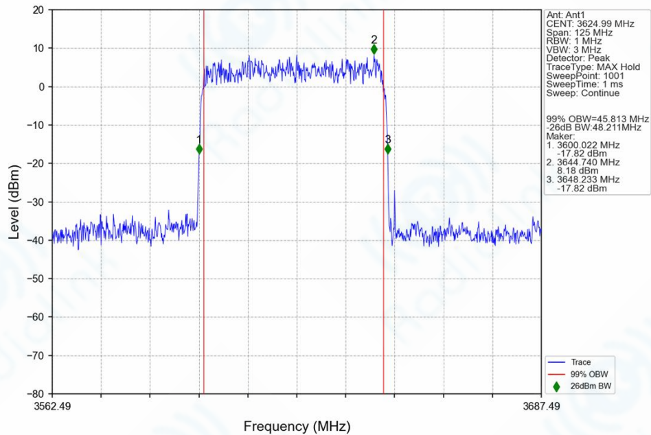
n78f_30kHz_SISO_NTNV_50MHz_DFT-s-OFDM 256 QAM_3624.99MHz_Outer_Full_Ant1
