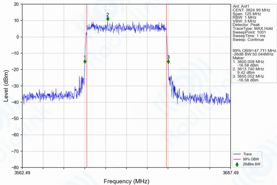
n78f_30kHz_SISO_NTNV_50MHz_CP-OFDM_16_QAM_3624.99MHz_Outer_Full_Ant1
