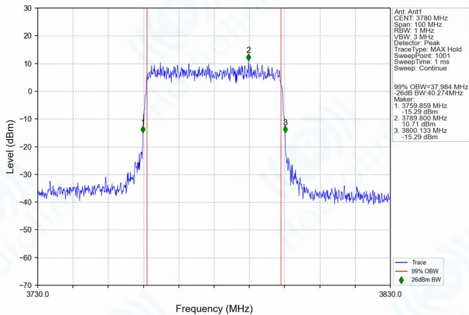
n78f_30kHz_SISO_NTNV_40MHz_CP-OFDM QPSK 3780MHz_Outer_Full_Ant1
