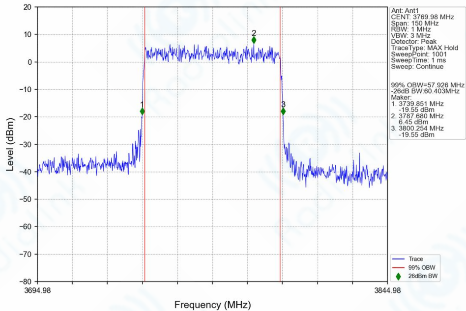
n78f_30kHz_SISO_NTNV_60MHz_CP-OFDM_QPSK_3769.98MHz_Outer_Full_Ant1
