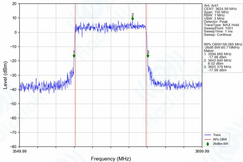
n78f_30kHz_SISO_NTNV_60MHz_CP-OFDM_16_QAM_3624.99MHz_Outer_Full_Ant1
