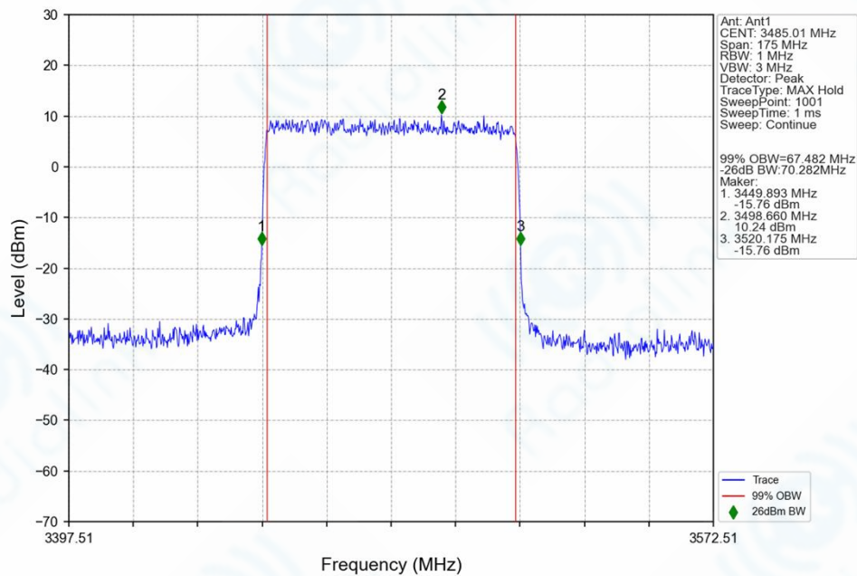
n78f_30kHz_SISO_NTNV_70MHz_CP-OFDM QPSK_3485.01MHz_Outer_Full_Ant1
