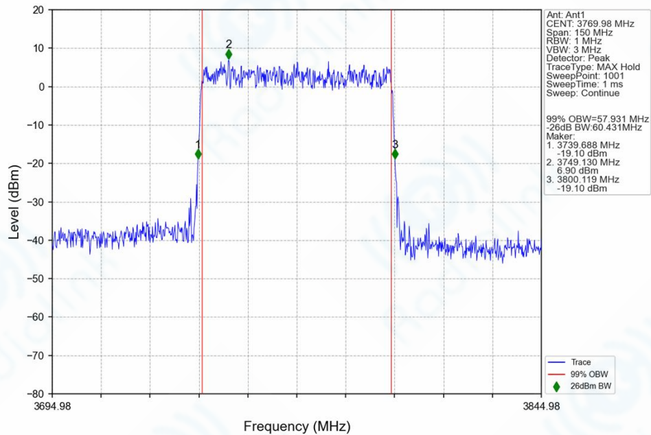
n78f_30kHz_SISO_NTNV_60MHz_DFT-s-OFDM_64_QAM_3769.98MHz_Outer_Full_Ant1
