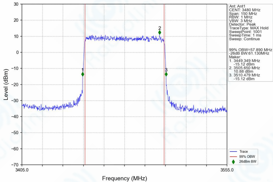
n78f_30kHz_SISO_NTNV_60MHz_DFT-s-OFDM_64_QAM_3480MHz_Outer_Full_Ant1
