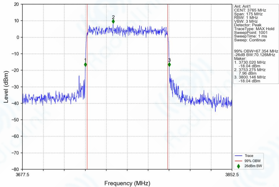
n78f_30kHz_SISO_NTNV_70MHz_CP-OFDM_64_QAM_3765MHz_Outer_Full_Ant1
