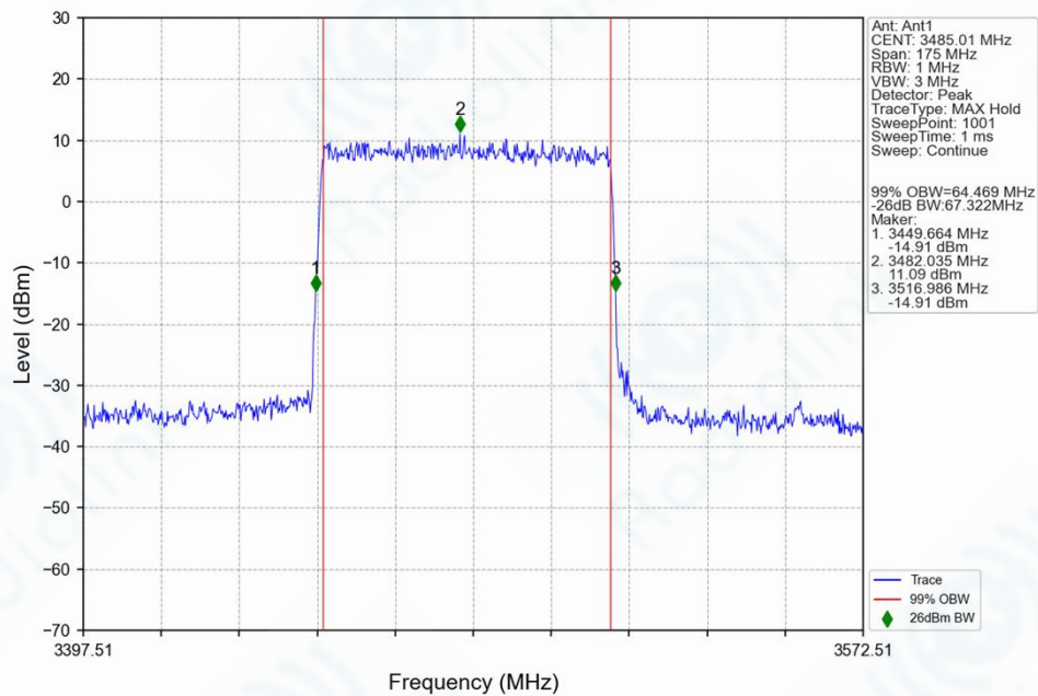
n78f_30kHz_SISO_NTNV_70MHz_DFT-s-OFDM_64_QAM_3485.01MHz_Outer_Full_Ant1
