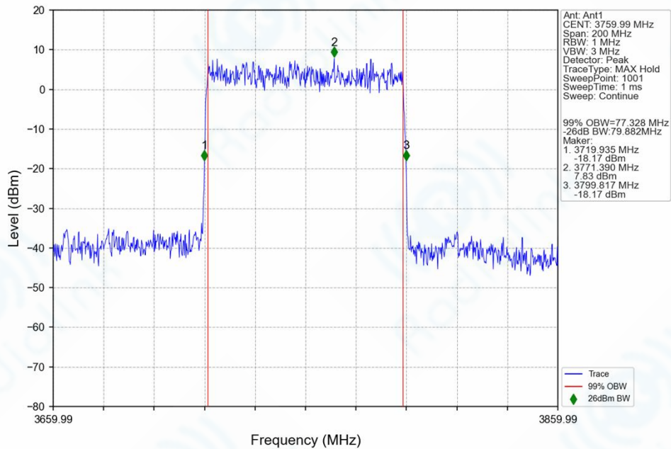
n78f_30kHz_SISO_NTNV_80MHz_DFT-s-OFDM_QPSK_3759.99MHz_Outer_Full_Ant1
