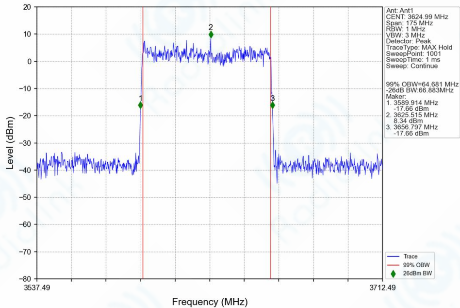
n78f_30kHz_SISO_NTNV_70MHz_DFT-s-OFDM 256 QAM_3624.99MHz_Outer_Full_Ant1
