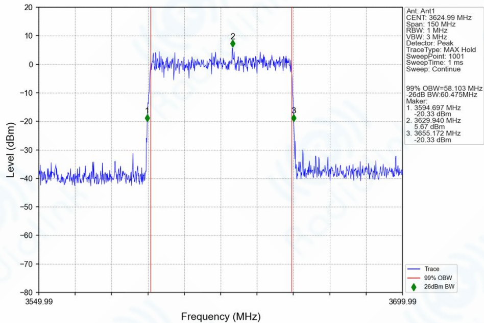
n78f_30kHz_SISO_NTNV_60MHz_CP-OFDM_256_QAM_3624.99MHz_Outer_Full_Ant1
