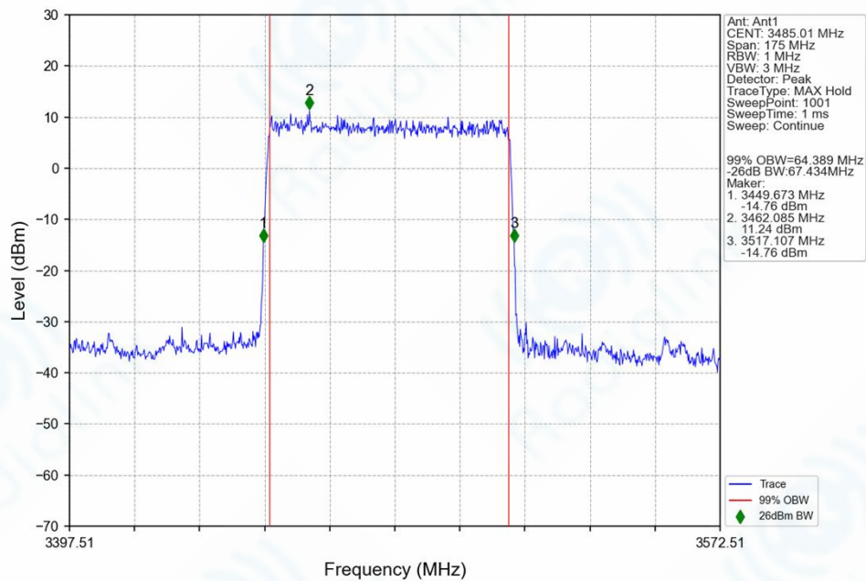
n78f_30kHz_SISO_NTNV_70MHz_DFT-s-OFDM QPSK_3485.01MHz_Outer_Full_Ant1
