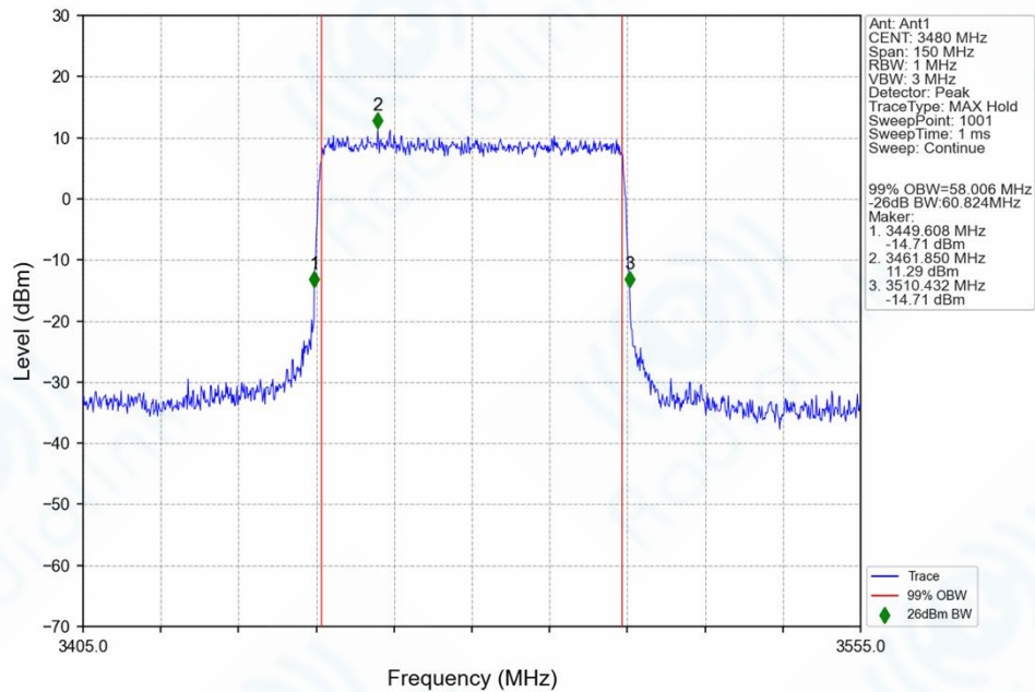
n78f_30kHz_SISO_NTNV_60MHz_CP-OFDM QPSK_3480MHz_Outer_Full_Ant1
