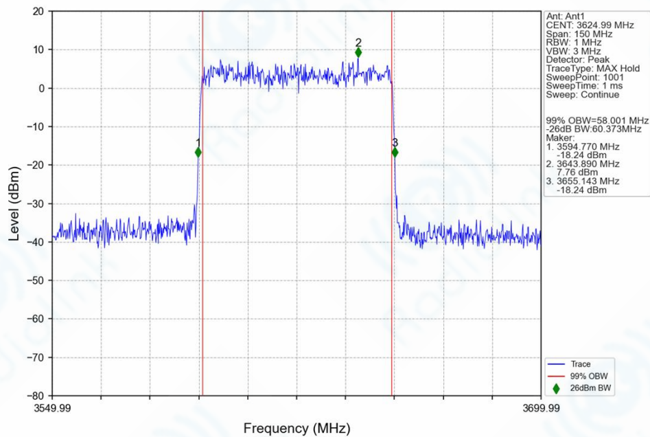
n78f_30kHz_SISO_NTNV_60MHz_DFT-s-OFDM_16_QAM_3624.99MHz_Outer_Full_Ant1
