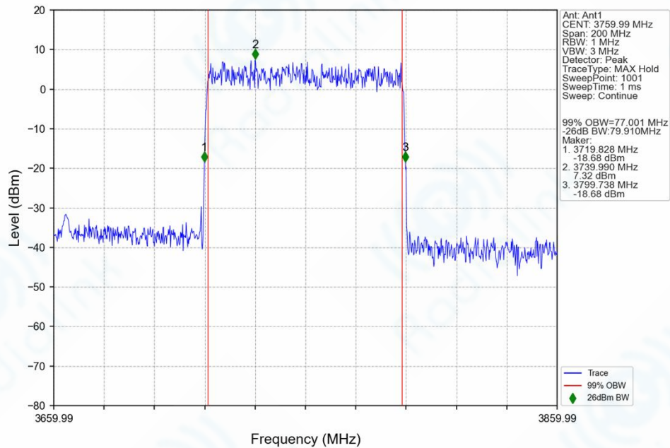
n78f_30kHz_SISO_NTNV_80MHz_DFT-s-OFDM_64_QAM_3759.99MHz_Outer_Full_Ant1
