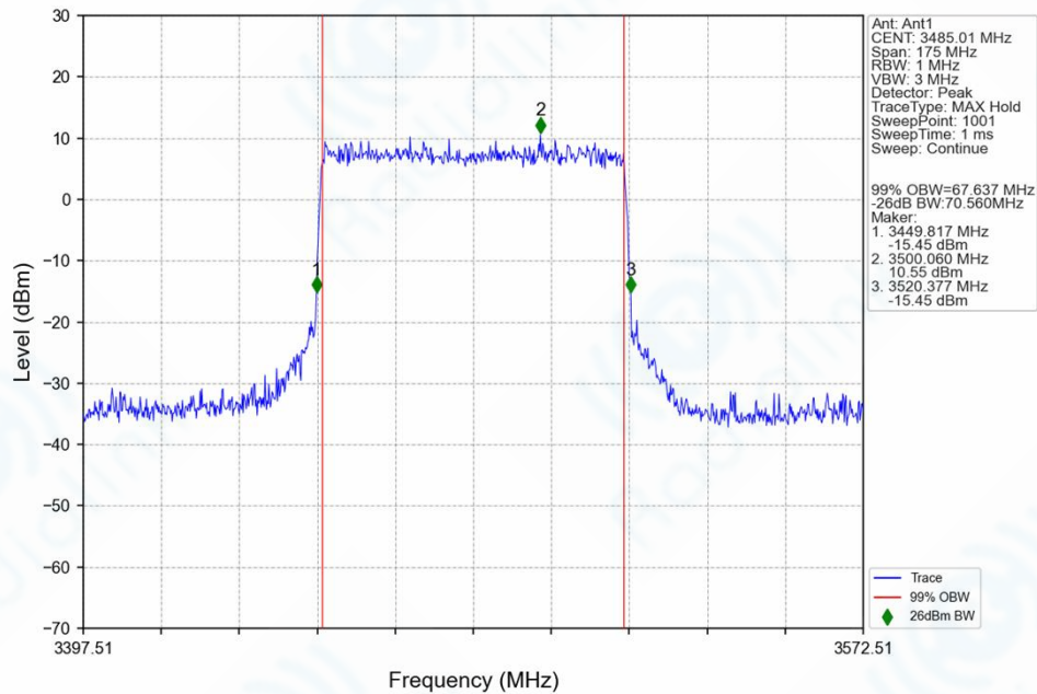
n78f_30kHz_SISO_NTNV_70MHz_CP-OFDM_64_QAM_3485.01MHz_Outer_Full_Ant1
