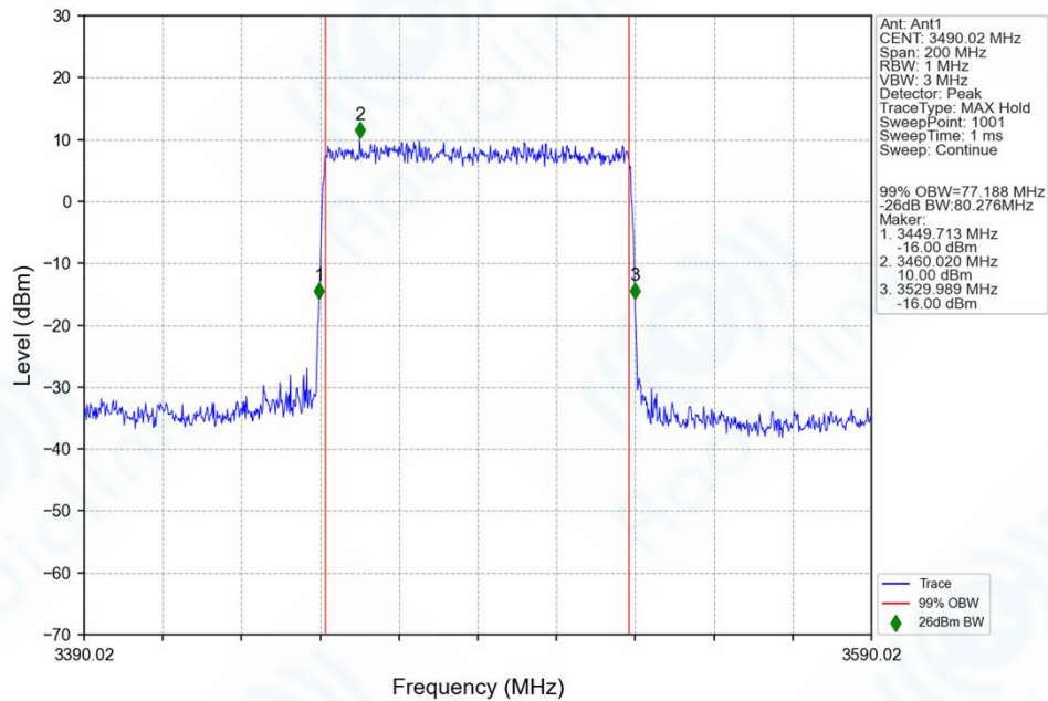
n78f_30kHz_SISO_NTNV_80MHz_DFT-s-OFDM_QPSK_3490.02MHz_Outer_Full_Ant1
