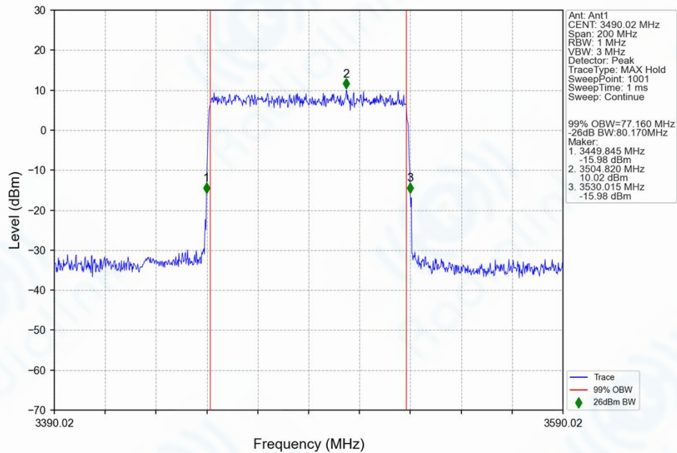
n78f_30kHz_SISO_NTNV_80MHz_DFT-s-OFDM_64_QAM_3490.02MHz_Outer_Full_Ant1
