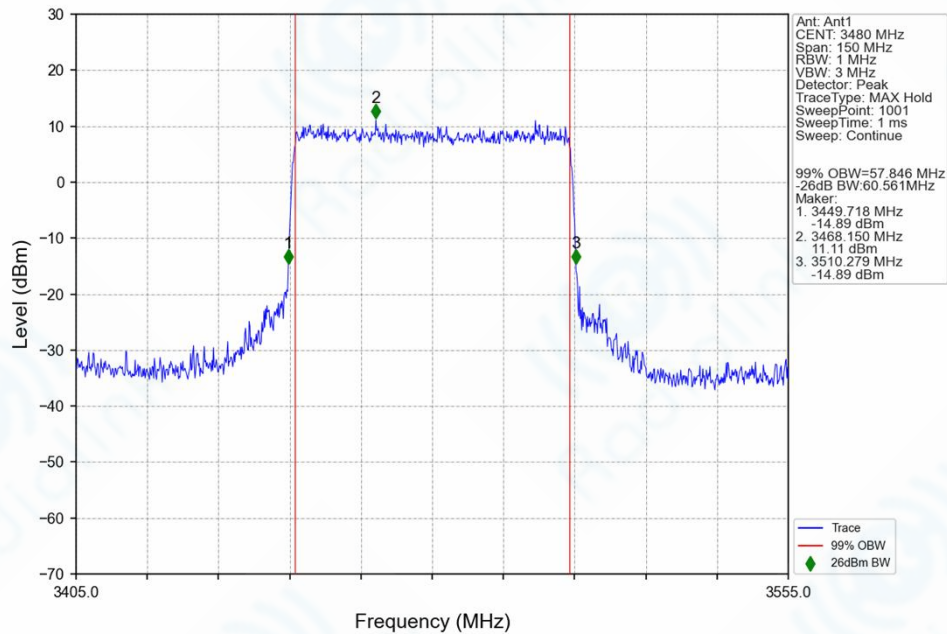
n78f_30kHz_SISO_NTNV_60MHz_CP-OFDM_64 QAM_3480MHz_Outer_Full_Ant1
