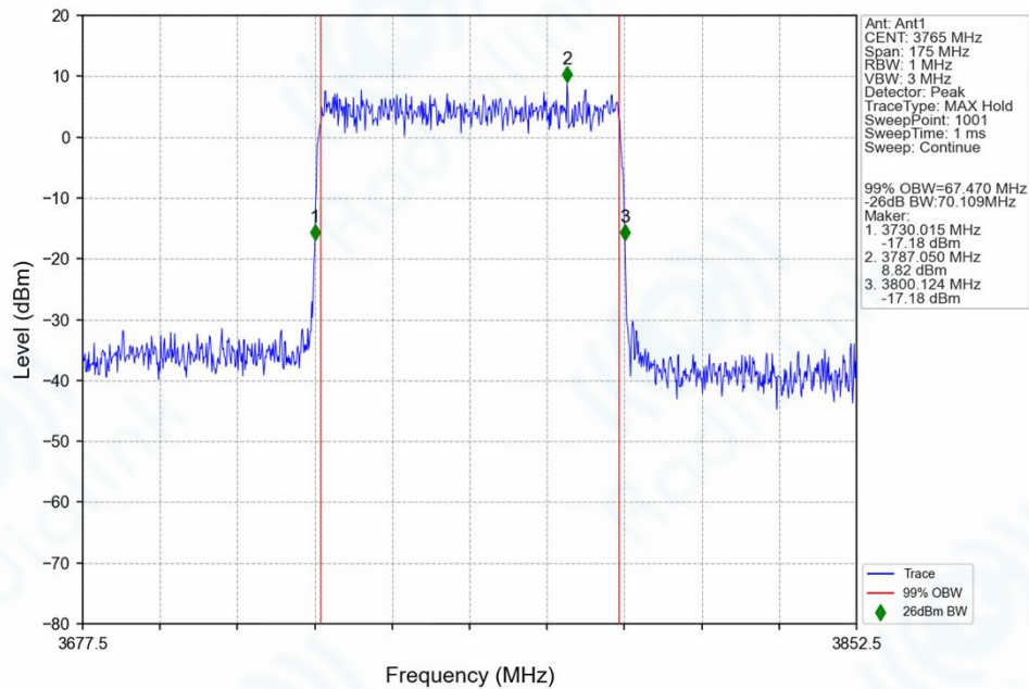
n78f_30kHz_SISO_NTNV_70MHz_CP-OFDM QPSK 3765MHz_Outer_Full_Ant1
