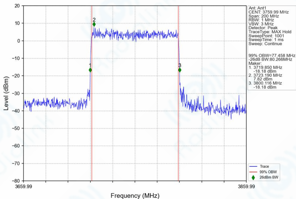
n78f_30kHz_SISO_NTNV_80MHz_CP-OFDM_64_QAM_3759.99MHz_Outer_Full_Ant1
