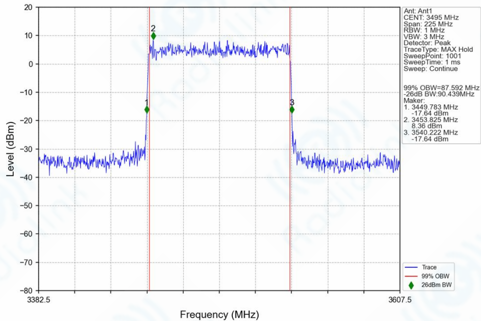
n78f_30kHz_SISO_NTNV_90MHz_CP-OFDM_64 QAM_3495MHz_Outer_Full_Ant1
