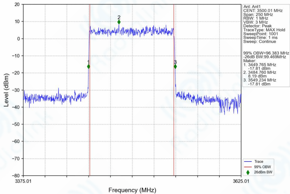
n78f_30kHz_SISO_NTNV_100MHz_DFT-s-OFDM 64 QAM_3500.01MHz_Outer_Full_Ant1
