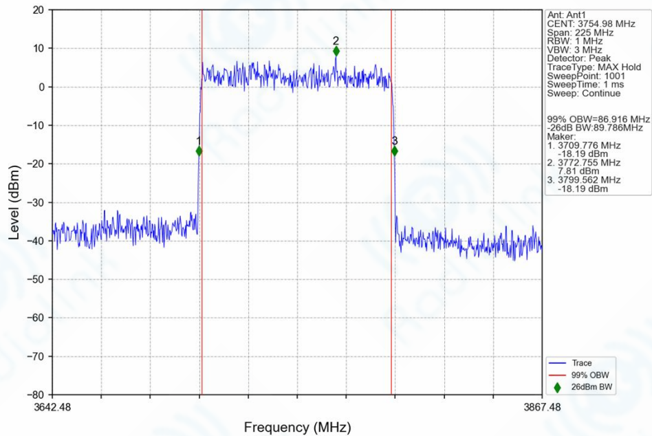
n78f_30kHz_SISO_NTNV_90MHz_DFT-s-OFDM_64_QAM_3754.98MHz_Outer_Full_Ant1
