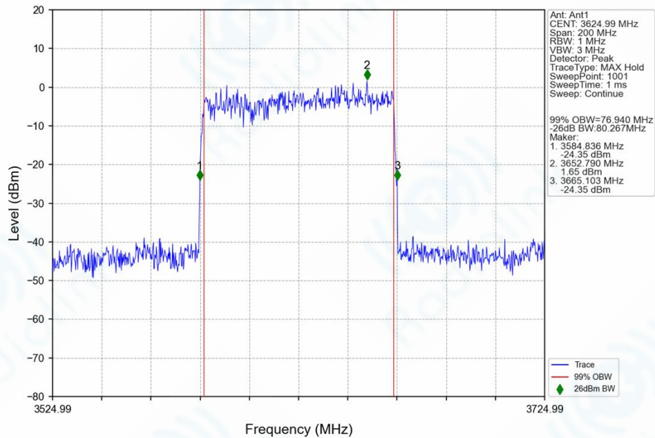
n78f_30kHz_SISO_NTNV_80MHz_DFT-s-OFDM_256_QAM_3624.99MHz_Outer_Full_Ant1
