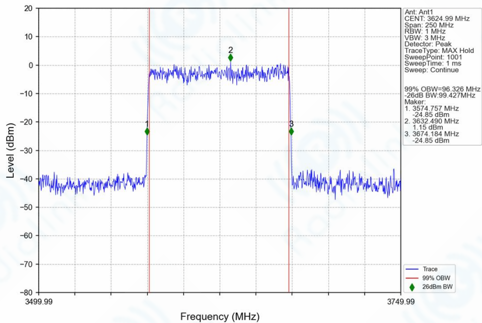
n78f_30kHz_SISO_NTNV_100MHz_DFT-s-OFDM 16 QAM_3624.99MHz_Outer_Full_Ant1
