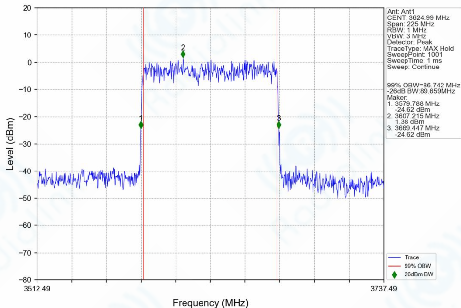
n78f_30kHz_SISO_NTNV_90MHz_DFT-s-OFDM_16_QAM_3624.99MHz_Outer_Full_Ant1
