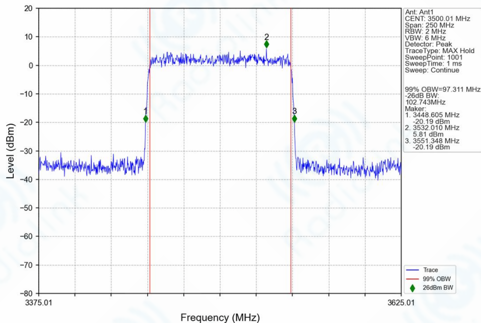
n78f_30kHz_SISO_NTNV_100MHz_CP-OFDM_QPSK_3500.01MHz_Outer_Full_Ant1
