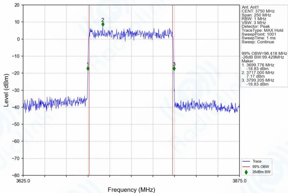
n78f_30kHz_SISO_NTNV_100MHz_DFT-s-OFDM_QPSK_3750MHz_Outer_Full_Ant1
