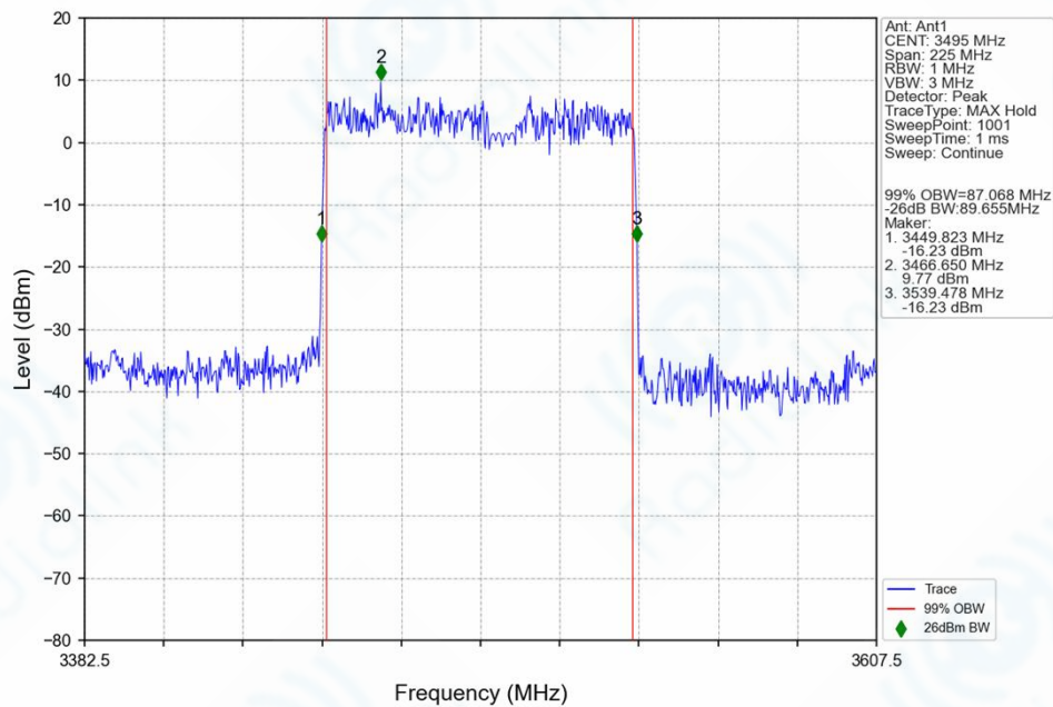
n78f_30kHz_SISO_NTNV_90MHz_DFT-s-OFDM_QPSK_3495MHz_Outer_Full_Ant1
