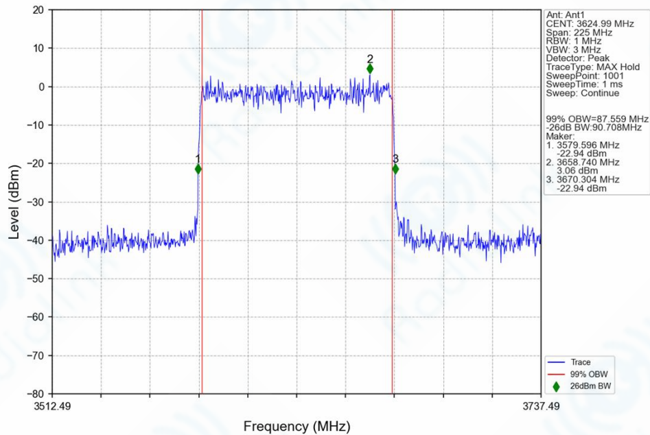
n78f_30kHz_SISO_NTNV_90MHz_CP-OFDM_16_QAM_3624.99MHz_Outer_Full_Ant1
