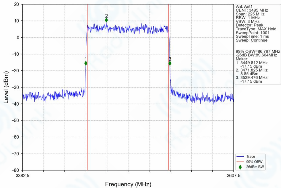
n78f_30kHz_SISO_NTNV_90MHz_DFT-s-OFDM_64_QAM_3495MHz_Outer_Full_Ant1
