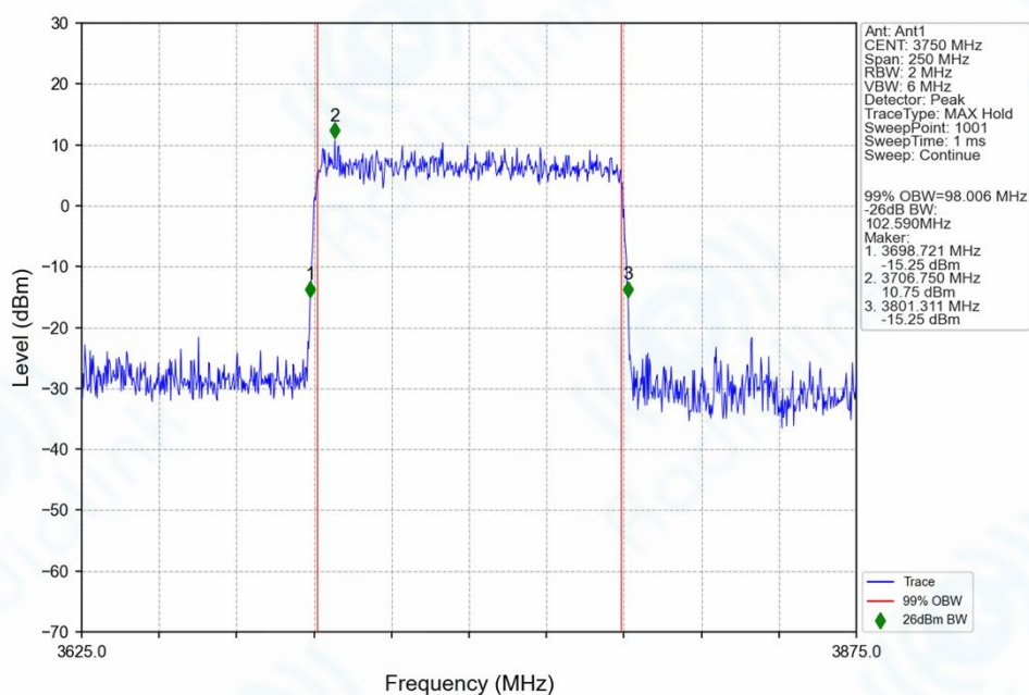
n78f_30kHz_SISO_NTNV_100MHz_CP-OFDM_QPSK_3750MHz_Outer_Full_Ant1
