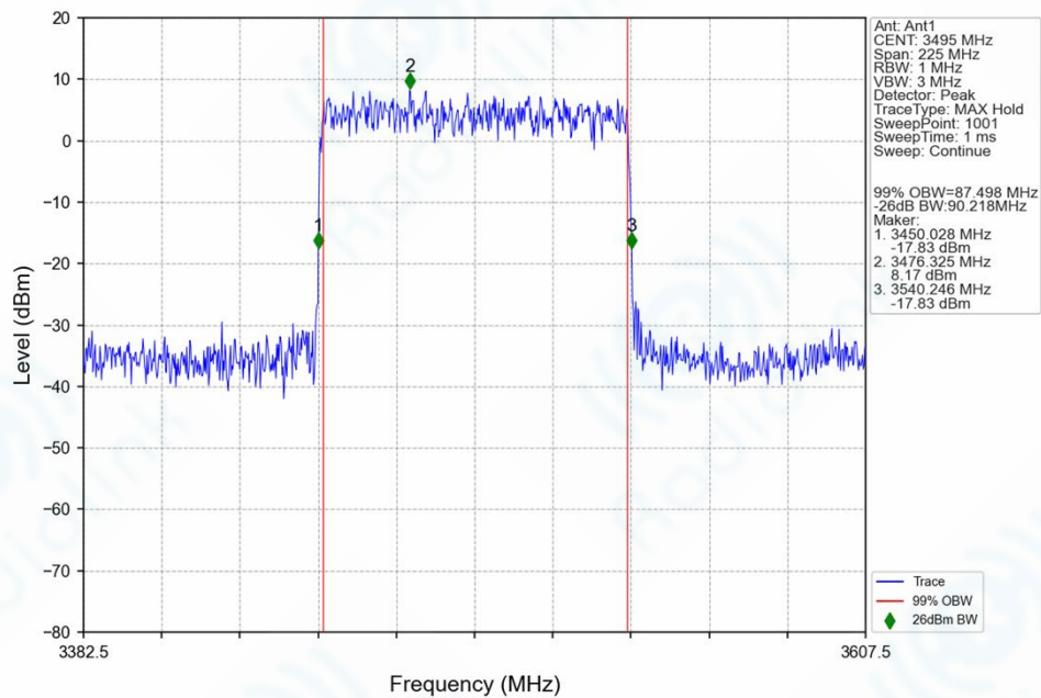
n78f_30kHz_SISO_NTNV_90MHz_CP-OFDM QPSK_3495MHz_Outer_Full_Ant1
