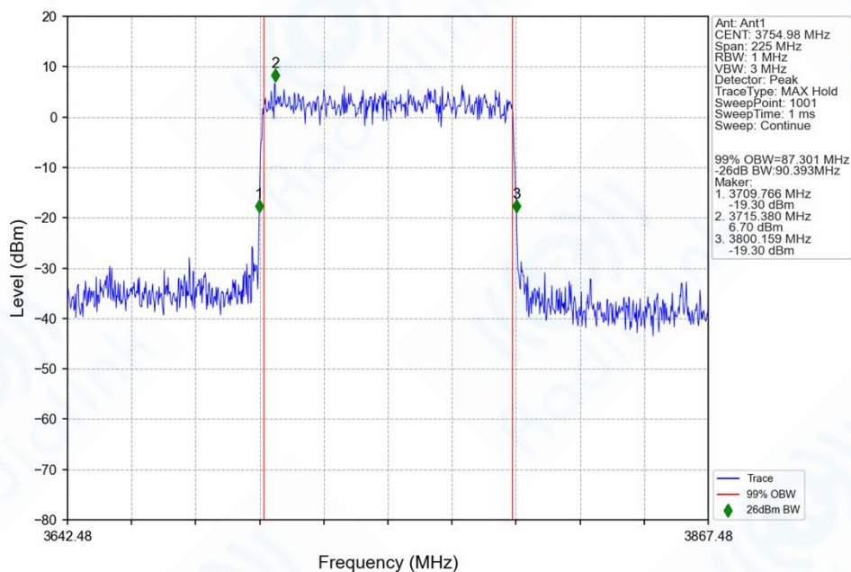
n78f_30kHz_SISO_NTNV_90MHz_CP-OFDM_64_QAM_3754.98MHz_Outer_Full_Ant1
