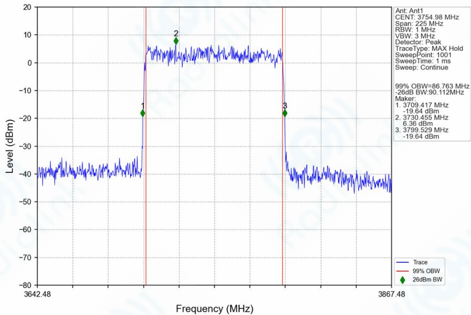
n78f_30kHz_SISO_NTNV_90MHz_DFT-s-OFDM_QPSK_3754.98MHz_Outer_Full_Ant1
