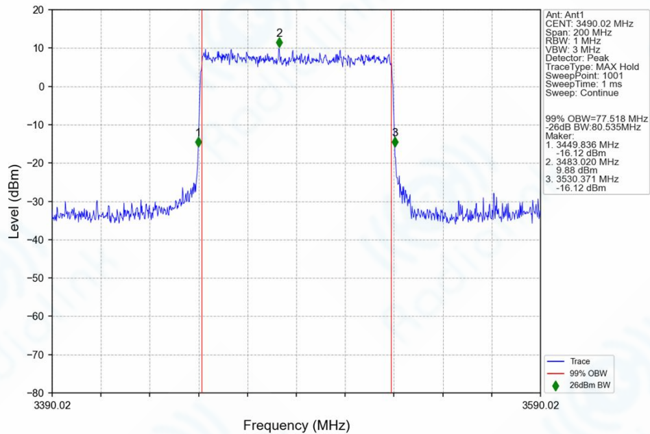
n78f_30kHz_SISO_NTNV_80MHz_CP-OFDM_64_QAM_3490.02MHz_Outer_Full_Ant1
