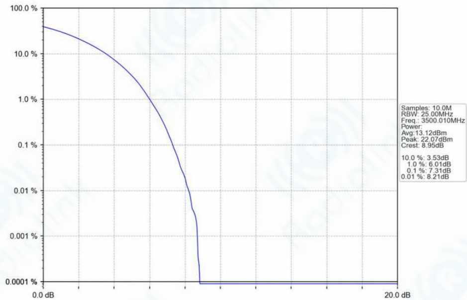
n78f_30kHz_SISO_NTNV_100MHz_DFT-s-OFDM QPSK 3500.01MHz_Outer_Full_Ant1
