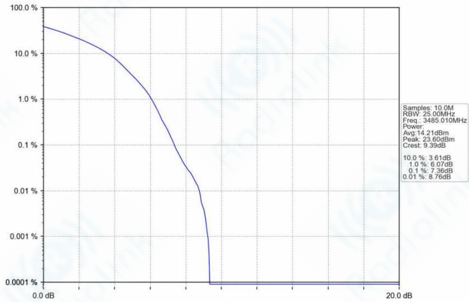
n78f_30kHz_SISO_NTNV_70MHz_DFT-s-OFDM_16_QAM_3485.01MHz_Outer_Full_Ant1
