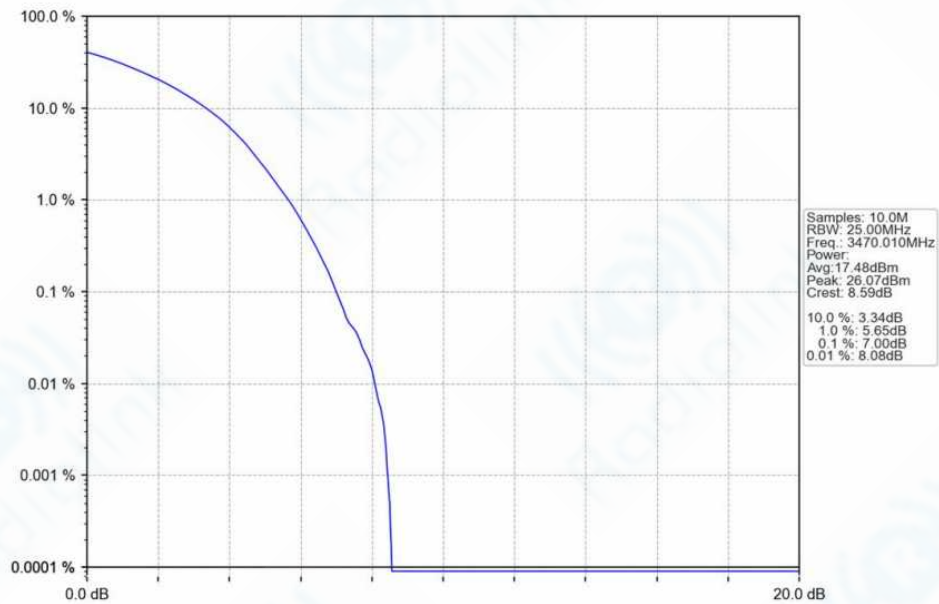
n78f_30kHz_SISO_NTNV_40MHz_DFT-s-OFDM_64_QAM_3470.01MHz_Outer_Full_Ant1
