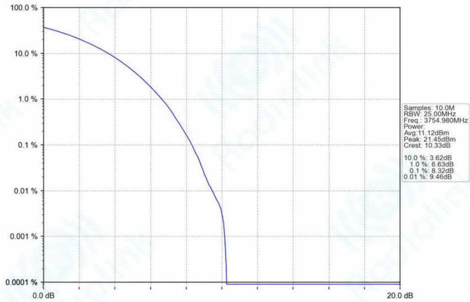
n78f_30kHz_SISO_NTNV_90MHz_CP-OFDM 16 QAM_3754.98MHz_Outer_Full_Ant1
