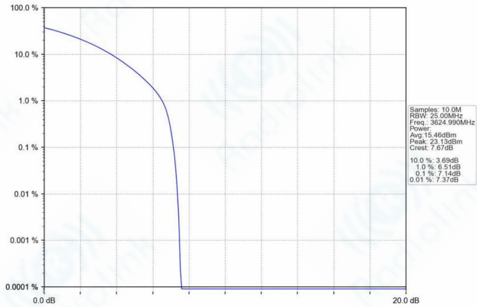
n78f_30kHz_SISO_NTNV_20MHz_CP-OFDM_64_QAM_3624.99MHz_Outer_Full_Ant1
