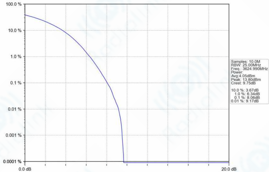
n78f_30kHz_SISO_NTNV_100MHz_DFT-s-OFDM_256_QAM_3624.99MHz_Outer_Full_Ant1
