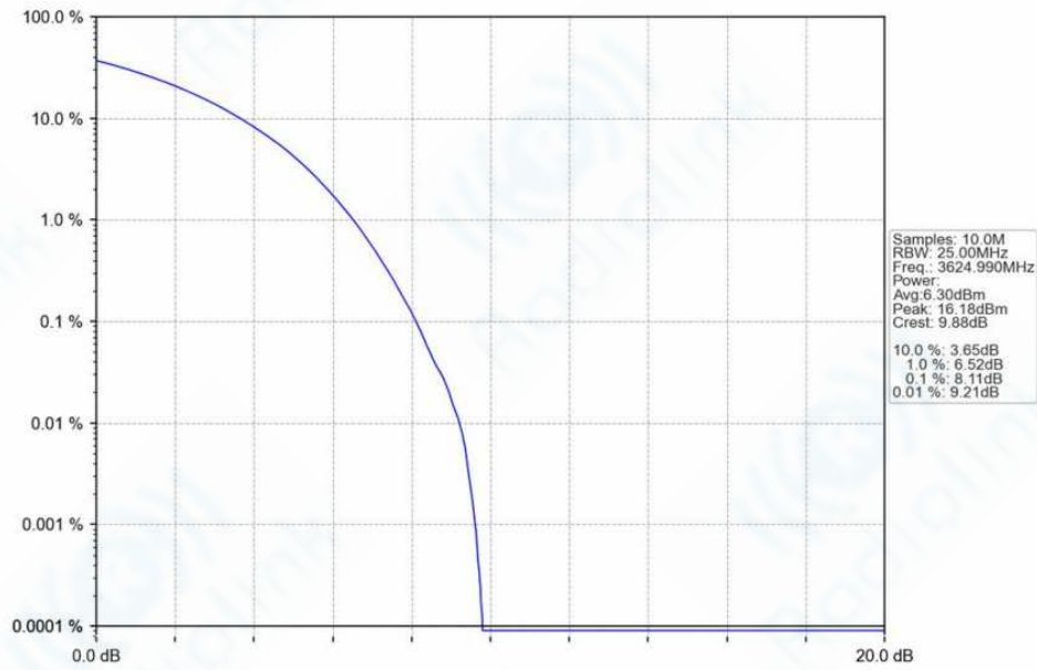
n78f_30kHz_SISO_NTNV_80MHz_CP-OFDM_QPSK_3624.99MHz_Outer_Full_Ant1
