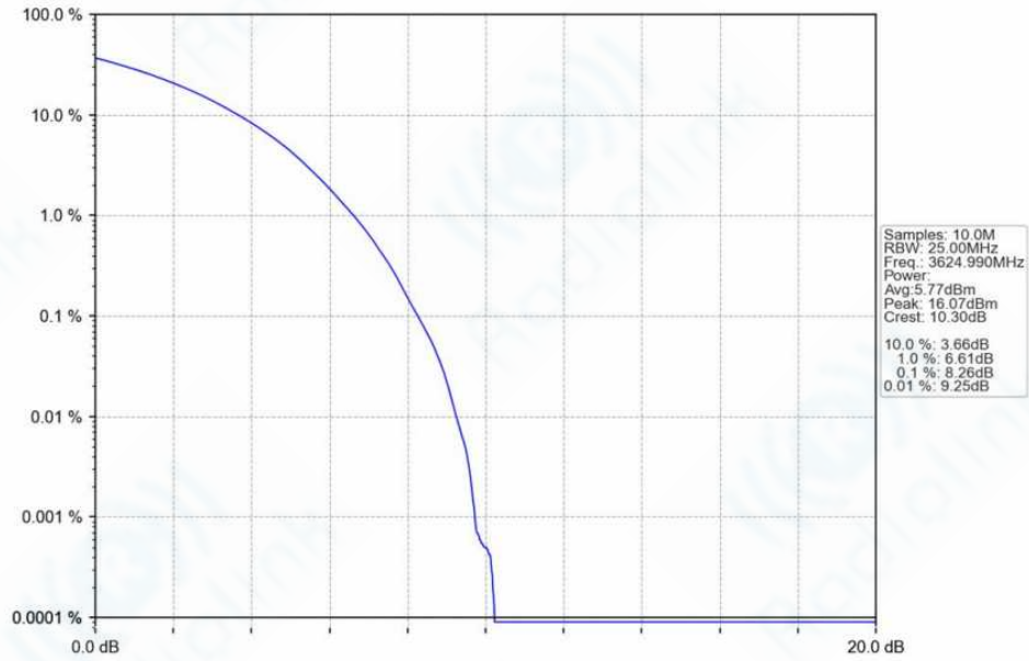
n78f_30kHz_SISO_NTNV_100MHz_CP-OFDM_QPSK_3624.99MHz_Outer_Full_Ant1
