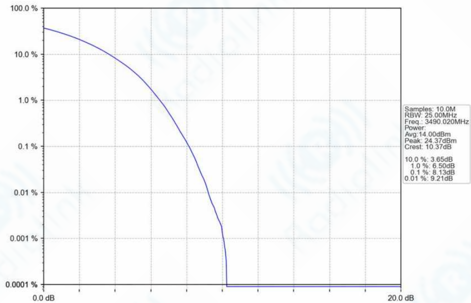
n78f_30kHz_SISO_NTNV_80MHz_CP-OFDM QPSK_3490.02MHz_Outer_Full_Ant1
