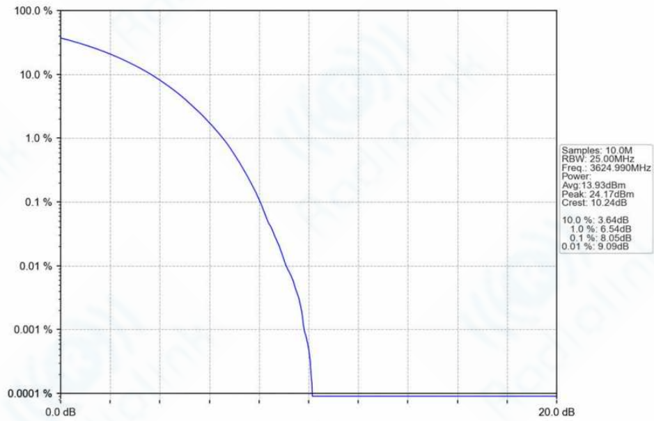
n78f_30kHz_SISO_NTNV_50MHz_CP-OFDM QPSK_3624.99MHz_Outer_Full_Ant1
