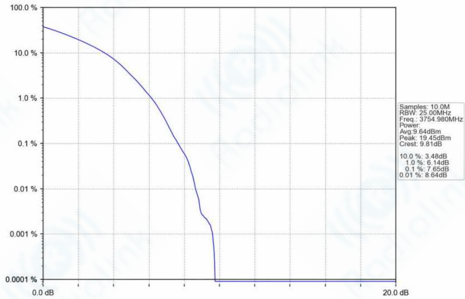
n78f_30kHz_SISO_NTNV_90MHz_DFT-s-OFDM 256 QAM_3754.98MHz_Outer_Full_Ant1
