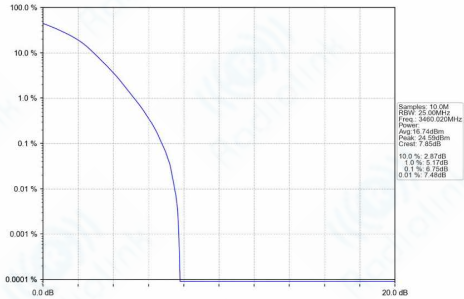
n78f_30kHz_SISO_NTNV_20MHz_DFT-s-OFDM 256 QAM_3460.02MHz_Outer_Full_Ant1
