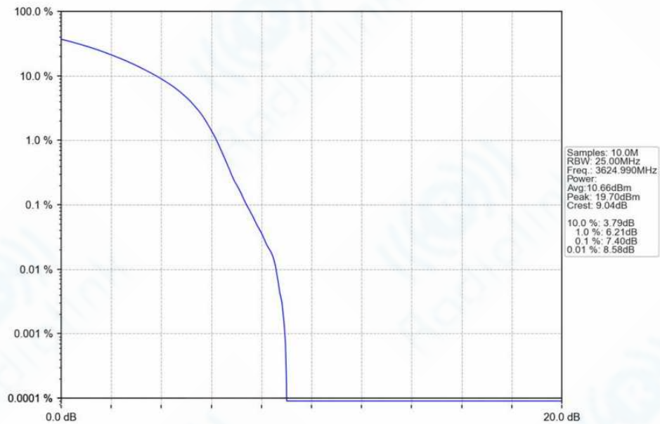
n78f_30kHz_SISO_NTNV_60MHz_DFT-s-OFDM_256_QAM_3624.99MHz_Outer_Full_Ant1
