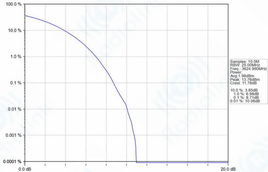
n78f_30kHz_SISO_NTNV_90MHz_CP-OFDM_256_QAM_3624.99MHz_Outer_Full_Ant1
