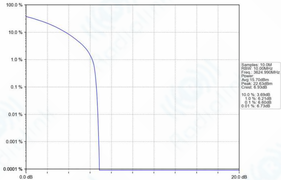
n78f_30kHz_SISO_NTNV_10MHz_CP-OFDM_16_QAM_3624.99MHz_Outer_Full_Ant1
