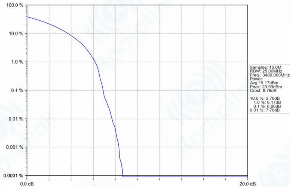
n78f_30kHz_SISO_NTNV_60MHz_DFT-s-OFDM_QPSK_3480MHz_Outer_Full_Ant1
