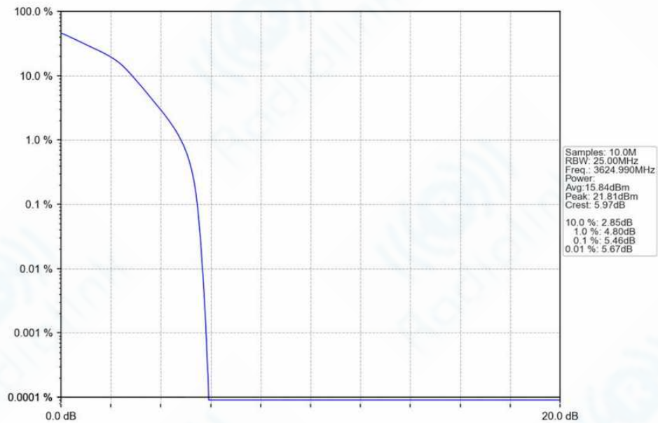
n78f_30kHz_SISO_NTNV_20MHz_DFT-s-OFDM_16_QAM_3624.99MHz_Outer_Full_Ant1
