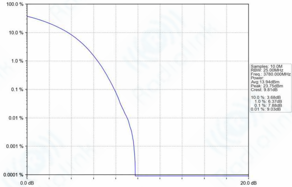
n78f_30kHz_SISO_NTNV_40MHz_CP-OFDM_16_QAM_3780MHz_Outer_Full_Ant1
