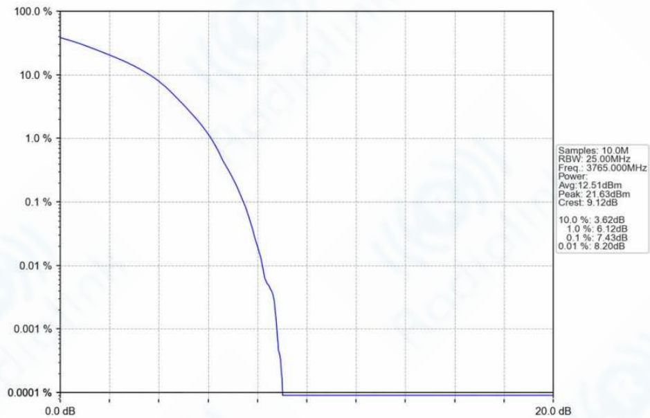
n78f_30kHz_SISO_NTNV_70MHz_DFT-s-OFDM_64_QAM_3765MHz_Outer_Full_Ant1
