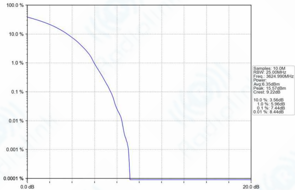
n78f_30kHz_SISO_NTNV_80MHz_DFT-s-OFDM_16_QAM_3624.99MHz_Outer_Full_Ant1
