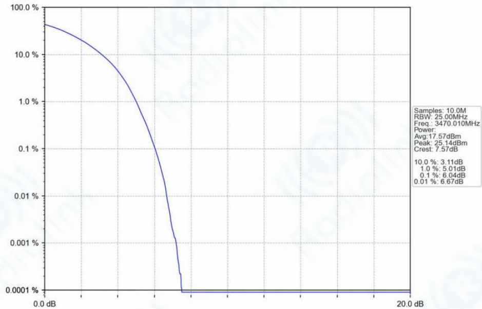
n78f_30kHz_SISO_NTNV_40MHz_DFT-s-OFDM_QPSK_3470.01MHz_Outer_Full_Ant1
