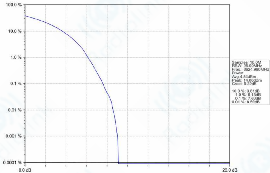
n78f_30kHz_SISO_NTNV_80MHz_DFT-s-OFDM 256 QAM_3624.99MHz_Outer_Full_Ant1
