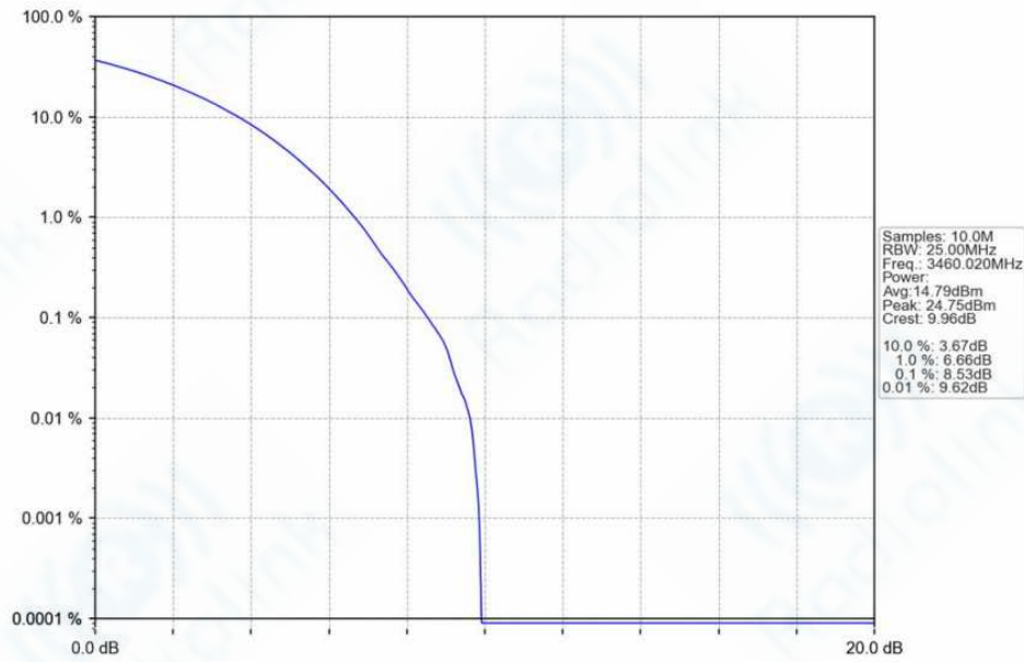
n78f_30kHz_SISO_NTNV_20MHz_CP-OFDM_256_QAM_3460.02MHz_Outer_Full_Ant1
