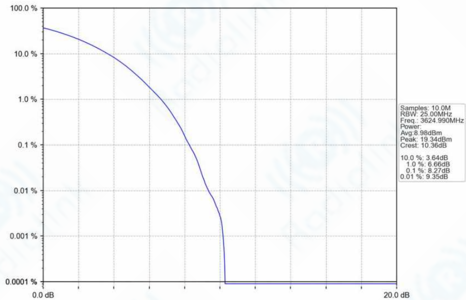
n78f_30kHz_SISO_NTNV_70MHz_CP-OFDM_256_QAM_3624.99MHz_Outer_Full_Ant1
