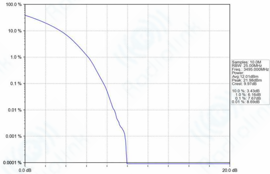
n78f_30kHz_SISO_NTNV_90MHz_DFT-s-OFDM_256_QAM_3495MHz_Outer_Full_Ant1
