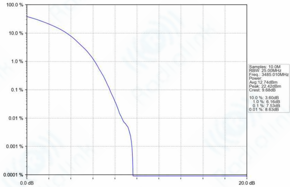
n78f_30kHz_SISO_NTNV_70MHz_DFT-s-OFDM_256_QAM_3485.01MHz_Outer_Full_Ant1
