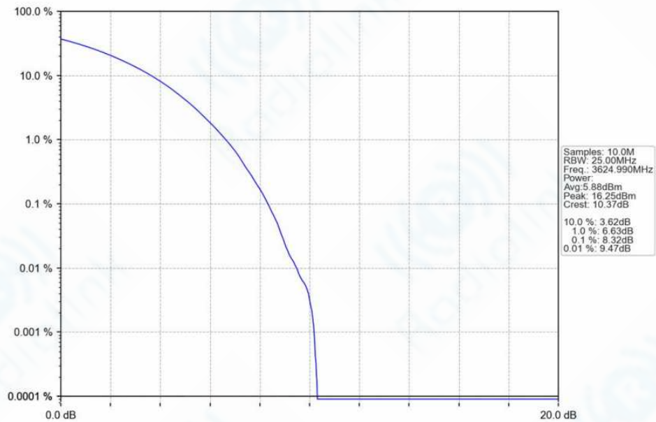
n78f_30kHz_SISO_NTNV_90MHz_CP-OFDM_16_QAM_3624.99MHz_Outer_Full_Ant1
