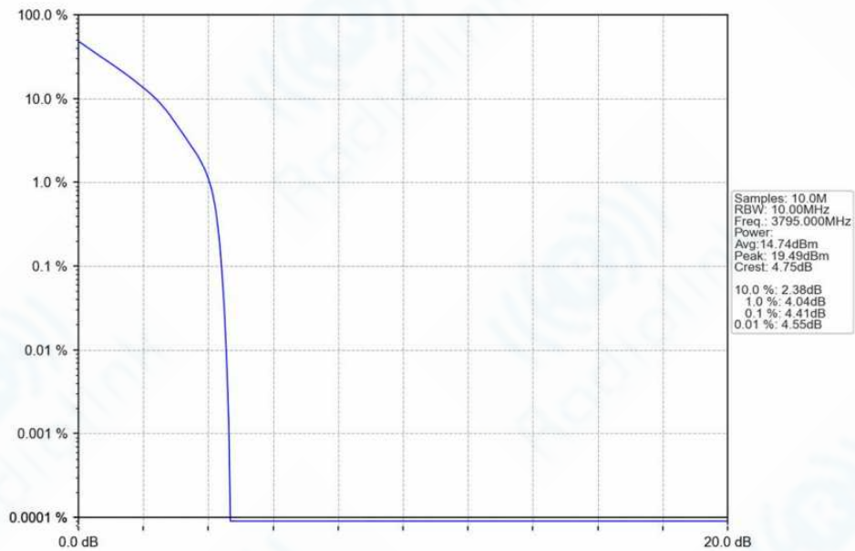
n78f_30kHz_SISO_NTNV_10MHz_DFT-s-OFDM QPSK_3795MHz_Outer_Full_Ant1
