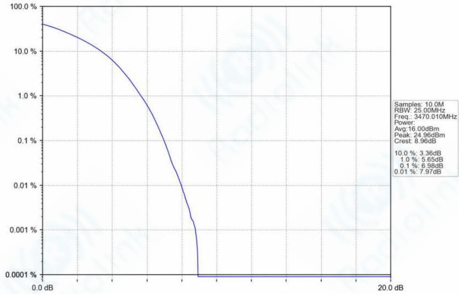
n78f_30kHz_SISO_NTNV_40MHz_DFT-s-OFDM_256_QAM_3470.01MHz_Outer_Full_Ant1
