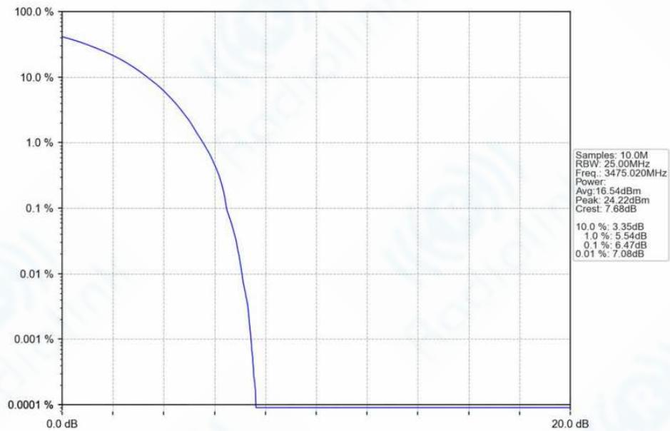
n78f_30kHz_SISO_NTNV_50MHz_DFT-s-OFDM_QPSK_3475.02MHz_Outer_Full_Ant1
