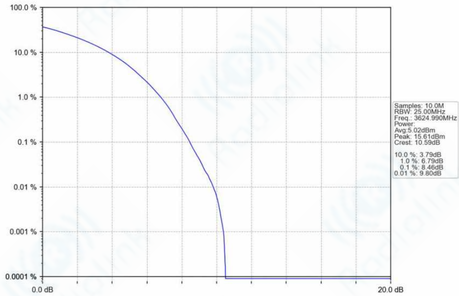
n78f_30kHz_SISO_NTNV_100MHz_CP-OFDM 64 QAM_3624.99MHz_Outer_Full_Ant1
