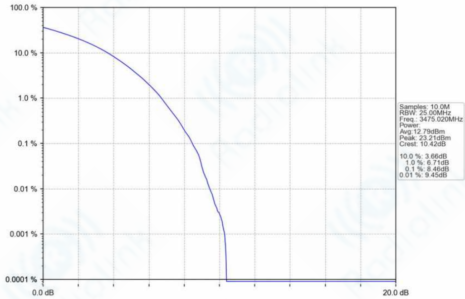
n78f_30kHz_SISO_NTNV_50MHz_CP-OFDM_256_QAM_3475.02MHz_Outer_Full_Ant1
