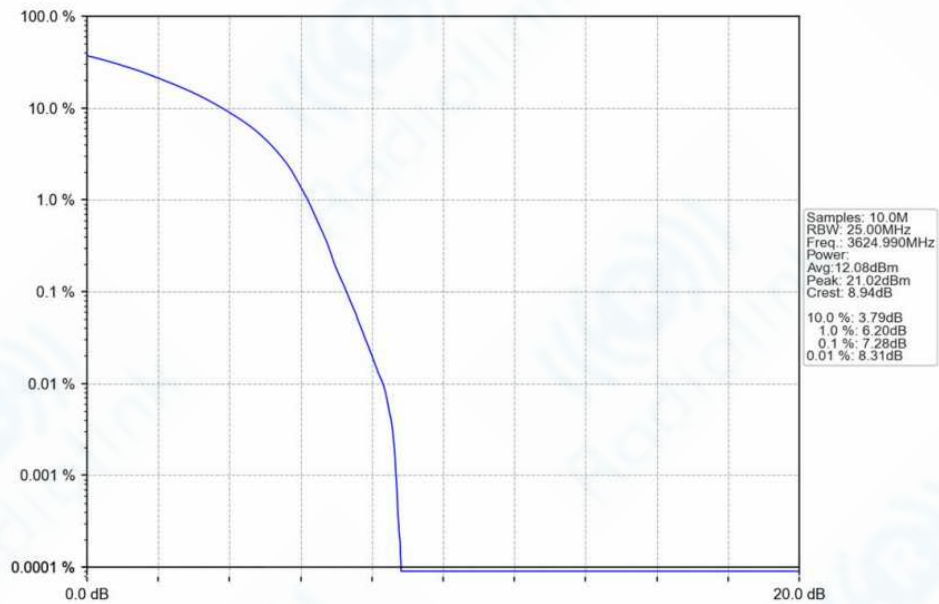
n78f_30kHz_SISO_NTNV_60MHz_DFT-s-OFDM_16_QAM_3624.99MHz_Outer_Full_Ant1
