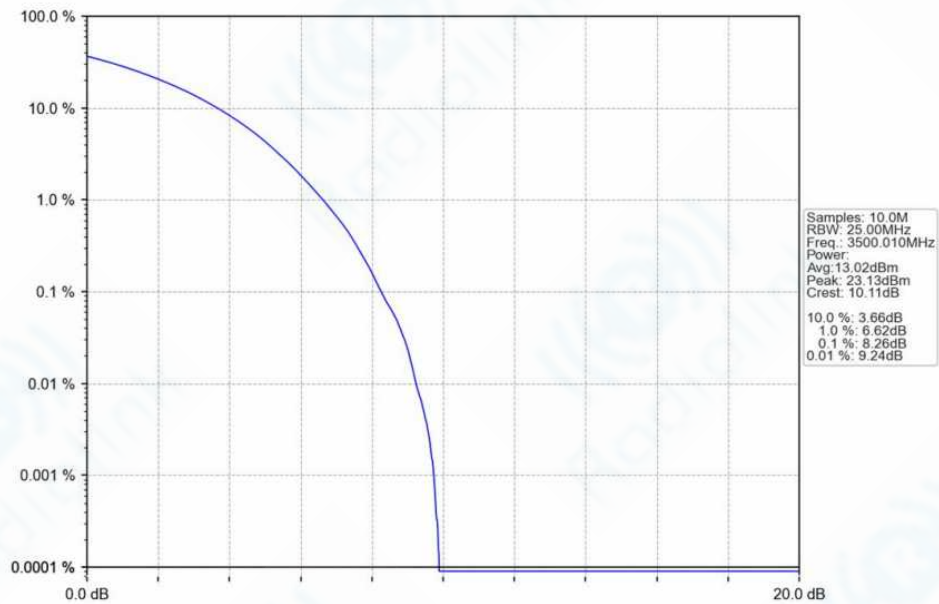
n78f_30kHz_SISO_NTNV_100MHz_CP-OFDM_QPSK_3500.01MHz_Outer_Full_Ant1
