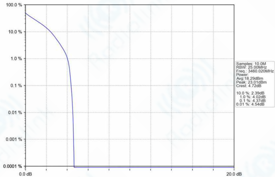
n78f_30kHz_SISO_NTNV_20MHz_DFT-s-OFDM_QPSK_3460.02MHz_Outer_Full_Ant1
