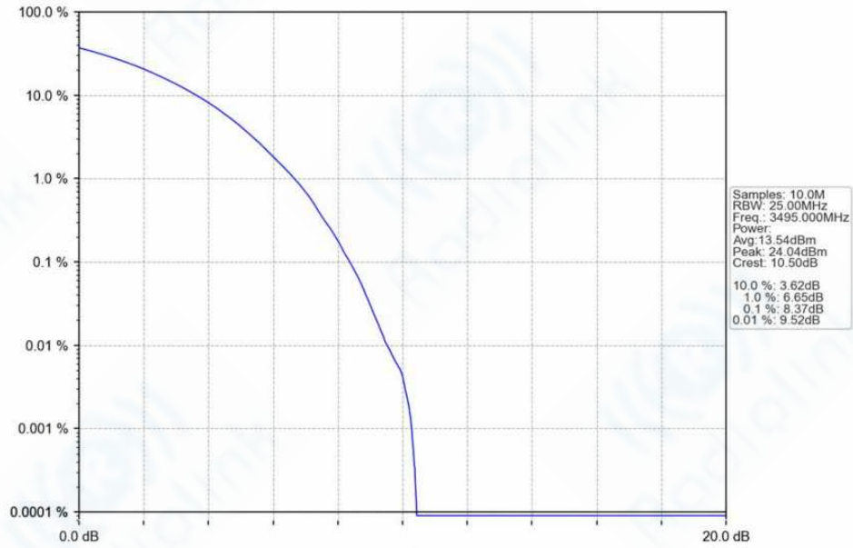
n78f_30kHz_SISO_NTNV_90MHz_CP-OFDM_16_QAM_3495MHz_Outer_Full_Ant1
