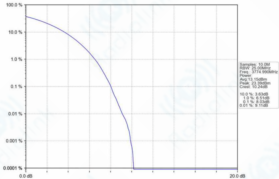
n78f_30kHz_SISO_NTNV_50MHz_CP-OFDM QPSK_3774.99MHz_Outer_Full_Ant1
