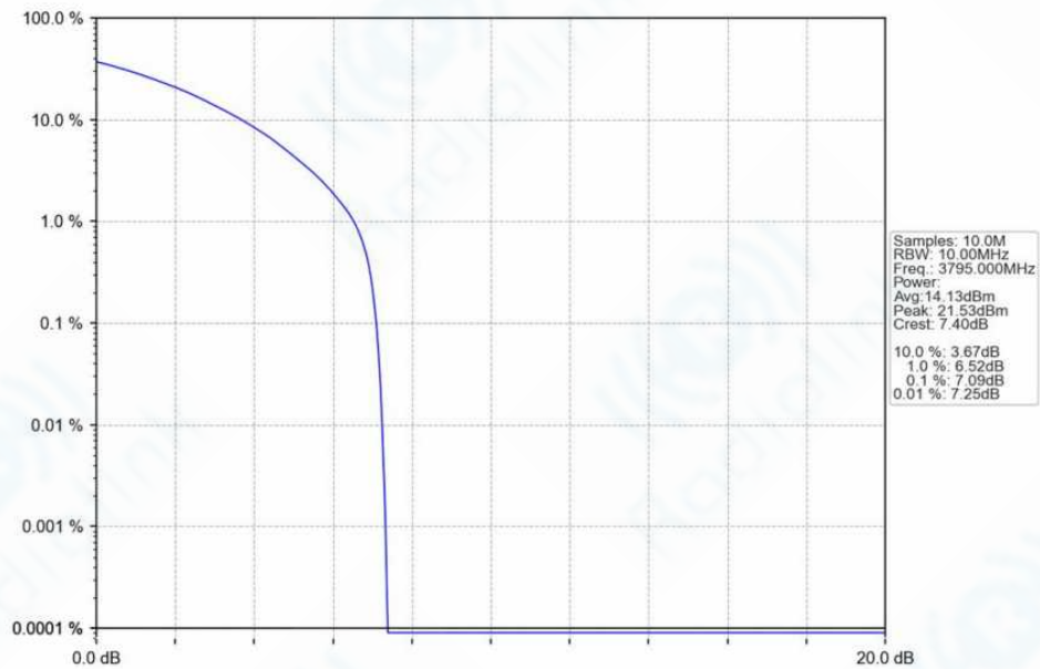
n78f_30kHz_SISO_NTNV_10MHz_CP-OFDM_64_QAM_3795MHz_Outer_Full_Ant1
