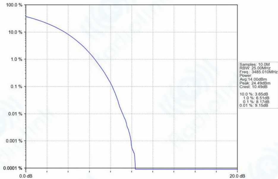
n78f_30kHz_SISO_NTNV_70MHz_CP-OFDM QPSK_3485.01MHz_Outer_Full_Ant1
