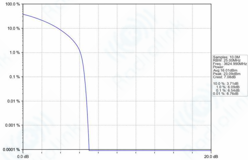
n78f_30kHz_SISO_NTNV_20MHz_CP-OFDM QPSK_3624.99MHz_Outer_Full_Ant1
