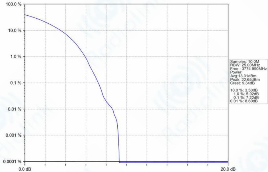
n78f_30kHz_SISO_NTNV_50MHz_DFT-s-OFDM_64_QAM_3774.99MHz_Outer_Full_Ant1
