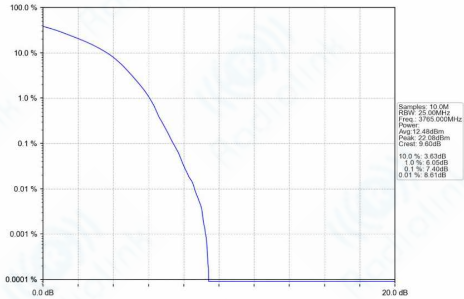
n78f_30kHz_SISO_NTNV_70MHz_DFT-s-OFDM_16_QAM_3765MHz_Outer_Full_Ant1
