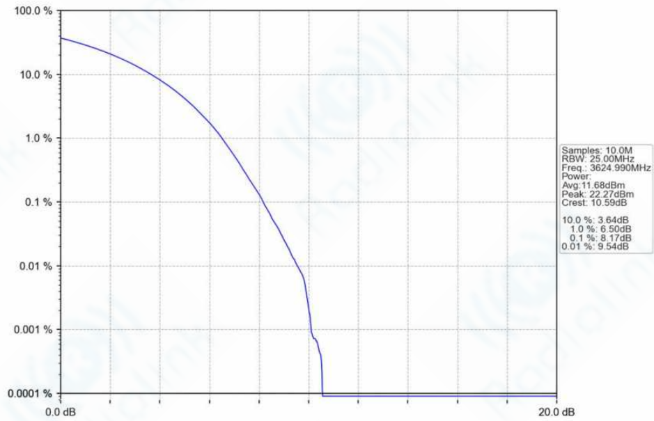
n78f_30kHz_SISO_NTNV_60MHz_CP-OFDM_64_QAM_3624.99MHz_Outer_Full_Ant1
