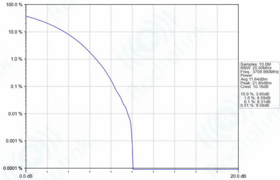
n78f_30kHz_SISO_NTNV_80MHz_CP-OFDM_16_QAM_3759.99MHz_Outer_Full_Ant1
