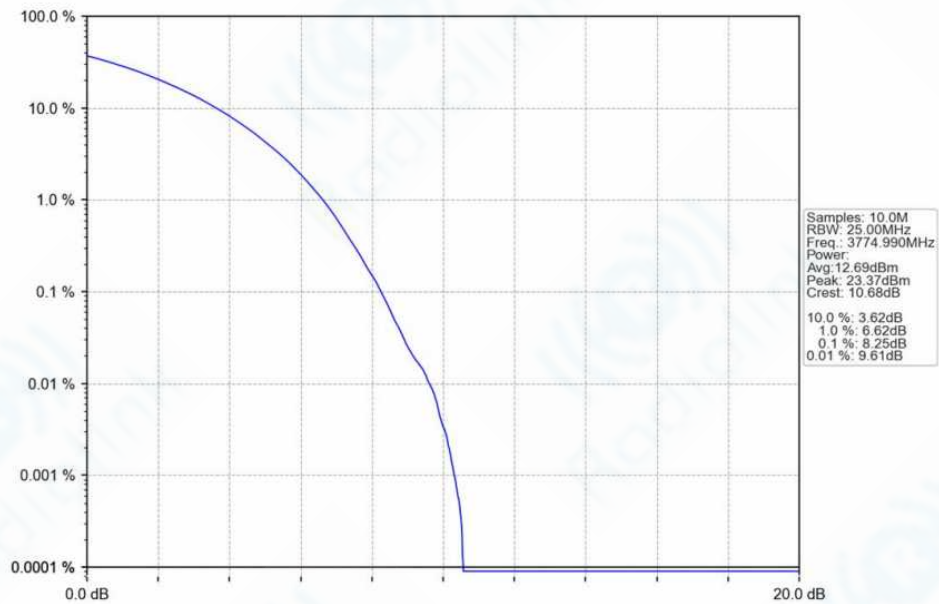
n78f_30kHz_SISO_NTNV_50MHz_CP-OFDM_64_QAM_3774.99MHz_Outer_Full_Ant1
