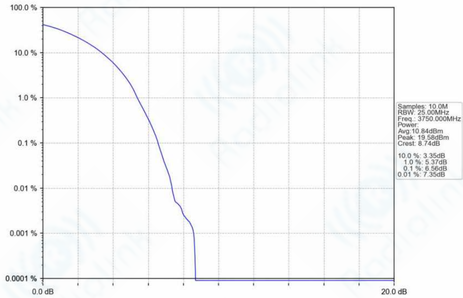
n78f_30kHz_SISO_NTNV_100MHz_DFT-s-OFDM PI/2 BPSK 3750MHz_Outer_Full_Ant1
