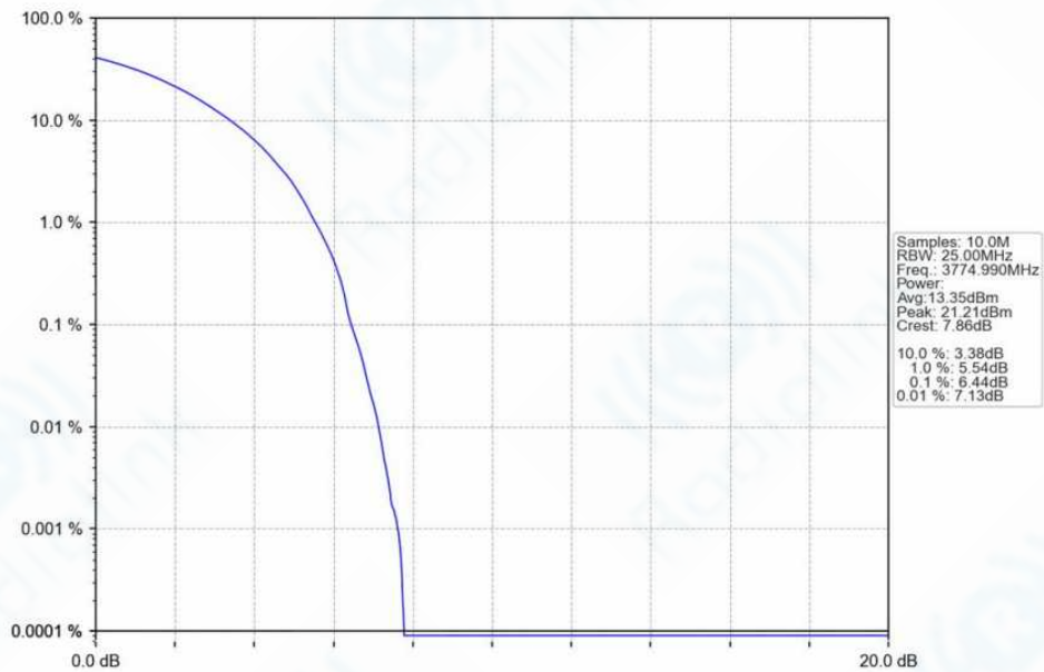
n78f_30kHz_SISO_NTNV_50MHz_DFT-s-OFDM_QPSK_3774.99MHz_Outer_Full_Ant1
