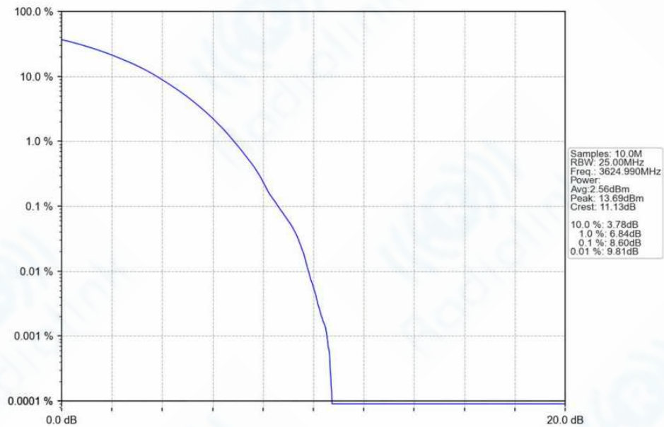
n78f_30kHz_SISO_NTNV_80MHz_CP-OFDM_256_QAM_3624.99MHz_Outer_Full_Ant1
