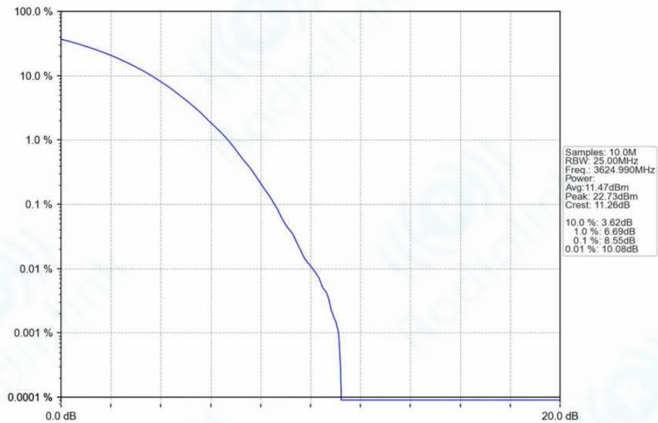
n78f_30kHz_SISO_NTNV_40MHz_CP-OFDM_256_QAM_3624.99MHz_Outer_Full_Ant1
