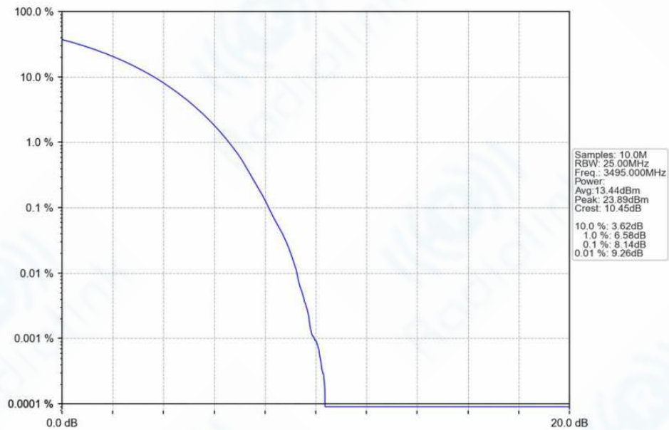
n78f_30kHz_SISO_NTNV_90MHz_CP-OFDM QPSK_3495MHz_Outer_Full_Ant1
