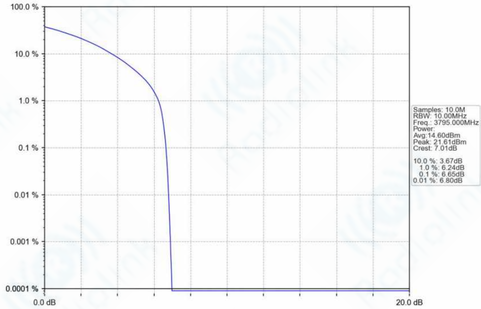
n78f_30kHz_SISO_NTNV_10MHz_CP-OFDM_16_QAM_3795MHz_Outer_Full_Ant1
