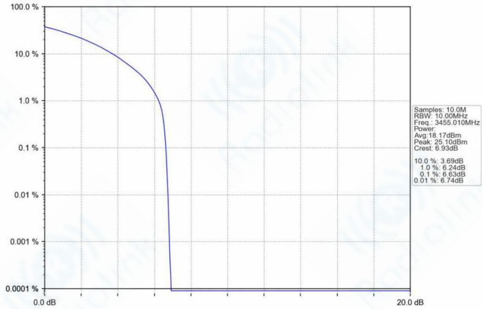
n78f_30kHz_SISO_NTNV_10MHz_CP-OFDM_16_QAM_3455.01MHz_Outer_Full_Ant1
