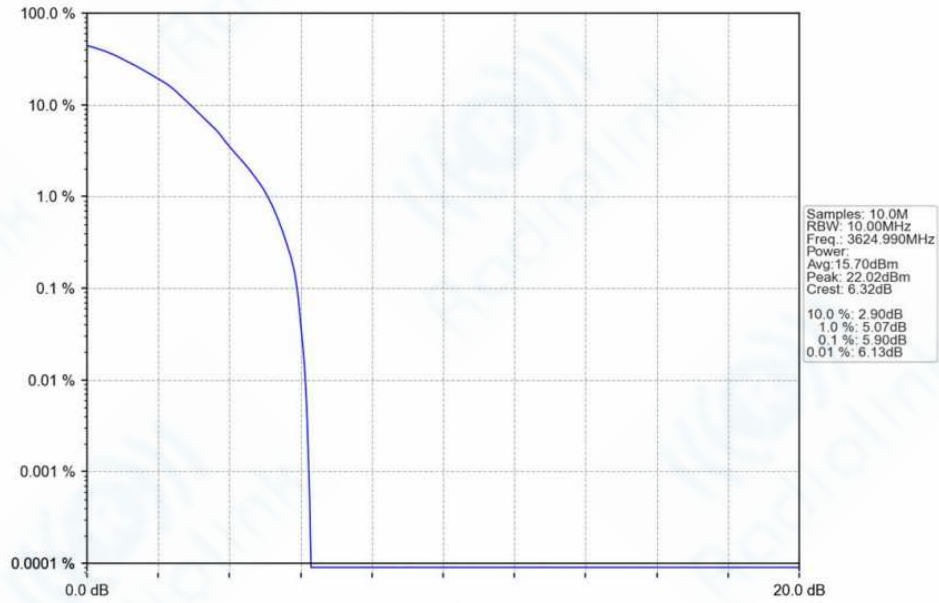
n78f_30kHz_SISO_NTNV_10MHz_DFT-s-OFDM_64_QAM_3624.99MHz_Outer_Full_Ant1
