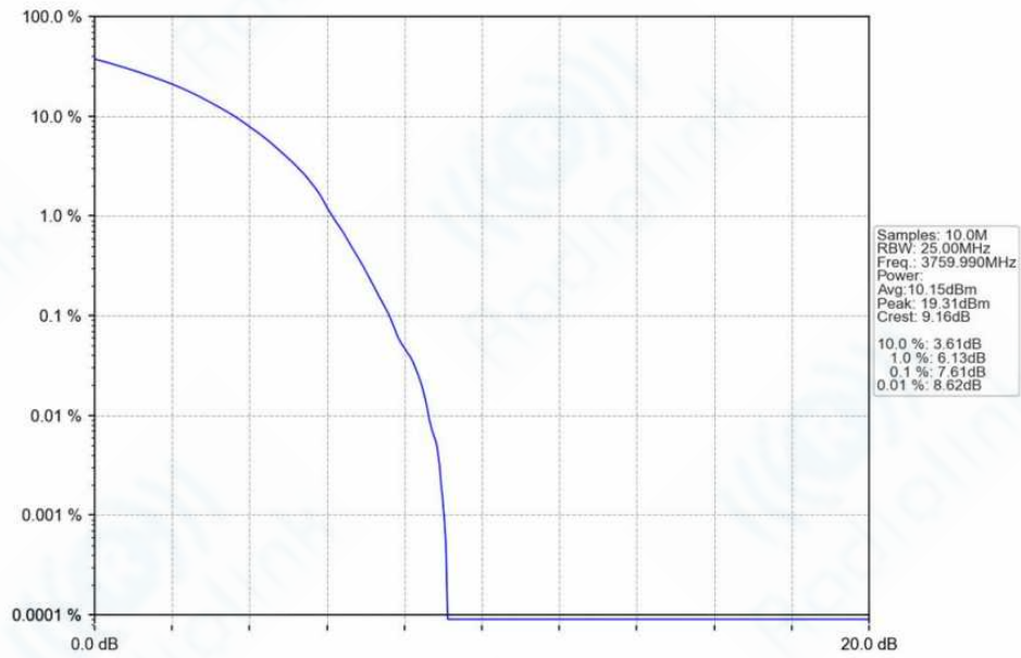
n78f_30kHz_SISO_NTNV_80MHz_DFT-s-OFDM 256 QAM_3759.99MHz_Outer_Full_Ant1
