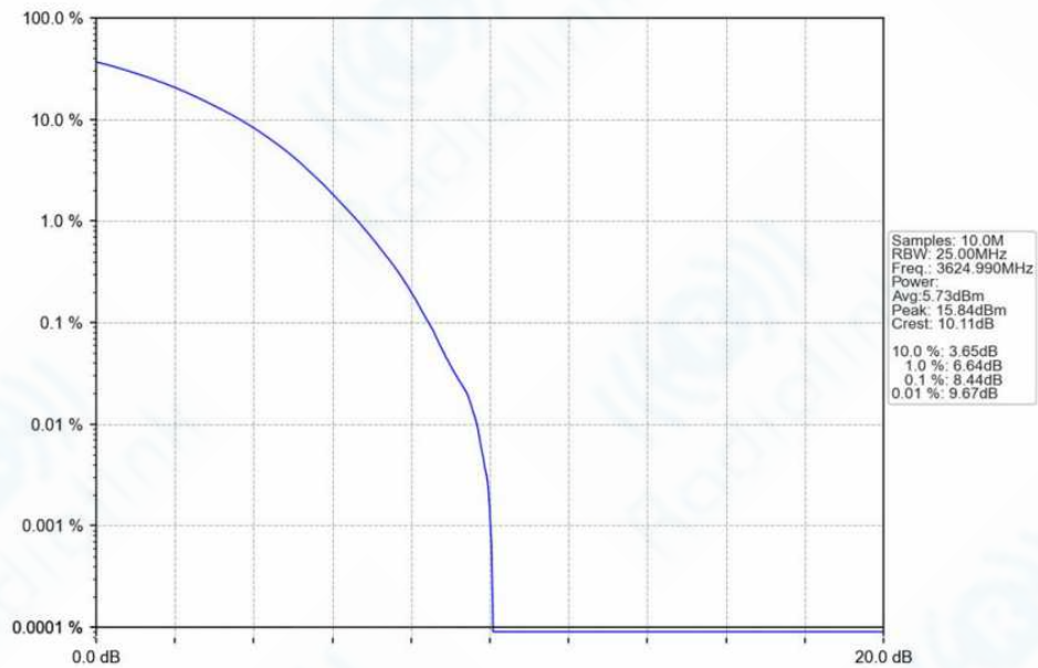
n78f_30kHz_SISO_NTNV_100MHz_CP-OFDM_16_QAM_3624.99MHz_Outer_Full_Ant1
