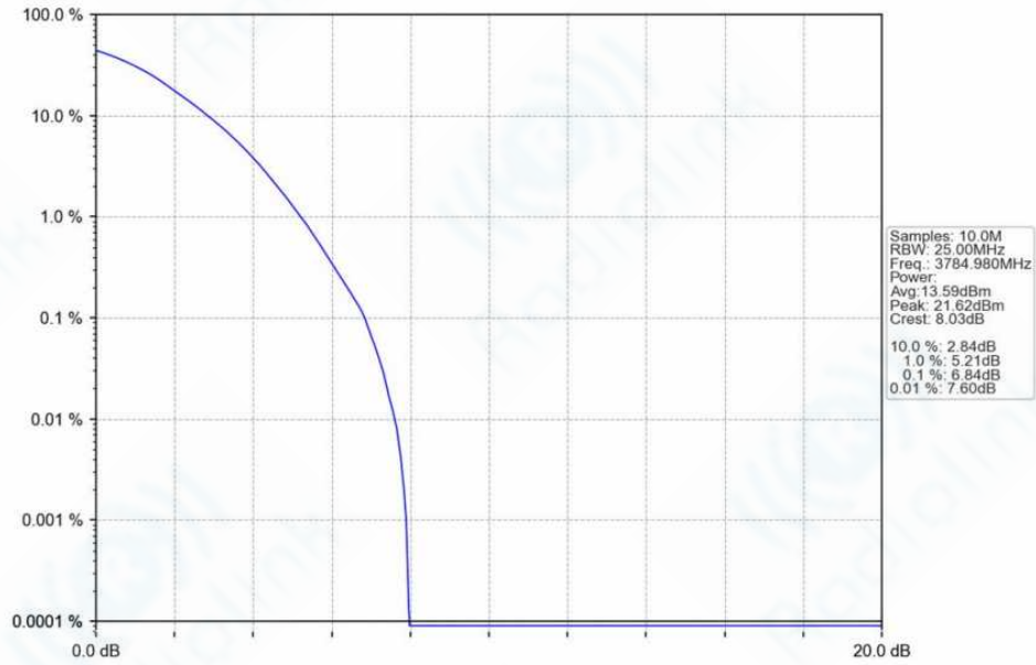
n78f_30kHz_SISO_NTNV_30MHz_DFT-s-OFDM 256 QAM_3784.98MHz_Outer_Full_Ant1
