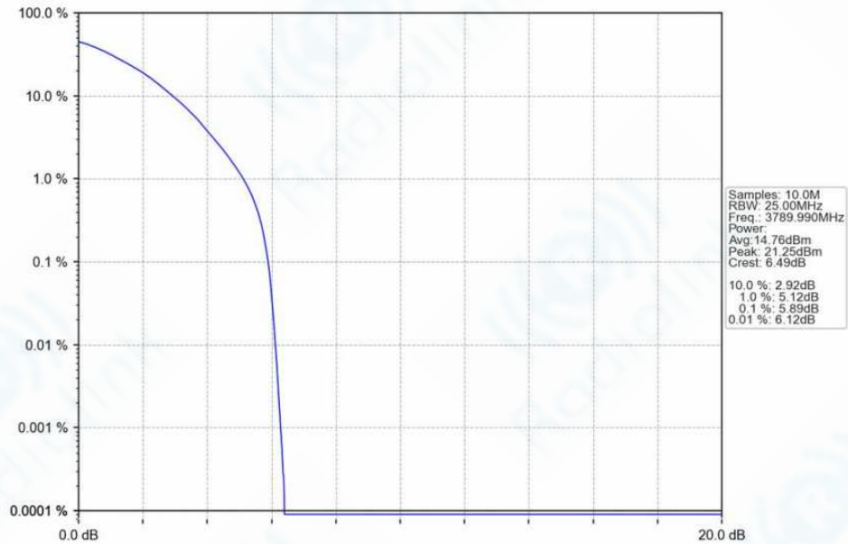
n78f_30kHz_SISO_NTNV_20MHz_DFT-s-OFDM_64_QAM_3789.99MHz_Outer_Full_Ant1
