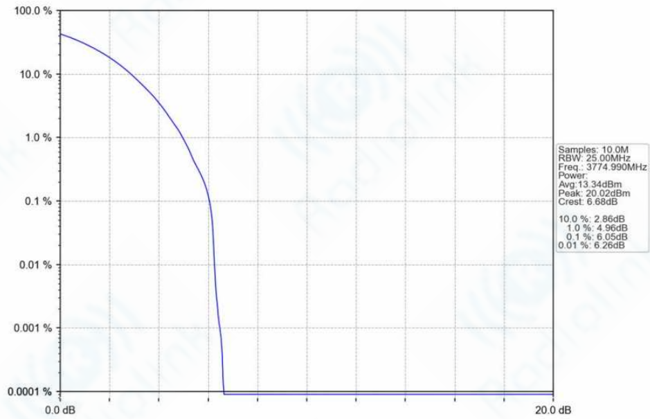
n78f_30kHz_SISO_NTNV_50MHz_DFT-s-OFDM_PI/2_BPSK_3774.99MHz_Outer_Full_Ant1
