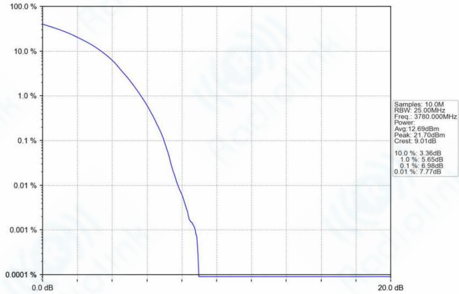
n78f_30kHz_SISO_NTNV_40MHz_DFT-s-OFDM_256_QAM_3780MHz_Outer_Full_Ant1
