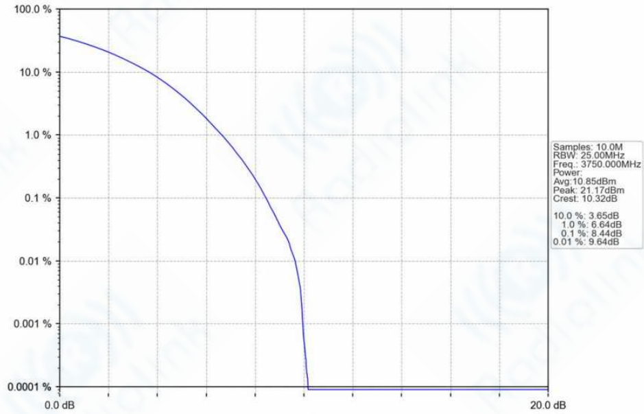
n78f_30kHz_SISO_NTNV_100MHz_CP-OFDM 16 QAM_3750MHz_Outer_Full_Ant1
