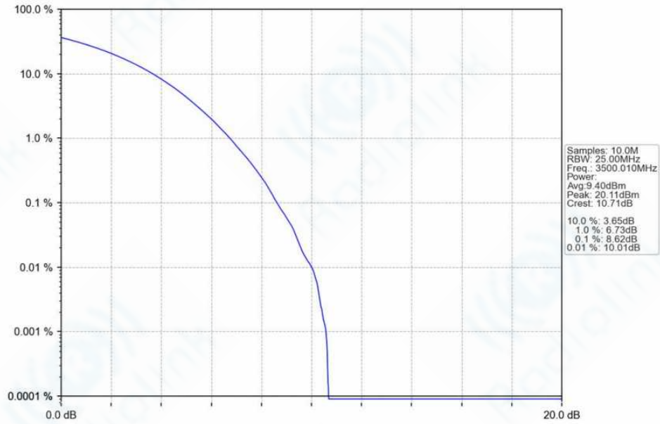
n78f_30kHz_SISO_NTNV_100MHz_CP-OFDM_256_QAM_3500.01MHz_Outer_Full_Ant1
