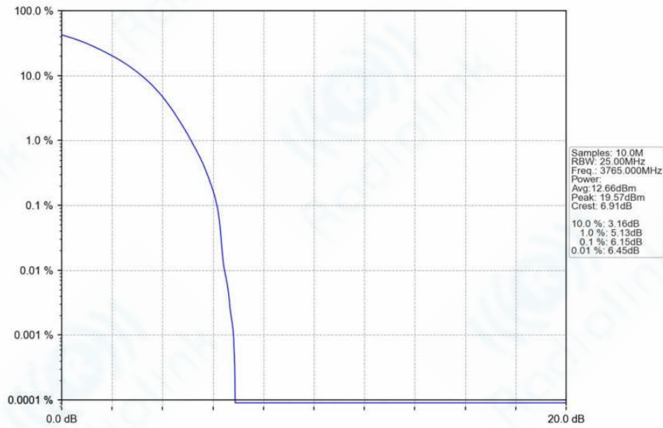
n78f_30kHz_SISO_NTNV_70MHz_DFT-s-OFDM_PI/2_BPSK_3765MHz_Outer_Full_Ant1
