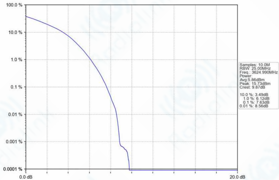
n78f_30kHz_SISO_NTNV_90MHz_DFT-s-OFDM_16_QAM_3624.99MHz_Outer_Full_Ant1
