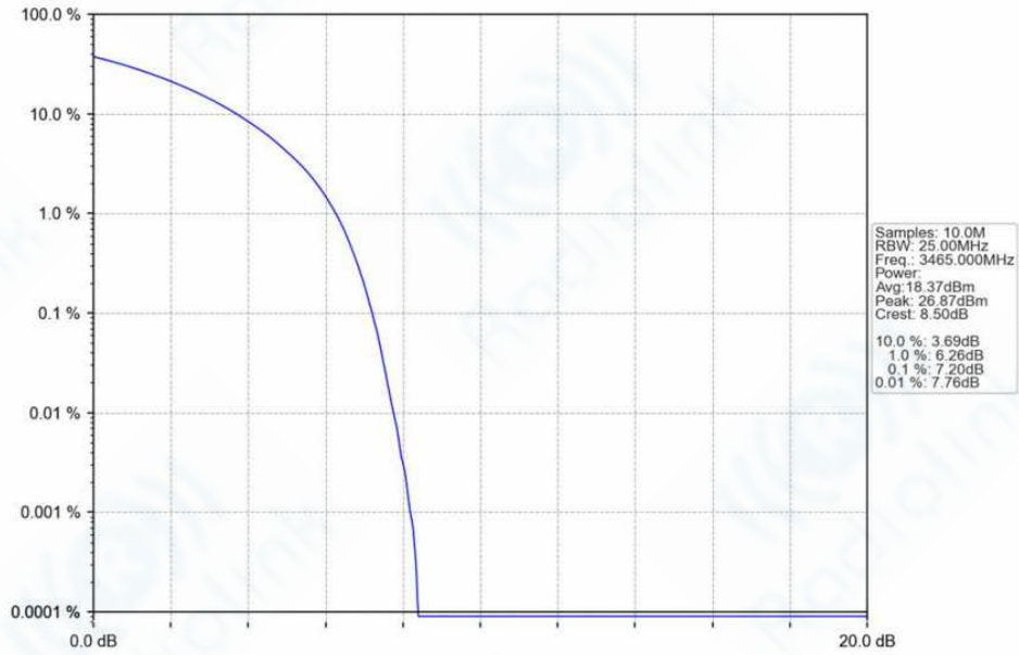
n78f_30kHz_SISO_NTNV_30MHz_CP-OFDM_16_QAM_3465MHz_Outer_Full_Ant1
