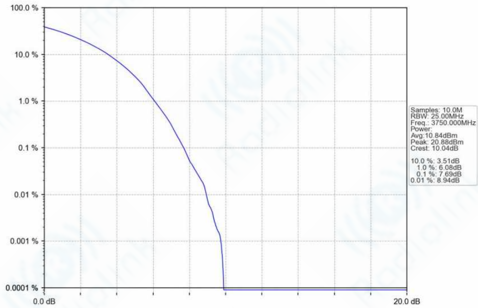
n78f_30kHz_SISO_NTNV_100MHz_DFT-s-OFDM 16 QAM_3750MHz_Outer_Full_Ant1
