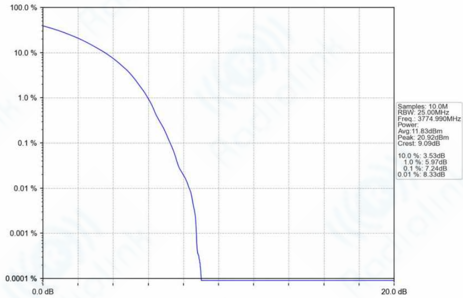
n78f_30kHz_SISO_NTNV_50MHz_DFT-s-OFDM 256 QAM_3774.99MHz_Outer_Full_Ant1
