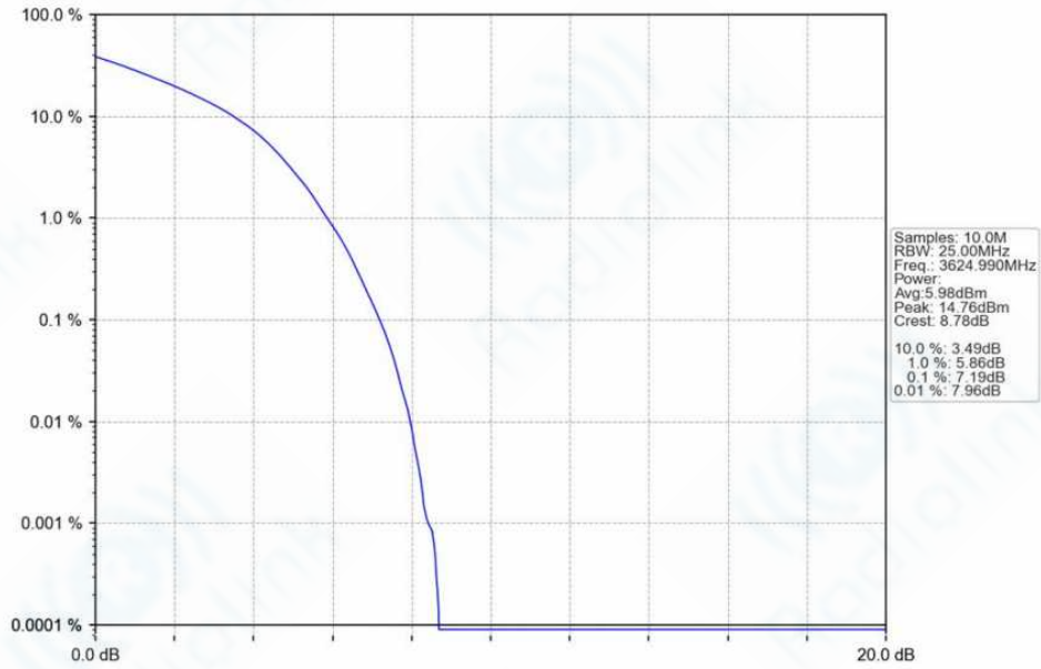
n78f_30kHz_SISO_NTNV_90MHz_DFT-s-OFDM_QPSK_3624.99MHz_Outer_Full_Ant1
