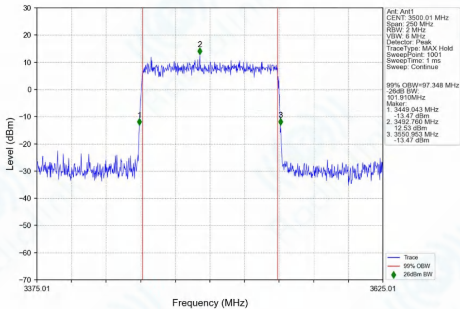
n78f_30kHz_SISO_NTNV_100MHz_CP-OFDM 64 QAM_3500.01MHz_Outer_Full_Ant1
