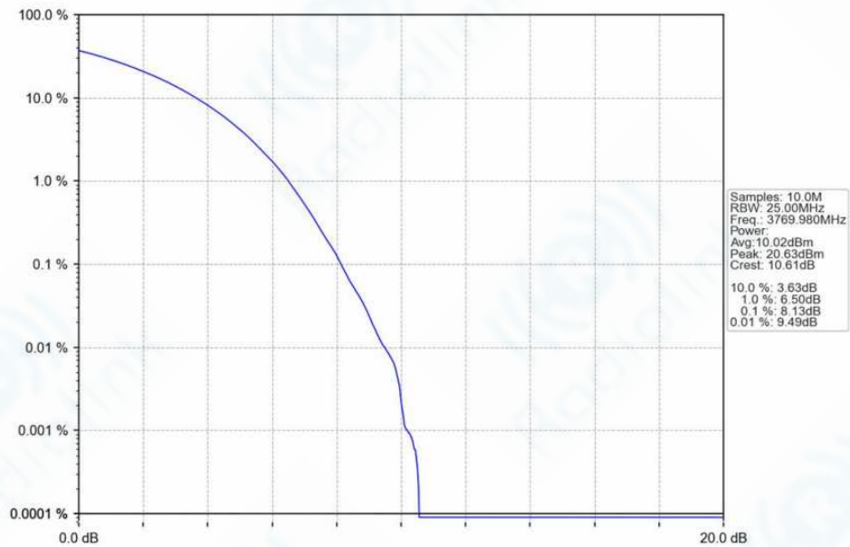
n78f_30kHz_SISO_NTNV_60MHz_CP-OFDM_64_QAM_3769.98MHz_Outer_Full_Ant1
