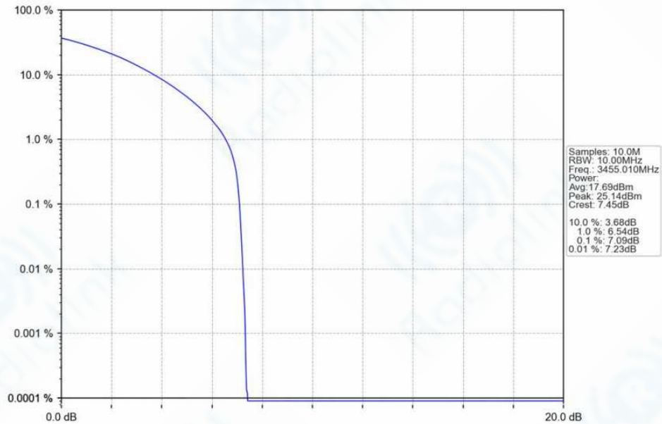
n78f_30kHz_SISO_NTNV_10MHz_CP-OFDM_64_QAM_3455.01MHz_Outer_Full_Ant1
