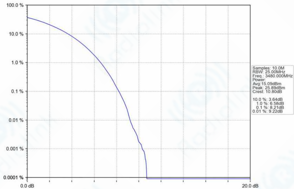
n78f_30kHz_SISO_NTNV_60MHz_CP-OFDM QPSK_3480MHz_Outer_Full_Ant1
