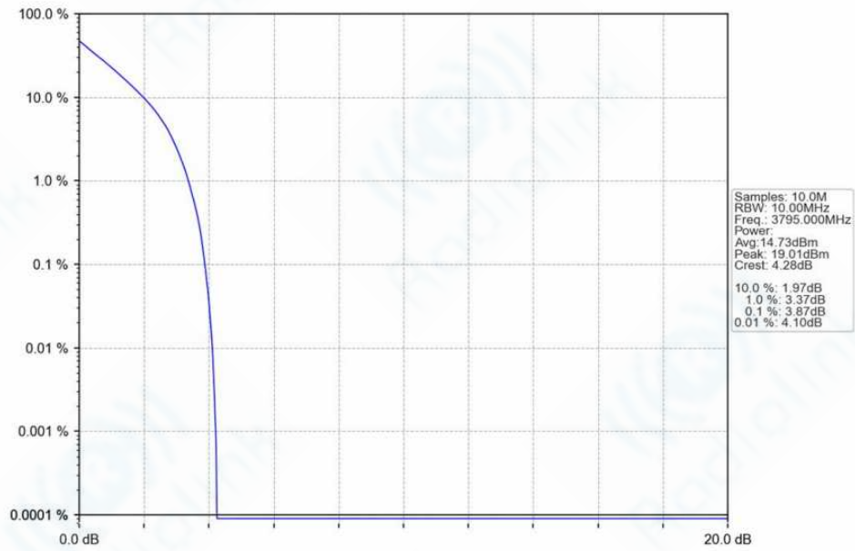
n78f_30kHz_SISO_NTNV_10MHz_DFT-s-OFDM_PI/2_BPSK_3795MHz_Outer_Full_Ant1
