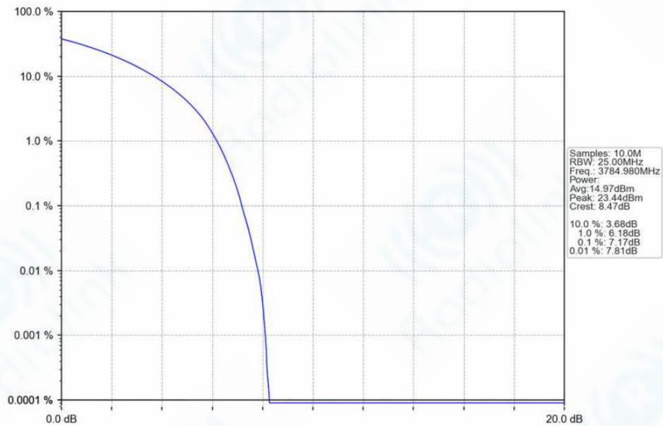
n78f_30kHz_SISO_NTNV_30MHz_CP-OFDM QPSK_3784.98MHz_Outer_Full_Ant1
