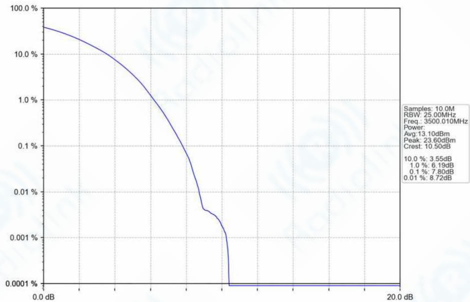
n78f_30kHz_SISO_NTNV_100MHz_DFT-s-OFDM 64 QAM_3500.01MHz_Outer_Full_Ant1
