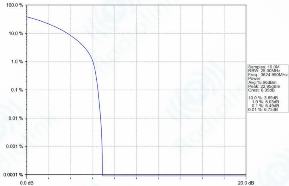
n78f_30kHz_SISO_NTNV_20MHz_CP-OFDM_16_QAM_3624.99MHz_Outer_Full_Ant1
