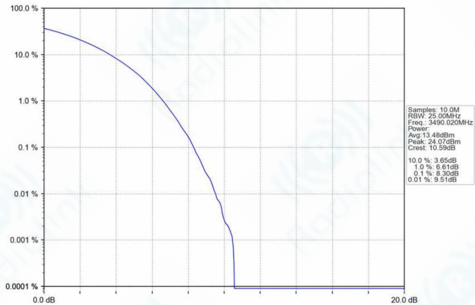
n78f_30kHz_SISO_NTNV_80MHz_CP-OFDM_64_QAM_3490.02MHz_Outer_Full_Ant1
