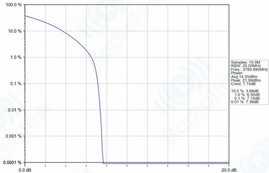
n78f_30kHz_SISO_NTNV_20MHz_CP-OFDM_64_QAM_3789.99MHz_Outer_Full_Ant1
