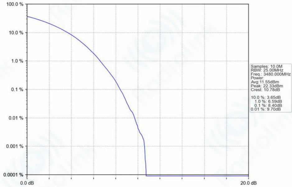
n78f_30kHz_SISO_NTNV_60MHz_CP-OFDM_256_QAM_3480MHz_Outer_Full_Ant1
