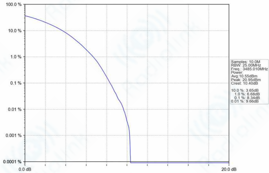
n78f_30kHz_SISO_NTNV_70MHz_CP-OFDM_256_QAM_3485.01MHz_Outer_Full_Ant1
