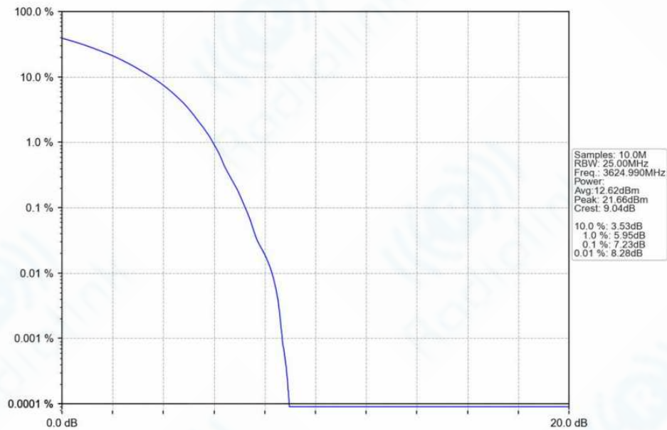
n78f_30kHz_SISO_NTNV_50MHz_DFT-s-OFDM_256_QAM_3624.99MHz_Outer_Full_Ant1
