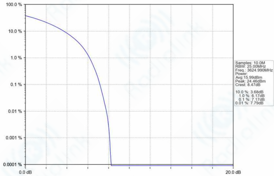
n78f_30kHz_SISO_NTNV_30MHz_CP-OFDM QPSK_3624.99MHz_Outer_Full_Ant1
