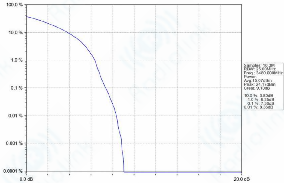
n78f_30kHz_SISO_NTNV_60MHz_DFT-s-OFDM_16_QAM_3480MHz_Outer_Full_Ant1
