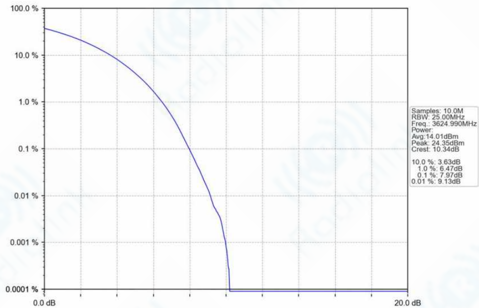
n78f_30kHz_SISO_NTNV_50MHz_CP-OFDM_16_QAM_3624.99MHz_Outer_Full_Ant1
