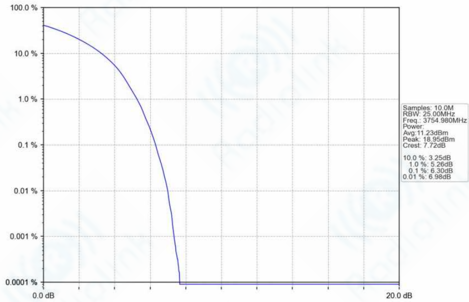
n78f_30kHz_SISO_NTNV_90MHz_DFT-s-OFDM PI/2 BPSK_3754.98MHz_Outer_Full_Ant1
