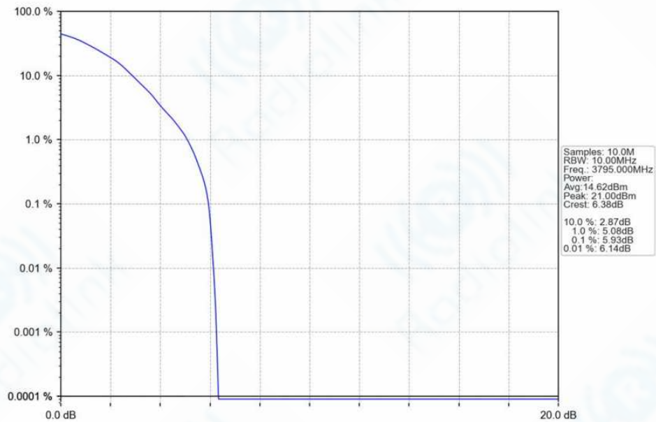
n78f_30kHz_SISO_NTNV_10MHz_DFT-s-OFDM_64_QAM_3795MHz_Outer_Full_Ant1
