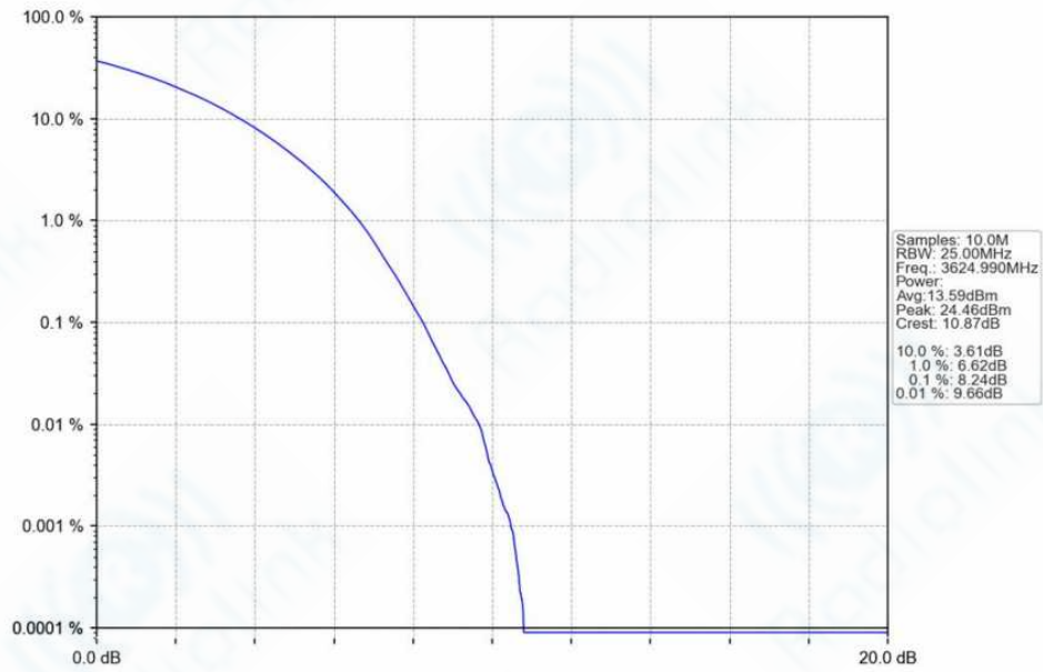
n78f_30kHz_SISO_NTNV_50MHz_CP-OFDM_64_QAM_3624.99MHz_Outer_Full_Ant1
