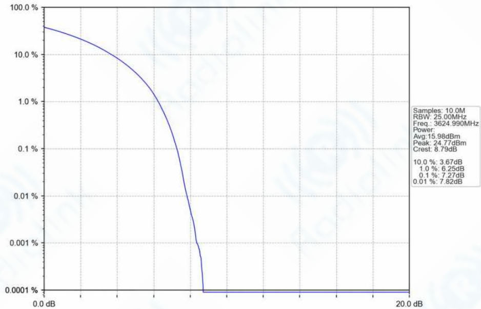
n78f_30kHz_SISO_NTNV_30MHz_CP-OFDM_16_QAM_3624.99MHz_Outer_Full_Ant1
