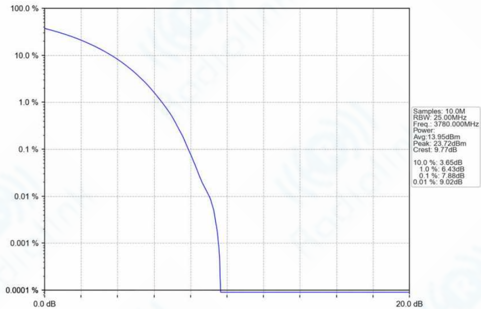
n78f_30kHz_SISO_NTNV_40MHz_CP-OFDM_QPSK_3780MHz_Outer_Full_Ant1
