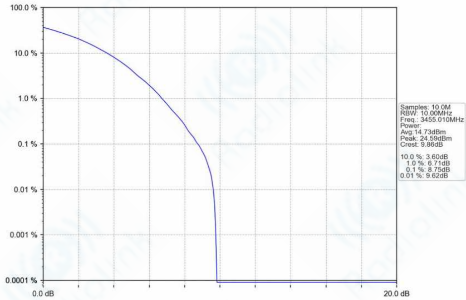
n78f_30kHz_SISO_NTNV_10MHz_CP-OFDM_256_QAM_3455.01MHz_Outer_Full_Ant1
