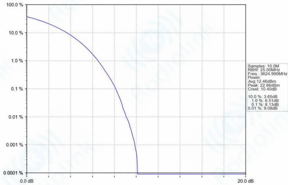
n78f_30kHz_SISO_NTNV_70MHz_CP-OFDM QPSK_3624.99MHz_Outer_Full_Ant1
