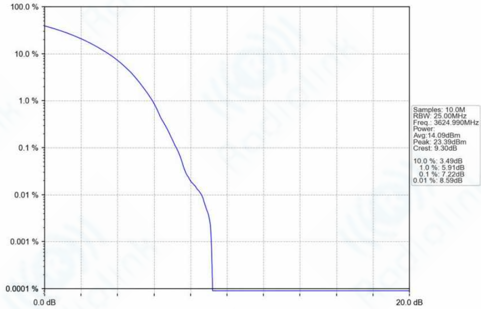
n78f_30kHz_SISO_NTNV_50MHz_DFT-s-OFDM_64_QAM_3624.99MHz_Outer_Full_Ant1
