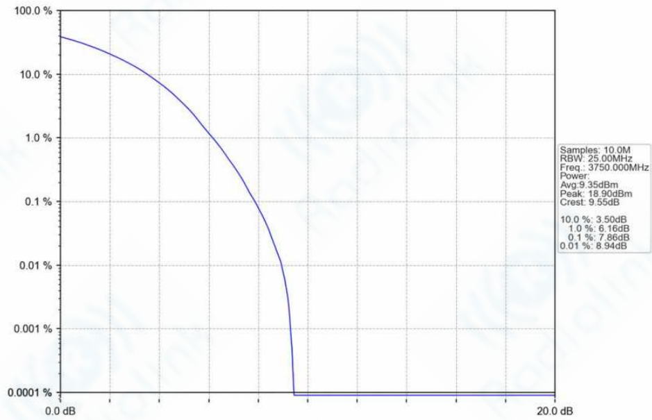
n78f_30kHz_SISO_NTNV_100MHz_DFT-s-OFDM_256_QAM_3750MHz_Outer_Full_Ant1
