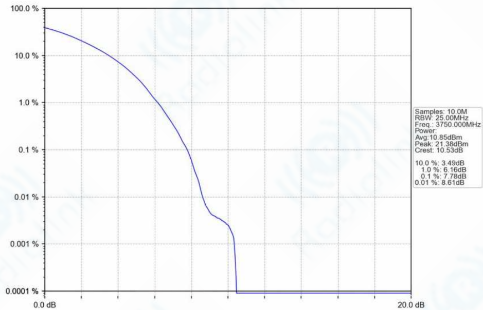
n78f_30kHz_SISO_NTNV_100MHz_DFT-s-OFDM 64 QAM_3750MHz_Outer_Full_Ant1
