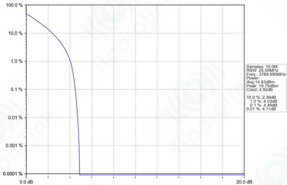
n78f_30kHz_SISO_NTNV_20MHz_DFT-s-OFDM_QPSK_3789.99MHz_Outer_Full_Ant1
