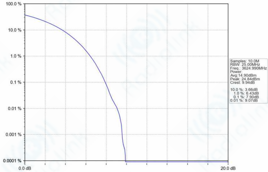
n78f_30kHz_SISO_NTNV_40MHz_CP-OFDM_QPSK_3624.99MHz_Outer_Full_Ant1
