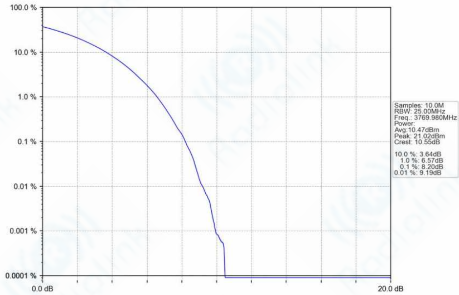
n78f_30kHz_SISO_NTNV_60MHz_CP-OFDM 16 QAM_3769.98MHz_Outer_Full_Ant1
