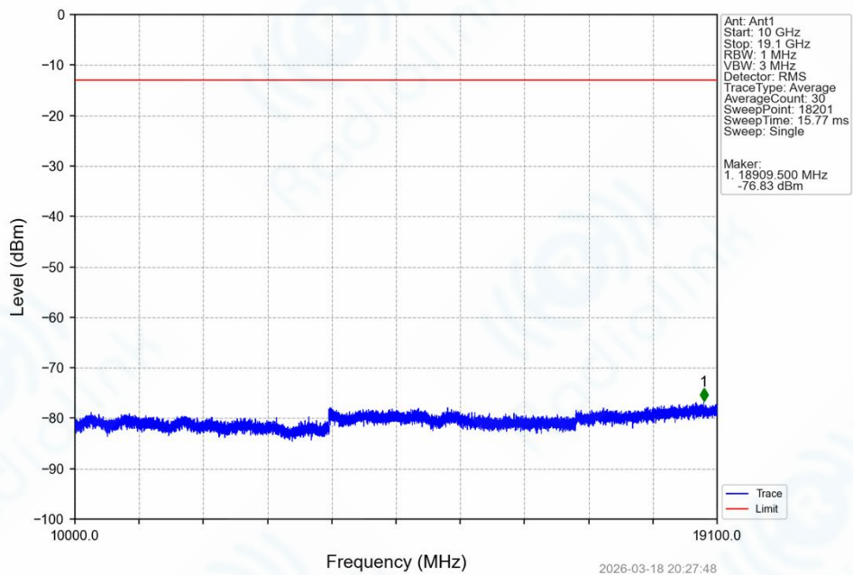
Band2_RMC_HCH_1907.6MHz_12.2kbps RMC_NTNV
