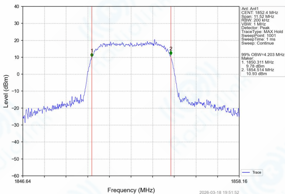
Band2_HSUPA_LCH_1852.4MHz_Subtest 1_NTNV
