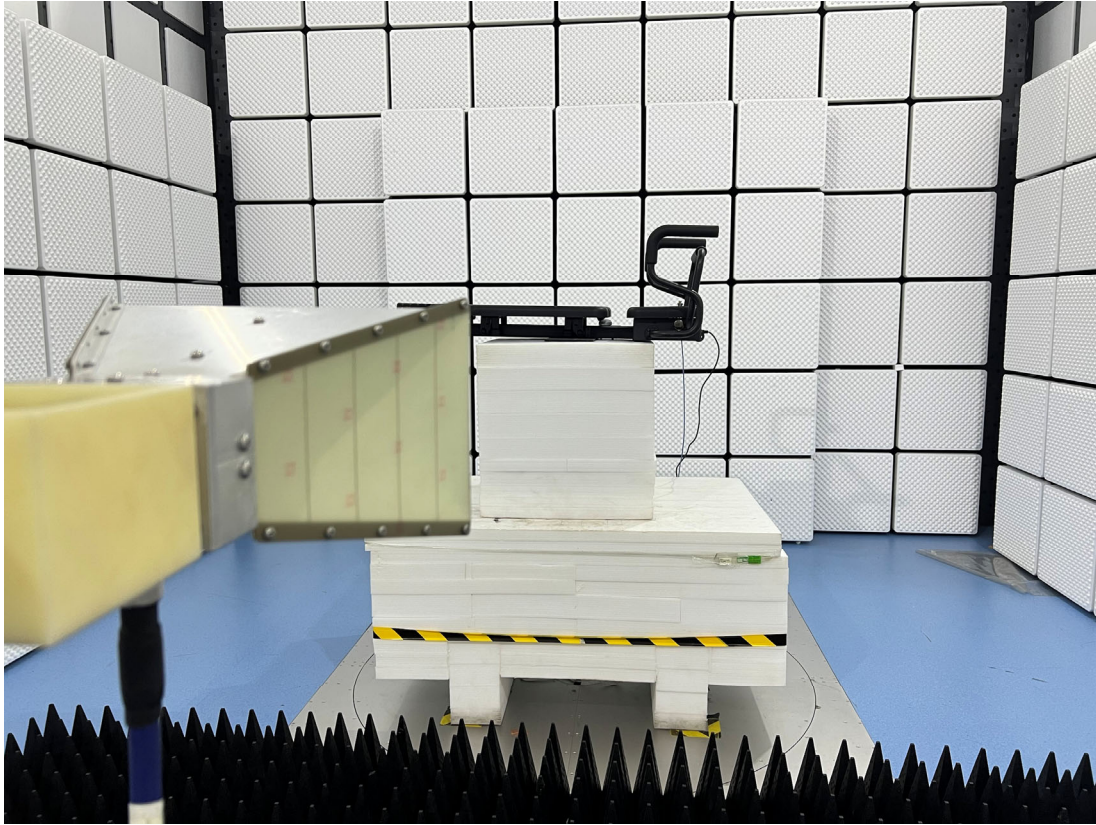
RE – Front View (18 GHz~25 GHz)
