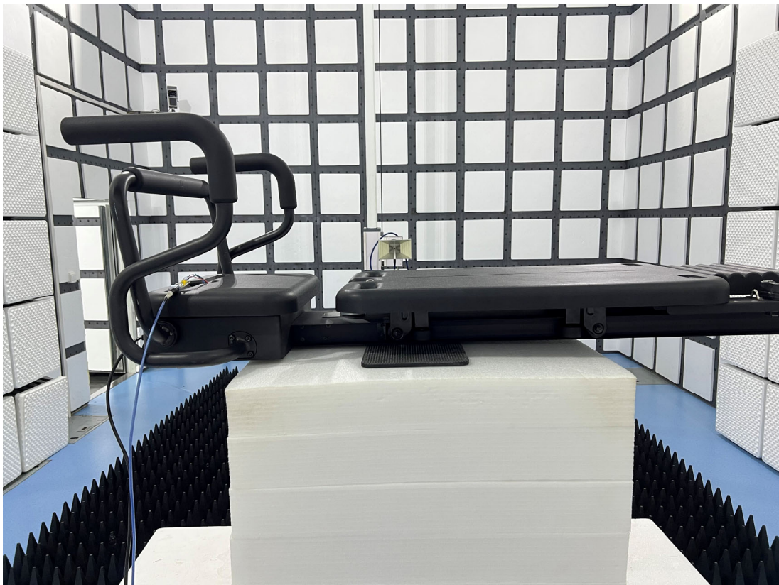
RE – Front View (1 GHz~18 GHz)
