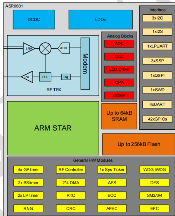
fig 1 Chip architecture
