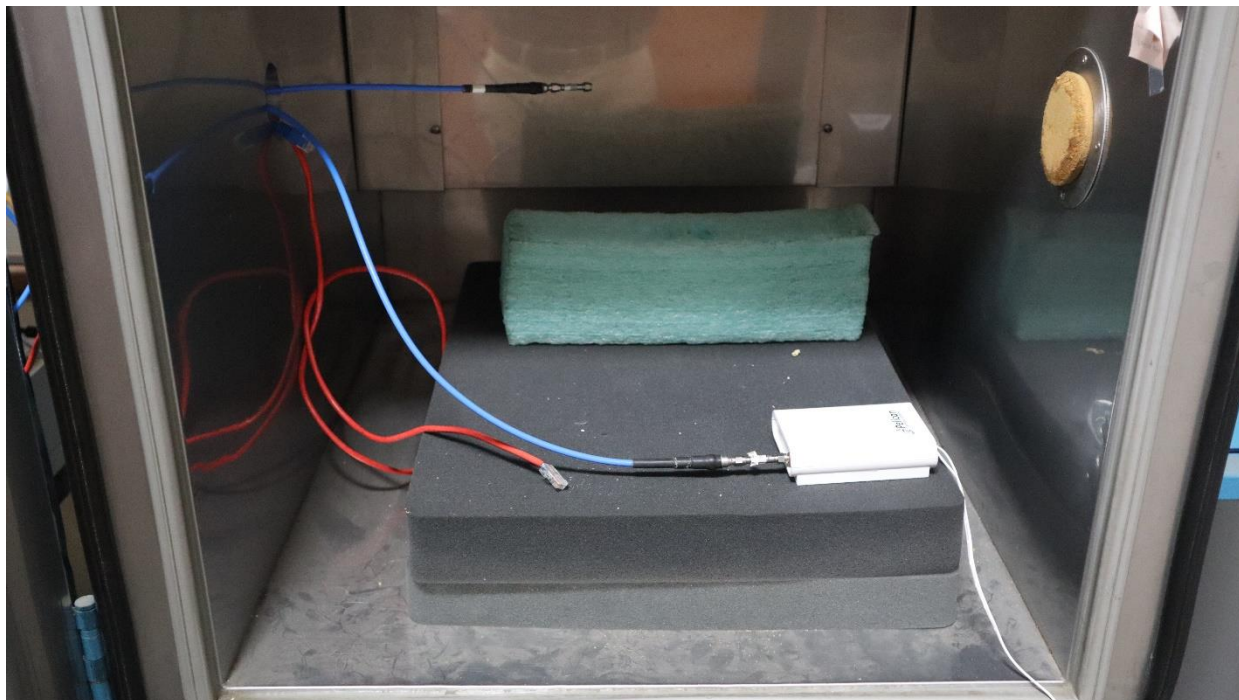
PELC01 915MHz Module RF Conducted
