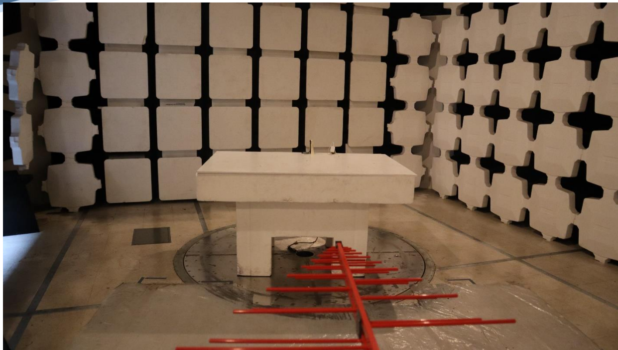
PELC01 915MHz Module Radiated Emissions 30MHz-1GHz
