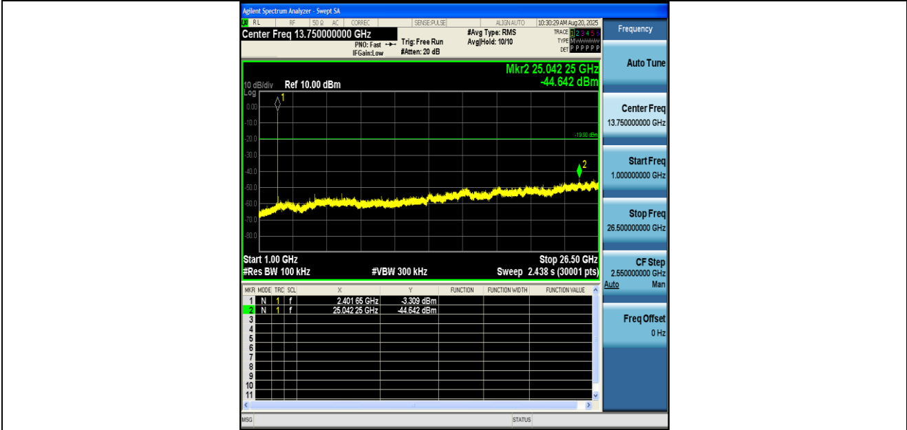
SRD-Ant1-2402-1000~26500-PASS
