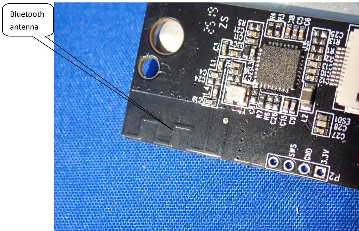
Internal Photo 9
