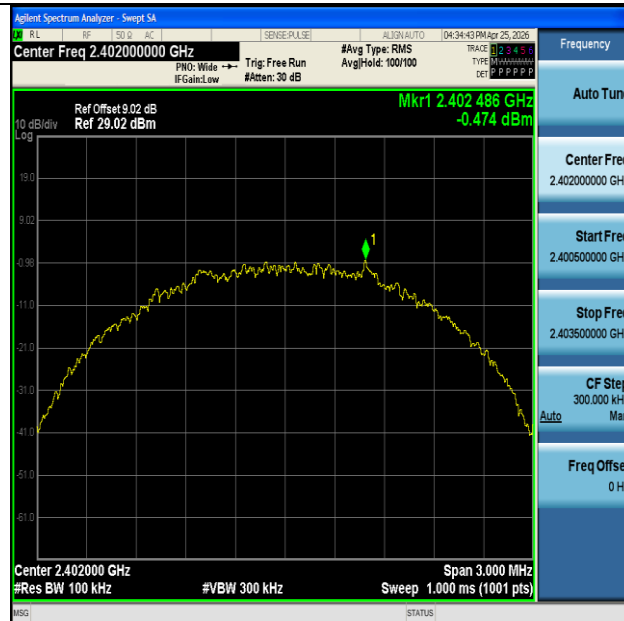
SRD-Ant1-2402-0~Reference-PASS
