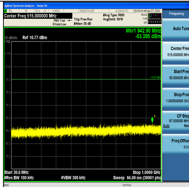
BLE_1M-Ant1-2480-30~1000-PASS
