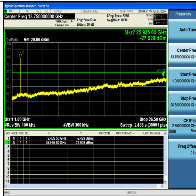
SRD-Ant1-2402-1000~26500-PASS
