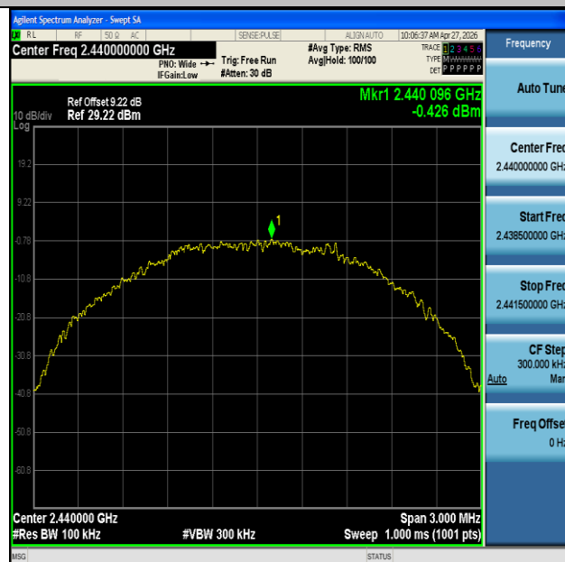
SRD-Ant1-2440-0~Reference-PASS
