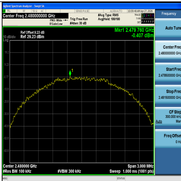
SRD-Ant1-2480-0~Reference-PASS
