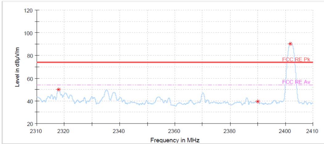
Lowest Channel (2 402 MHz)_Peak
