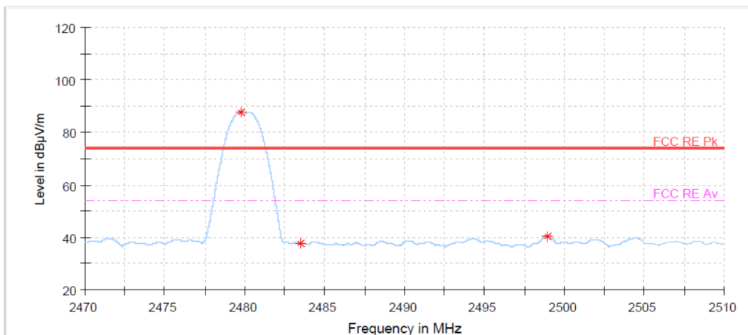
Highest Channel (2 480 MHz)_Peak
