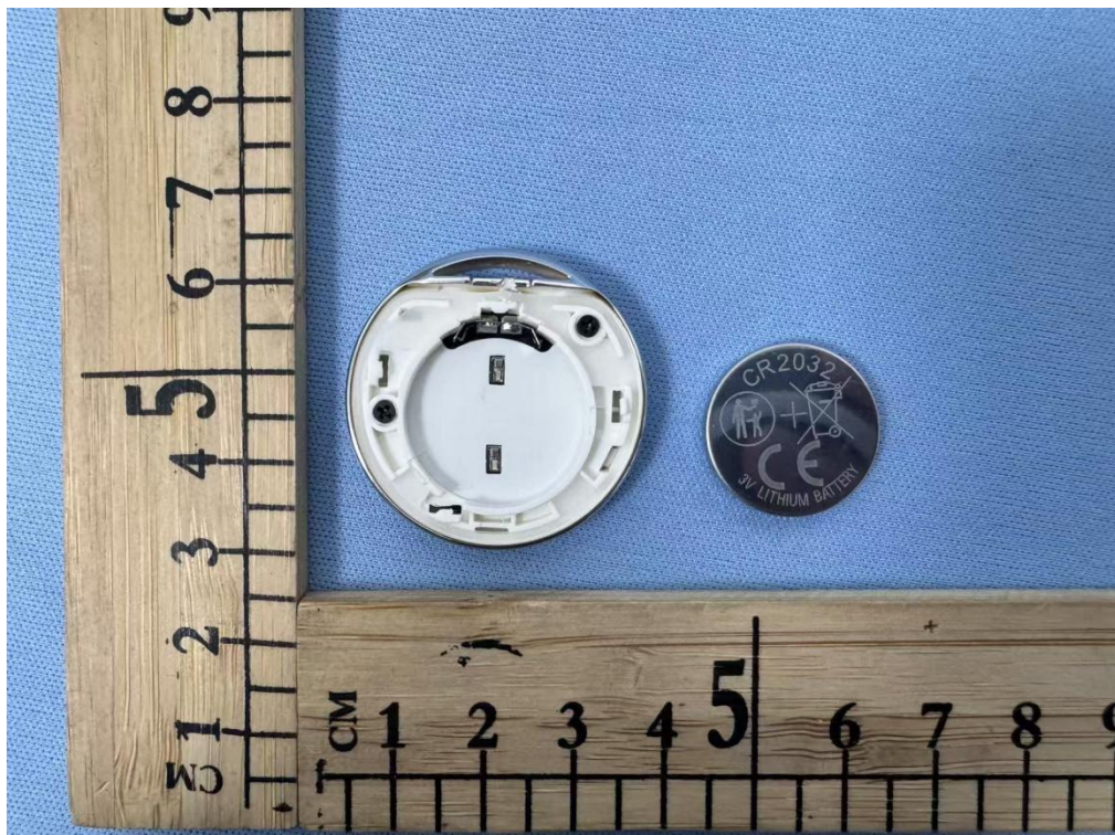
Internal Photos (Model:TX12)
