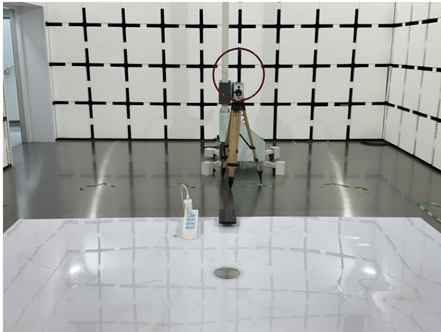
Radiation (9KHz-30MHz)
