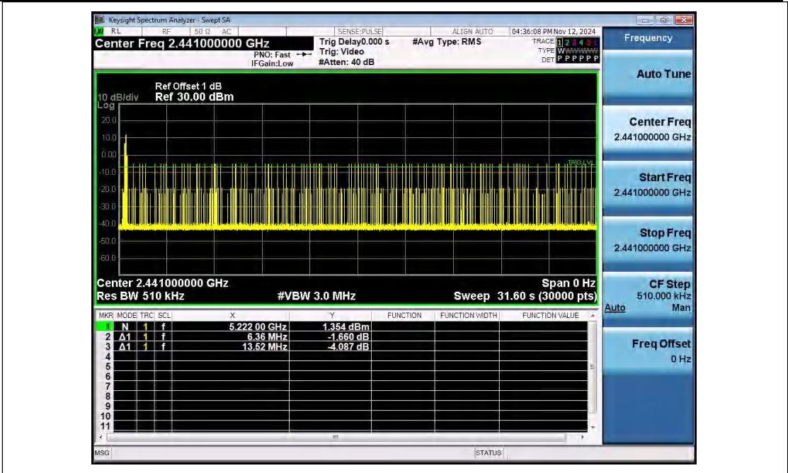
Dwell_Time_(Hopping)_NVNT_ANT1_3-DH3_2441_00_One_Burst_Time
