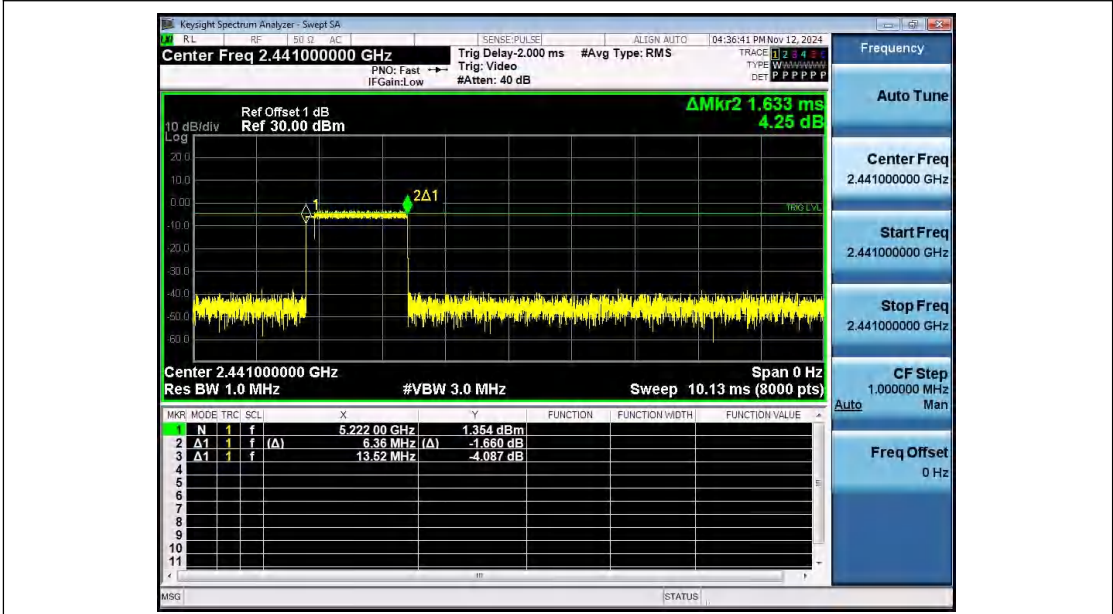
Dwell_Time_(Hopping)_NVNT_ANT1_3-DH3_2441_00_Accumulated
