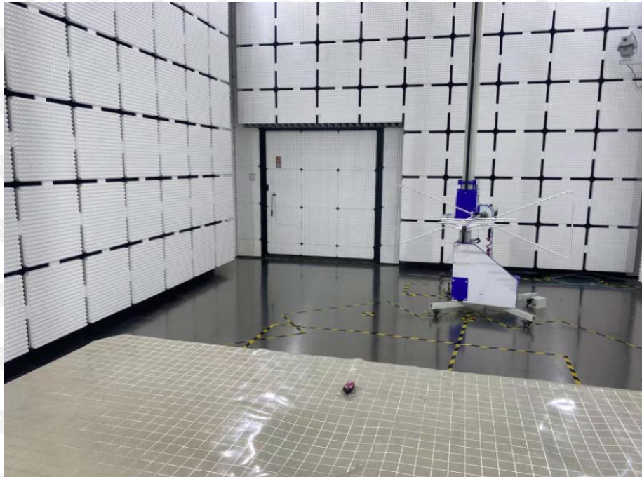
Below 1GHz
