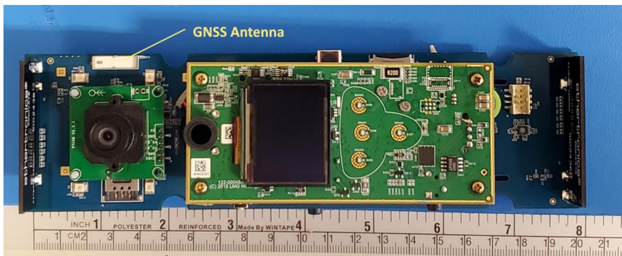
Circuit Board Stack + Battery (Top):
