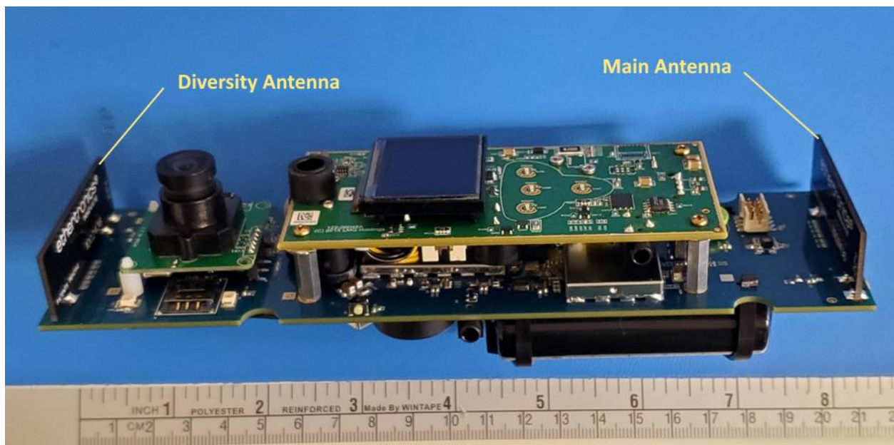
Circuit Board Stack + Battery (Side):
