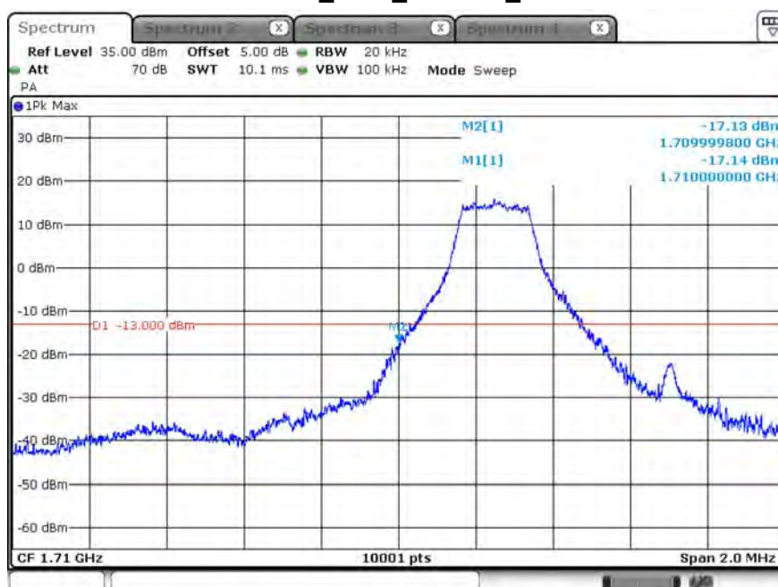
CH19957_1.4M_16-QAM_1RB0
