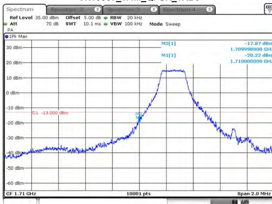
CH19957_1.4M_QPSK_1RB0
