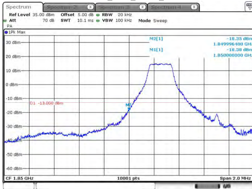
CH18607_1.4M_QPSK_1RB0
