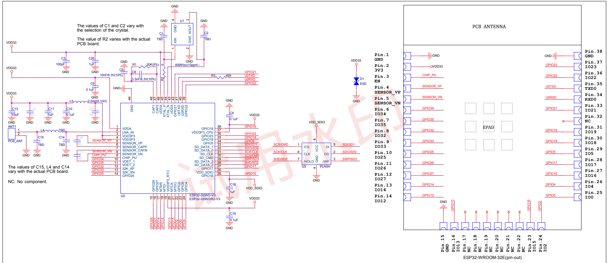
Figure 5: ESP32-WROOM-32E Schematics
