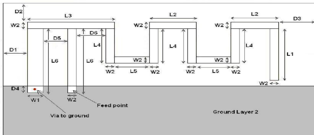
Figure 3: Antenna Dimensions
