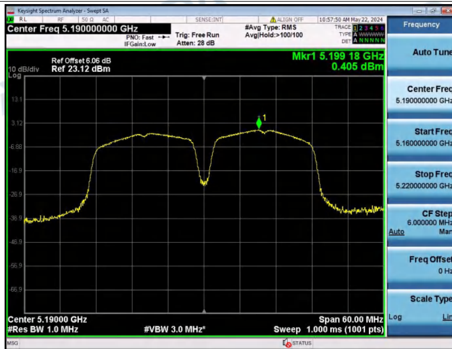
Power_Spectral_Density_NVNT_ANT1_802_11ac(VHT40)_5190
