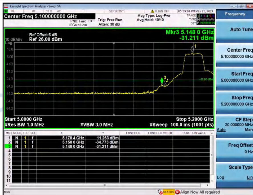
Bandedge_NVNT_ANT1_802_11n(HT20)_5180
