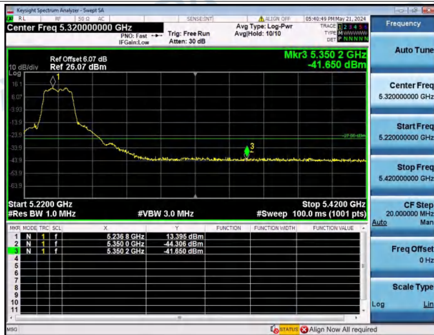
Bandedge_NVNT_ANT1_802_11a_5240
